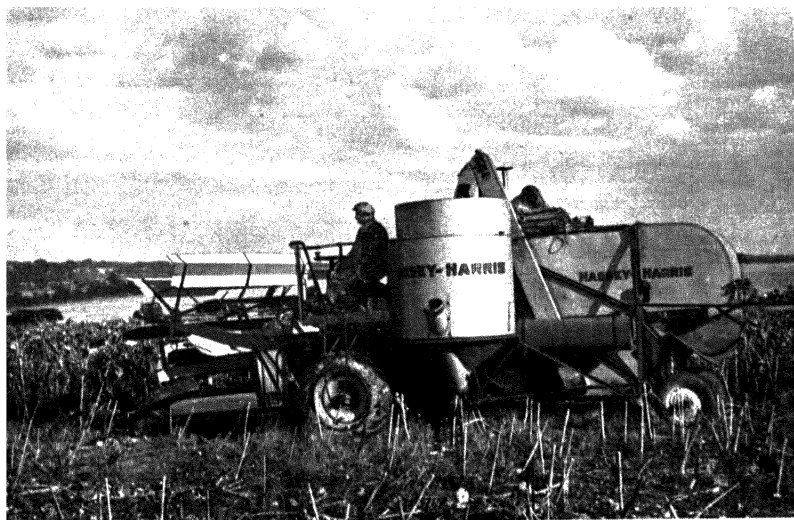
11 (b). Massey-Harris Self-Propelled Combine, harvesting sunflowers at Stoke Charity, Hants, 1944
