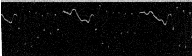
FIG. 3.—WAVE-FORM OF CLARINET: UPPER REGISTER.
