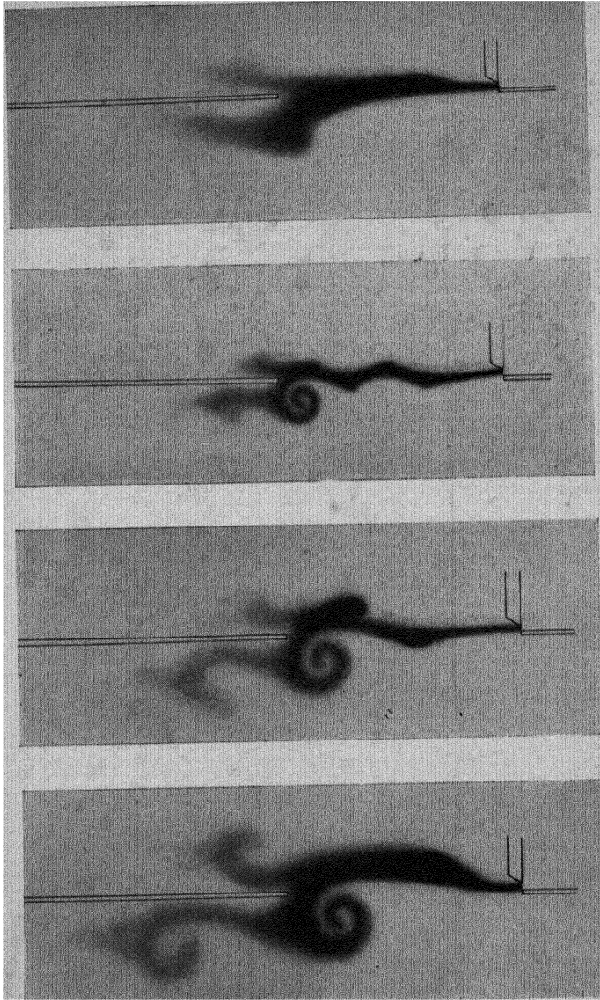
FORMATION OF EDDIES IN AN EDGE-TONE, II (after Carrère).
