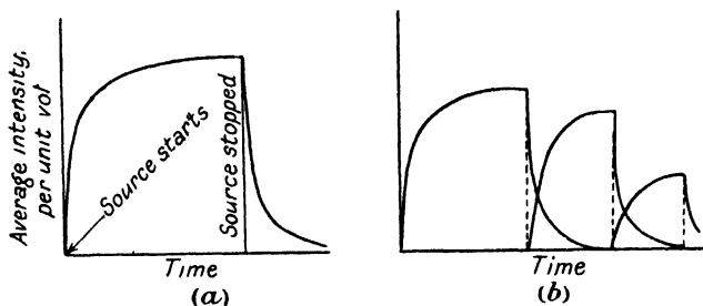
FIG. 27.—Rise and Fall of Loudness in an Auditorium.
