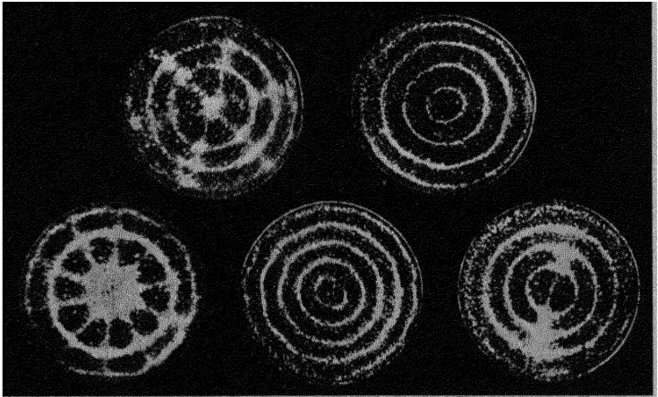
FIG. 2.—SAND FIGURES ON VIBRATING PLATE (after Schulze).
