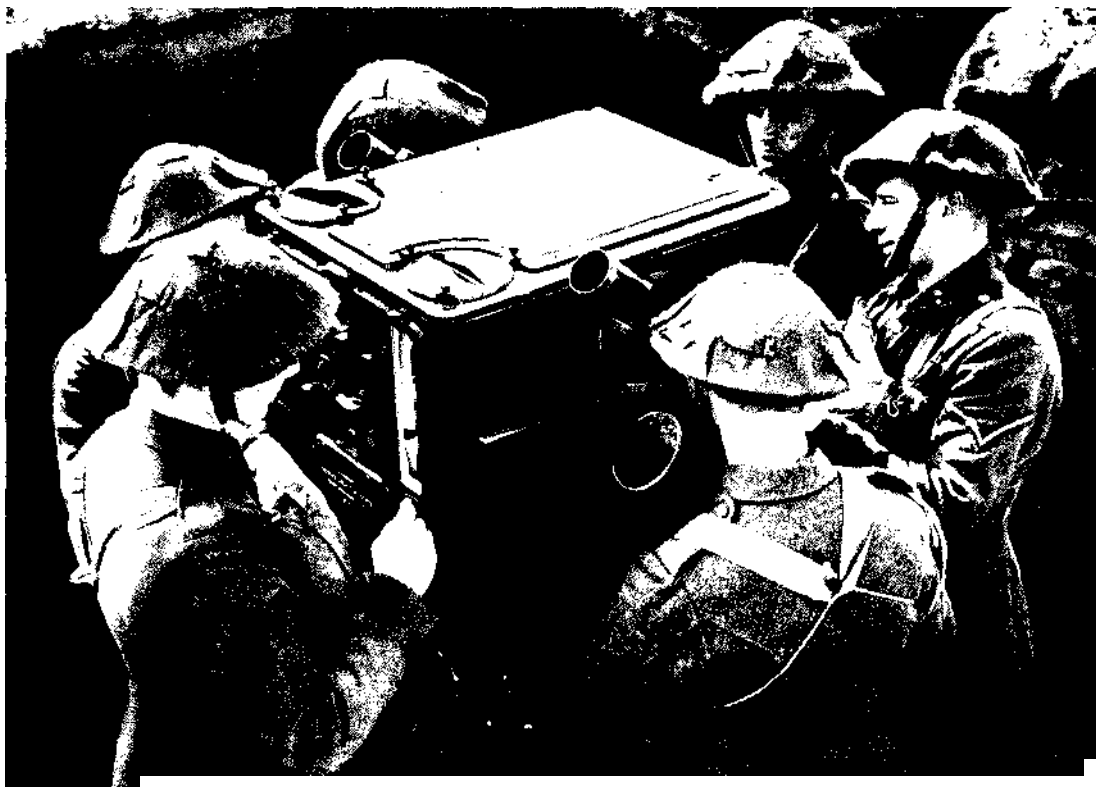
Men of the B.E.F. operating a predictor used for predicting the speed of approaching enemy planes in a trench behind the lines in France
