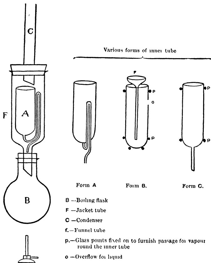
FIG. 1.—Lloyd's Extraction Apparatus.
