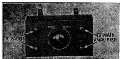
FIG. 47.—Royal Amplitone frequency control, a tuned filter, shown connected in Fig. 36.
