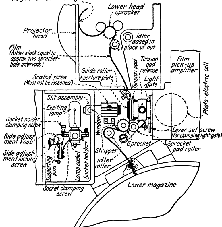
FIG. 7.—Film-reproducing attachment for use with Simplex projector, showing threaded film. (Western Electric Type D 86012.)
