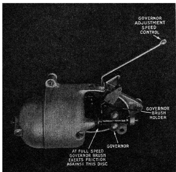
FIG. 75.—Driving motor with mechanical governor for speed control, used on earlier models of Western Electric non-synchronous reproducing turntables.
