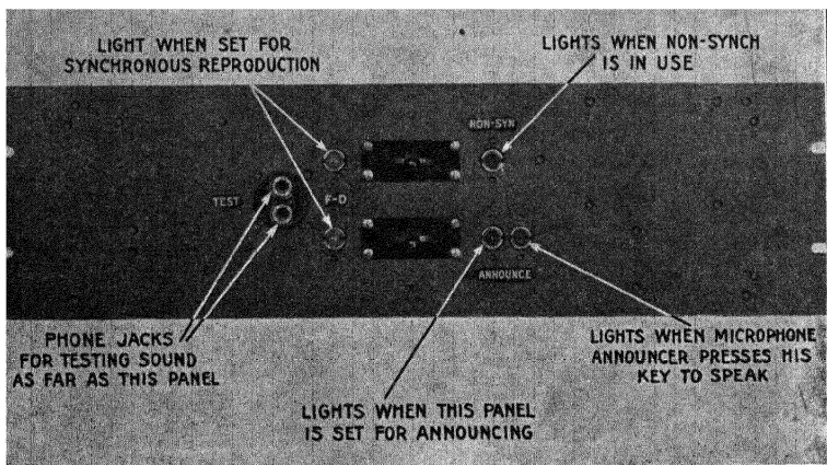
FIG. 44.—Western Electric type D 88449 switching panel for synchronous and non-synchronous reproduction, and for announcing.
