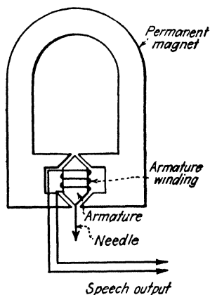
FIG. 30.—Diagram of typical disc reproducer.
