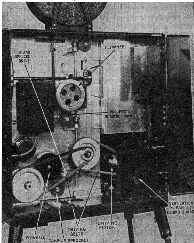
FIG. 26.—Drive side of RCA-Photophone model 4PP-6B portable projector.
