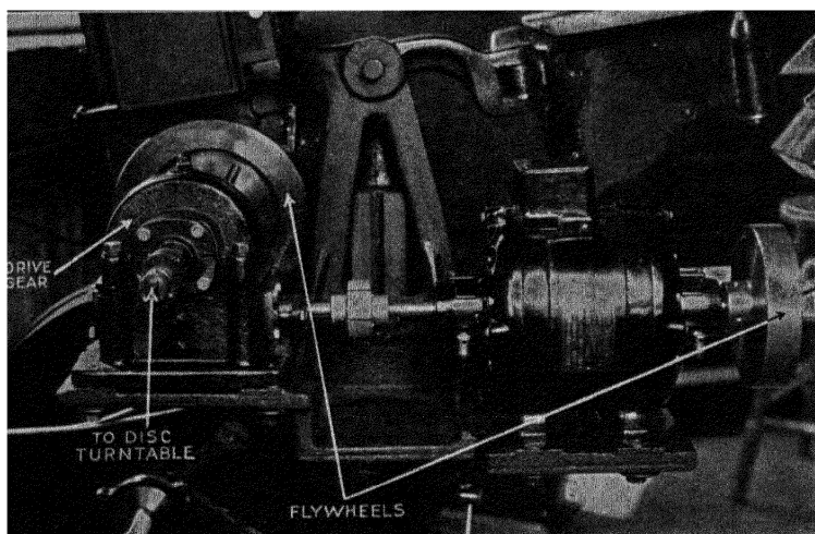
FIG. 23.—Royal Amplitone direct drive, type for Simplex only, disc and film.
