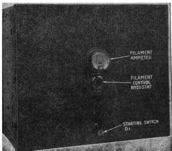
FIG. 53.—External view, front, of Western Electric 46A amplifier. This amplifier is the same in fundamental design as the 46B shown in Fig. 54.
