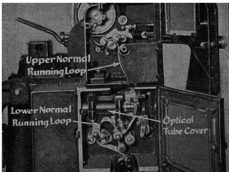
FIG. 22.—Patent sound-on-film attachment, type for Simplex, showing film threaded up in projector and in attachment.
