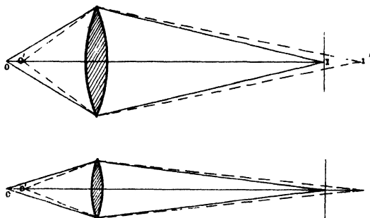
FIG. 14.—Diagram showing that “diffusion depth” of focus is larger with a lens of small than with a lens of high N.A. The unbroken and broken lines show image formation of two axial points O and O' an equal distance apart. The image-disc of O' in the plane of the image of O is seen to be much smaller in the case of the lens of small N.A.
