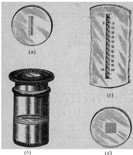
FIG. 48. EYEPIECE MICROMETERS
