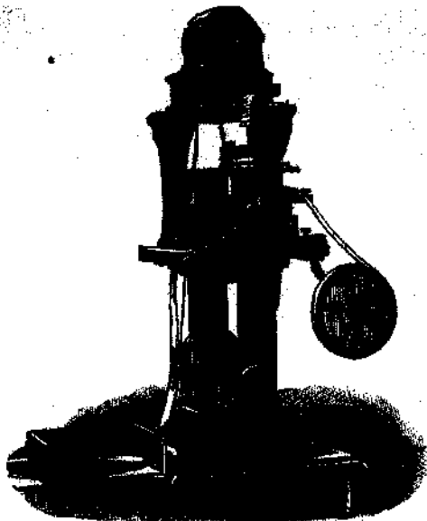
THE SIPHON RECORDER (later pattern).
