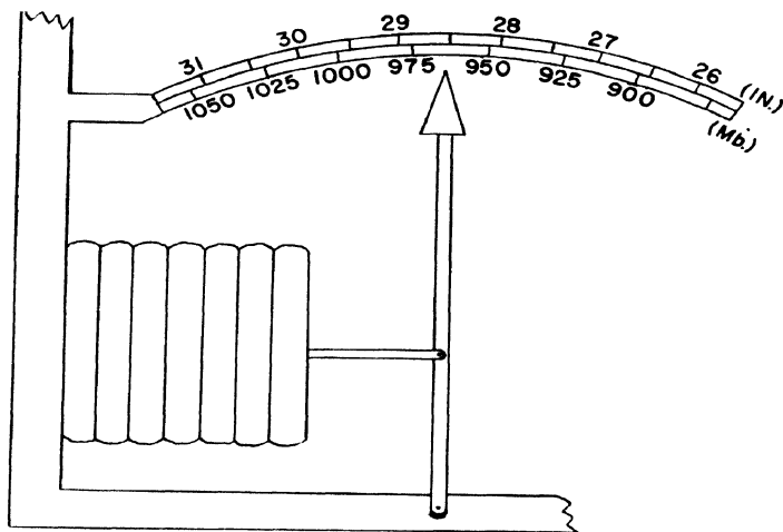
Fig. 13a. Schematic Drawing of an Aneroid Barometer.
