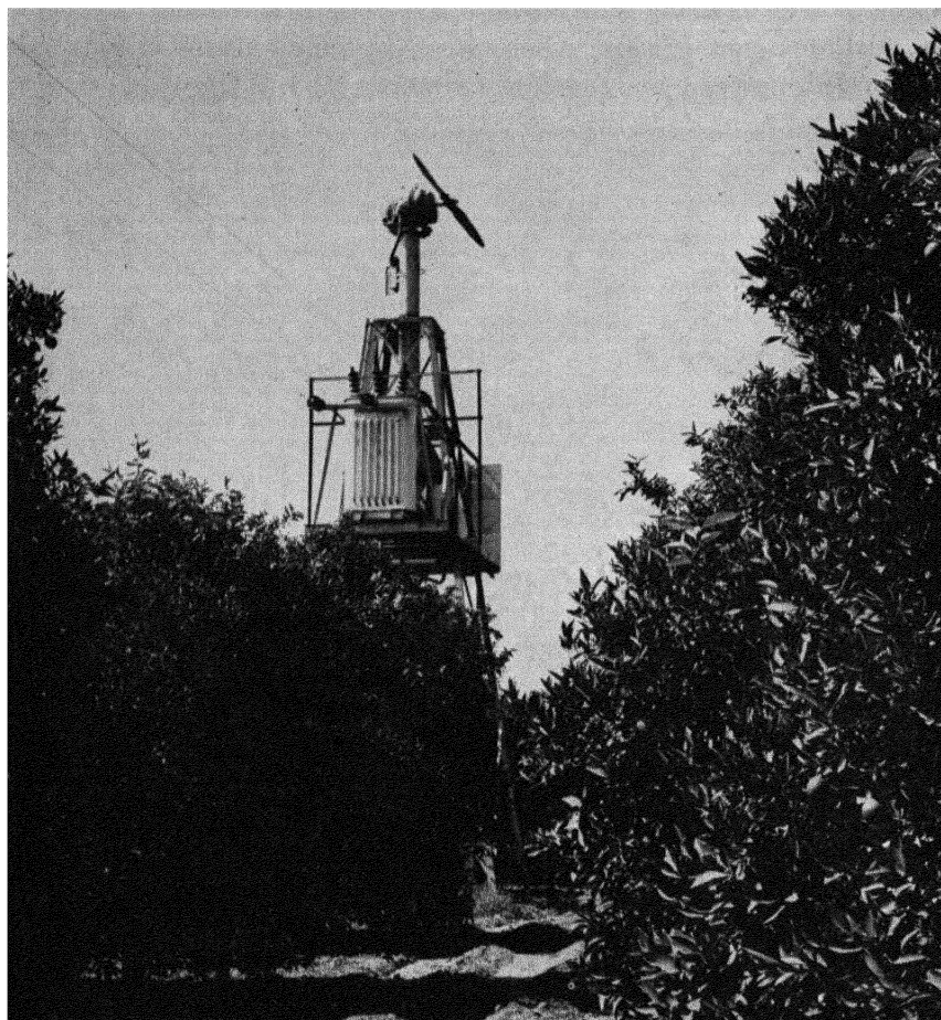
Fig. 63. Wind Machine for Fighting Freezes. This type of device is being extensively used in the California citrus groves. Most freezes are associated with sharp temperature inversions and may be averted by thoroughly stirring the lower air. Sunkist Photo.
