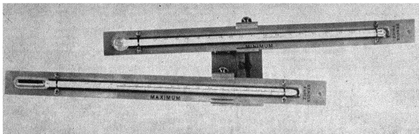
Fig. 5. Maximum and Minimum Thermometers with Townsend Support. Courtesy, Friez Instrument Division, Bendix Aviation Corp., Baltimore, Md.
