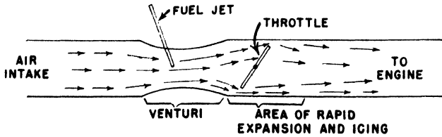
Fig. 121. Carburetor Icing. Air pressure is reduced on the engine side of the venturi, causing rapid cooling by expansion. Cooling is further accelerated by vaporization of the liquid fuel.
