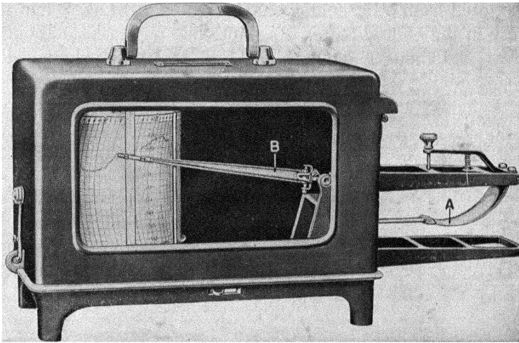
Fig. 6. Thermograph. A clock mechanism rotates the cylinder beneath the recording pen. Temperature changes cause changes in the curvature of the Bourdon tube, A, resulting in vertical movements of the arm, B. Courtesy, Friez Instrument Division, Bendix Aviation Corp.
