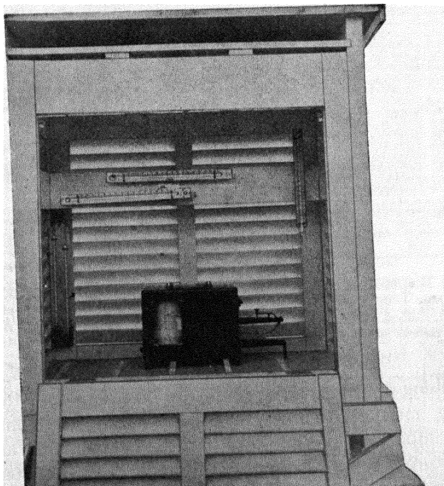
Fig. 7. Instrument Shelter with Door Open and Instruments in Place. Courtesy, U. S. Weather Bureau.
