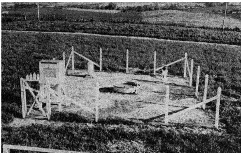
Fig. 24. Class A Evaporation Station. From left to right the instruments and equipment are an instrument shelter, weighing rain gage, evaporation pan with stillwell and anemometer, and a standard 8-inch rain gage. Courtesy, U. S. Weather Bureau.
