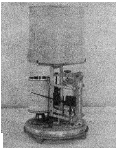
Fig. 42. Fergusson Weighing Rain Gage. Outside cover has been removed; makes a permanent, continuous record of the rate and amount of rainfall. Courtesy, U. S. Weather Bureau.
