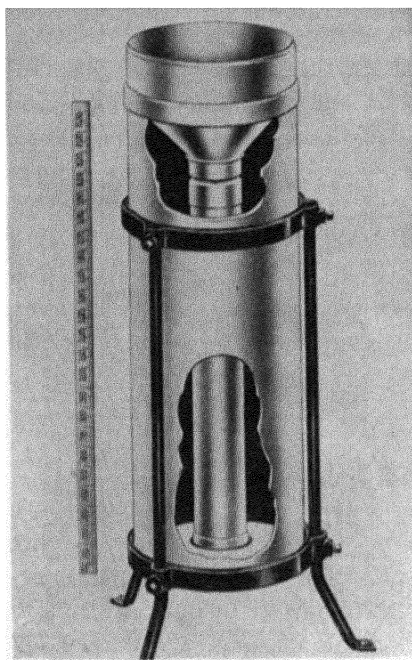
Fig. 41. Rain Gage. Standard 8-inch pattern, with measuring stick. Courtesy, Friez Instrument Division, Bendix Aviation Corp.
