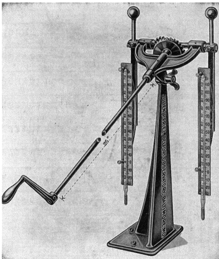
Fig. 22. Whirled Psychrometer. For humidity observations, a wet muslin sleeve is fitted over the bulb of one of the thermometers, which are then whirled rapidly by turning the crank. Courtesy, Friez Instrument Division, Bendix Aviation Corp.
