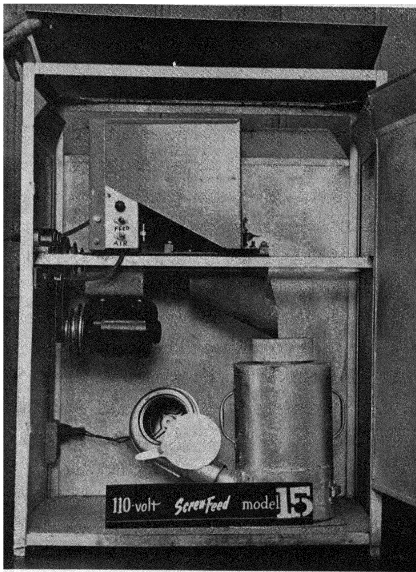
Fig. 68. Cloud Seeding Generator Foundry coke is impregnated with a carefully controlled solution of silver iodide and placed in a hopper. A screw-type feed releases fuel into the furnace at lower right. Silver iodide is vaporized in the intense heat of the burning coke and is emitted into the air stream at the rate of about 1,000,000,000,000,000 ( 10^{15} ) crystals per minute, each crystal being the potential center of a raindrop. (Note vents at top of generator.) Courtesy, Water Resources Development Corp., Denver, Colorado.
