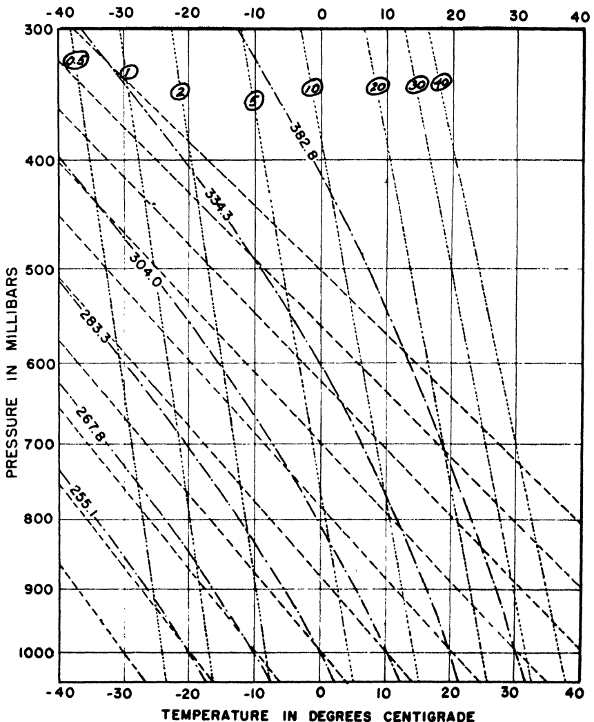
Fig. 55. The Adiabatic Chart. Drawing by Herbert Beaujon.
