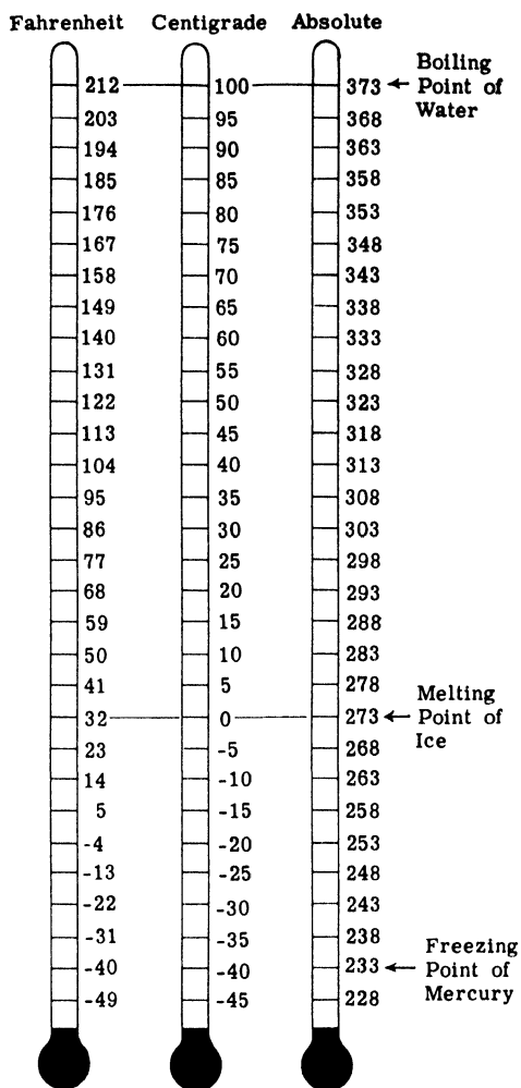
Fig. 4. Thermometer Scales Compared.
