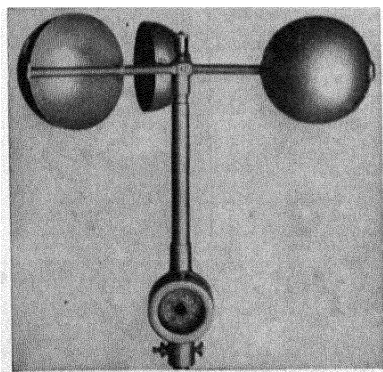
Fig. 18. Robinson 3-cup Anemometer. Totalizing dials indicate the total miles of wind, and electrical contacts operate a speed indicator and recorder. Courtesy, Friez Instrument Division, Bendix Aviation Corp.
