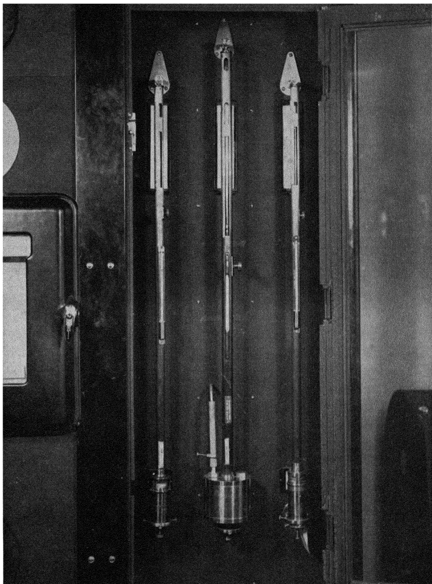
Fig. 11. Mercurial Barometers Mounted in Case. From left to right, Fortin type with screw to adjust level of mercury in cistern, fixed-cistern type, and a barometer combining principles of the other two. Courtesy, U. S. Weather Bureau.
