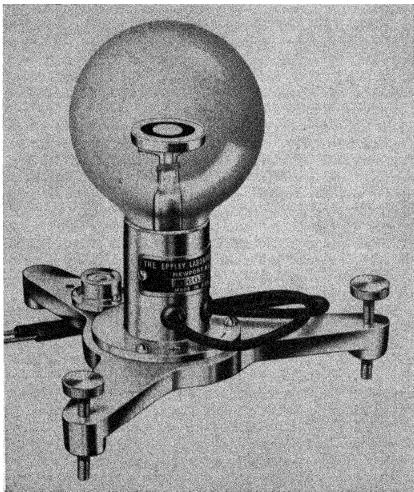
Fig. 47. Pyrheliometer. Two circular rings of equal area, one black and the other white, are connected by thermocouple to produce an electromotive force proportional to the intensity of solar radiation. Courtesy, Eppley Laboratory, Inc., Newport, R.I.
