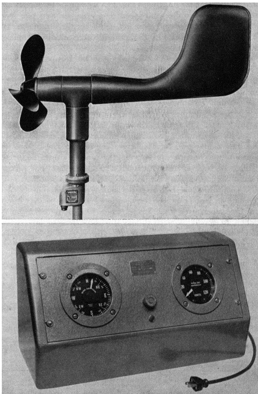
Fig. 19. Aerovane. Instantaneous direction and speed of the wind may be read remotely from the dials connected to this instrument. Courtesy, Friez Instrument Division, Bendix Aviation Corp.
