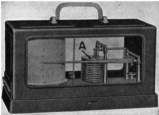
Fig. 14. Barograph. The flexible, metallic chambers, A, are partially exhausted of air and a system of internal springs are balanced against the outside air pressure. Changing air pressure results in compression or expansion which causes a vertical movement of the pen. Courtesy, Friez Instrument Division, Bendix Aviation Corp.
