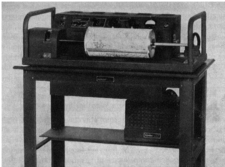
Fig. 145. Facsimile. This instrument reproduces maps and charts from a master copy drawn in Washington, D. C. It requires a line connection similar to telegraph. A modification of this machine can reproduce maps from radio transmissions. Courtesy, Times Facsimile Corp., New York, New York.
