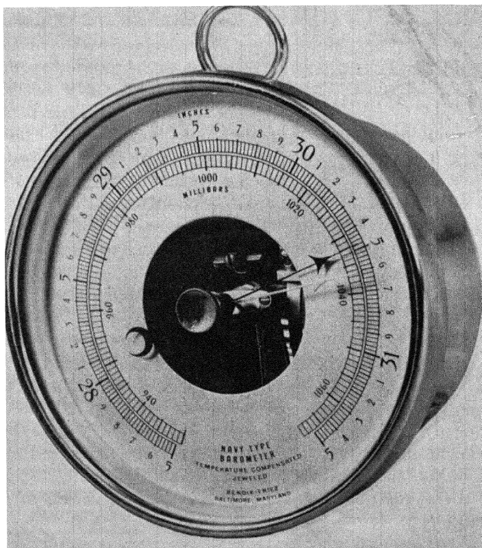
Fig. 13b. Navy Type Aneroid Barometer Calibrated in Inches and Millibars. Courtesy, Friez Instrument Division, Bendix Aviation Corp.
