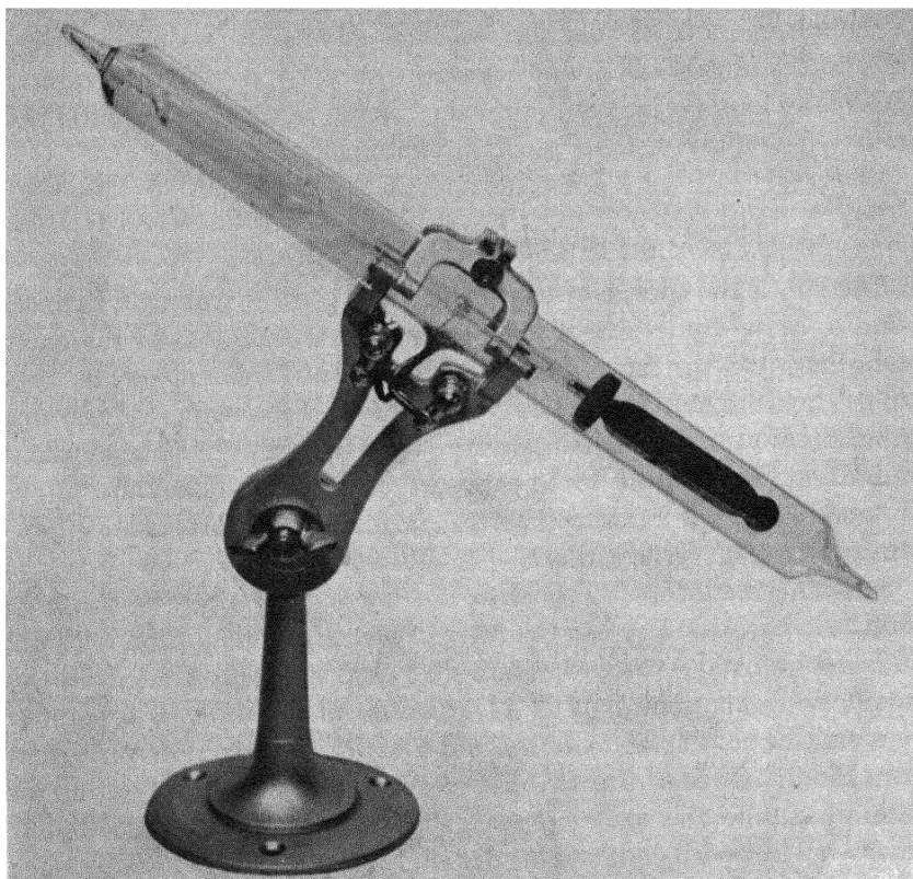
Fig. 43. Electrical Sunshine Recorder. Courtesy, Friez Instrument Division, Bendix Aviation Corp.
