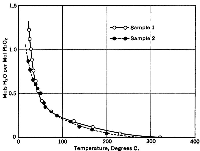
FIG. 44.—Dehydration isobars of hydrous PbO 2 .
