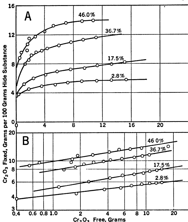
FIG. 64.—Adsorption of \text{Cr}_2\text{O}_3 by hide substance from chrome sulfate tanning liquors of varying degrees of basicity.
