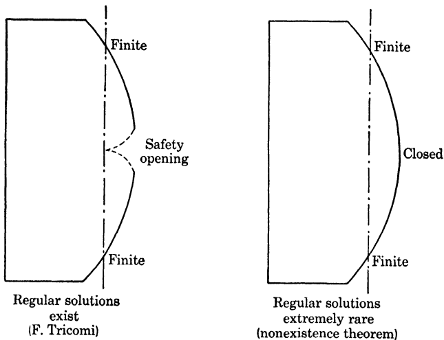
FIG. 8. Transonic flow with entrance and exit corners.
