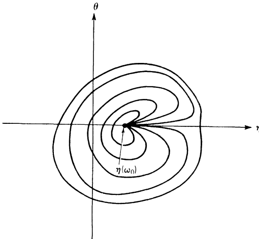
FIG. 3. \psi_1 + A\psi_2 streamlines. \eta = -\ln [\tau(2\beta + 1)] .
