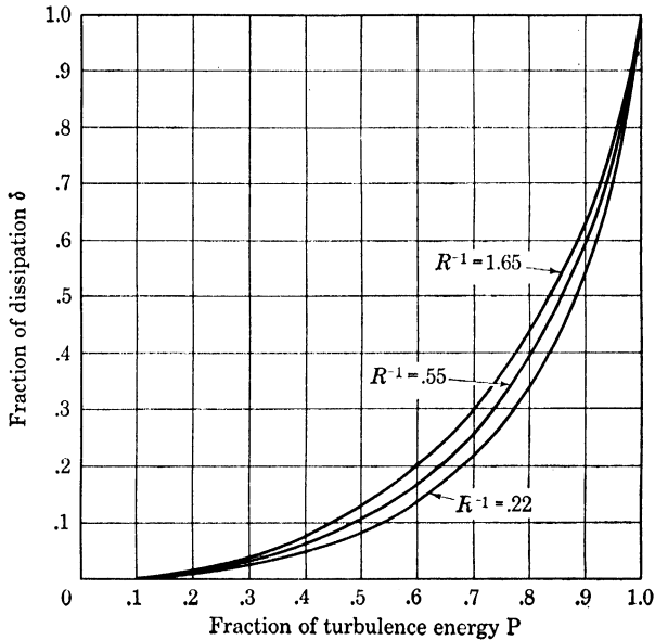
FIG. 2. Fraction of energy dissipation against fraction of energy content for R^{-1} = 0, 0.22, 0.55, 1.65 (corresponding to \kappa R_{\lambda} = \infty, 16, 5, 1 , approximately).
