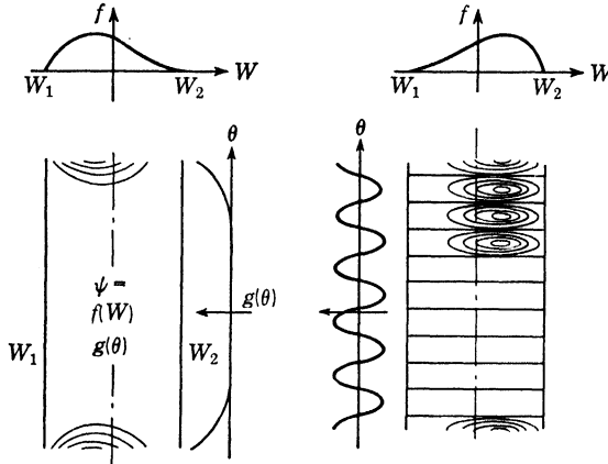
FIG. 3. The subsonic and supersonic types of disturbances in mixed flows.
