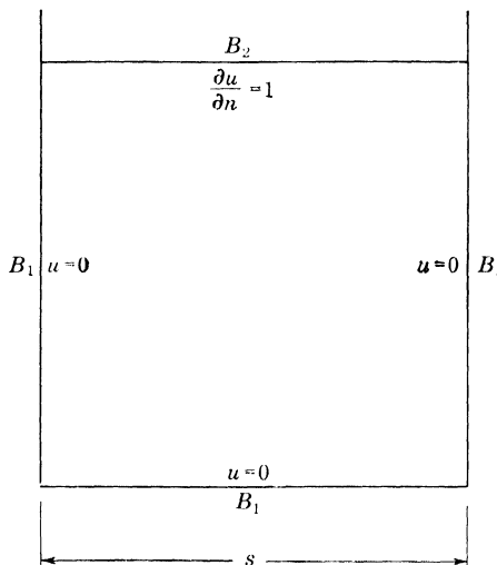
FIG. 9. Channel with square cross section.
