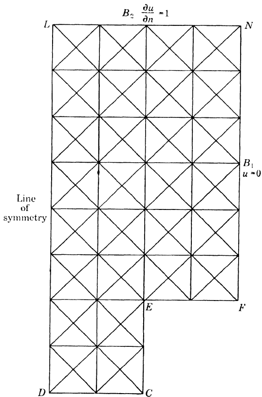
FIG. 16. Channel with irregular cross section: triangulation in half section for n = 8 .
