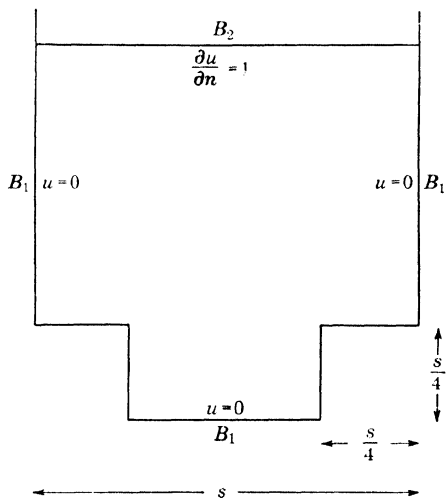
FIG. 15. Channel with irregular cross section.
