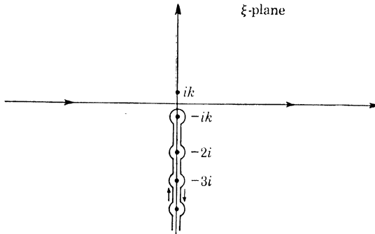
FIG. 1. The horizontal contour is the integration path for subsonic \tau ; the indented contour is that for supersonic \tau . The points -mi are those at which F(-i\xi, \tau) has simple poles.
