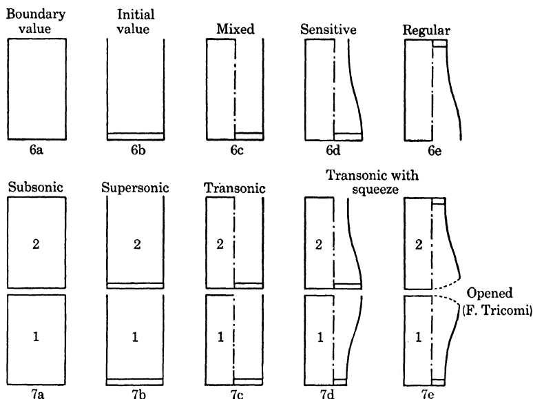
FIGS. 6 and 7. (6a-e) Adequate boundary conditions. (7a-e) Unifications.
