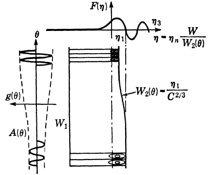
FIG. 5. Supersonic type of disturbances at variable distances W_2(\theta) .
