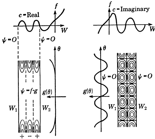
FIG. 2. Subsonic and supersonic disturbances.
