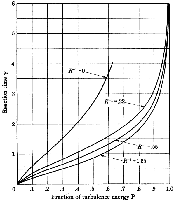
FIG. 1. "Reaction time" against fraction of turbulence energy for R^{-1} = 0, 0.22, 0.55, 1.65 (corresponding to \kappa R_{\lambda} = \infty, 16, 5, 1 , approximately).
