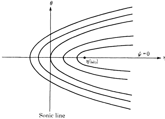
FIG. 2. Contours of \psi_1 = \text{constant} . \eta = -\ln [\tau(2\beta + 1)] .
