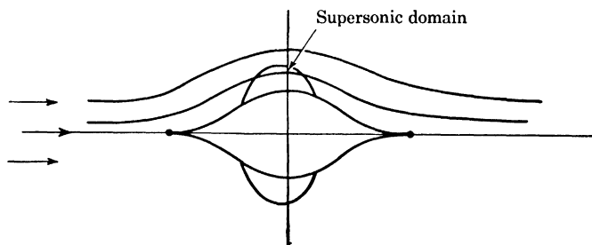
FIG. 4. The upper half of this flow field corresponds to the "hodograph" depicted in Fig. 3.
