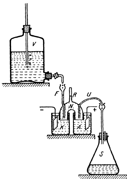
FIG. 4. Apparatus for electro-osmosis.
