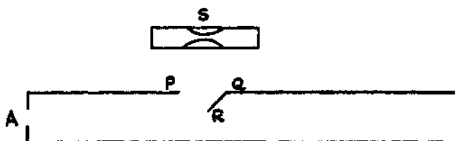
FIG. 23 Abney level and clinometer
