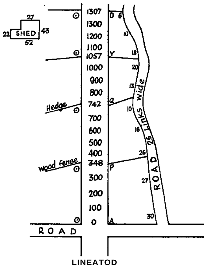
FIG. 19. Field-book entry
