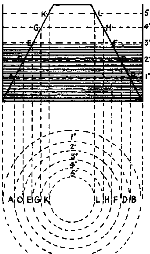
FIG. 13. Contouring
