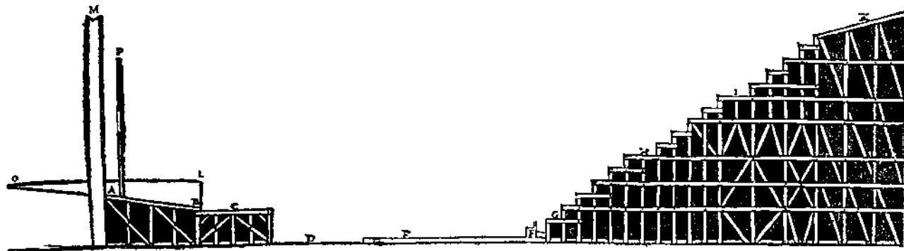
THE PROFILO OR SECTION OF A STAGE
