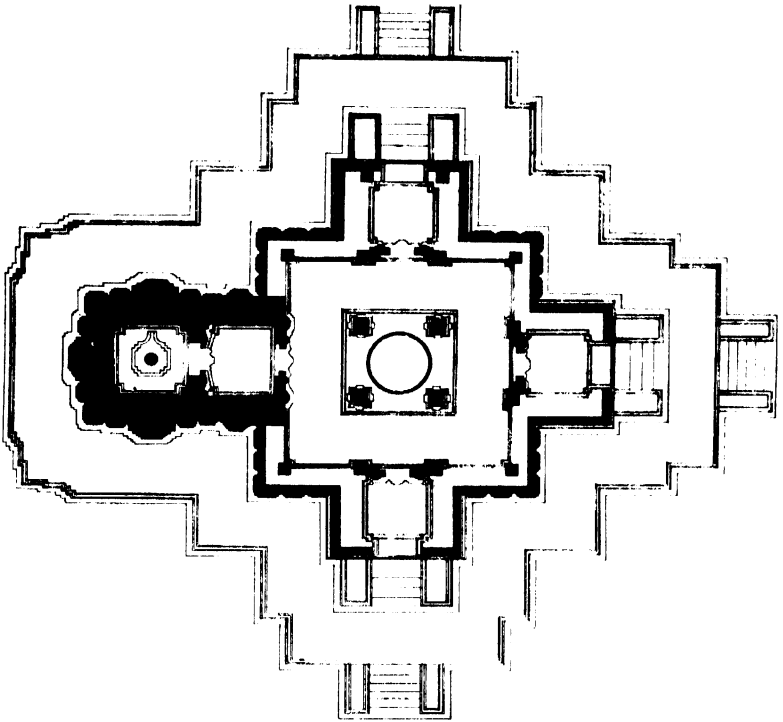
(a) PLAN OF THE SOMESHVARA TEMPLE: PILLALMARI. Scale: 18 ft. to 1 in.
