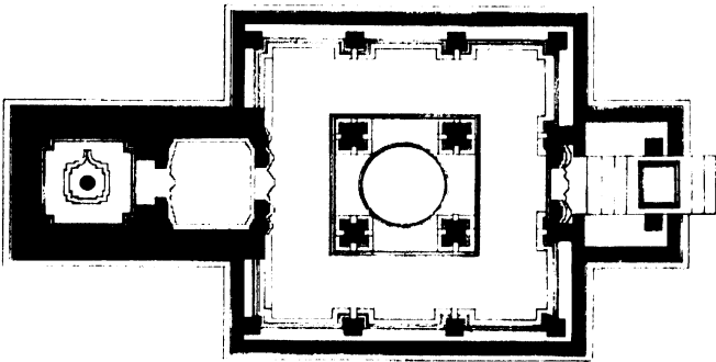
(b) PLAN OF THE RAMESHVARA TEMPLE: PILLALMARI. Scale: 18 ft. to 1 in.
