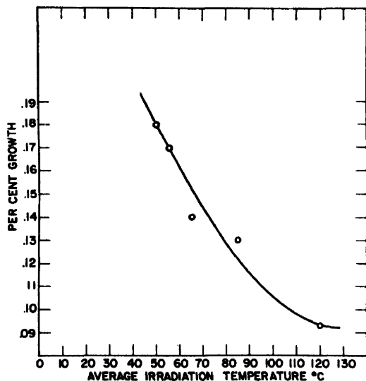
Figure 19. Per cent growth vs average irradiation temperature of graphite samples; integrated flux 1.2 \times 10^{20} neutrons/cm 2
