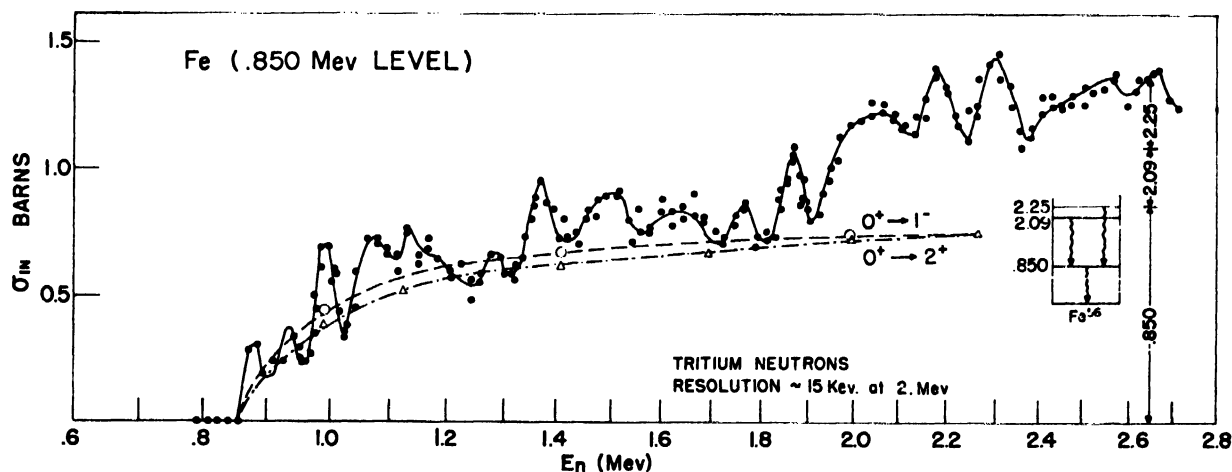
Figure 8. Neutron inelastic scattering by Iron as a function of energy. The dashed curves were calculated using the Hauser-Feshbach theory
