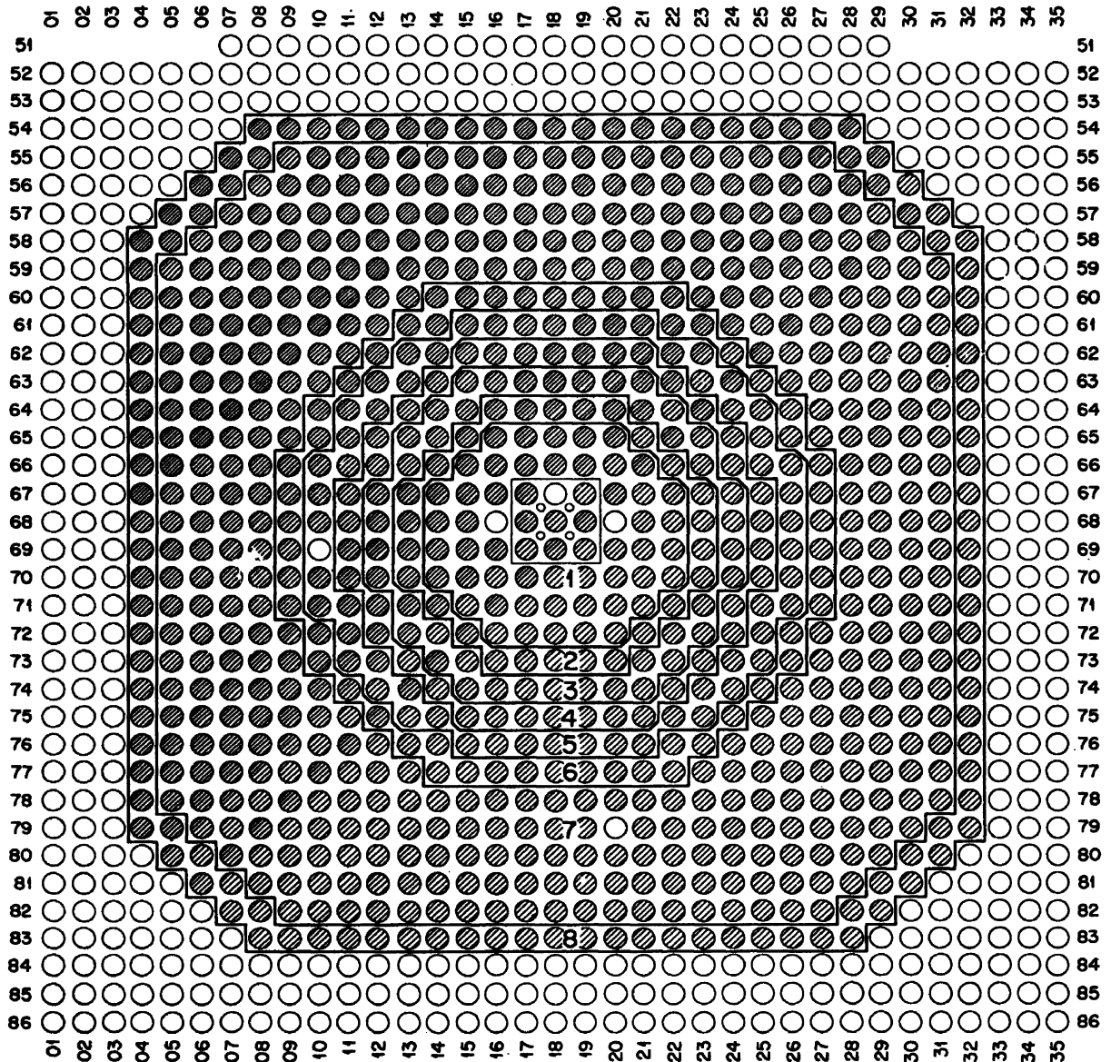
Figure 8. The present fuel loading pattern of the graphite reactor showing a much expanded core size and shorter rows at the center to depress the temperature in that region. This loading consists of 54.1 tons of normal uranium
