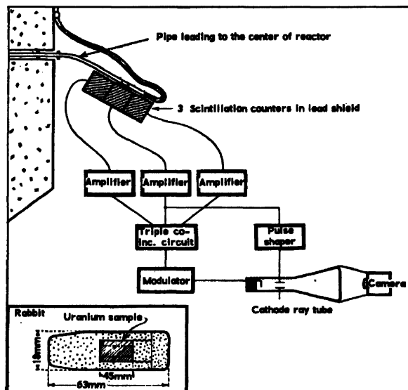
Figure 1. Experimental arrangement
