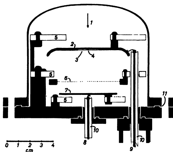
Figure 1. Section through H_2 -recoil chamber: (1) direction of incident neutrons, (2) high-voltage electrode, (3) polyethylene layer, (4) polonium source for calibration purposes, (5) glass insulators, (6) grid, (7) collector electrode, (8) lead through to preamplifier, (9) high-voltage lead through, (10) steatite insulator, (11) lead gasket
