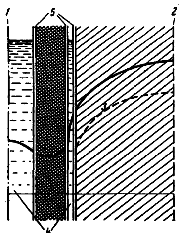
Figure 3. Distribution of the thermal neutron flux in the lattice cell: (1) axis of the channel; (2) outer boundary of cell; (3) graphite; (4) water; (5) aluminum
