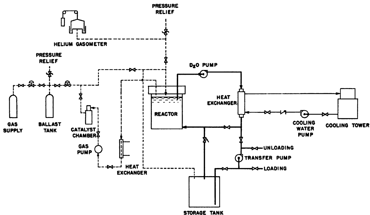
Figure 4. Natural uranium heavy water research reactor flow diagram
