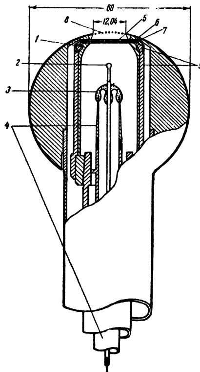
Figure 6. Cross section through central electrode: (1) outer electrode of counter; (2) collecting electrode; (3) insulator; (4) pin of collecting electrode; (5) film; (6) film supporting mesh; (7) spring; (8) spherical mesh; and (9) cylinder
