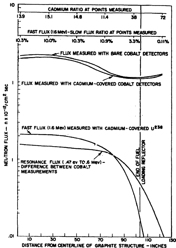
Figure 12. Neutron flux measurements in experimental hole E-13, power level 26 megawatts
