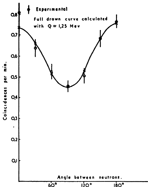
Figure 2. Comparison of the calculated and the experimental results
