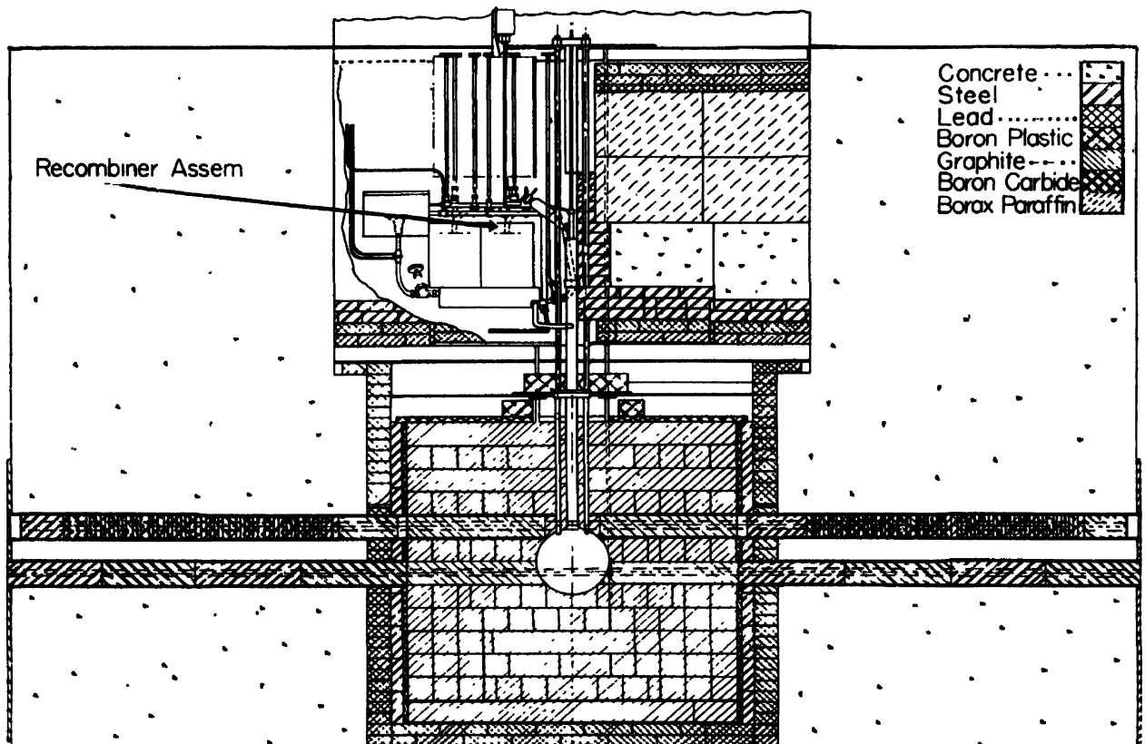
Figure 7. East-west vertical section of water boiler (Supo model)
