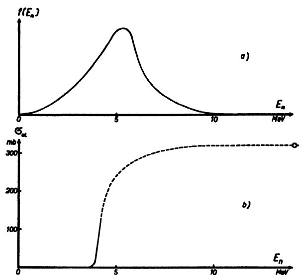
Figure 6. (a) Energy spectrum of Ra-Be neutrons (Racey et al. 5 ), (b) cross section for O^{16}(n,\alpha)C^{13} . Smooth curve, our measurement; punctuated curve, arbitrary extrapolation; o, denotes Lillie's measurement states of O^{17} at 7.81 \pm 0.02 and 7.95 \pm 0.02 Mev above the ground state.
