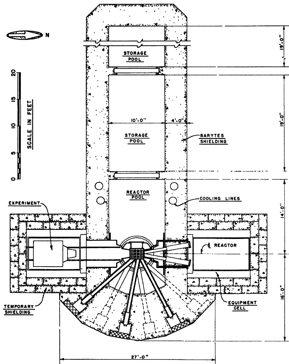
Figure 20. Reactor and pool structure, horizontal section
