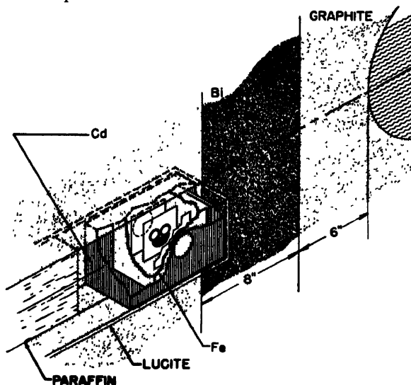
Figure 2. Position of the fission calorimeter in the south thermal column of the Los Alamos homogeneous reactor. The reactor sphere is on the right
