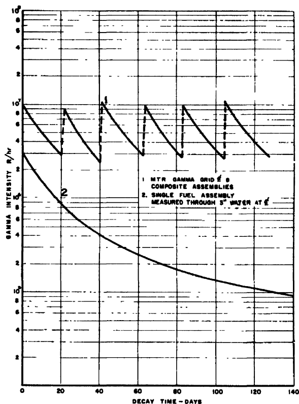
Figure 11. MTR gamma irradiation facility decay curves of spent fuel assemblies
