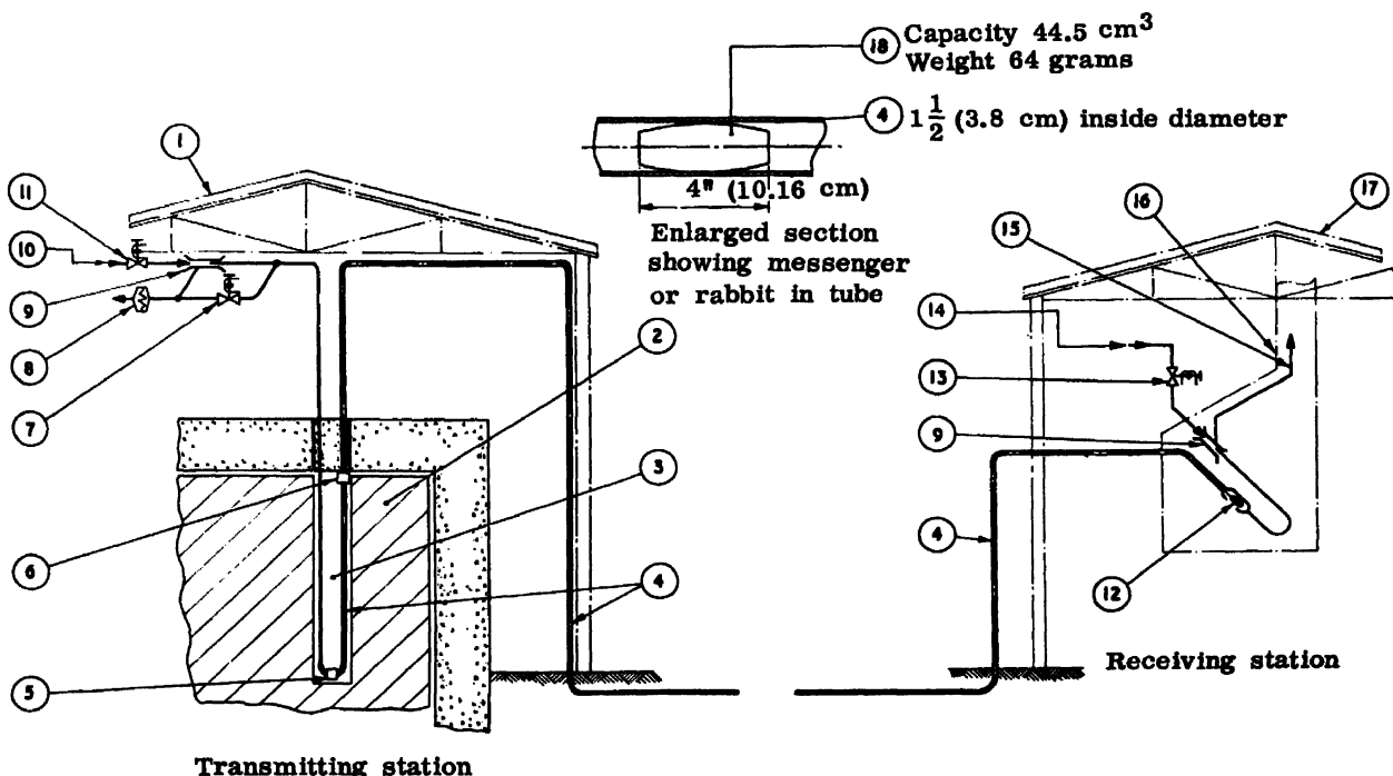
Figure 1. 220 rabbit installation. Description: (1) reactor building; (2) reactor; (3) experimental hole; (4) rabbit or messenger tube; (5) "in reactor" position switch; (6) "transit in reactor" switch; (7) solenoid exhaust valve; (8) filter before discharging air to building; (9) air injection; (10) air supply 30 psig; (11) solenoid air injection valve; (12) receiving station; (13) air injection valve (return to reactor); (14) air supply 30 psig (return to reactor); (15) air exhaust to stack; (16) laboratory fume cupboard; (17) laboratory building; (18) rabbit or messenger
