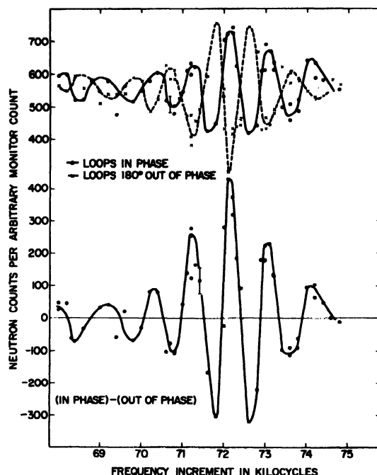
Figure 2. Resonance curve of neutron intensity as a function of radio frequency in coils. Pattern is characteristic of the "separated RF loop" method
