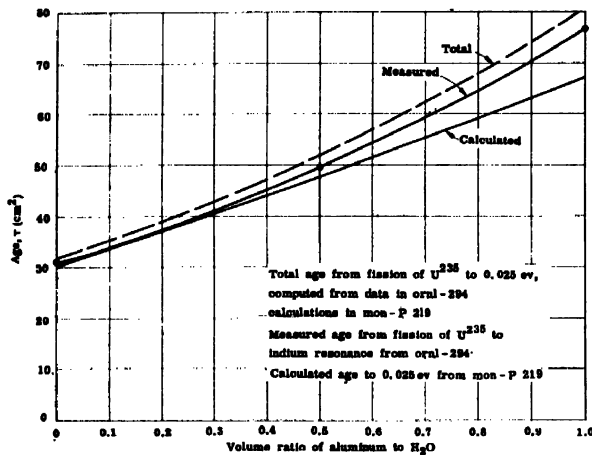
Figure 6. Age, \tau fission neutrons in \text{H}_2\text{O} -Al mixtures
