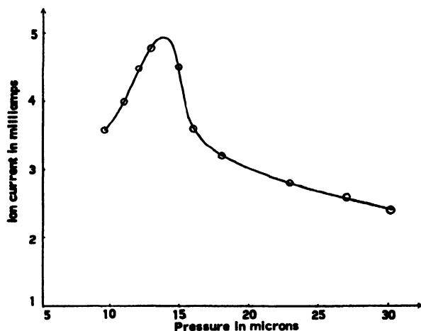
Figure 1. Curve showing variation of ion current with pressure keeping wattage input of the oscillator and extracting voltage constant. The probe current varies from 4.5 to 9 ma
