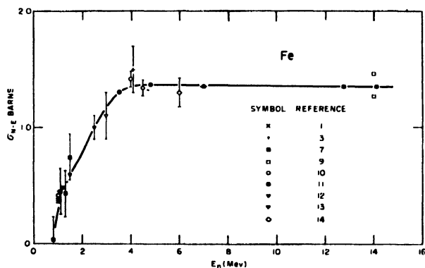
Figure 6. Non-elastic cross section (in barns) of Fe as a function of neutron energy
