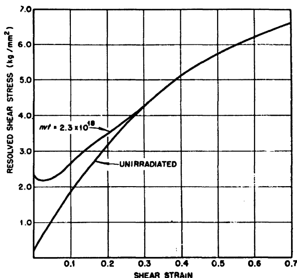
Figure 1. Stress-strain curves of copper crystals
