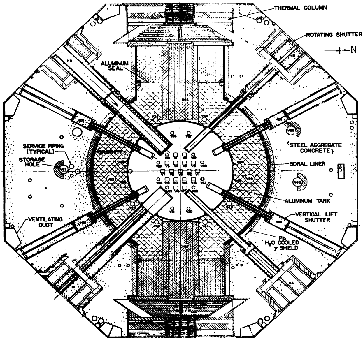
Figure 11. Section through principal beam holes
