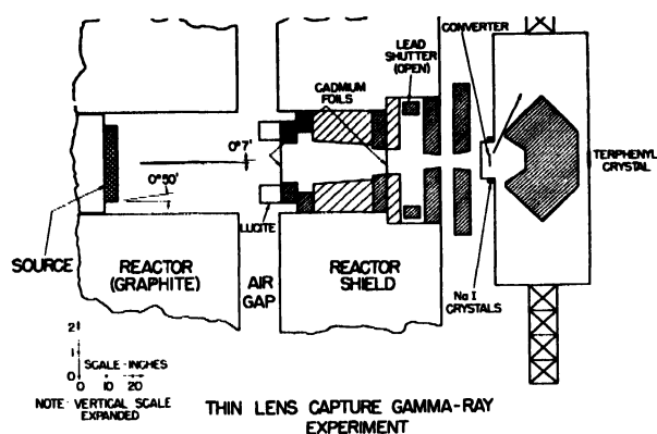
Figure 3. Experimental arrangement for prompt gamma-ray experiment with thin lens \beta spectrometer. The gamma rays are collimated by lead apertures and pass into the spectrometer vacuum, through a converter and into the beam catcher. Two NaI crystals outside the direct beam but near the converter are used to detect the K X-rays of the converter
