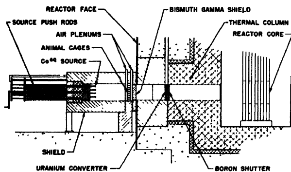
Figure 10. Fast neutron exposure chamber
