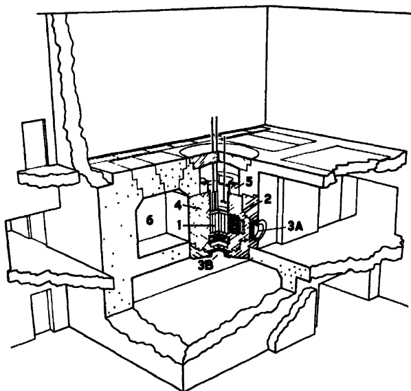
Figure 7. Perspective of medical research reactor
