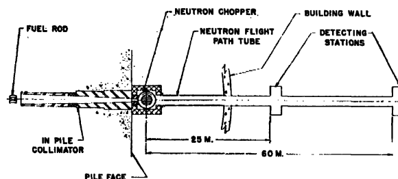
Figure 4. Diagram of fast chopper
