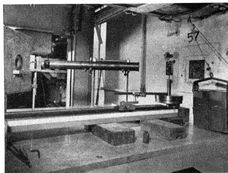
Figure 20. Neutron collimator used by the Oak Ridge School of Reactor Technology (ORSORT) for performing short experiments. The setup shown is for an experiment in the diffraction of neutrons with a crystal
