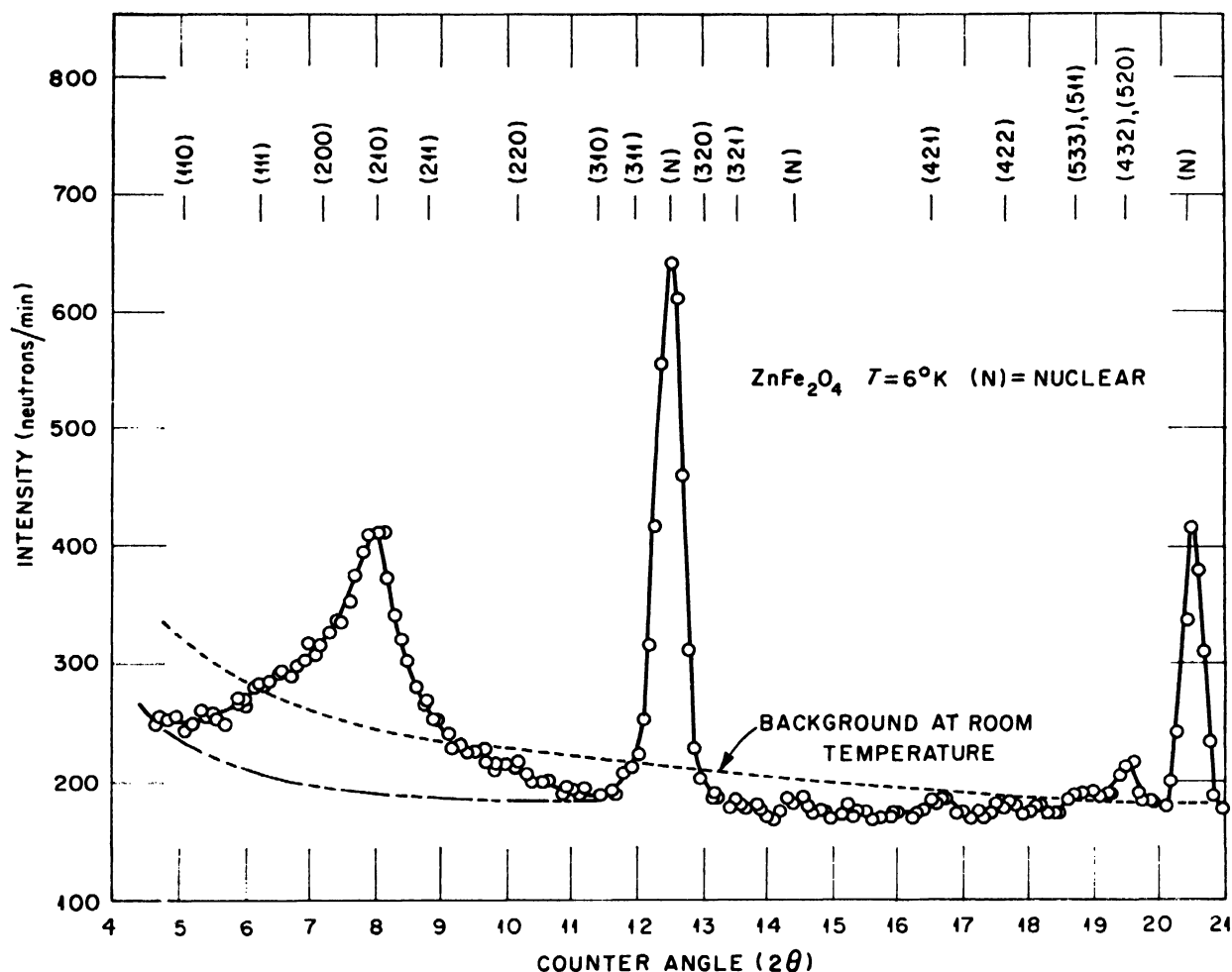
Figure 20. Low temperature pattern for \text{ZnFe}_2\text{O}_4 representing a complicated antiferromagnetic phase (Corliss and Hastings)
