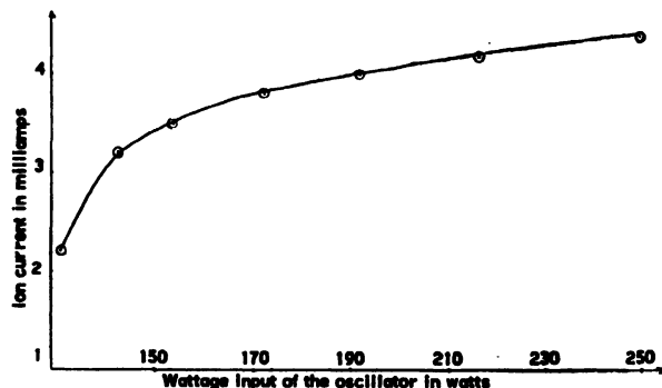
Figure 2. Curve showing variation of ion current with wattage input of the oscillator keeping the pressure and extracting voltage constant. The probe current varies from 5 to 8 ma
