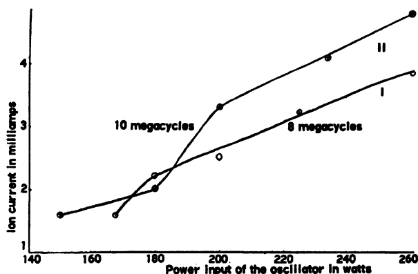
Figure 4. Curves showing variation of ion current at 8 and 10 megacycles frequency of the oscillator with power input of the oscillator keeping the pressure and extracting voltage constant. In curve I the probe current varies from 5 to 8 ma. In curve II the probe current varies from 4.5 to 9 ma
