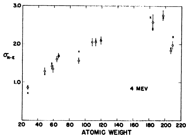
Figure 9. Non-elastic cross sections of fifteen elements at 4 Mev. The x's denote cross sections obtained by subtracting measured elastic cross sections from the total cross sections and have probable errors of 0.2 to 0.3 barns. The cross sections indicated by open circles were obtained by sphere transmission measurements
