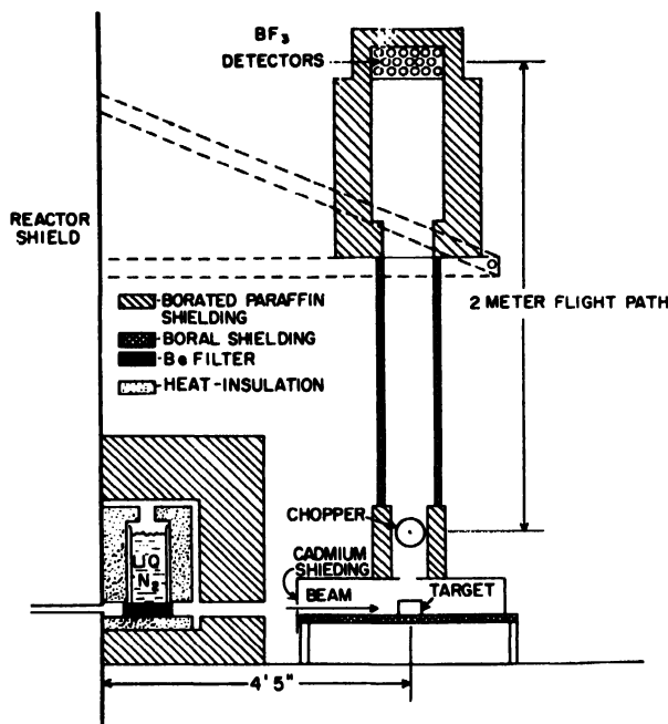
Figure 9. Apparatus for observation of the energy spectrum of Be filtered slow neutrons after scattering in a crystal lattice
