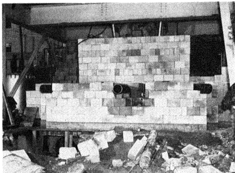
Figure 28. The stacking of the unmortared concrete block shielding. The large pipes are the beam hole tubes
