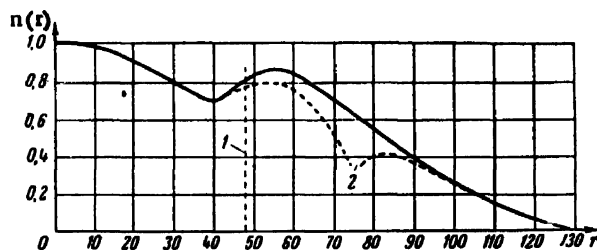
Figure 6. Distribution of the flux of thermal and epithermal neutrons along the radius of the "homogenized" reactor; (a) theoretical curve; (1) border of the active zone, (2) location of a "loop"
