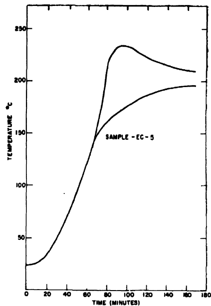
Figure 17. Time vs temperature plot of a graphite sample in a furnace held at 200°C; temperature of irradiation, 60°C
