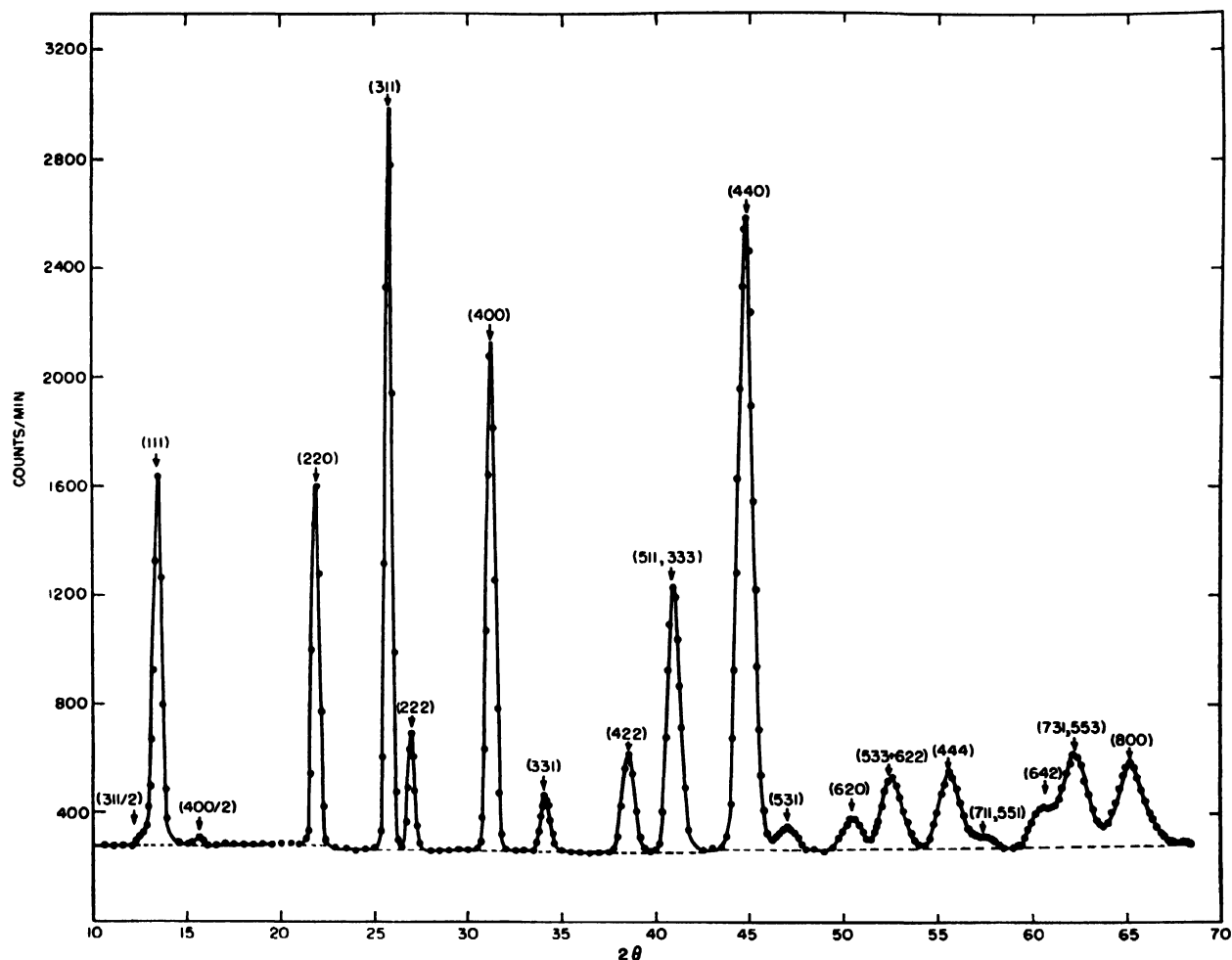
Figure 19. High resolution diffraction pattern for \text{MgFe}_2\text{O}_4 (Corliss and Hastings)
