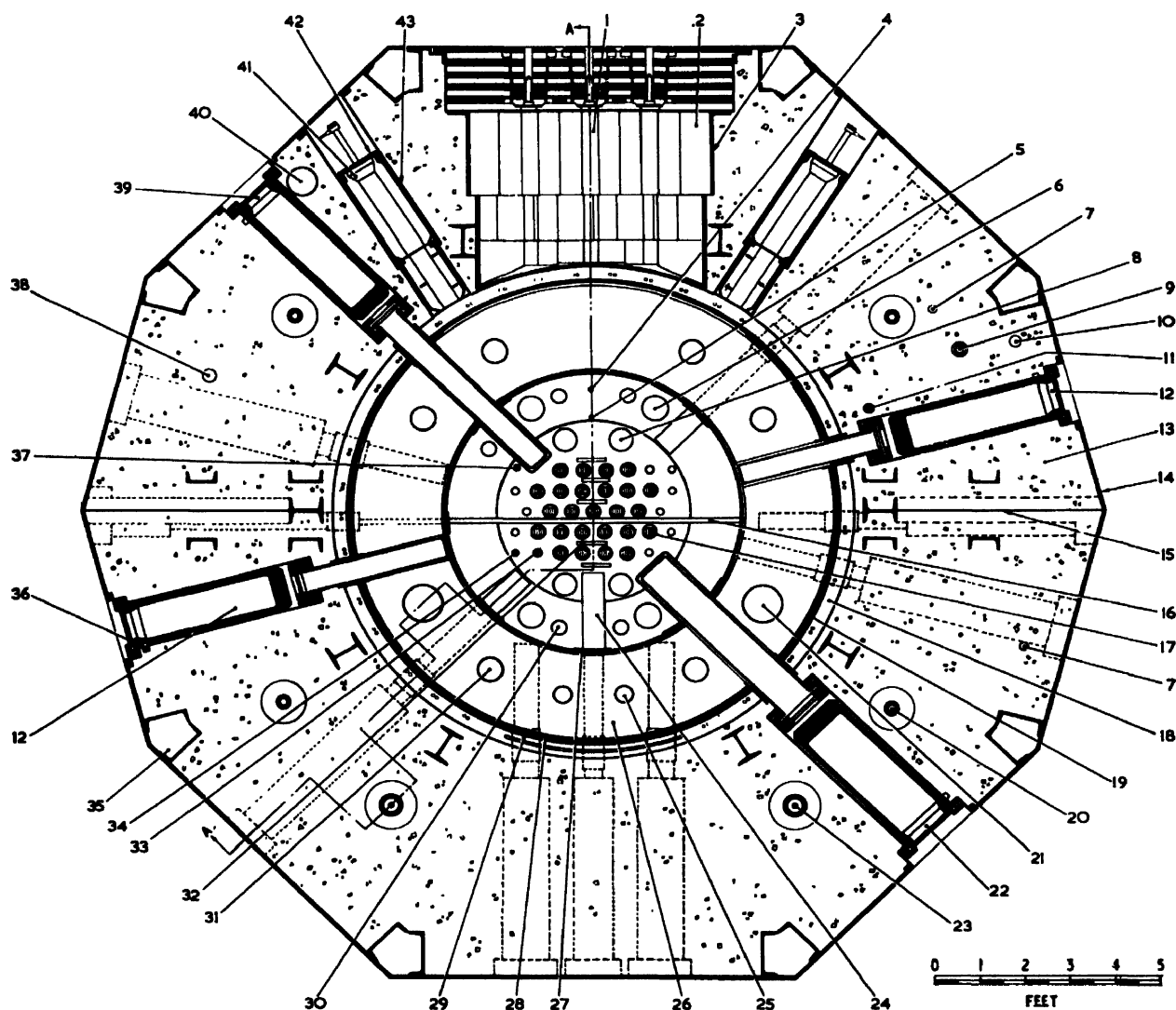
Figure 2. Reactor E.443: section in plan at half-depth of reactor core. Description: (1) thermal column; (2) thermal column graphite reflector; (3) thermal column boron lining; (4) 1 in. heavy water overflow pipe; (5) 1 in. aluminium tank drain pipe; (6) 7 in. heavy water outlet pipe; (7) 2 in. helium supplementary expansion line; (8) 6 V vertical experimental facility; (9) 2 in. anti-syphon weir pipe; (10) 3 in. helium balance line; (11) 1 in. anti-syphon weir pipe; (12) 6 HGR horizontal experimental facility; (13) concrete biological shield; (14) outer casing plates; (15) top structure; (16) 2 ton horizontal experimental facility; (17) fuel element; (18) lead shield with cooling coils; (19) steel tank; (20) 3 in. mortuary hole; (21) 10 VGR vertical experimental facility; (22) 10 H horizontal experimental facility; (23) 6 in. mortuary hole; (24) 4 H horizontal experimental facility; (25) 4 VGR vertical experimental facility; (26) graphite reflector; (27) aluminium tank; (28) lead thermal bond; (29) boron lining in steel tank; (30) 4 V vertical experimental facility; (31) 6 VGR vertical experimental facility; (32) coarse control rods with drive; (33) safety rod with drive; (34) 2 V vertical experimental facility; (35) service station; (36) CO 2 purge connection; (37) fine control rod with drive; (38) 3½ in. air suction manifold interconnector; (39) 6 H horizontal experimental facility; (40) helium expansion main; (41) ion chamber fittings; (42) ion chamber plug; and (43) ion chamber liner
