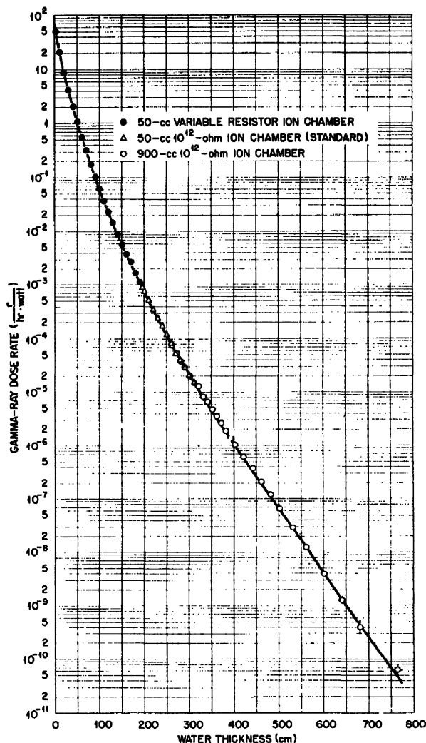
Figure 17. Gamma-ray dose rate as a function of distance from the Bulk Shielding Reactor
