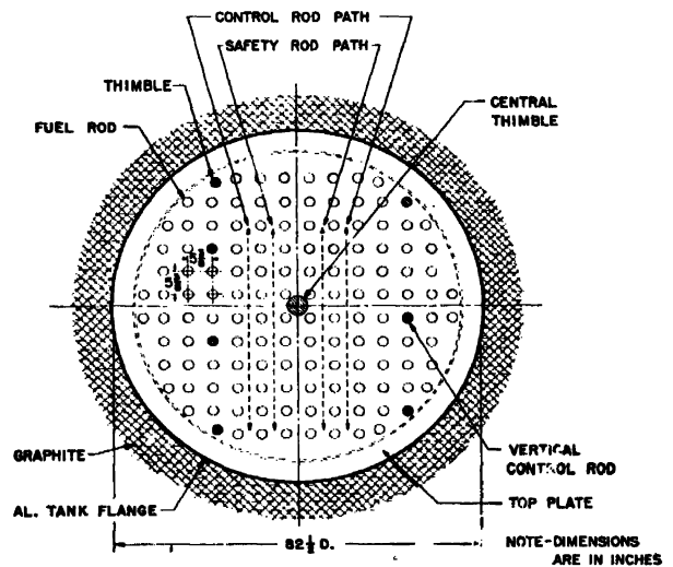
Figure 2. Lattice of natural uranium heavy water research reactor
