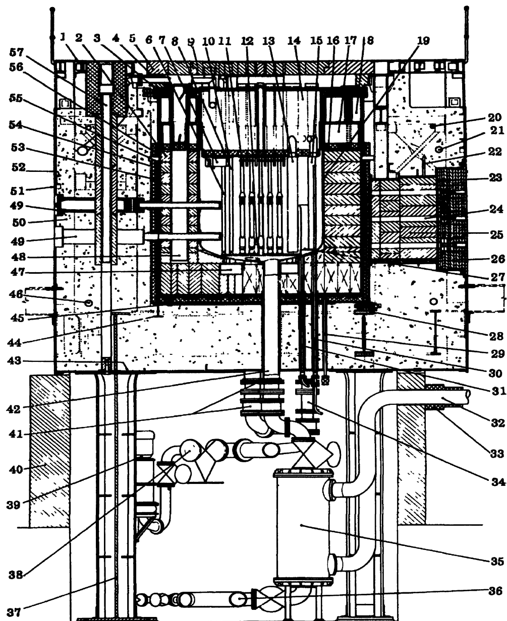
Figure 2a. Reactor E.443: section in elevation
