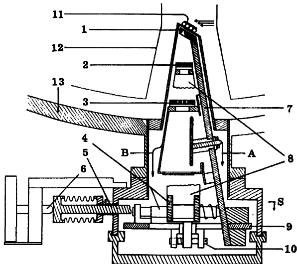
Figure 12. Modified deflection apparatus for measurements at high pressures
