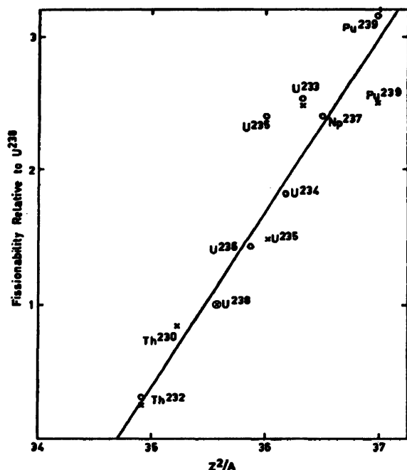
Figure 4. The fissionability of several materials relative to U^{238} are plotted as a function of the Z^2/A values of the bombarded nuclei. The circles represent an average of the data obtained from gamma rays at two betatron energies, 17 and 20 Mev. The crosses are data of McElhinney and Ogle (see reference 22)
