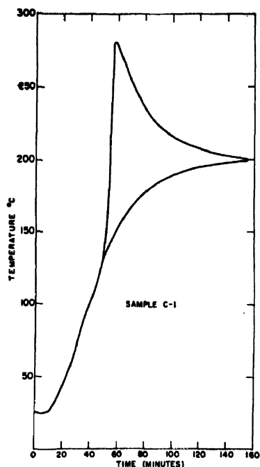
Figure 13. Time vs temperature plot of a graphite sample in a furnace held at 200°C; temperature of irradiation, 55°C
