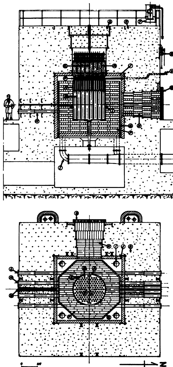
Figure 1. Vertical and horizontal cross sections of the reactor
