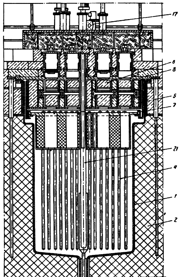
Figure 2. Cross section showing the location of the slit-shutters
