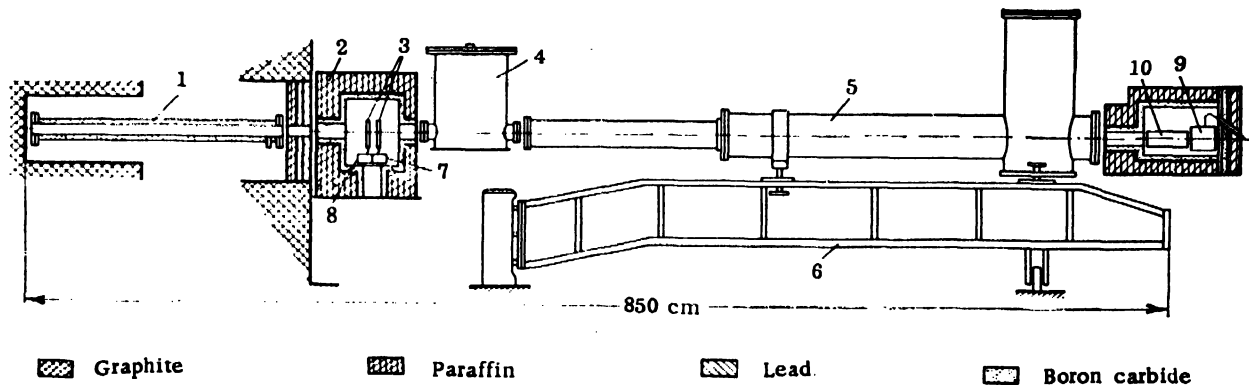
Figure 1. Diagram of installation: (1) collimator; (2) monitor shield; (3) monitor counters; (4) beryllium filter; (5) scattering chamber; (6) movable table; (7) cathode followers I; (8) cathode followers II; (9) cathode followers of the main counter; and (10) main counter
