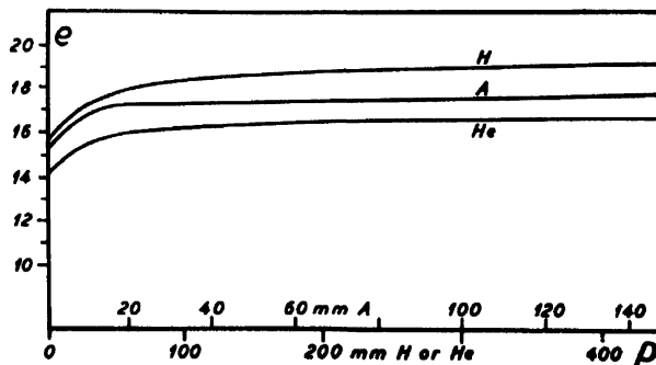
Figure 13. The total charge of the light fragment in hydrogen, helium and argon as function of the pressure
