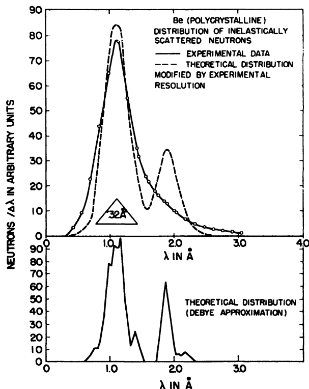
Figure 10. Wave-length spectrum of neutrons after scattering in polycrystalline Be, measured as shown in Fig. 9. Incident neutrons were beryllium filtered ( \lambda > 4.4 \text{ \AA} )
