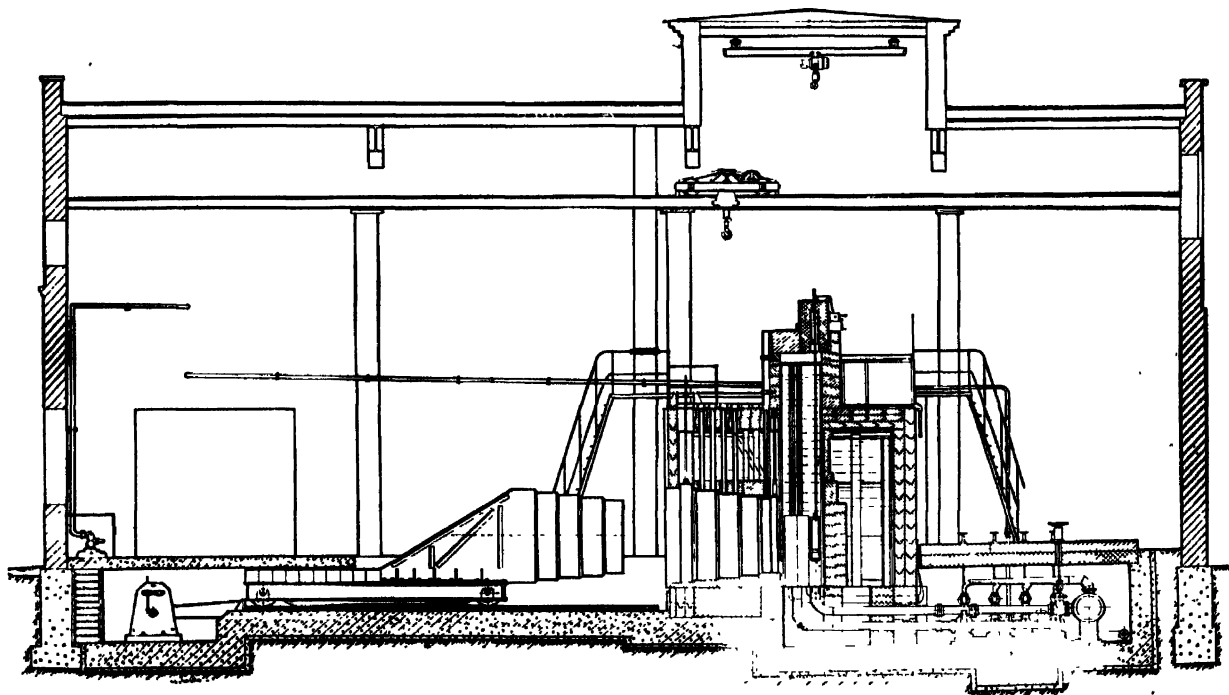
Figure 7. Section of the reactor
