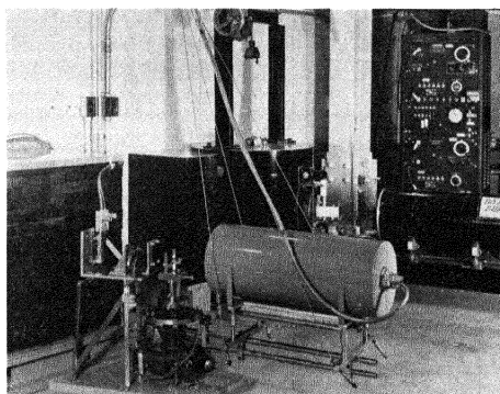
Figure 11. A view of two neutron spectrometers showing the external shielding required to keep the background neutron count low
