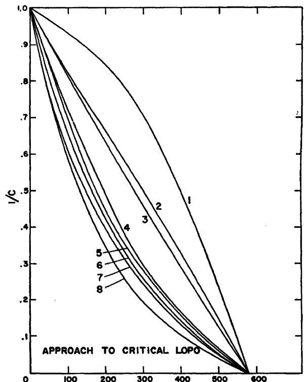
Figure 3. Grams U^{235} in sphere: (1) Mn foils at sphere center; (2) U^{235} chamber 3 in. from center; (3) Mn foils at node of 3rd harmonic; (4) BF_3 + Cd + CH_2 outside reflector, BF_3 + Cd outside reflector; (5) U^{235} chamber against outer sphere surface; (6) BF_3 chamber outside reflector; and (7) In foils 3 in. from sphere surface; (8) In + Cd foils 3 in. from sphere surface
