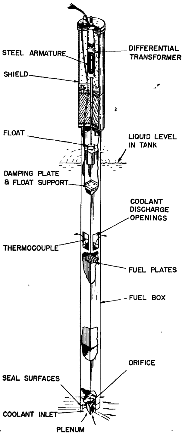
Figure 7. Fuel element
