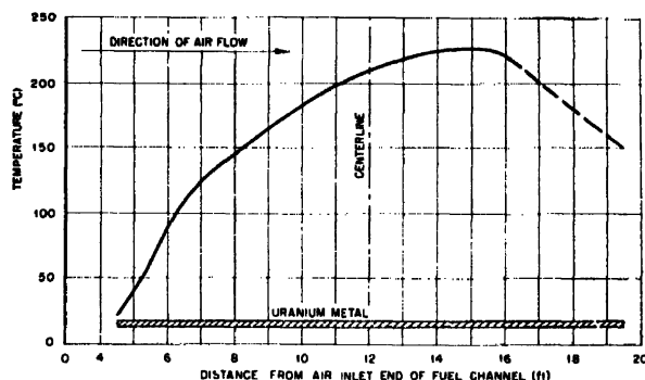
Figure 6. Temperature traverse through a fuel channel showing that the peak temperature is downstream from the reactor center
