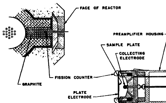
Figure 3. Ionization chamber for fission counting and high neutron flux
