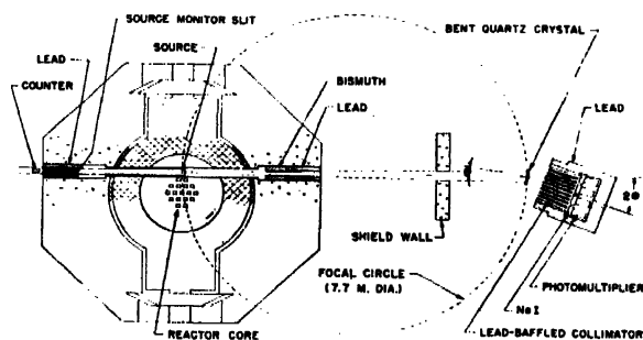
Figure 7. Gamma-ray spectrometer installation
