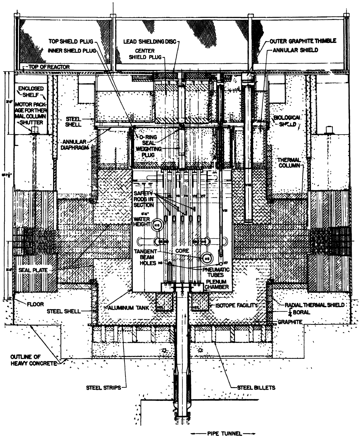
Figure 12. Elevation of research reactor
