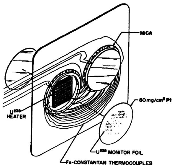
Figure 1. Center plate of the Los Alamos fission calorimeter. The cell on the right contains a heater of U^{235} similar to the U^{235} heater. Flux monitoring foils of U^{235} are on each side of the U^{235} heater
