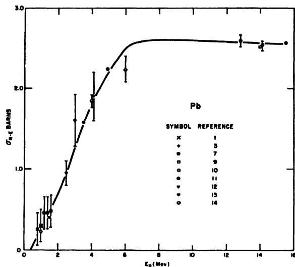
Figure 7. Non-elastic cross section (in barns) of Pb as a function of neutron energy
