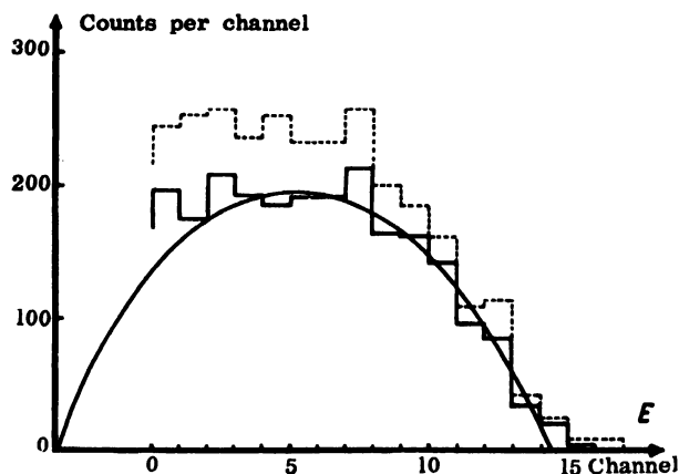
Figure 3. Recoil pulse spectrum for 105^\circ neutrons ( E_n = 2.38 Mev): punctuated curve (histogram), experimental result; smooth curve, corrected for scattered neutrons
