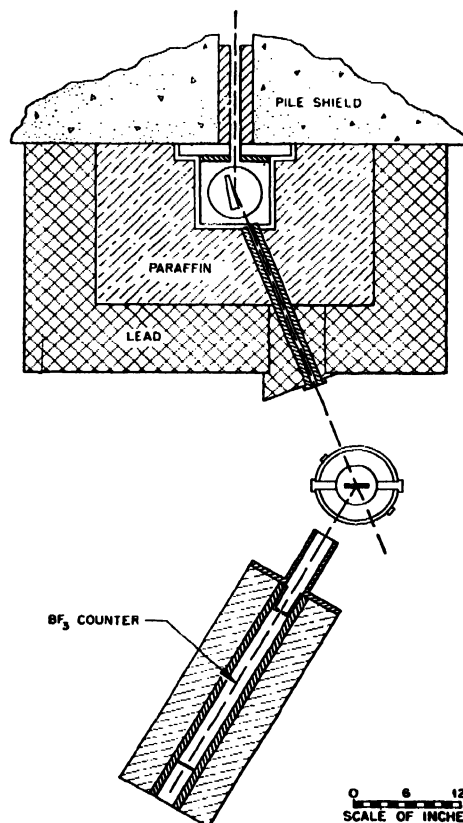
Figure 2. Diagrammatic sketch of neutron spectrometer
