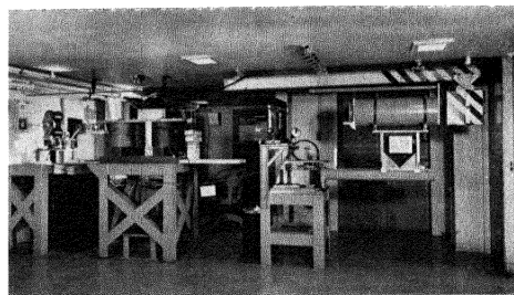
Figure 19. Equipment at a neutron collimator for performing a Stern-Gerlach experiment with neutrons
