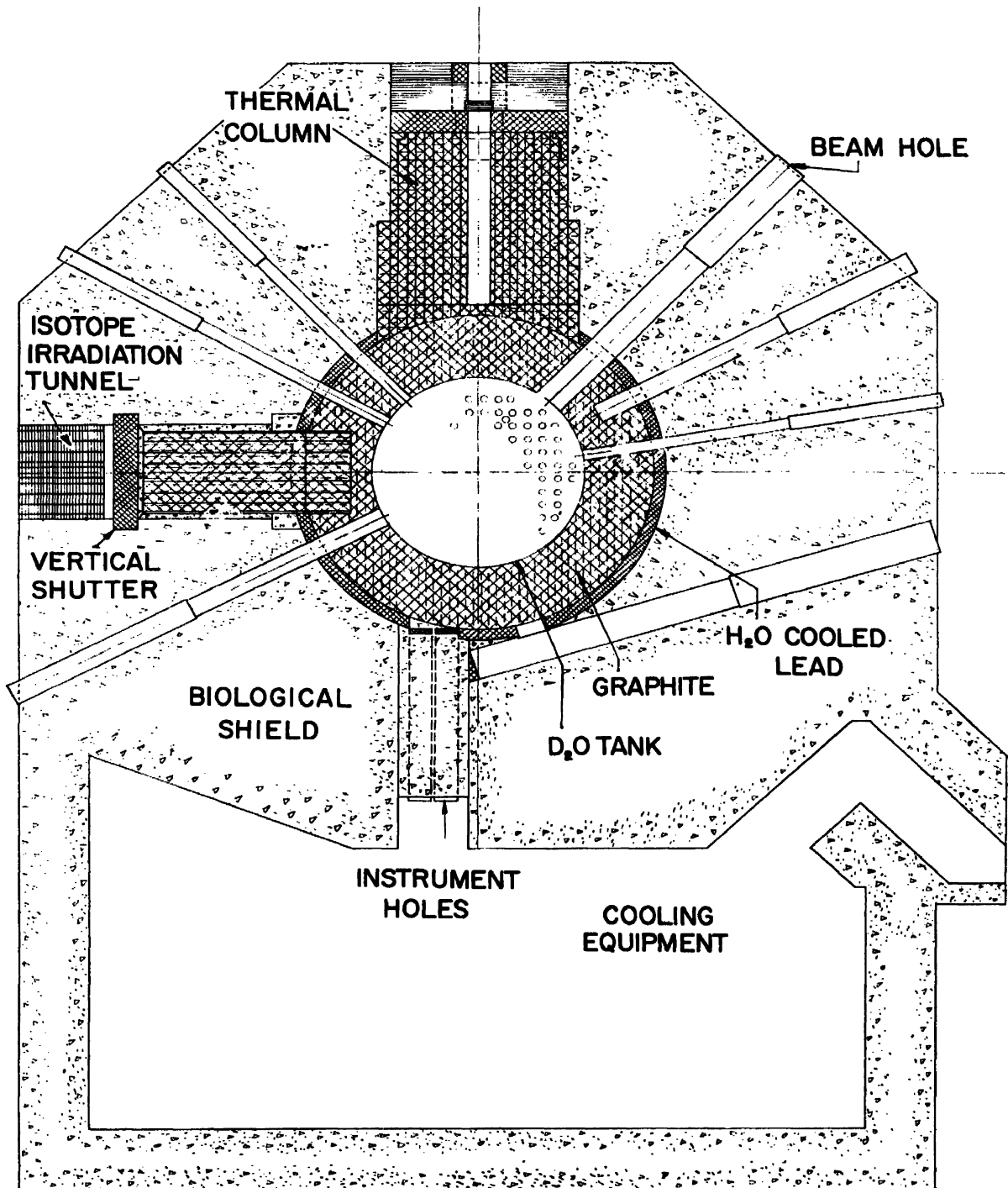
Figure 5. Horizontal section through principal experimental facilities
