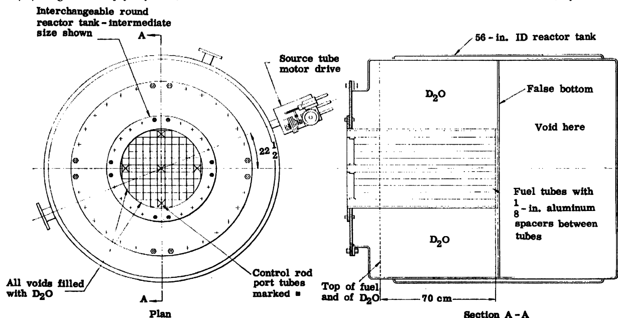
Figure 7. Assembly for \text{D}_2\text{O} reflector
