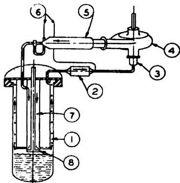
Figure 26. Schematic gas system: (1) spray condenser; (2) steel wool entrainment trap; (3) flow meter; (4) centrifugal pump; (5) catalyst chamber; (6) sampling tubes; (7) reflux condenser; and (8) solution baffle
