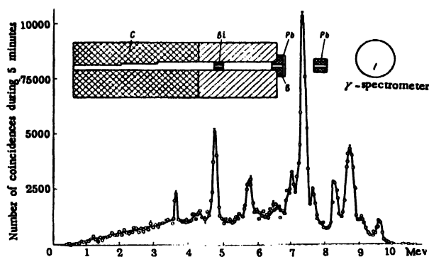
Figure 17. Coincidence gamma-ray spectrum from graphite thermal column
