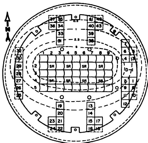
Figure 10. MTR reactor tank horizontal cross section gamma heat flux at midplane
