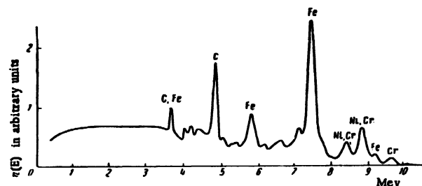
Figure 18. Corrected gamma-ray spectrum from graphite thermal column
