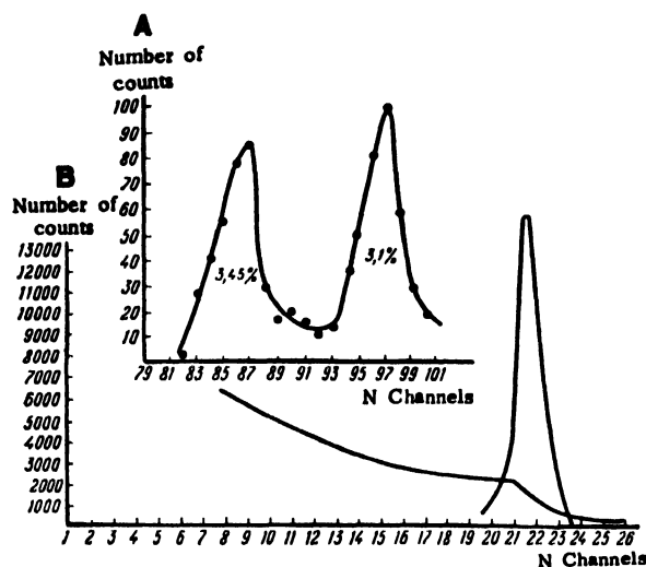
Figure 2. Alpha-particle spectrum (a), and direct neutron beam spectrum (b)
