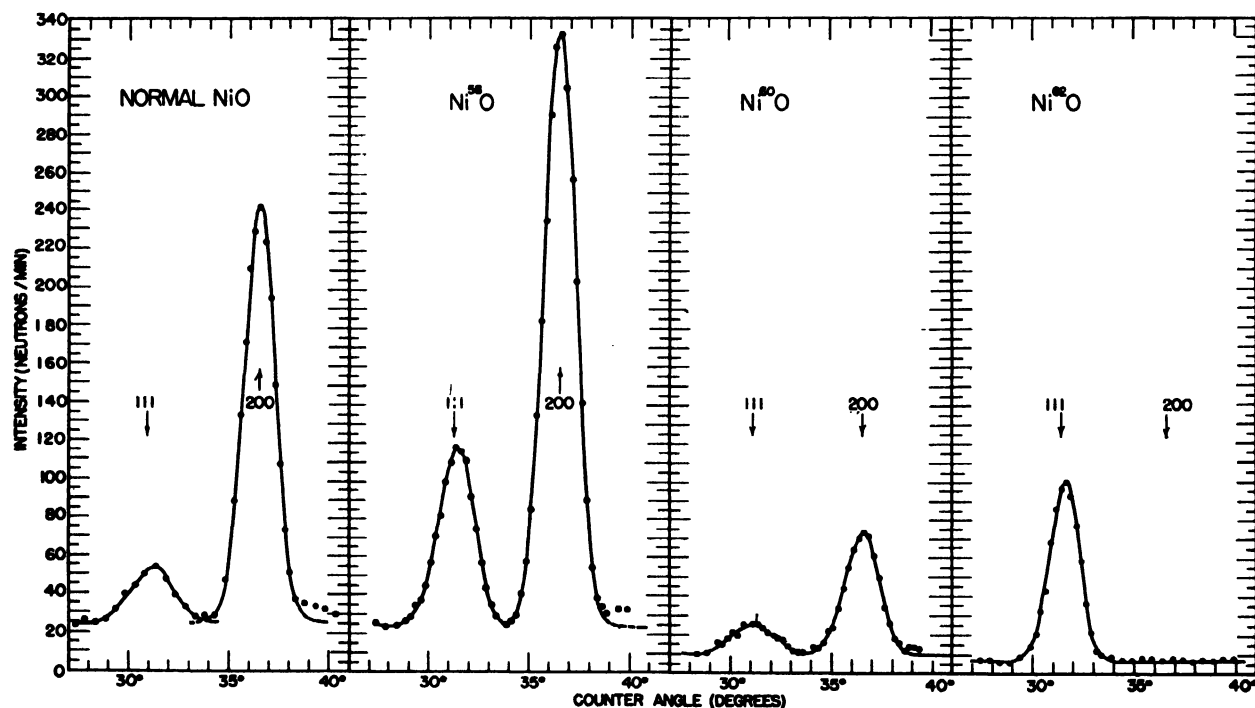
Figure 4. First two diffraction peaks from NiO with normal and isotopically enriched nickel
