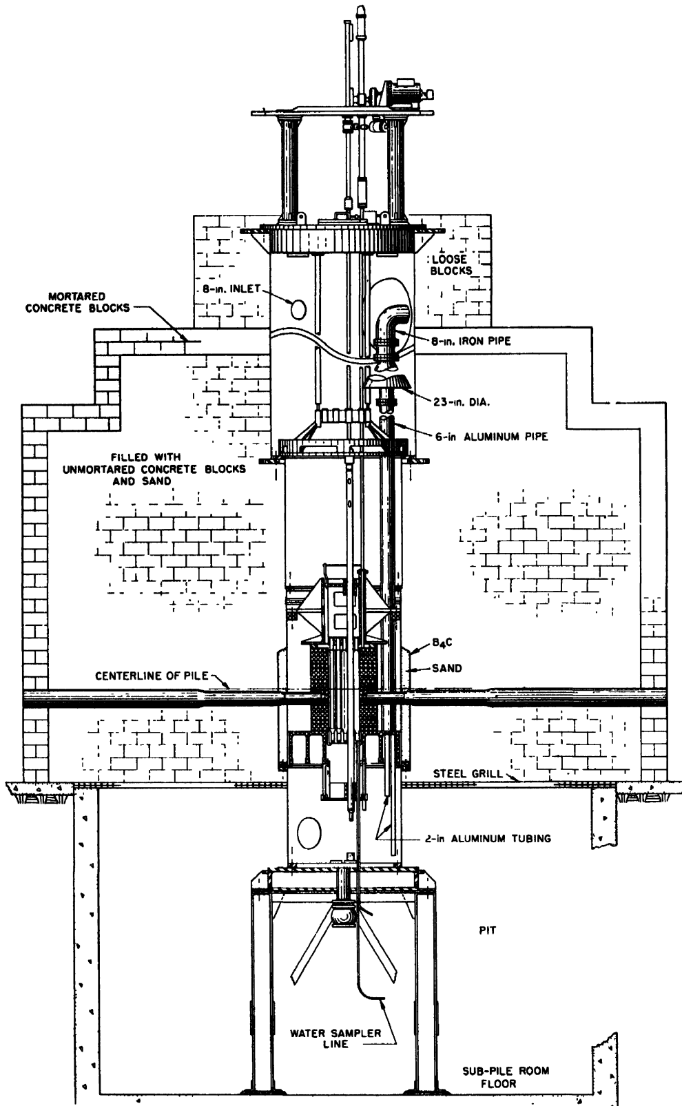
Figure 24. Sectional drawing of the LITR showing the reactor tank, core, beam holes, shielding and internal water lines
