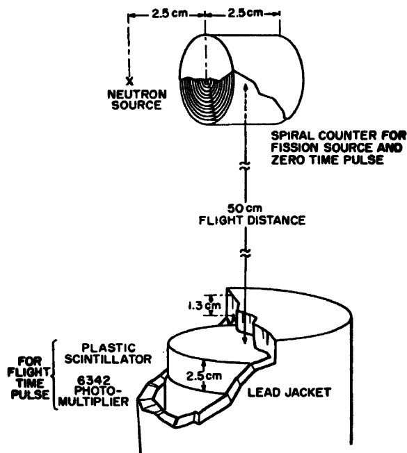
Figure 7. Schematic diagram of the time-of-flight equipment used for energy measurements of fission neutrons
