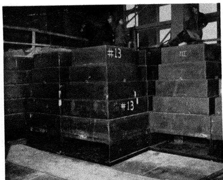
Figure 10. Interlocking and removable shielding blocks installed on the top face
