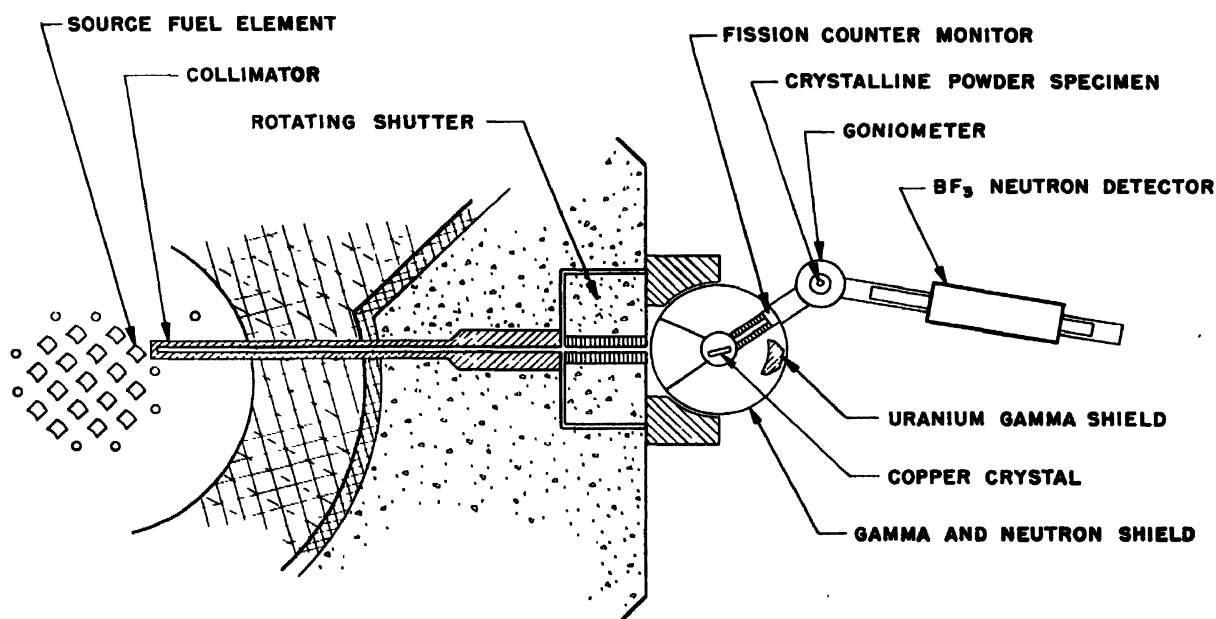
Figure 2. Diagram of the crystal diffraction apparatus
