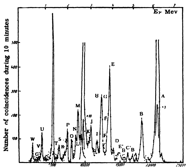
Figure 7. Coincidence gamma-ray spectrum from sodium
