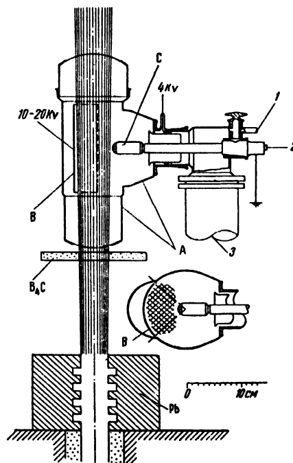
Figure 1. Over-all view of the apparatus: (A) vacuum tank; (B) auxiliary electrode; (1) to glass reservoir; (2) to amplifier; and (3) to pump
