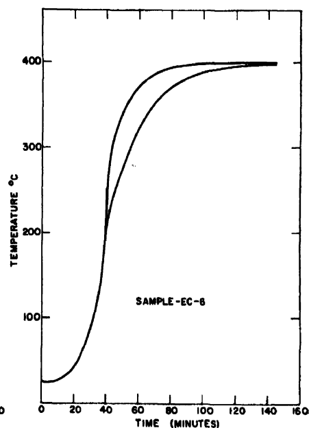
Figure 18. Time vs temperature plot of a graphite sample in a furnace held at 400°C; temperature of irradiation, 60°C
