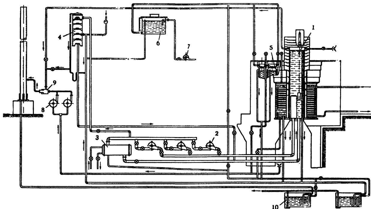
Figure 4. Reactor flow diagram: (1) reactor; (2) centrifugal pump; (3) heat exchanger; (4) de-aerator; (5) storage; (6) water tank; (7) pump; (8) ventilator; (9) air ejector; (10) holding tank
