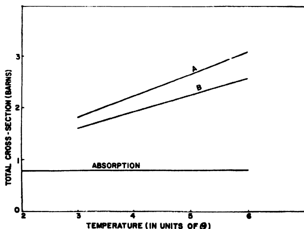
Figure 4. Lead, total cross section against temperature: curve B, total theoretical cross section using incoherent approximation of Placzek; curve A, total theoretical cross section with correction included
