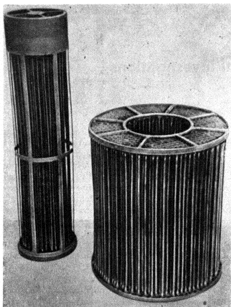
Figure 2. Mobile and stationary parts of the core
