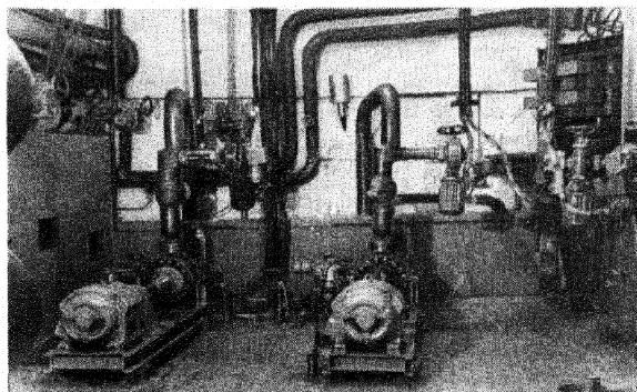
Figure 23. High pressure circulation pumps of the "loop" with water cooling
