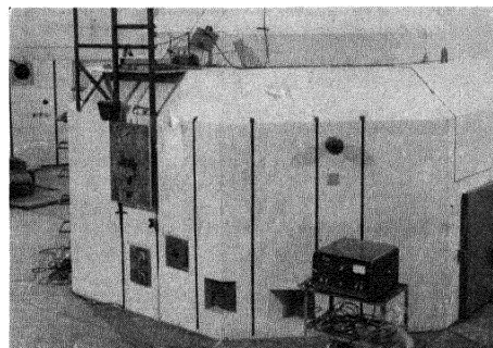
Figure 1. The shield assembly of the Raleigh Research Reactor
