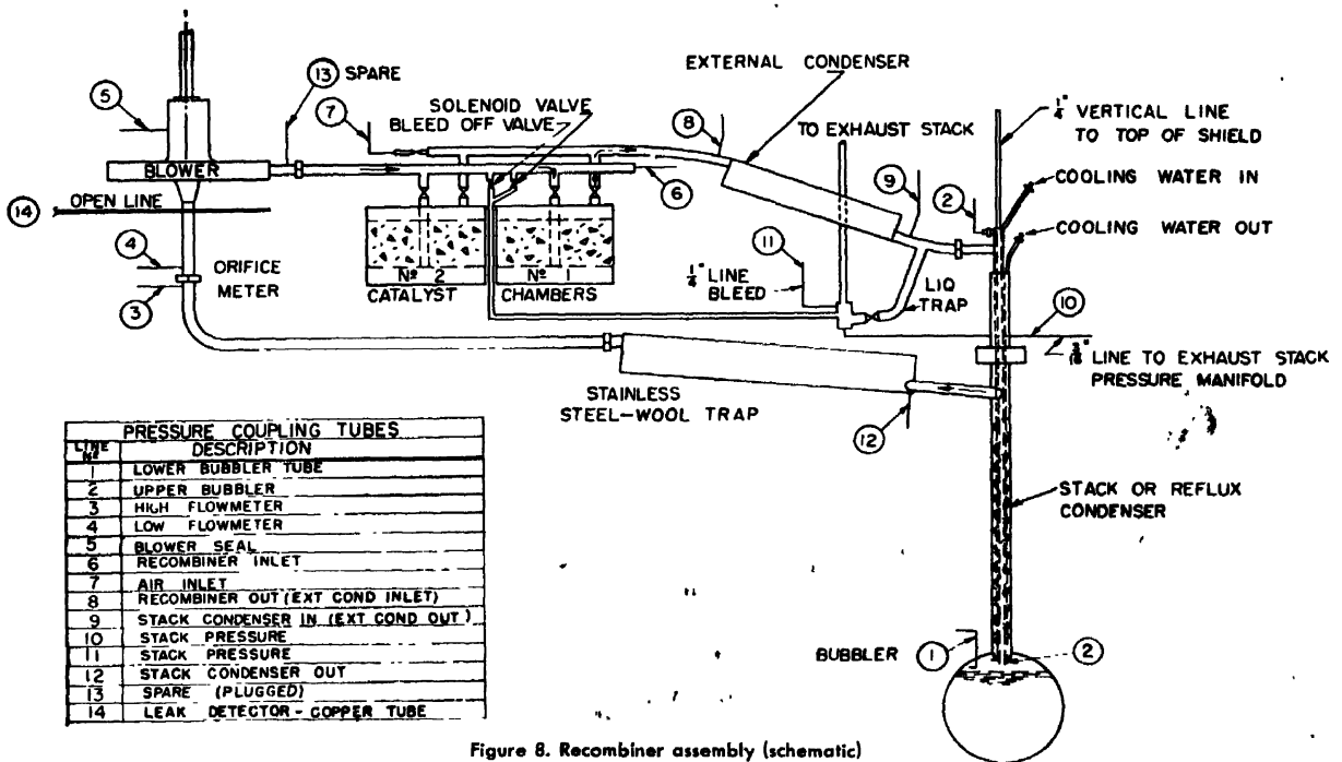
Figure 8. Recombiner assembly (schematic)
