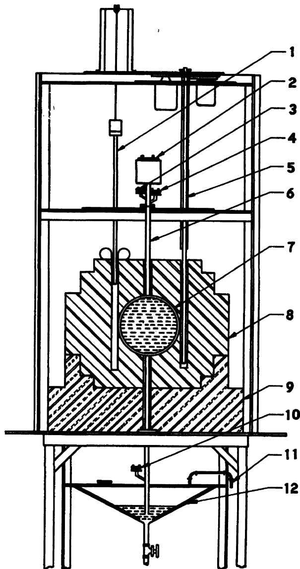
Figure 1. Cross section, LOPO: (1) Cd safety curtain; (2) overflow; (3) safety electrode; (4) level electrode; (5) Cd control rod; (6) upper pipe; (7) stainless steel sphere containing enriched uranyl sulfate ( \text{UO}_2\text{SO}_4 ); (8) BeO reflector; (9) graphite reflector; (10) level electrode; (11) air pipe; (12) dump basin
