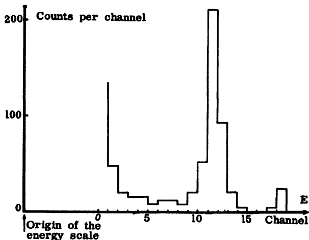
Figure 4. Pulse height distribution for the \text{O}^{16}(n,\alpha)\text{C}^{13} reaction at E_n = 4.11 Mev
