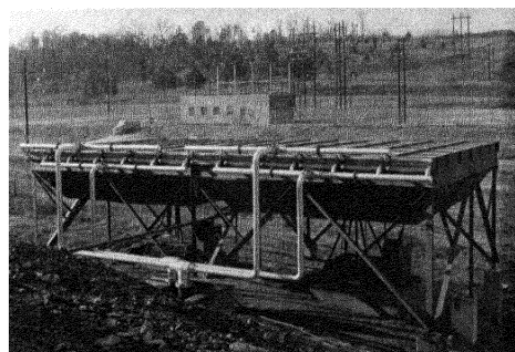
Figure 32. The water-to-air heat exchangers used for removing heat from the reactor cooling water
