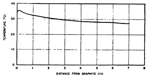
Figure 3. Temperature traverse through the concrete shield of the graphite reactor showing that gamma heating is not excessive nor is the temperature differential through the shield great enough to cause severe stresses
