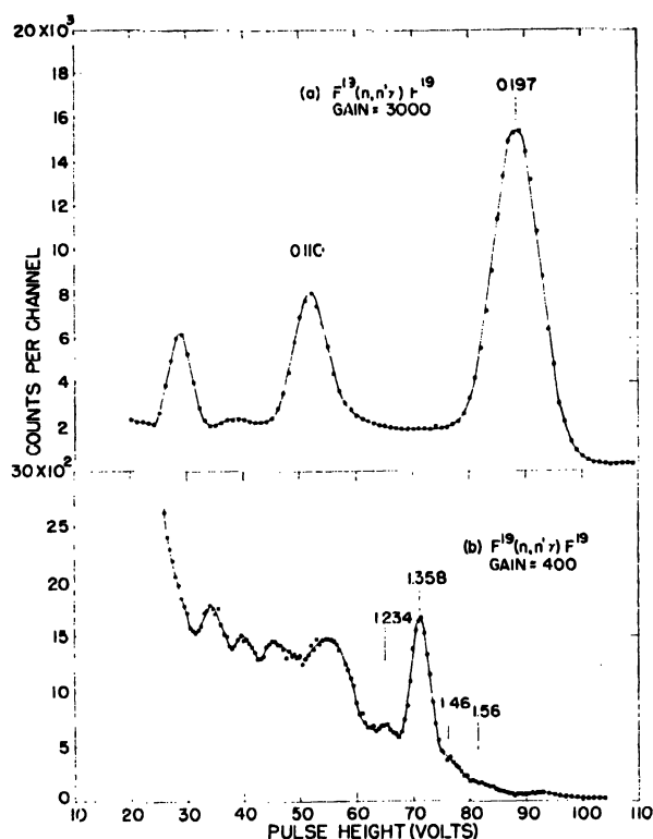
Figure 3. Pulse-height distributions obtained with a Teflon ring scatterer ( CF_2 ). The photopeaks of the gamma rays produced in F^{19} are identified by their energies in Mev. The amplifier gain has been changed in the two pulse-height distributions
