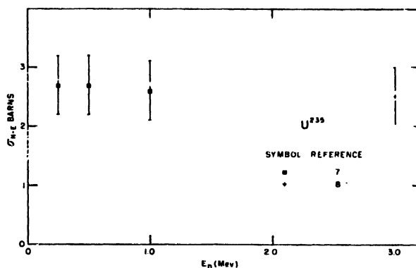
Figure 11. Non-elastic cross section of U^{235}
