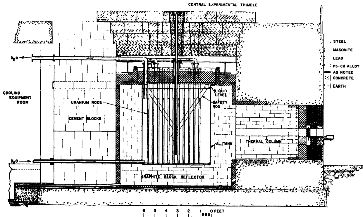
Figure 1. Vertical section of natural uranium heavy water research reactor
