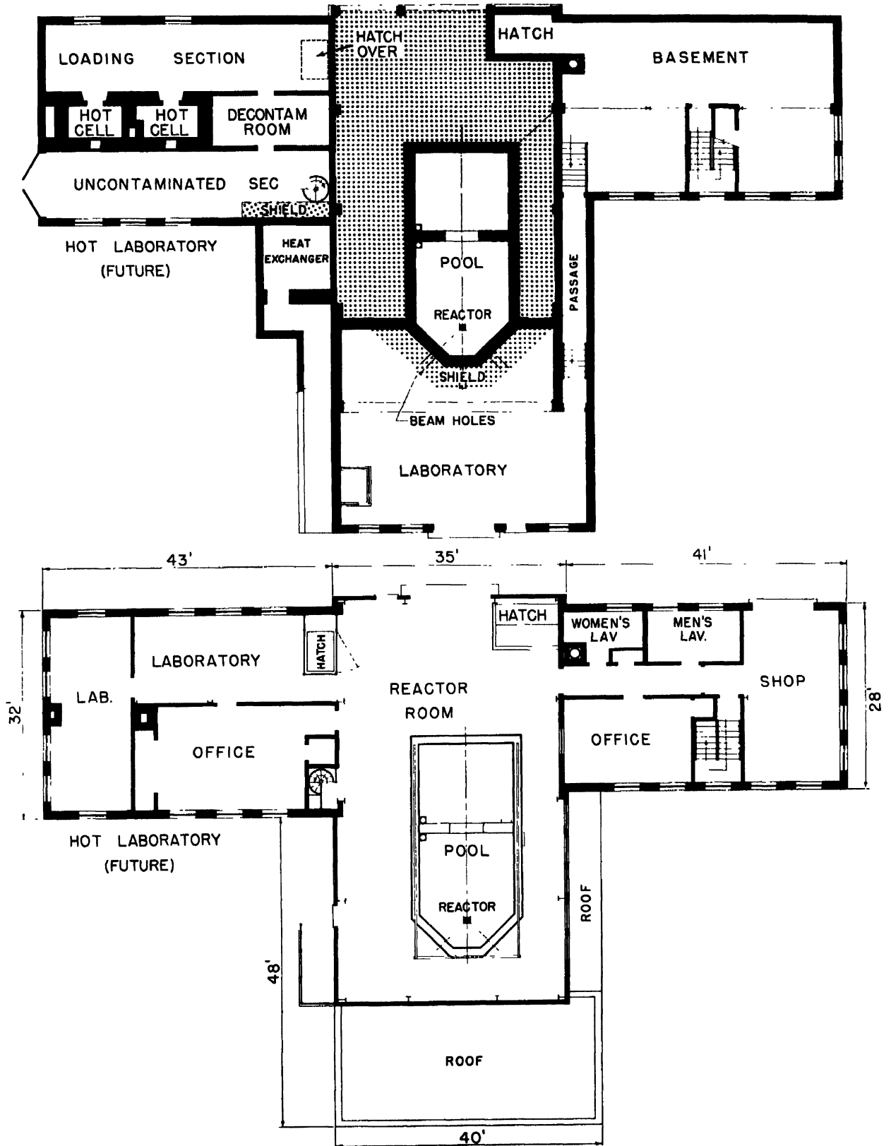
Figure 2. (At top) The Pennsylvania State University reactor facility: basement and laboratory Figure 3. (At bottom) The Pennsylvania State University reactor facility: main floor
