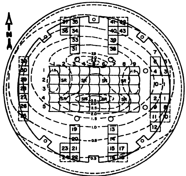
Figure 8. MTR reactor tank horizontal cross section maximum thermal flux values at midplane
