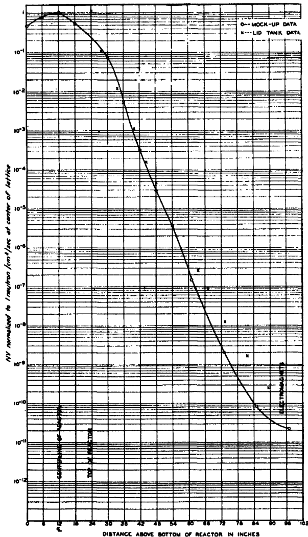
Figure 14. Neutron attenuation in water above reactor lattice: o = mock-up data, x = lid tank data
