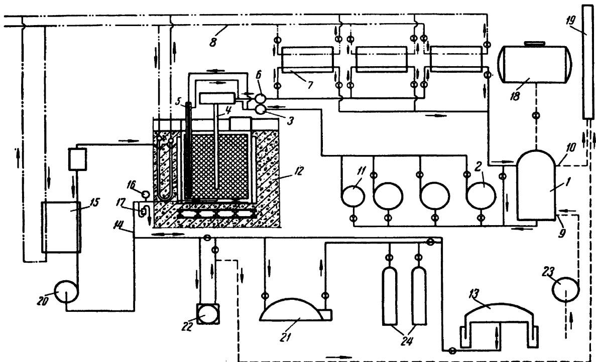
Figure 12. Flow diagram: (1) degassing tank; (2) centrifugal pumps; (3) distributor; (4) fuel assembly; (5) cooling channels in the reflector; (6) collector; (7) heat-exchangers; (8) pipe-line for river water; (9) air-pipe; (10) pipe-line to the ventilation stack; (11) emergency pump; (12) reactor shell; (13) gas holder; (14) helium pipe-line; (15) gas cooler; (16) water detector; (17) water lock; (18) emergency supply of distilled water; (19) ventilation stack; (20) gas blower; (21) compressor; (22) vacuum pump; (23) ventilator; and (24) helium storage
