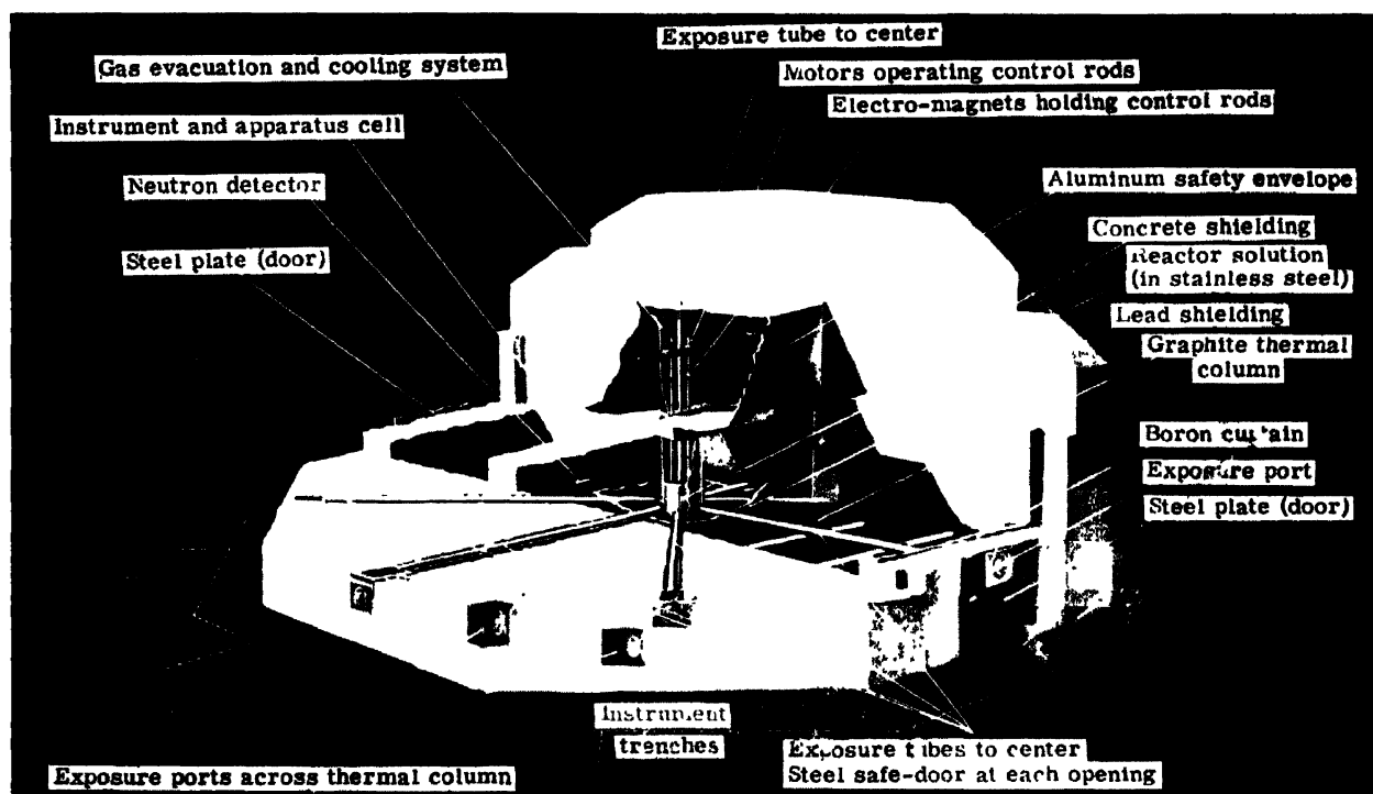
Figure 17. Raleigh reactor, North Carolina State College
