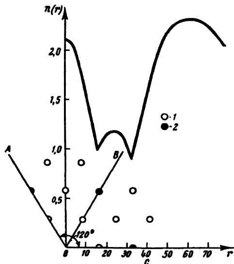
Figure 4. Thermal neutron flux along symmetrical directions OA, OB and OC; (1) uranium rods; (2) absorbing rods
