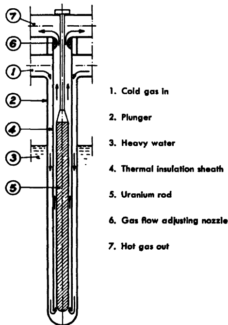
Figure 2b. Details of a reactor cell
