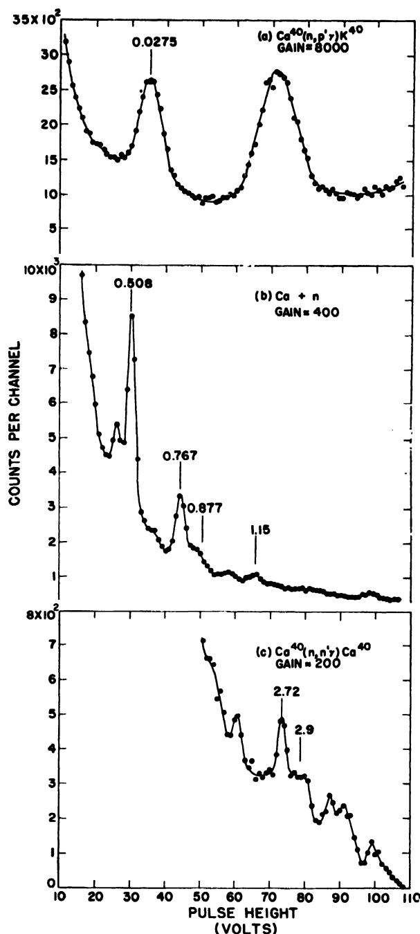
Figure 4. Pulse-height distributions obtained with a Ca ring. The photopeaks of the gamma rays produced by neutron interactions with Ca are identified by their energies in Mev; however, in (c) the peaks identified are the pair peaks of 3.74- and 3.9-Mev gamma rays
