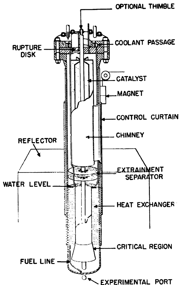
Figure 28. Test tube reactor
