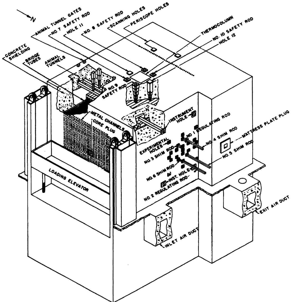
Figure 1. A cutaway sketch of the normal-uranium, graphite-moderated reactor
