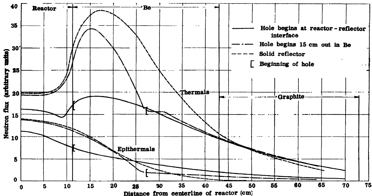
Figure 12. 4-kg slab reactor ( 71 \times 22.5 \times 66 cm); 2% H_2O in Be: neutron distributions along axis of 6-in. hole at edge of reactor
