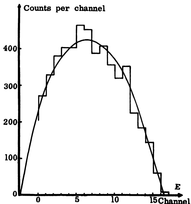
Figure 2. Recoil pulse spectrum due to forward neutrons, E_n = 3.65 Mev: histogram, experimental curve; smooth curve, theoretical curve
