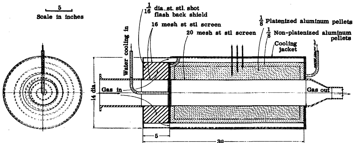
Figure 27. Catalyst chamber, Supo II
