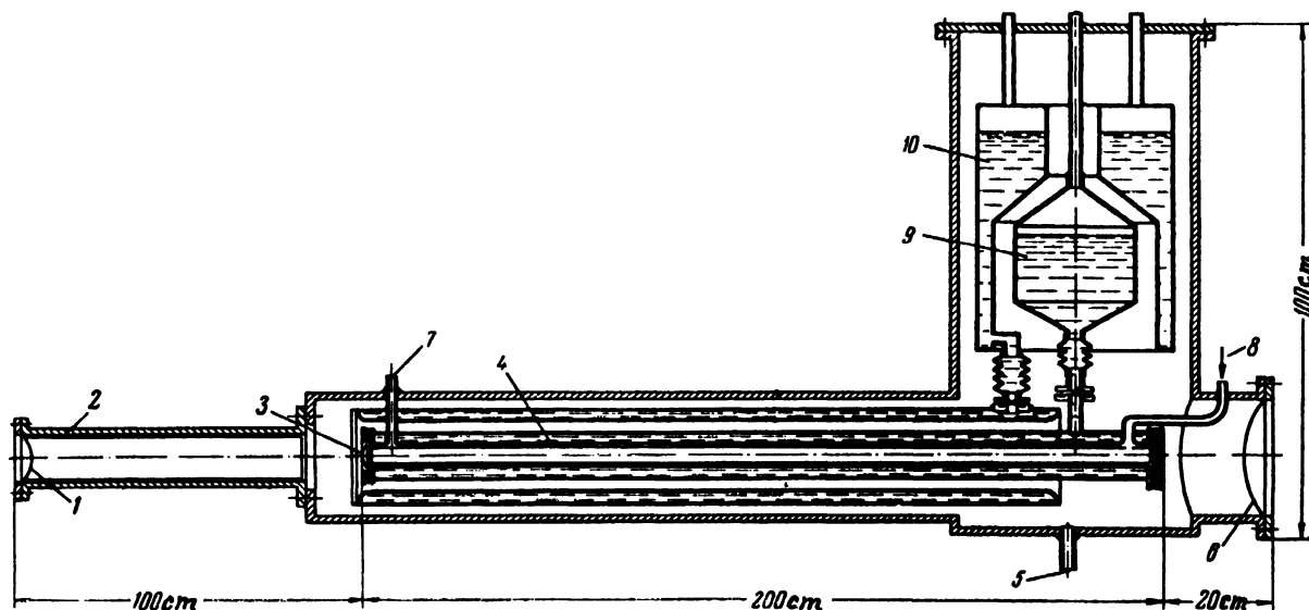
Figure 2. Scattering chamber: (1) aluminium window, 0.2 mm thick; (2) cadmium; (3) aluminium window, 0.2 mm thick; (4) cadmium; (5) diffusion pump; (6) aluminium window, 0.2 mm thick; (7) and (8) filling system; (9) liquid hydrogen; and (10) liquid nitrogen
