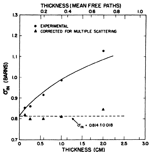
Figure 6. Cross section for excitation of the 850-keV gamma ray in Fe by neutron inelastic scattering as measured with rings of different sizes. The inner and outer diameters were 5.08 cm and 7.08 cm, respectively, with only the axial thickness being varied. The circles give the cross sections calculated from Equation 1, while the triangles give these cross sections after correction for multiple neutron scattering. The solid curve shows the theoretical variation of the gamma-ray yield caused by multiple scattering
