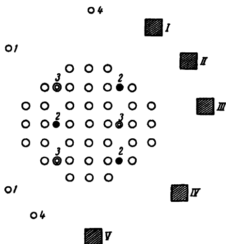
Figure 7. Arrangement of control rods and "loop" channels: (1) rods for automatic control; (2) shim rods, manual; (3) shim rods, automatic; (4) safety rods. "Loop" channels: (I) with gas cooling; (II) with high pressure water cooling; (III) with liquid metals cooling; (IV) with medium pressure water cooling; and (V) with high pressure water cooling
