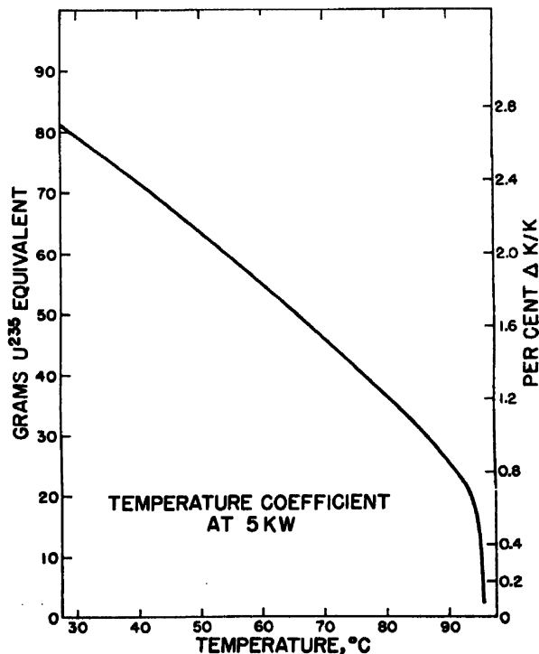
Figure 16. Temperature coefficient at 5 kw
