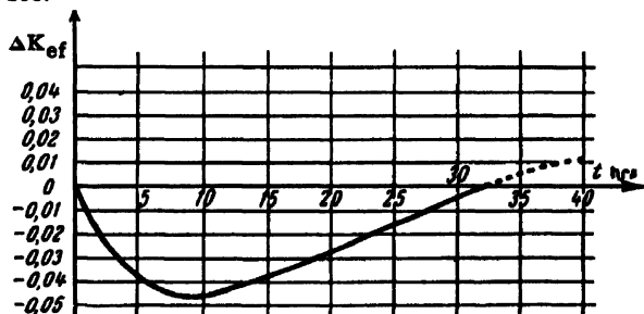
Figure 8. Drop in reactivity after the reactor is shut down (time after shutdown on the abscissa)
