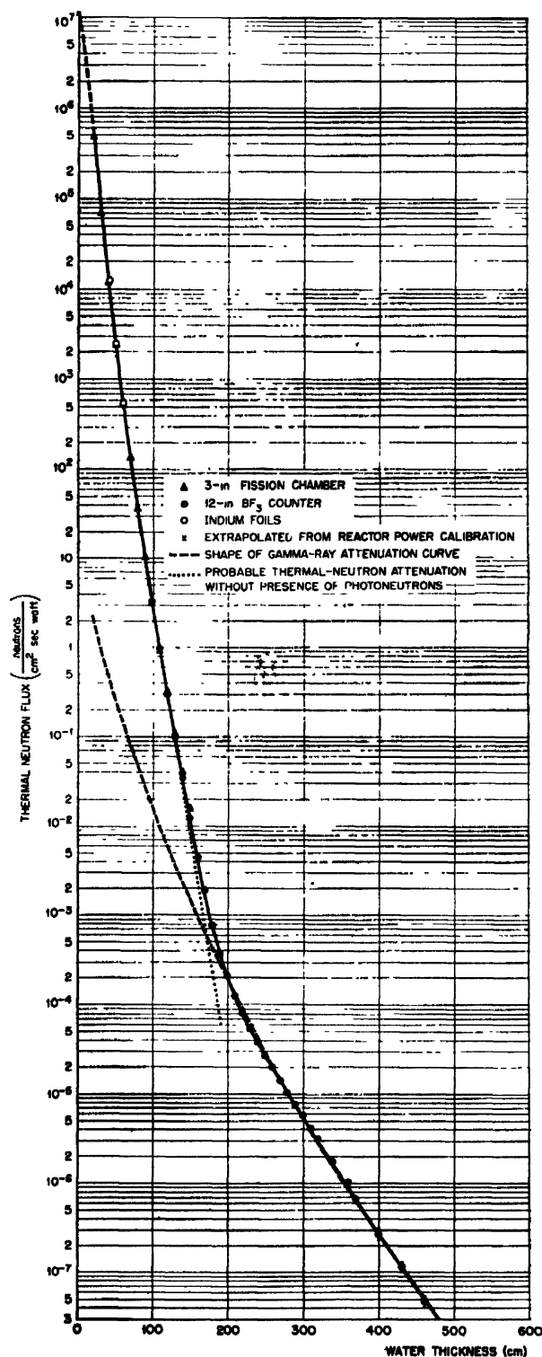
Figure 18. Thermal-neutron flux as a function of distance from the Bulk Shielding Reactor
