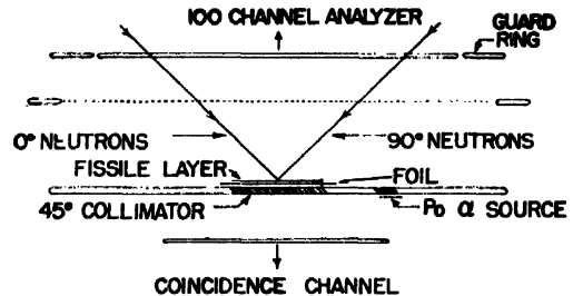
Figure 15. Schematic diagram of the fragment angular correlation experiment. Fission fragments in the upper ionization chamber are recorded only when in coincidence with complimentary fragments that go through the collimator into the lower ionization chamber
