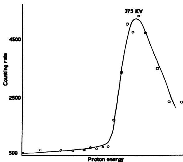
Figure 6. Gamma radiation from copper excited by proton bombardment
