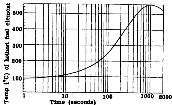
Figure 16. Heating of fuel elements after shutdown from 2000 kw: no water or helium in reactor tank
