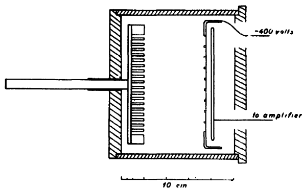
Figure 2. Arrangement for measuring the specific ionization by fission fragments along the path
