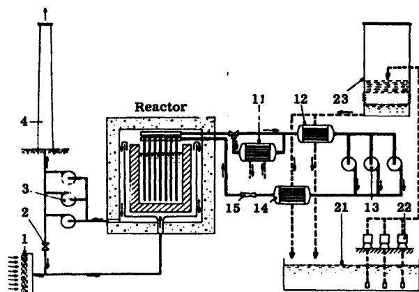
Figure 2a. Cooling circuit schematic. Air: 1. filter; 2. by pass; 3. fans. Nitrogen: 11. heat exchanger for heating building; 12. main heat exchanger; 13. blowers 14. auxiliary heat exchanger; 15. venturi. Water: 21. pool; 22. pumps; 23. cooling tower
