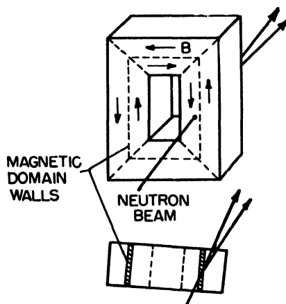
Figure 8. Experimental arrangement for direct observation of refraction and depolarization of neutron beams at a single magnetic domain boundary. Beam polarization arrangement is shown in Fig. 1
