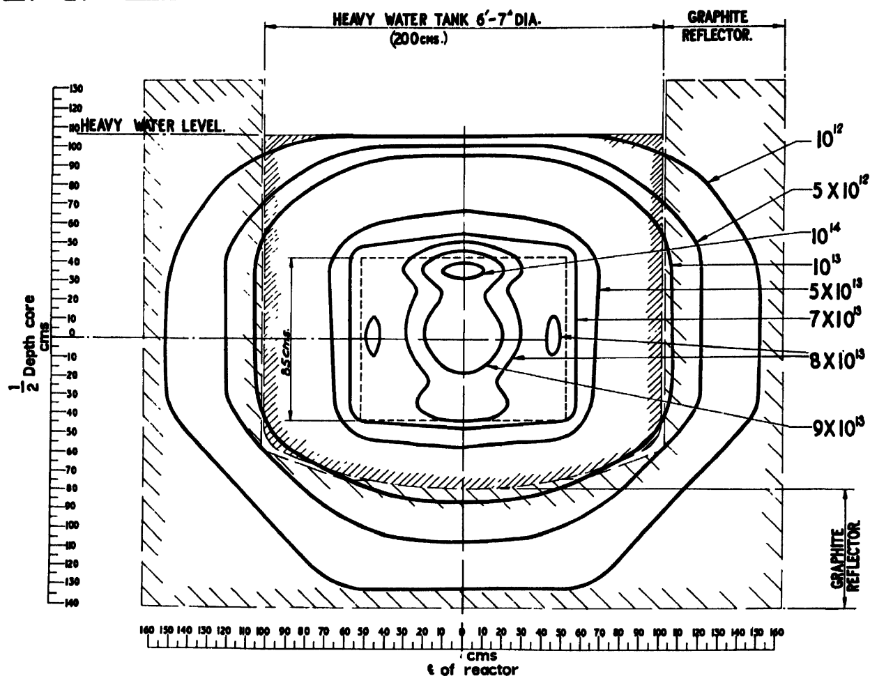
Figure 3. Undisturbed thermal flux distribution n/\text{cm}^2/\text{sec} in E.443
