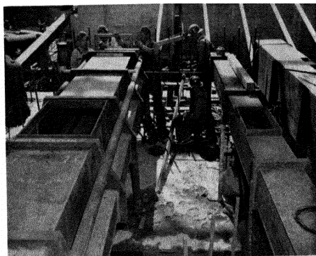
Figure 11. Steel liners being installed in foundation of the Brookhaven reactor to provide irradiation tunnel facilities on bottom face
