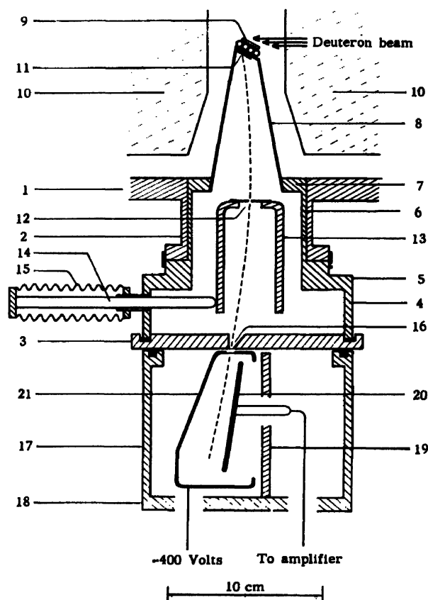
Figure 8. Apparatus for measuring the deflection of fission fragments in a magnetic field
