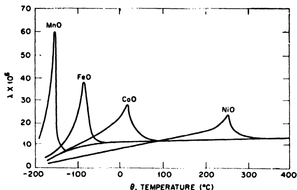
Figure 22. Thermal expansion of various oxides in the temperature regions of the antiferromagnetic transitions (Foex)
