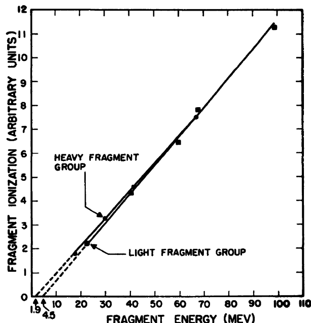
Figure 3. Energy-ionization relation of fission fragments in nitrogen
