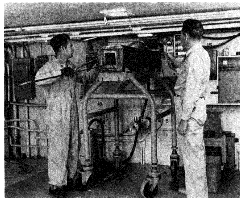
Figure 15. A view of operators removing radioisotope targets from a "stringer" hole. Notice the vacuum cleaner which removes dust from the graphite tray as it is withdrawn from the reactor through a lead shield
