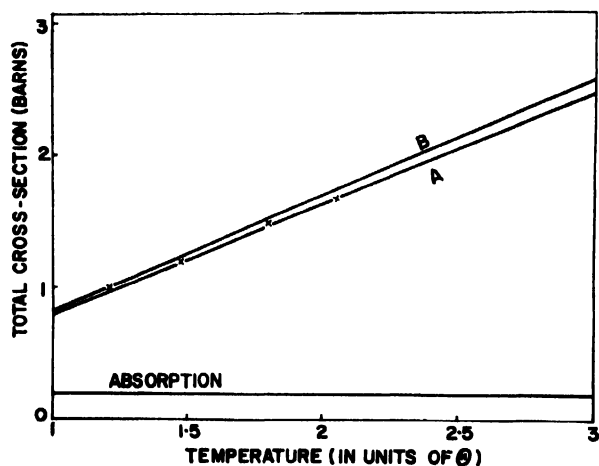
Figure 1. Magnesium, total cross section against temperature: curve B, total theoretical cross section using incoherent approximation of Placzek; curve A, total theoretical cross section with correction included; X, experimental points (Squires)
