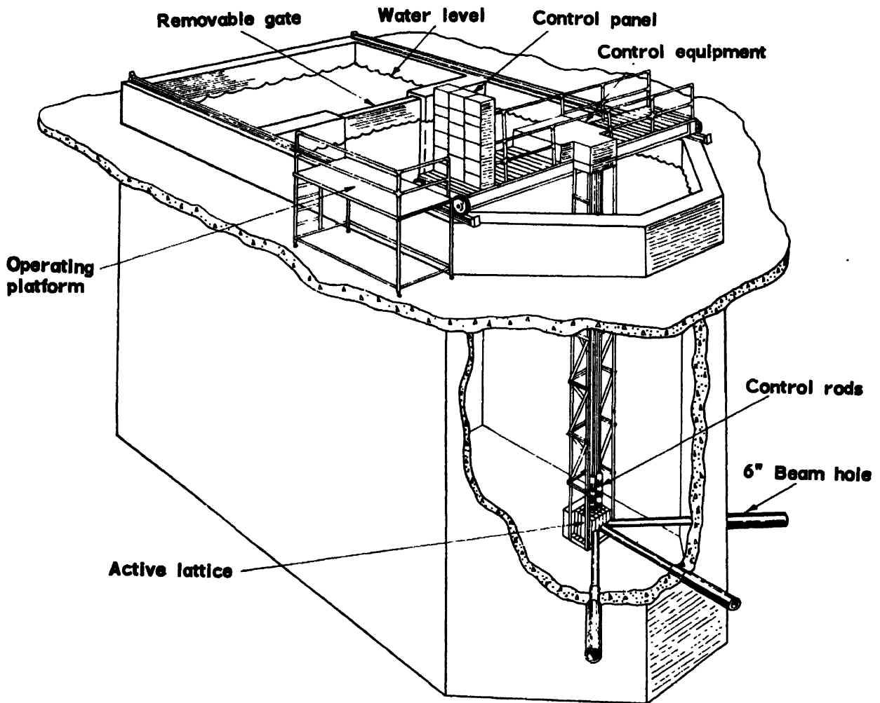
Figure 1. Open pool reactor
