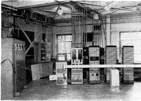
Figure 33. The chopper type neutron velocity selector used for cross-section measurements in the dE/E neutron region. The beam strength for these neutrons is 2 \times 10^{12} n/cm 2 -sec
