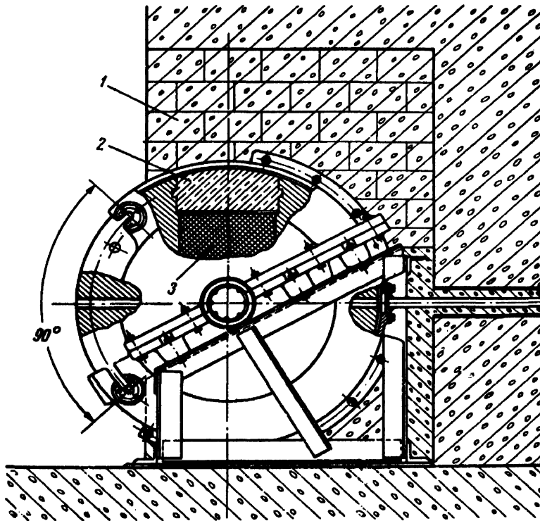
Figure 11. Beam hole shutter: (1) shielding bricks; (2) lead, and (3) paraffin
