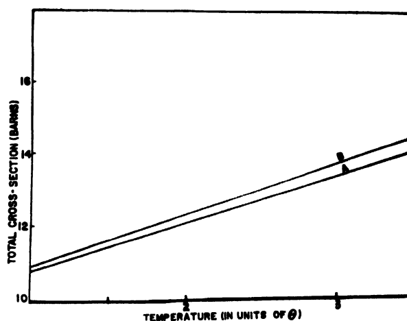
Figure 3. Iron, total cross section against temperature: curve B, total theoretical cross section using incoherent approximation of Placzek; curve A, total theoretical cross section with correction included; X, experimental points (Squires) including magnetic scattering
