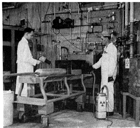
Figure 35. Lead shield for the beam hole shield plugs. The vacuum cleaner is used throughout any removal of plugs or experiment pieces to clean up radioactive dust
