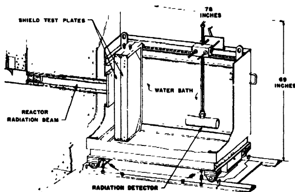
Figure 11. Shield test apparatus
