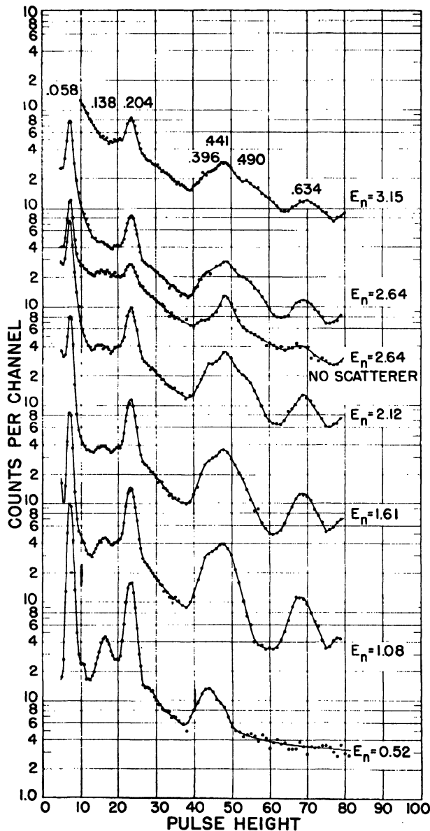
Figure 2. Low-energy background pulse-height distribution produced by neutrons of the energies shown, normalized to a constant neutron flux incident on the scatterer. A carbon ring scatterer was used in the arrangement illustrated in Fig. 1. Photopeak energies are given in Mev just above the top curve. The ordinate changes by a factor of 10 for each energy; however, the same scale is used for the two curves at E_n = 2.64 Mev
