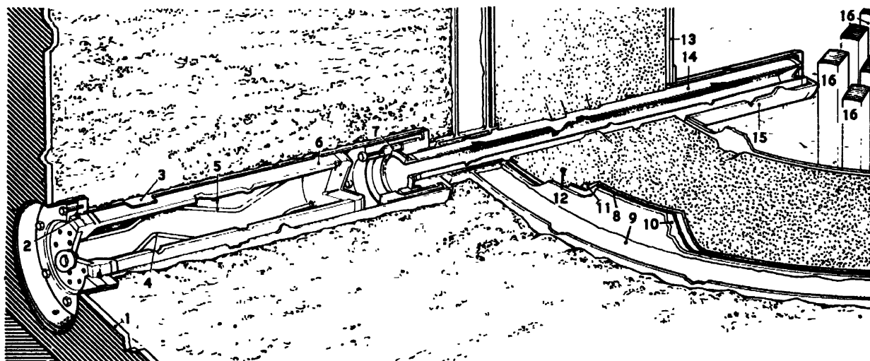
Figure 4. Reactor E.443: 6 in. horizontal experimental hole entering heavy water. (1) Steel facing on outside concrete biological shield; (2) gas sealing of shield plug; (3) steel liner tube in concrete shield; (4) shielding plug; (5) tip water cooling line; (6) biological shielding plug (concrete filling not shown); (7) aluminium liner tube sealing arrangement; (8) steel vessel; (9) lead thermal shield; (10) boron sheet; (11) lead; (12) graphite; (13) heavy water tank; (14) aluminium liner tube 6 in. inside diameter (removable); (15) fixed re-entrant aluminium tube from heavy water tank; and (16) fuel elements
