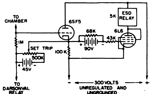
Figure 7. Electronic relay
