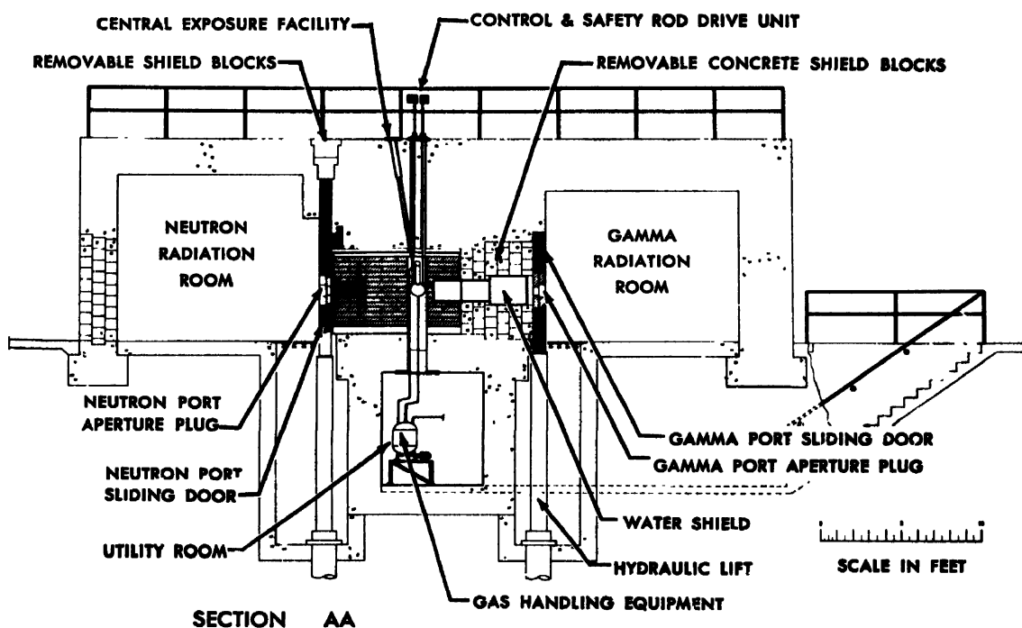
Figure 21. NAA medical reactor, side view
