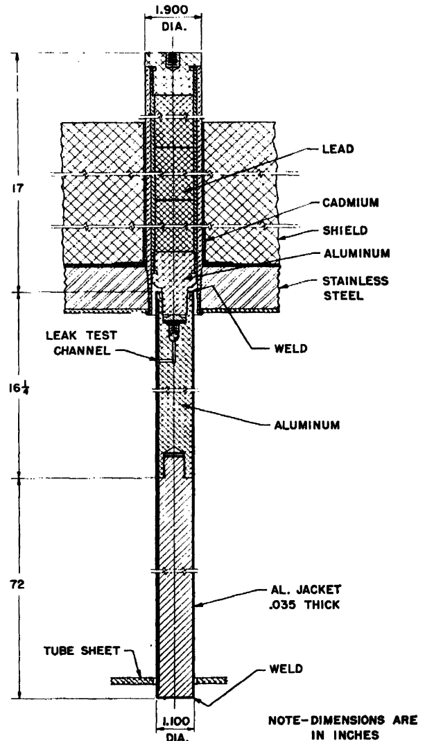
Figure 3. Natural uranium fuel rod
