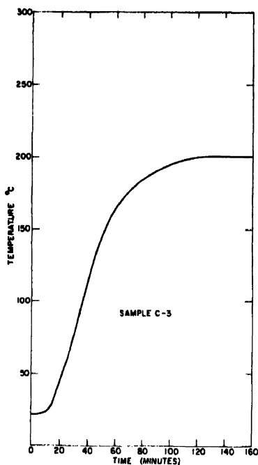
Figure 15. Time vs temperature plot of a graphite sample in a furnace held at 200°C; temperature of irradiation, 150°C
