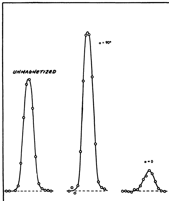
Figure 10. Influence of magnetic field orientation on ferromagnetic scattering in (111) reflection of \text{Fe}_3\text{O}_4
