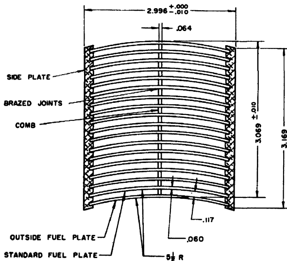
Figure 1. MTR cross section of fuel assembly
