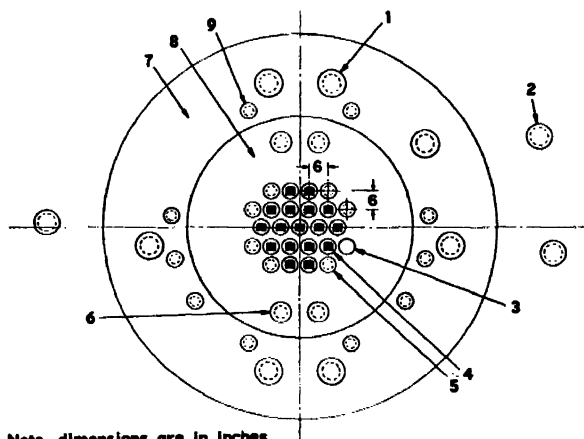
Figure 8. Fuel elements and experimental thimbles: (1) 5\frac{3}{4} dia. exp. thimble holes in graphite; (2) 6 dia. storage holes for radioactive samples; (3) Regulating rod; (4) Fuel elements; (5) 3\frac{1}{8} dia. exp. thimble holes in D_2O ; (6) 4 dia. exp. thimble holes in D_2O ; (7) Graphite zone; (8) D_2O zone; (9) 3\frac{3}{16} dia. exp. thimble holes in graphite
