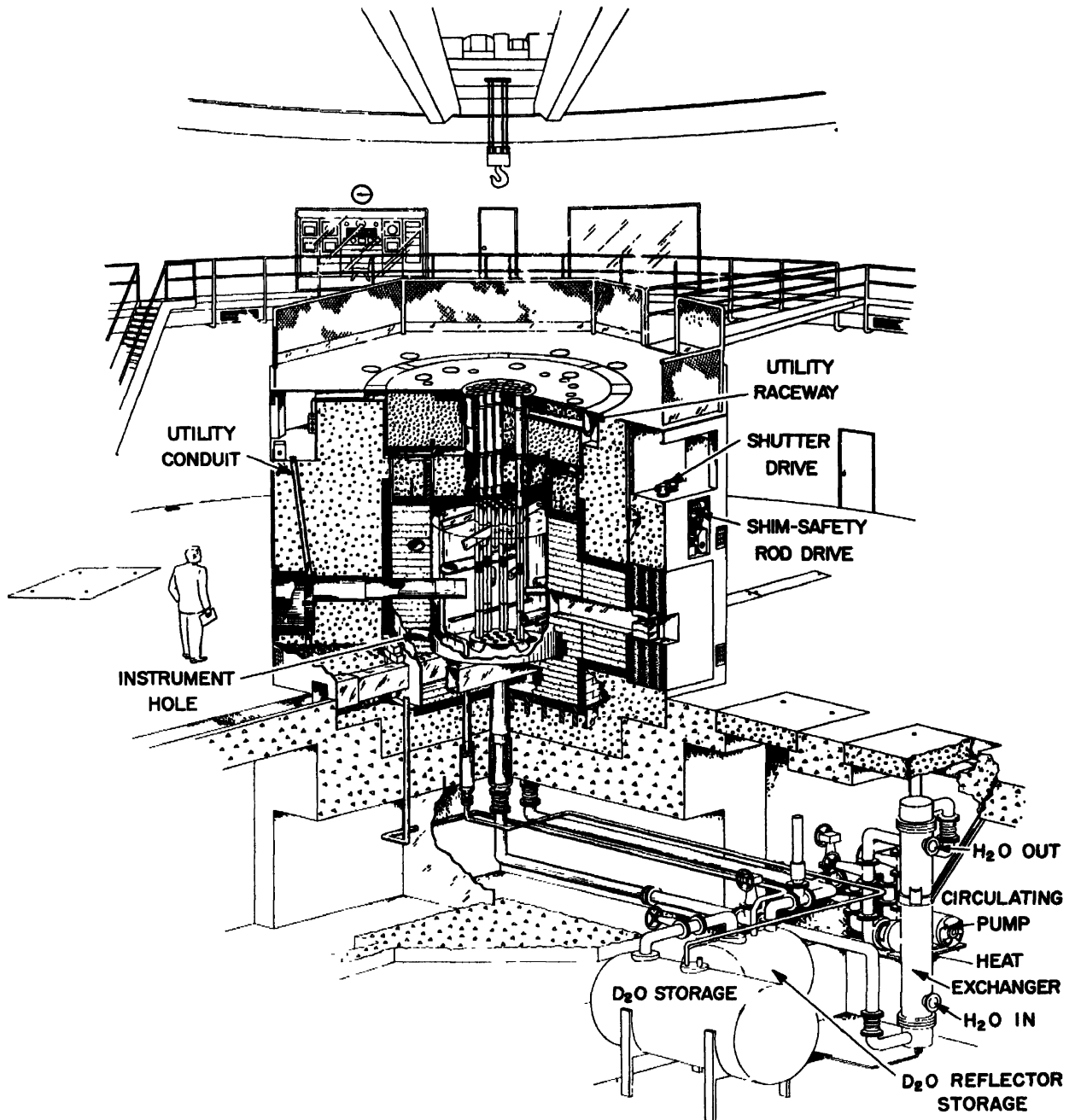
Figure 14. Pictorial assembly and research reactor
