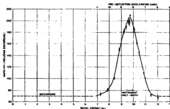
Figure 2. Singly-charged \text{Cl}^{37} neutrino recoils: magnet set at 3713 hp
