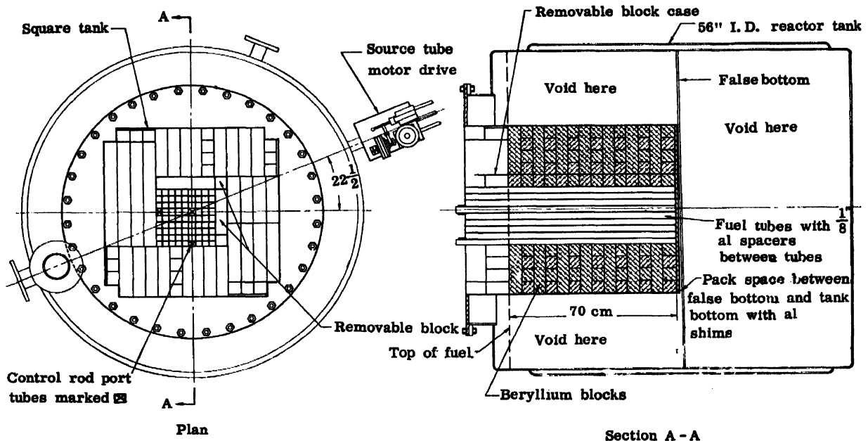
Figure 8. Assembly for beryllium reflector
