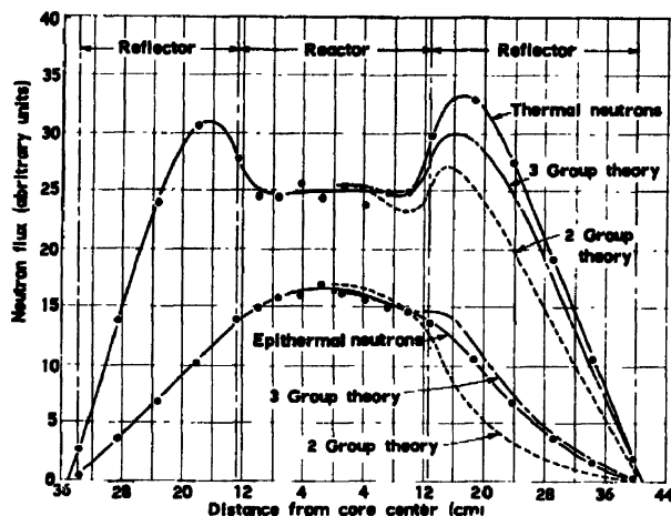
Figure 10. Radial neutron distributions; beryllium reflector
