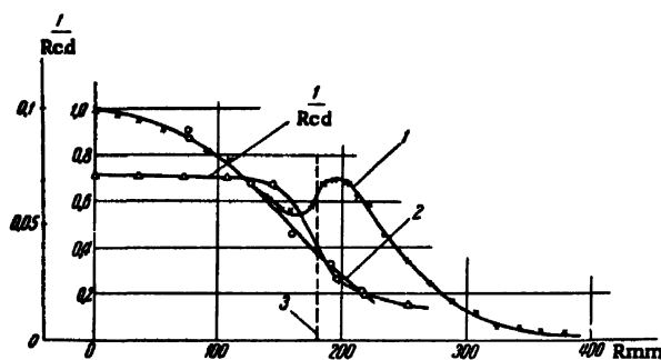
Figure 15. Thermal and resonance neutron distributions along the core radius: (1) thermal neutrons; (2) resonance neutrons; and (3) core boundary
