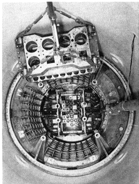
Figure 30. Looking down into the reactor tank as assembled for 500 kw operation. The return water line from the bottom section is now 8 inches in diameter. The upper assembly of grids hangs from a bracket at top of the tank. The shaft it hangs by is a removable handling tool
