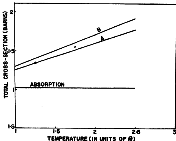
Figure 2. Aluminium, total cross section against temperature: curve B, total theoretical cross section using incoherent approximation of Placzek; curve A, total theoretical cross section with correction included; X, experimental points (Cassels)
