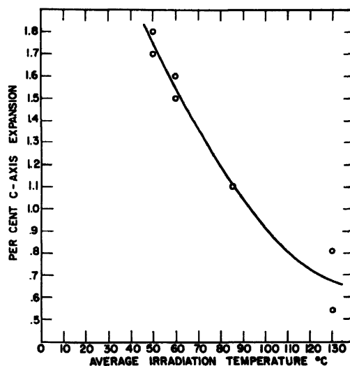
Figure 20. Per cent c -axis expansion vs average irradiation temperature of graphite samples; integrated flux 1.2 \times 10^{20} neutrons/cm 2
