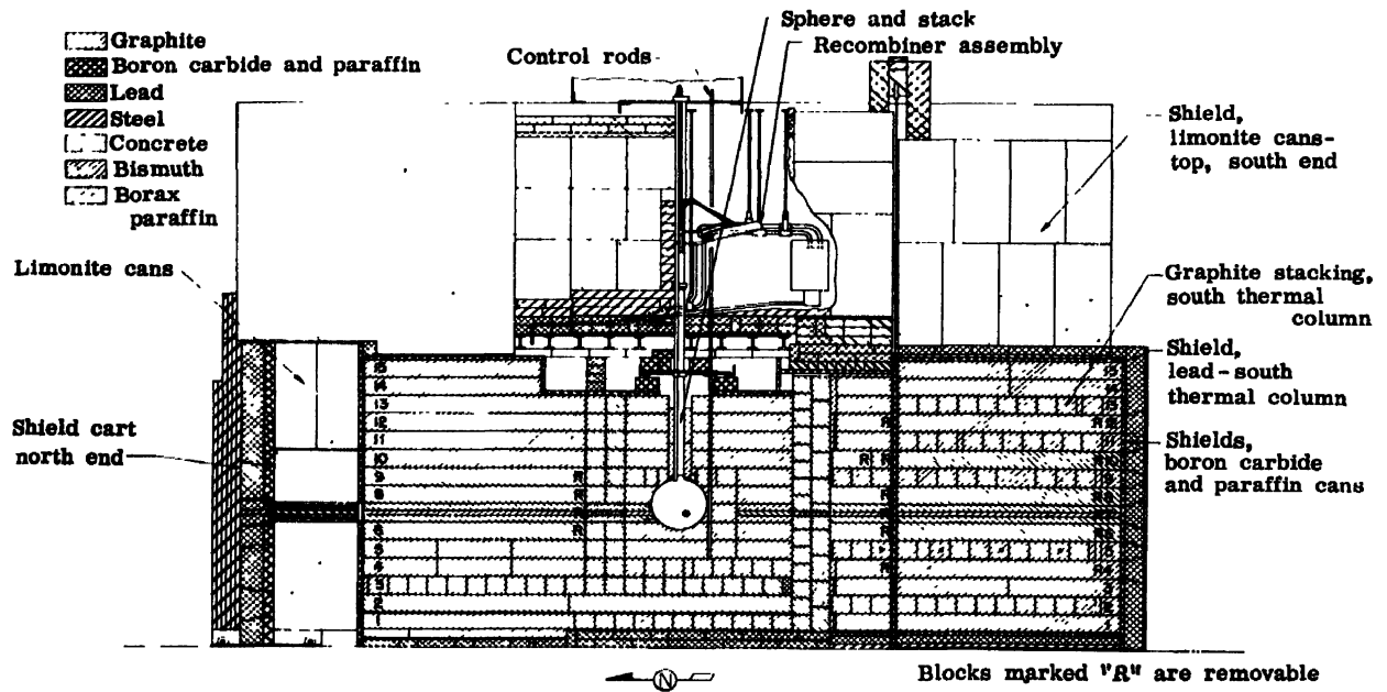
Figure 6. North-south vertical section of water boiler (Supo model)
