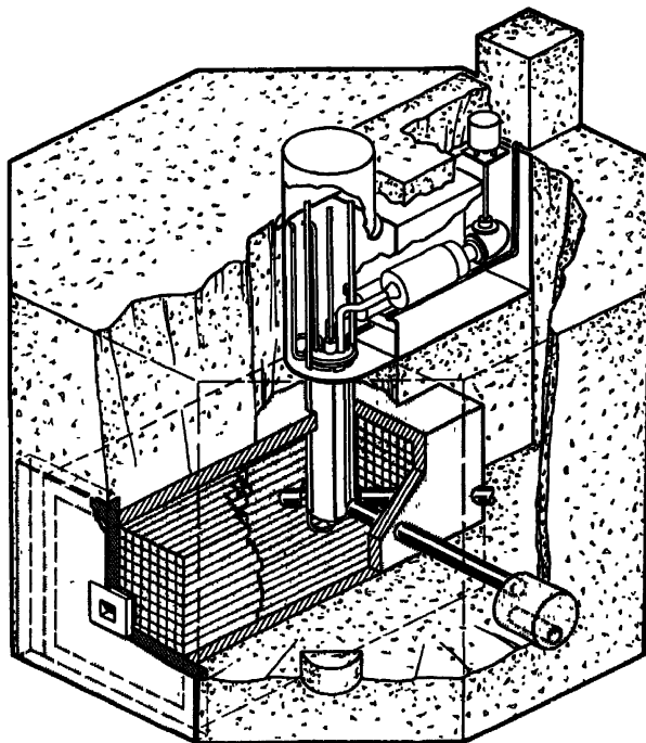
Figure 24. Schematic, Supo II
