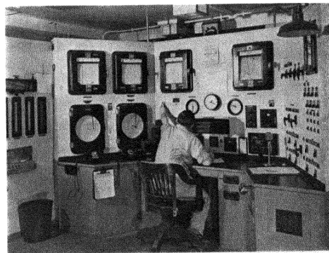
Figure 4. Control console of the graphite reactor showing operator throwing "scram" switch to shut the reactor down
