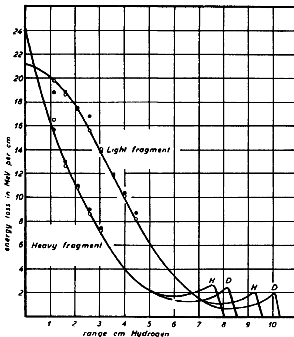
Figure 5. Energy loss along range in hydrogen and deuterium. Open and full circles correspond to H_2 and D_2 , respectively
