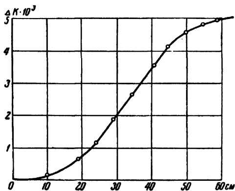
Figure 14. Reactivity compensated by an iron rod
