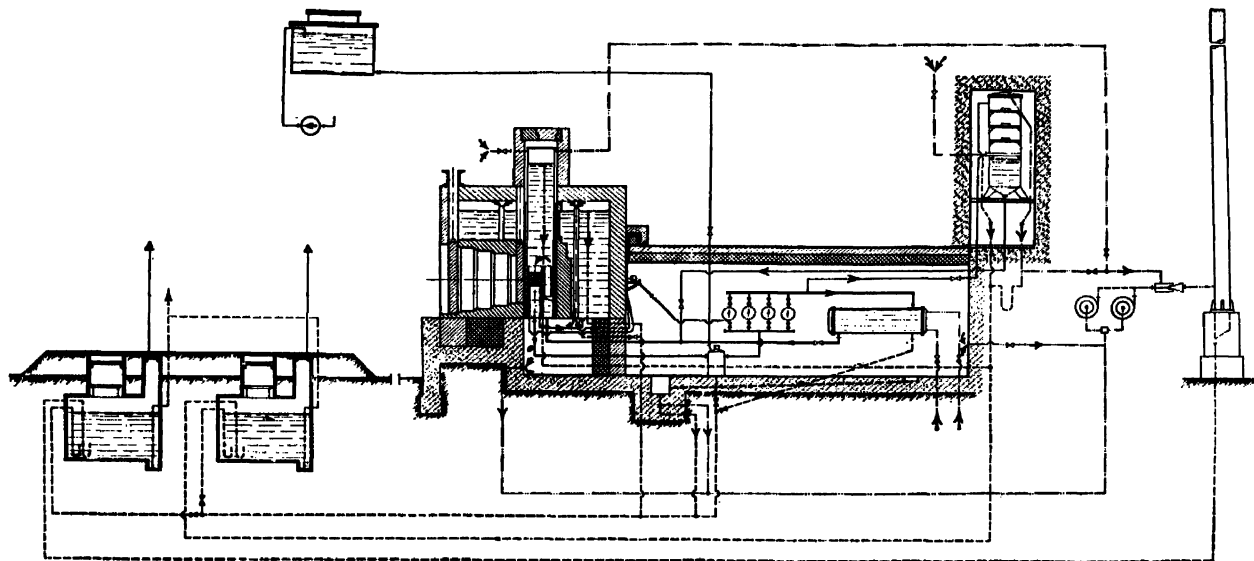
Figure 11. Flow diagram of the reactor
