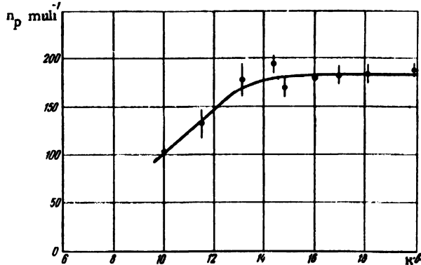
Figure 7. Decay proton counting rate, plotted against accelerating potential
