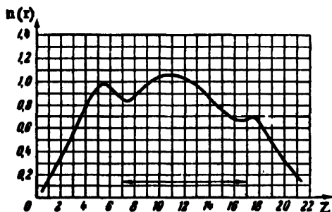
Figure 5. The neutron flux at different levels of the reactor. The core is indicated by a double arrow
