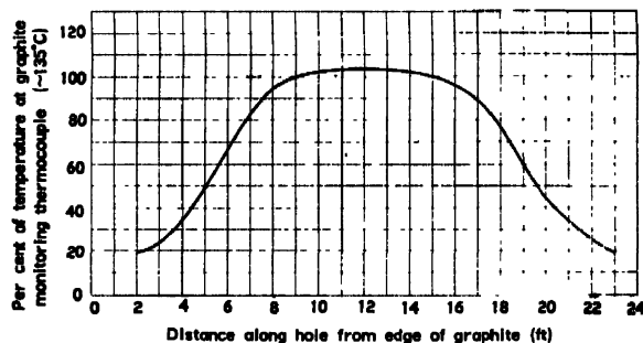
Figure 10. A typical temperature traverse through a 4-in. square hole showing a flattening at the center
