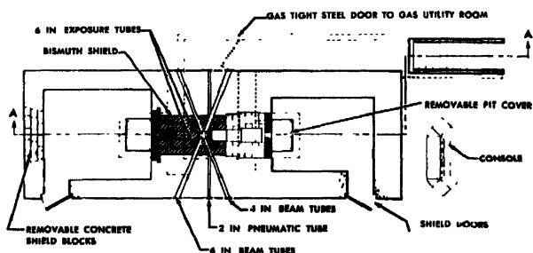
Figure 20. NAA medical reactor, top view
