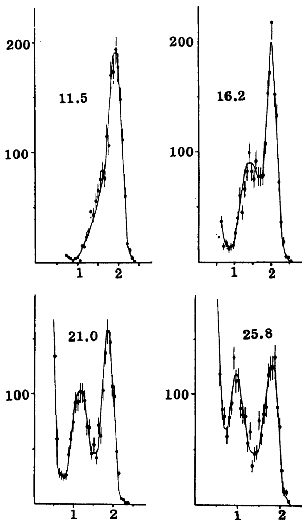
Figure 3. Ionization distributions in deuterium corresponding to distances between uranium layer and ionization chamber ranging from 11.5 to 25.8 mm D_2 . Ordinate: number of fragments; abscissa: pulse size in Mev per mm D_2
