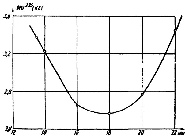
Figure 12. Dependence of the critical fuel loading on the lattice spacing
