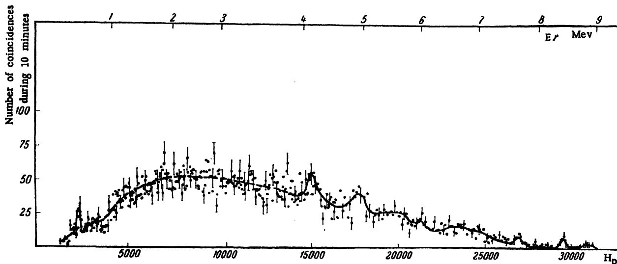
Figure 4. Coincidence background gamma-ray spectrum
