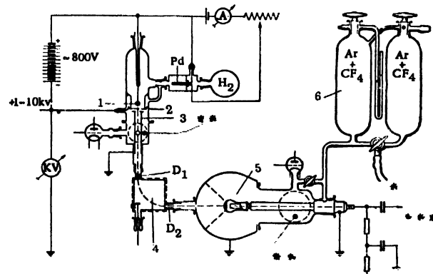
Figure 4. Set-up for measuring proton pulse height distribution: (1, 2, 3) electrodes; (4) chamber of magnetic spectrograph, ( D_1 and D_2 ) diaphragms; (5) counter; and (6) glass reservoir; * to f.v. pump, ** to h.v. pump, *** to amplifier
