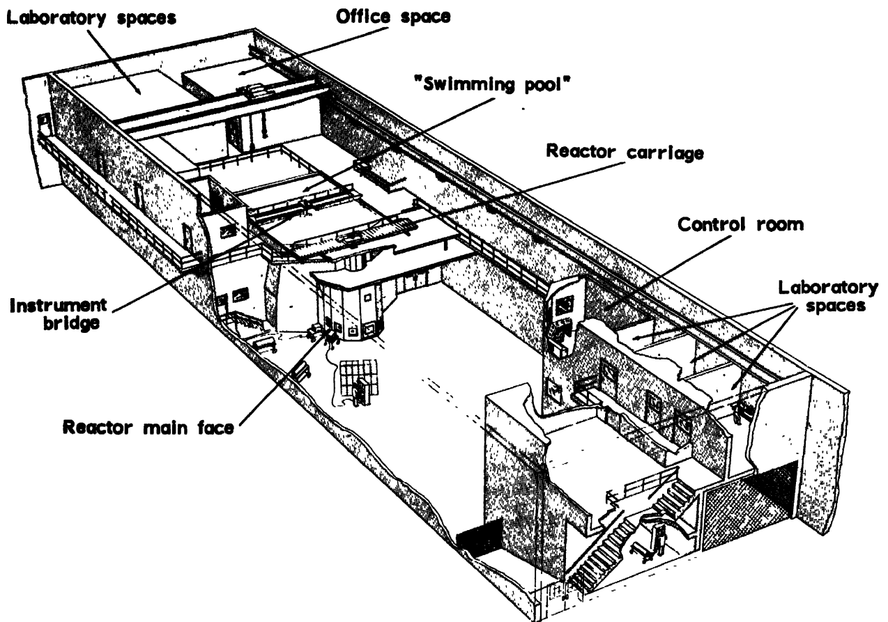
Figure 4. Proposed NRL research reactor facility
