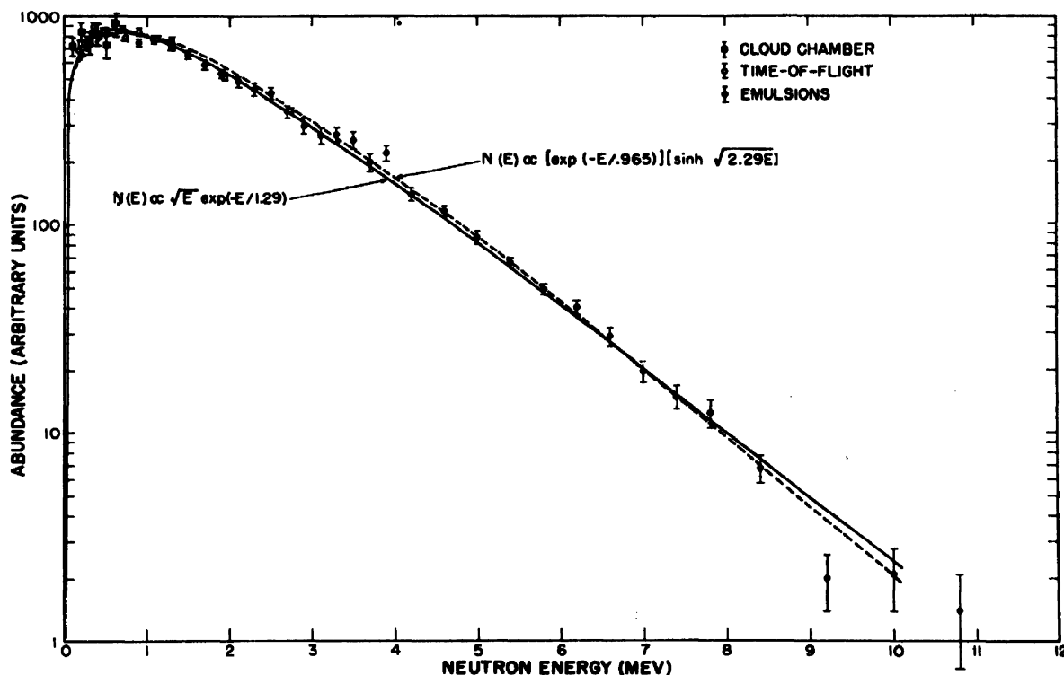
Figure 8. Comparison of semi-empirical expressions of the energy spectrum of fission neutrons with recent measurements of thermal-neutron-induced fission of U^{235}
