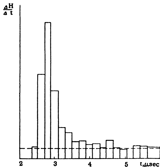
Figure 9. Proton time-of-flight distribution at 180 degrees
