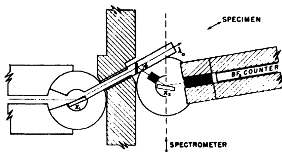
Figure 11. Crystal spectrometer arrangement at Chalk River, Canada, for study of energy change of monochromatic neutron beam of near-thermal energy in crystal lattices (courtesy B. N. Brockhouse)
