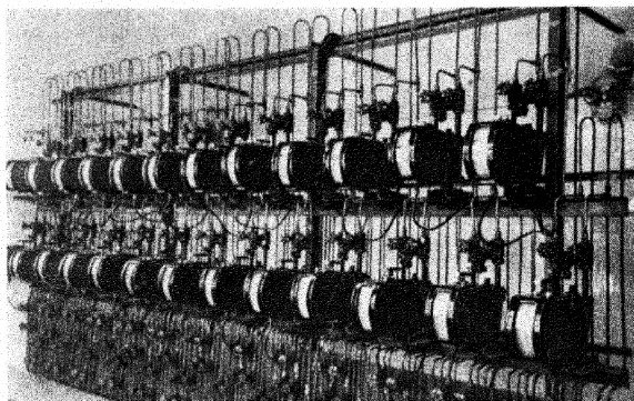
Figure 22. Shield with meters registering flow through the cooling channels of the reactor
