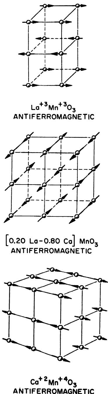
Figure 24. Some magnetic structures observed in the (La, Ca) MnO_3 series of compounds
