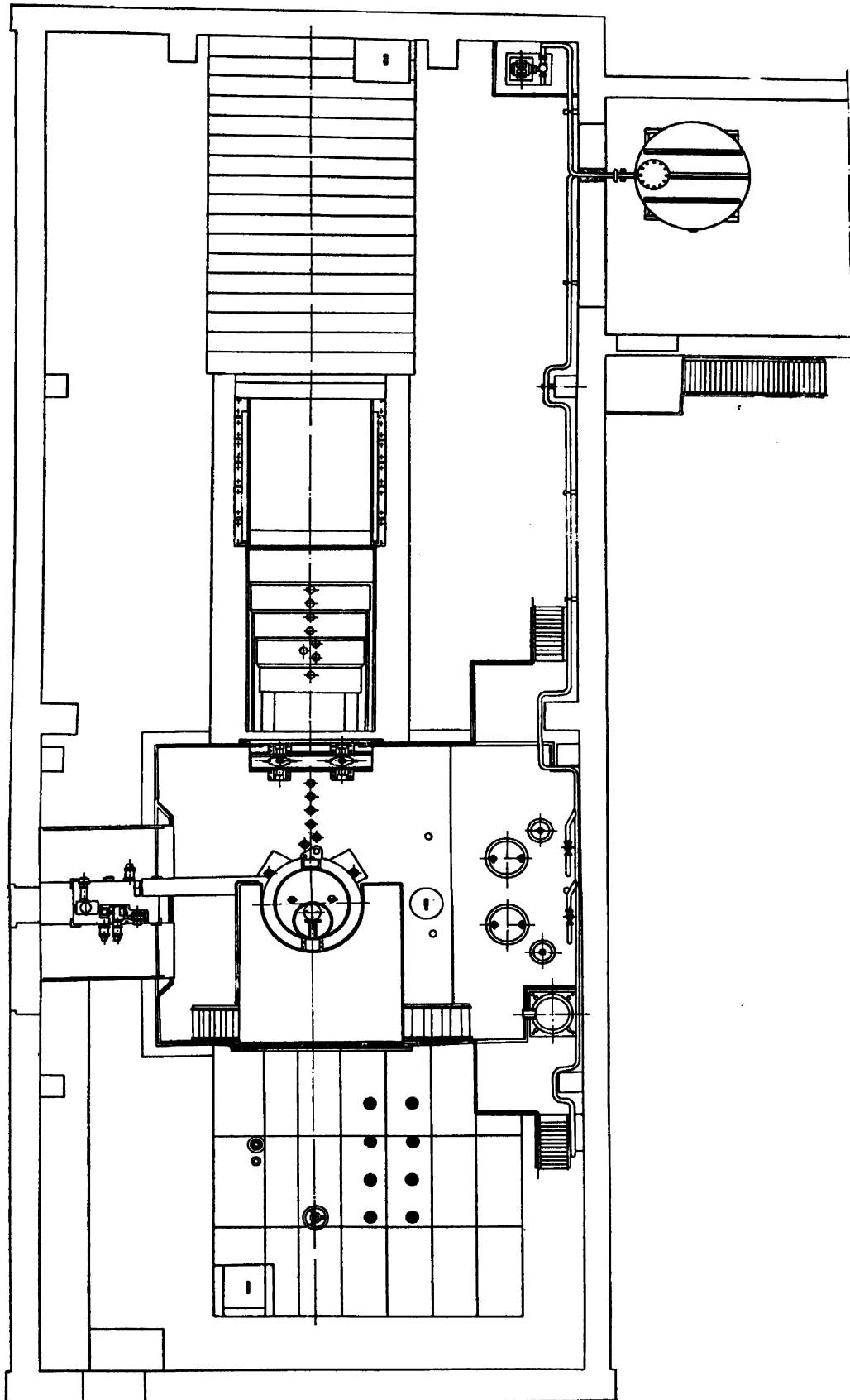
Figure 8. Plan view of the reactor
