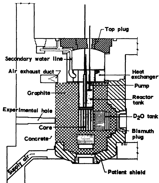
Figure 8. Section through medical research reactor
