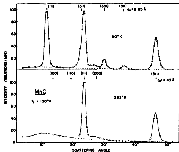
Figure 13. Room temperature and low temperature patterns for MnO showing antiferromagnetic superstructure lines which have developed at the lower temperature
