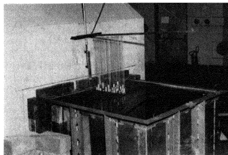
Figure 3. Apparatus beside the reactor shield for studying slowing-down lengths of fission neutrons in water-metal mixtures
