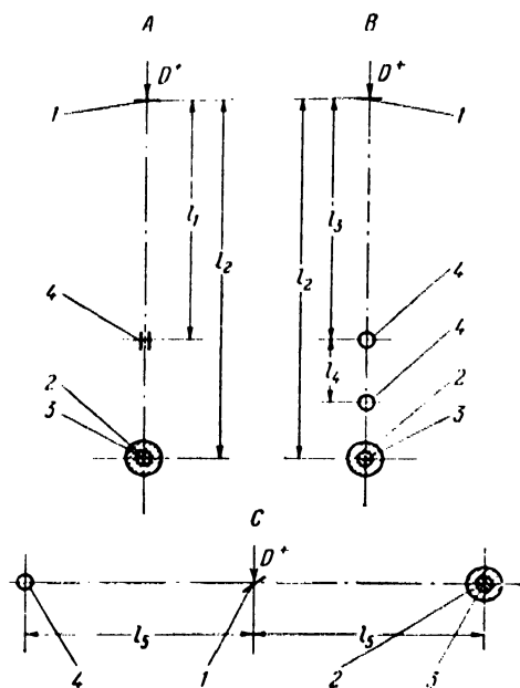
Figure 1. The experimental arrangements for measuring inelastic scattering cross sections: (1) target; (2) scatterer; and (3) detector; (4) monitor; (5) l_1 = 18 , l_2 = 30 , l_3 = 19 , l_4 = 24 , l_5 = 18 for 2.5-Mev neutrons and l_1 = 30 for 14-Mev neutrons
