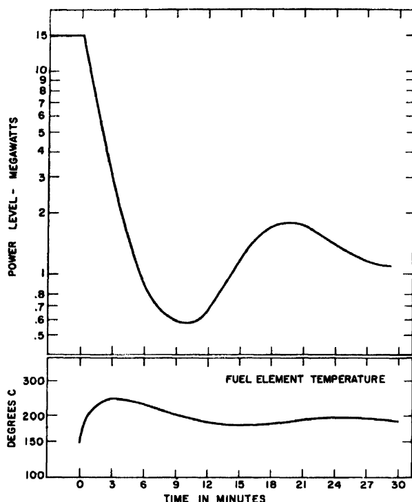
Figure 21. Behavior of reactor following a loss of coolant (with control rods locked out)
