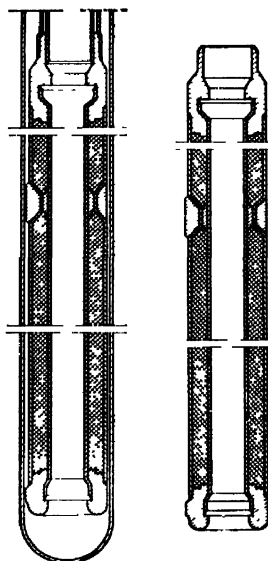
Figure 13. (Left) RPT fuel assembly
