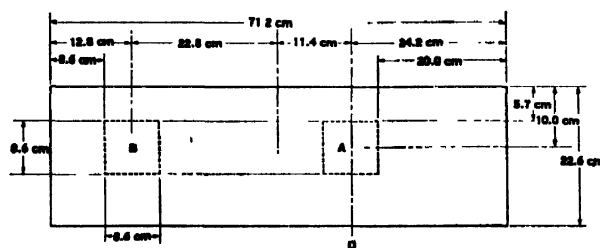
Figure 13. Test positions of large Cd rods in the core of the 4-kg mockup assembly
