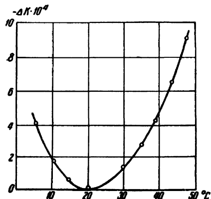
Figure 13. Variation of reactivity with change of water temperature
