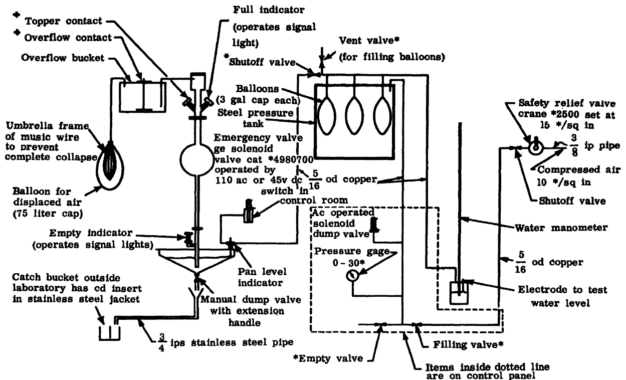
Figure 2. LOPO solution system. Fluid handling system: note, * = hose needle valve; † = opens solenoid dump valve automatically; electrical connections not shown
