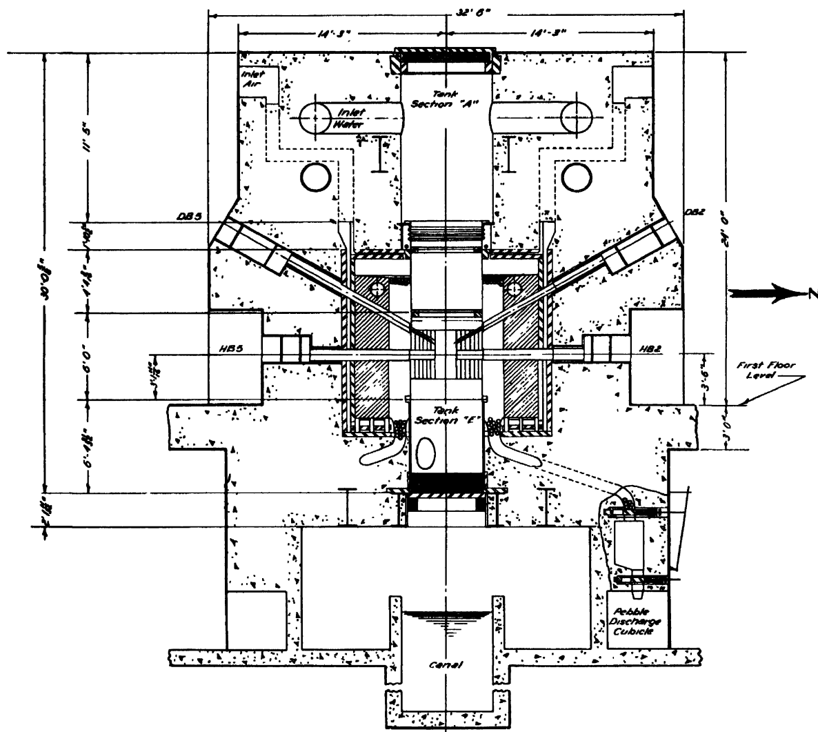
Figure 4. MTR north-south vertical section
