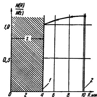
Figure 16. Thermal neutron distribution within a lattice cell: (1) fuel element boundary; and (2) effective cell radius
