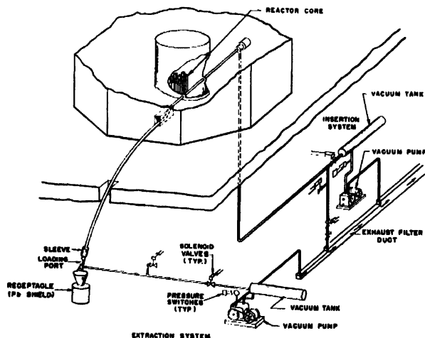
Figure 6. Diagram of rabbit installation
