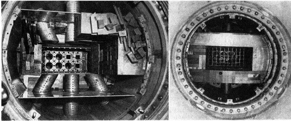
Figure 25. (Left) A view of the LITR core space with the permanent beryllium being stacked around the beam hole thimbles Figure 26. (Right) A view of the LITR core space with the stacked beryllium in place prior to being covered with the sheet aluminum housing
