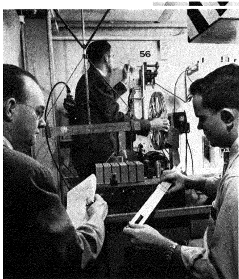
Figure 14. The oscillator used in making neutron absorption measurements. The drive mechanism was made from a washing machine
