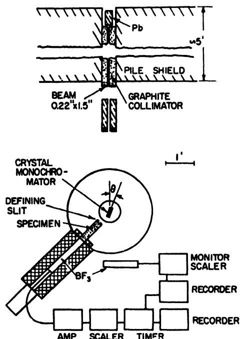
Figure 12. Arrangement of crystal spectrometer for studies of long wave-length neutrons (4-10 Å) through crystal lattices
