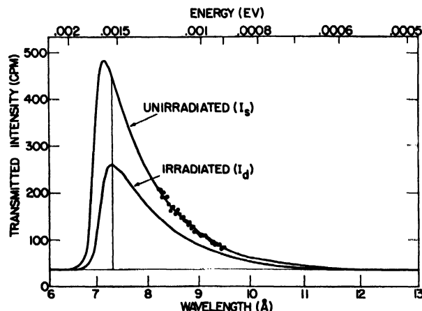
Figure 13. Decrease in slow neutron transmission of graphite by scattering from lattice defects created by fast neutron radiation damage in a reactor
