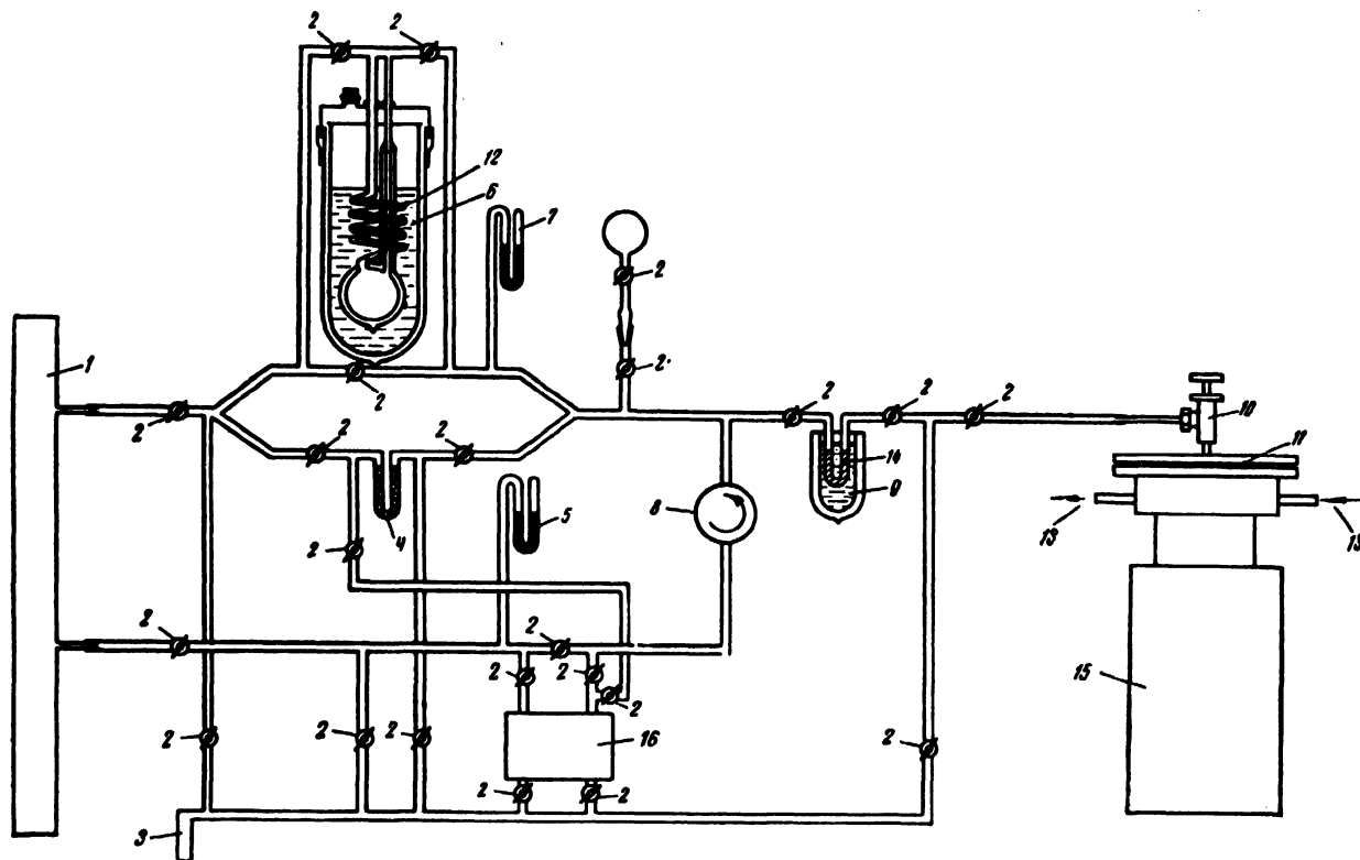
Figure 3. Scheme for filling scattering chamber: (1) scattering chamber; (2) stopcock; (3) to pump; (4) catalyst; (5) manometer; (6) liquid hydrogen; (7) manometer; (8) mixer; (9) liquid nitrogen; (10) valve; (11) copper washer; (12) catalyst; (13) cooling water; (14) cold trap; (15) electrical heater of container; and (16) gas-analyzer
