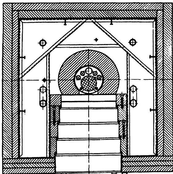
Figure 9. Horizontal section of the reactor
