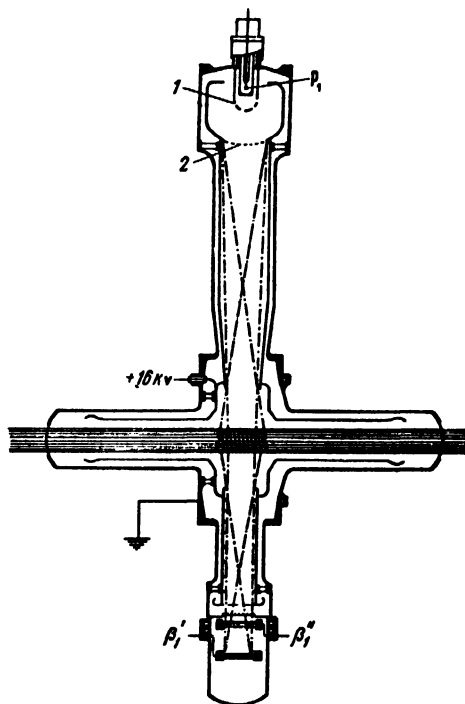
Figure 8. Over-all view of apparatus for studying angular correlation: ( P_1 ) proton counter; (1, 2) grids between which accelerating potential is applied, ( \beta_1' and \beta_1'' ) electron counters
