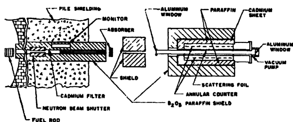
Figure 12. Annular scattering chamber
