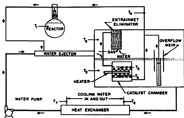
Figure 22. NAA wet gas handling system
