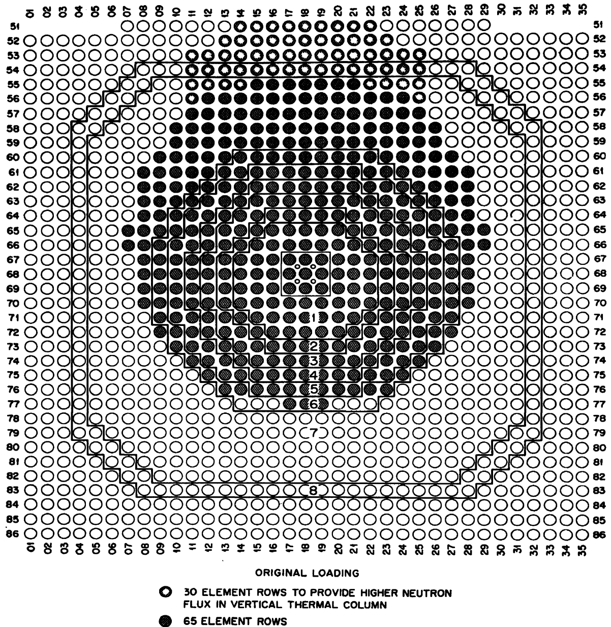
Figure 7. First operating fuel loading of 35.7 tons of normal uranium. The 30-element rows at the top were to provide a higher neutron flux in the vertical thermal column
