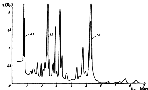
Figure 12. Corrected gamma-ray spectrum from sulphur
