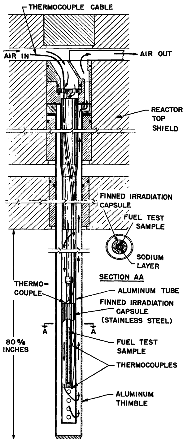
Figure 9. High temperature irradiation apparatus
