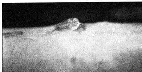
Figure 2. The picture shows one large, approx. 3 mm high, and one small blister on one of the active rods. The large blister is scratched on top when the element is extracted from the reactor, due to small clearance in the fuel element hole in top of tank. This rod was permanently removed because of the large blister. (Photograph is taken from the projected picture)
