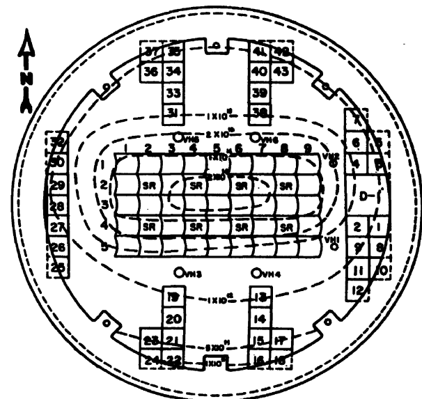
Figure 9. MTR reactor tank horizontal cross section fast neutron flux values at midplane
