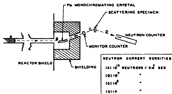
Figure 12. A schematic sketch of a neutron spectrometer with the parts named
