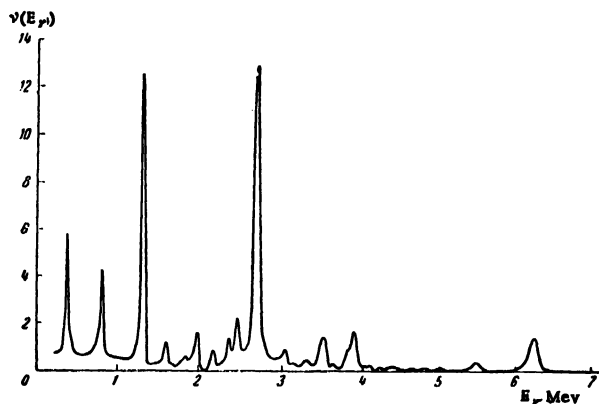
Figure 8. Corrected gamma-ray spectrum from sodium
