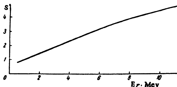
Figure 3. Gamma-spectrometer efficiency as a function of energy
