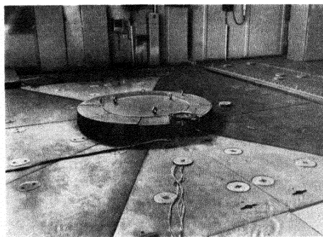
Figure 18. Top view of reactor: the top shielding of the reactor is seen
