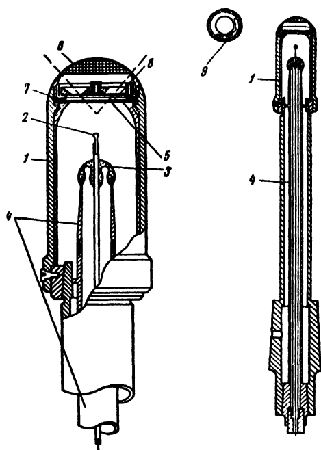
Figure 2. Cross section through central electrode: (1) outer electrode of counter; (2) collecting electrode; (3) insulator; (4) pin of collecting electrode; (5) film; (6) film supporting wire mesh; (7) spring; (8) spherical mesh; and (9) alpha-particle source
