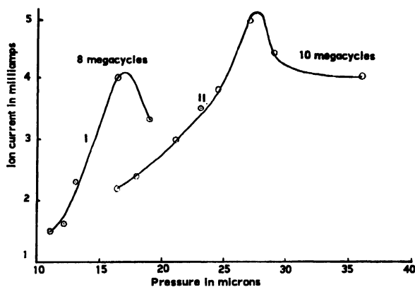
Figure 3. Curves showing variation of ion current with pressure at 8 and 10 megacycles frequency of the oscillator keeping the wattage input of the oscillator and extracting voltage constant. In curve I the probe current varies from 5 to 8 ma. In curve II the probe current varies from 5 to 9 ma
