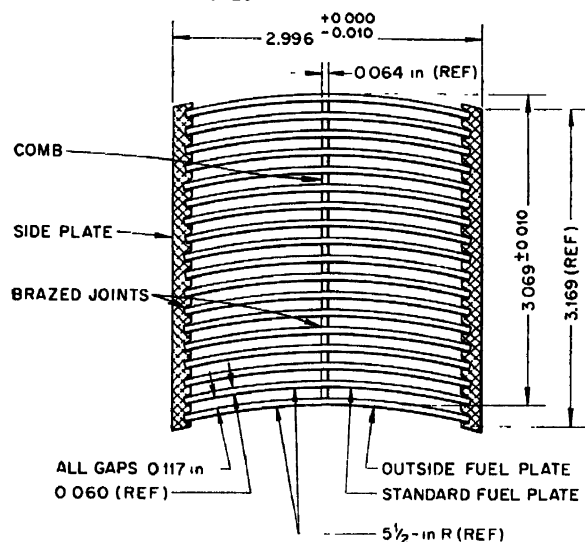
Figure 2. Cross section of MTR fuel assembly
