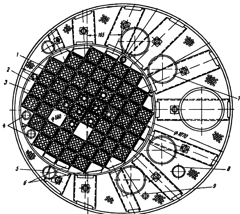
Figure 1. Reactor active core: (1) lattice; (2) supporting plate, (3) safety and control rods; (4) experimental holes; (5) channel for the starting ionization chamber; (6) plugs; (7) channel for the working ionization chamber; (8) overflow pipe; and (9) level indicator channel
