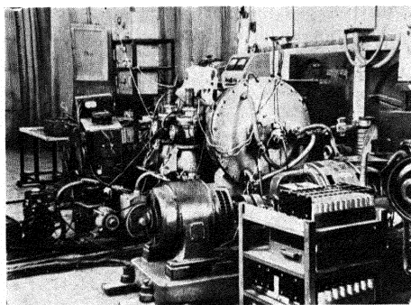
Figure 5. Arrangement for the investigation of the \beta -decay of the neutron
