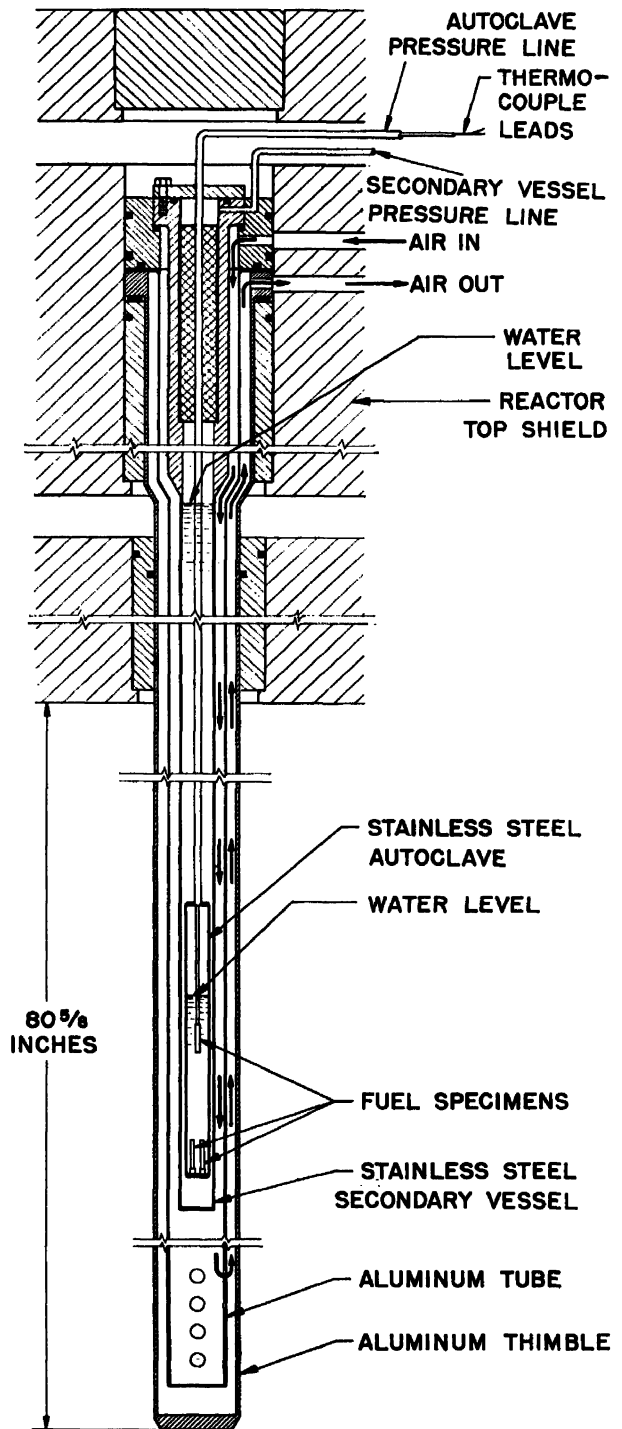
Figure 8. Pressurized water autoclave
