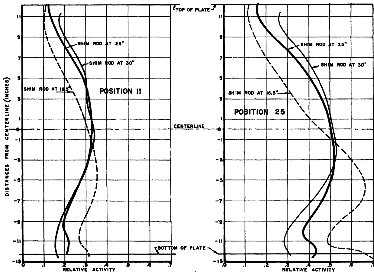
Figure 5. Vertical flux traverses in fuel assemblies
