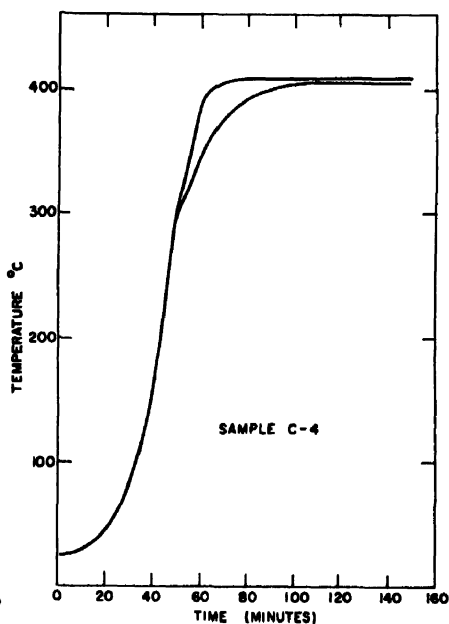
Figure 16. Time vs temperature plot of a graphite sample in a furnace held at 400°C; temperature of irradiation, 65°C. Some of the stored energy of this sample was released in a furnace held at 200°C
