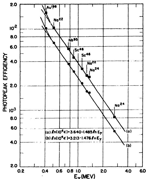
Figure 5. Photopeak efficiency of a NaI crystal 2.57 cm long and 2.54 cm in diameter for ring sources placed symmetrically about the crystal as in Fig. 1. The sources were enclosed in toroids of rectangular cross section with the following dimensions: (a) od = 7.08 cm, id = 5.08 cm, thickness = 1.00 cm; (b) od = 10.16 cm, id = 5.08 cm, thickness = 1.27 cm. The curves have been corrected for self-absorption in the sources
