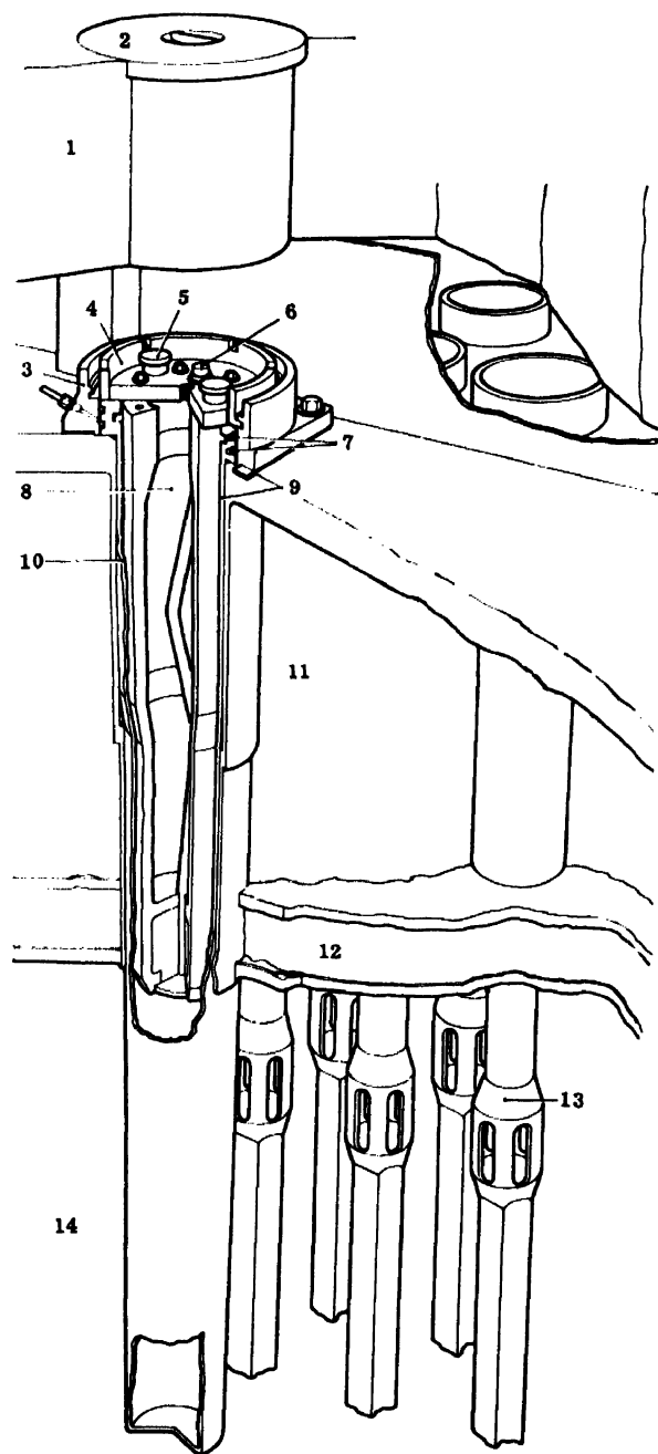
Figure 6. Reactor E.443: 6" dia. vertical experimental hole in heavy water. (1) Mild steel reactor top plate; (2) removable plug; (3) adaptor; (4) retaining ring; (5) shield plug locking control; (6) experimental hole purge connector; (7) aluminium liner tube sealing rings; (8) biological shielding plug (concrete filling not shown); (9) aluminium liner tube; (10) stainless steel liner tube in biological shield; (11) biological shield; (12) lead thermal shield; (13) fuel elements; (14) heavy water
