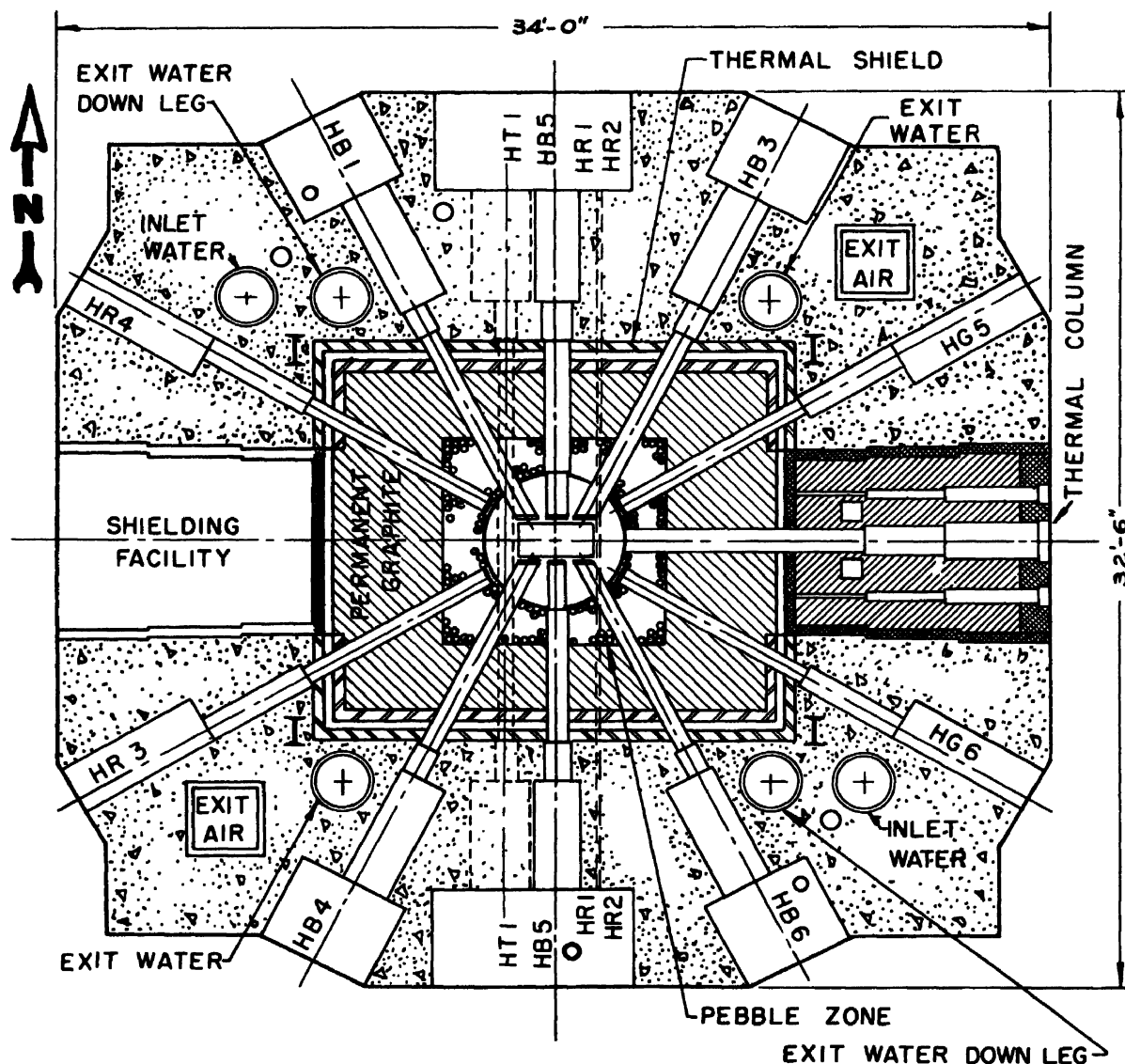
Figure 3. MTR horizontal section
