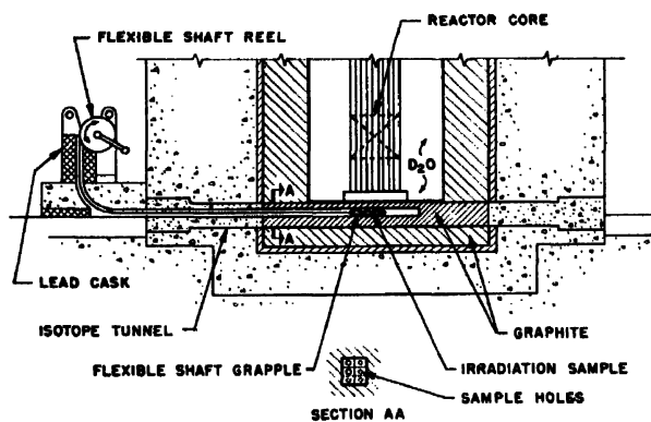
Figure 5. Diagram of the irradiation tunnel beneath the reactor
