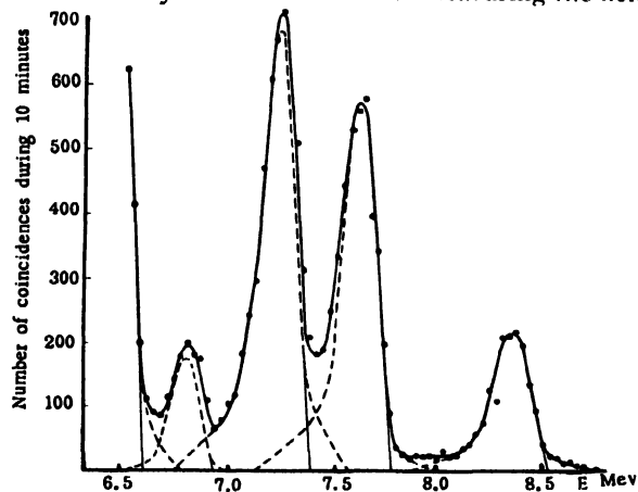
Figure 2. Analysis of coincidence spectrum peaks for gamma rays of chlorine
