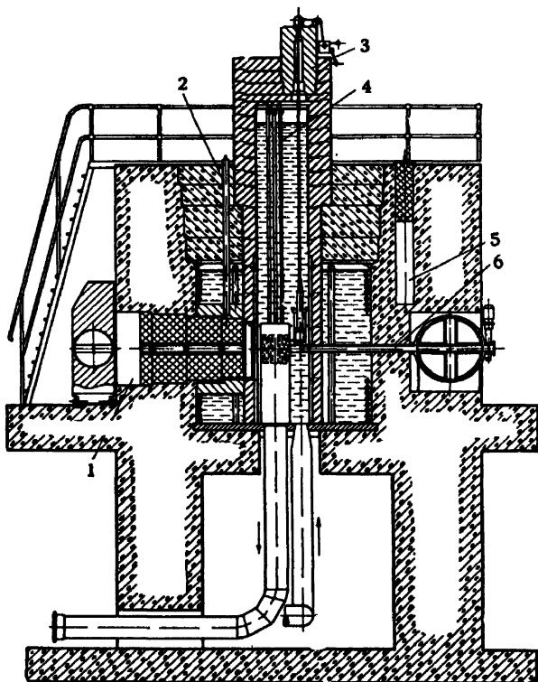
Figure 2. Vertical section of the reactor: (1) thermal column; (2) vertical hole; (3) lead container; (4) control rod tubes; (5) biological hole; and (6) horizontal hole
