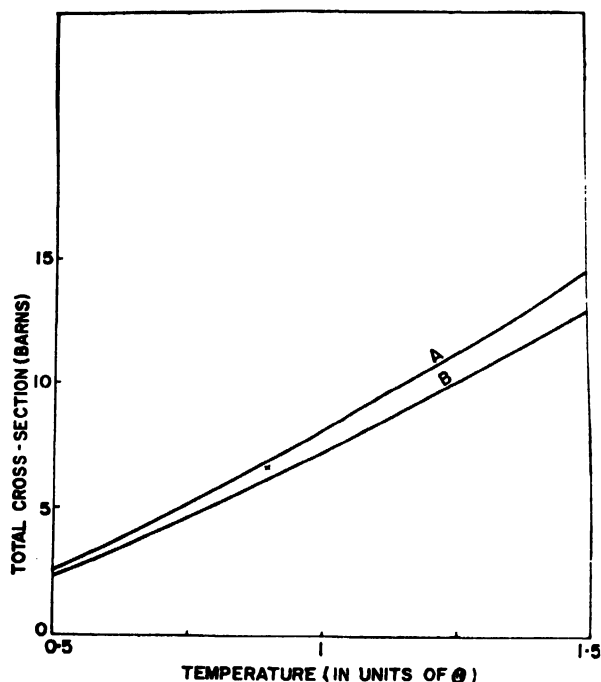
Figure 5. Beryllium, total cross section against temperature: curve B, total theoretical cross section using incoherent approximation of Placzek; curve A, total theoretical cross section with correction included; X, experimental points (Hughes)
