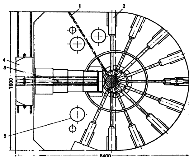
Figure 3. Horizontal section through the reactor: (1) experimental hole (curved); (2) horizontal hole; (3) thermal column holes; (4) thermal column shielding; (5) storage for radioactive materials
