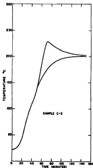
Figure 14. Time vs temperature plot of a graphite sample in a furnace held at 200°C; temperature of irradiation, 65°C
