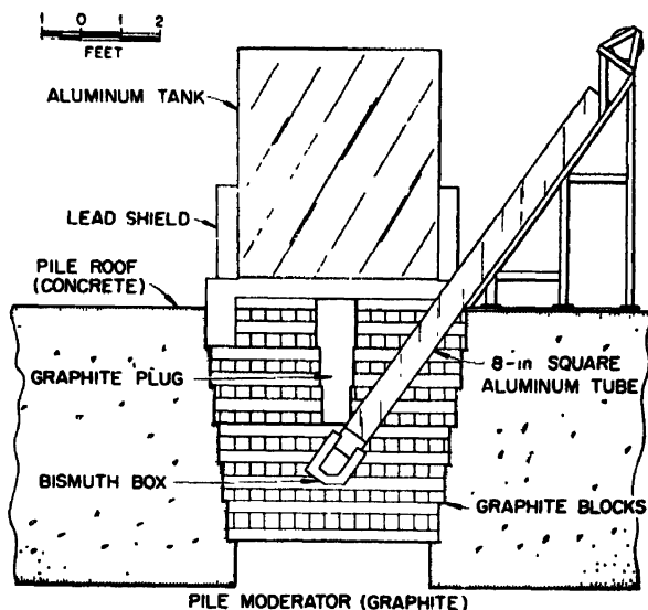
Figure 17. A sectional sketch of the vertical thermal column showing the inclined biological tunnel
