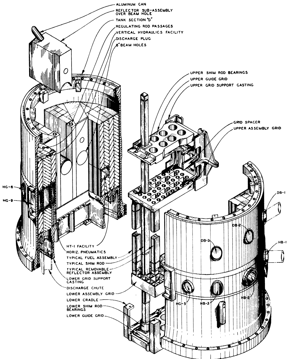
Figure 1. Pictorial cross section, reactor tank
