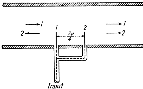
FIG. 3.—A method of launching a TE_{0,1} mode in one direction only.
