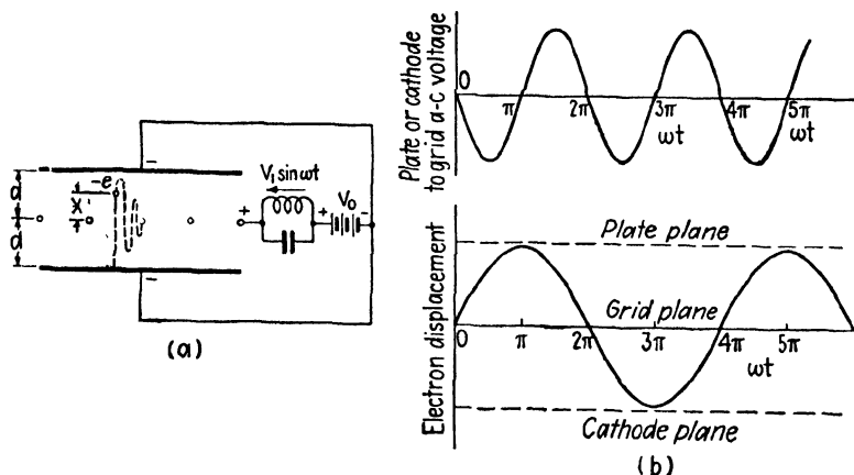
FIG. 1.—Positive-grid oscillator.
