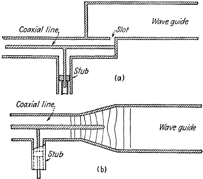
FIG. 4.—Methods of exciting wave guides from coaxial lines.
