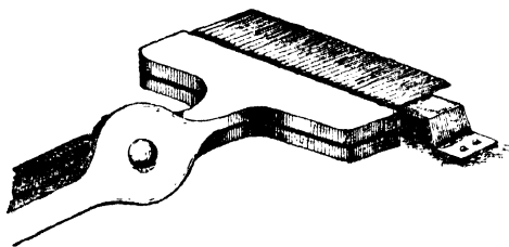
Row of single needles held in pliers for removing roughness left on separation at heads.
