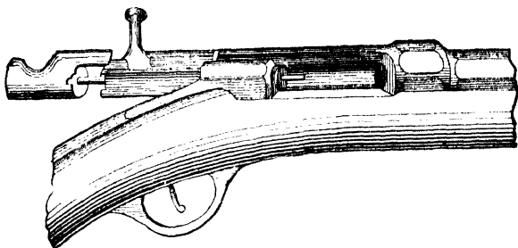
Bolt Gun—Breech open.
