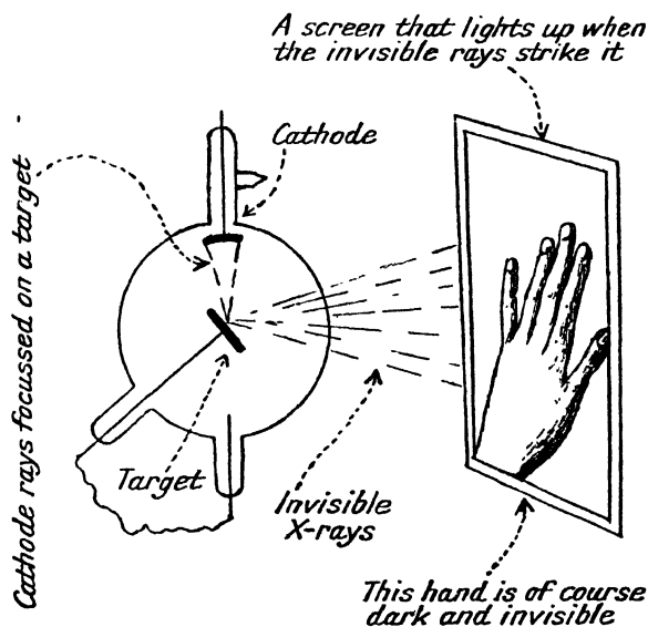
FIG. 23.—An X-ray tube.
