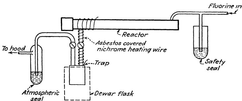
Fig. 34. Apparatus assembly for preparation and purification of tantalum-(niobium)(V) fluoride.
