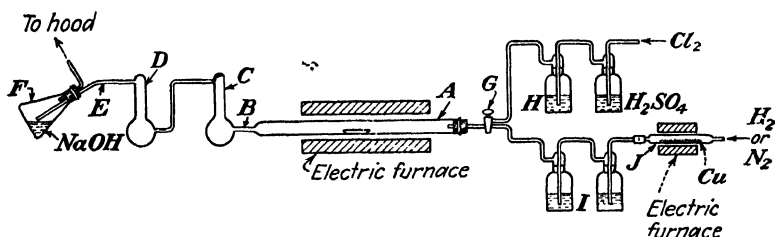
FIG. 29. Apparatus for the preparation and purification of tungsten(VI) chloride.
