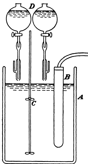
FIG. 14. Apparatus for precipitation of zirconium hafnium phosphates.
