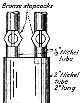
FIG. 33. Metal trap for condensation of tantalum-(niobium)(V) fluoride.
