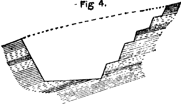
Section which requires benching back on one side.
