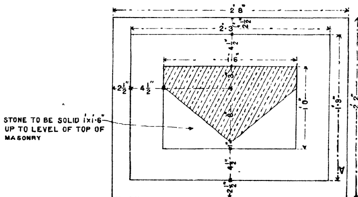
Fig. 25 SECTIONAL PLAN AT A.A.
