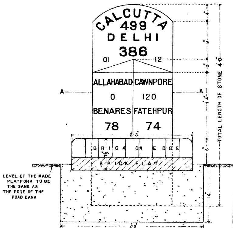
Fig 24 ELEVATION
