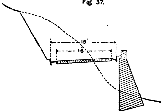
Section at salient curve showing "banking."
