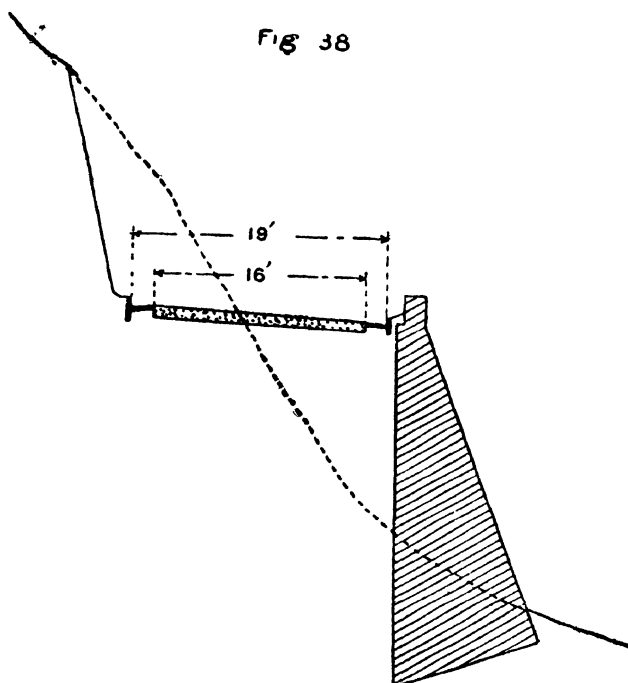
Section at re-entrant curve showing "banking."
