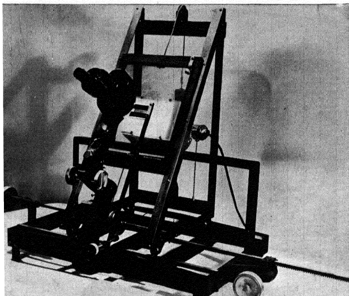
Fig. 25.—Machine used for magnitude measurements and star-counts.
