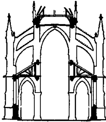
CROSS-SECTION OF A GOTHIC CATHEDRAL, SHOWING THE ARRANGEMENT OF THE NAVE AND SIDE AISLES, THE FLYING BUTTRESSES AND BUTTRESS PIERS SUPPORTING THE NAVE VAULTING.
