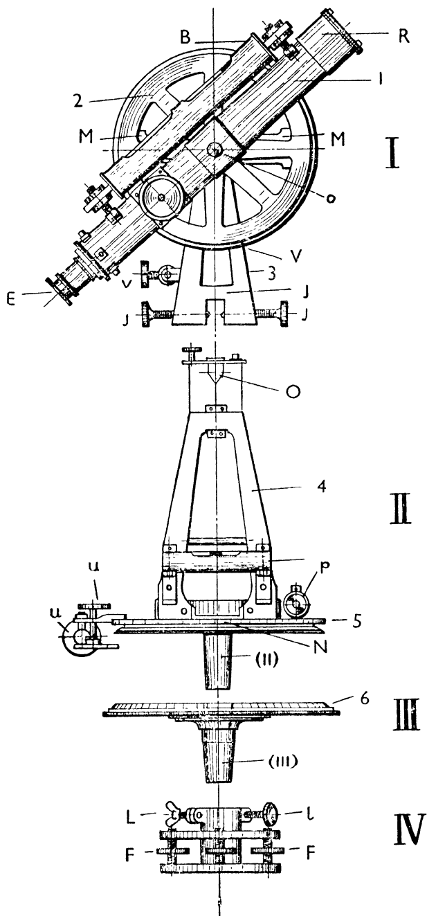
FIG. 83 THE THEODOLITE
