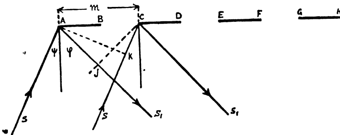
FIG. 7.—Reflection grating.
