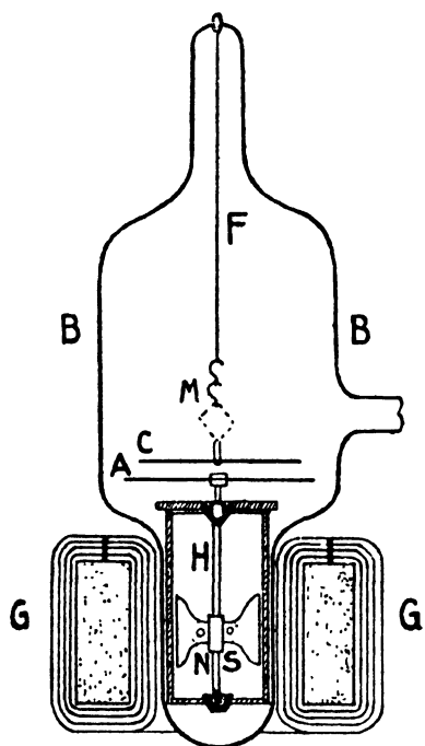
FIG. 21.—Molecular manometer of Langmuir and Dushman.
