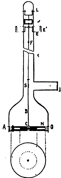
FIG. 20.—Viscosity manometer.
