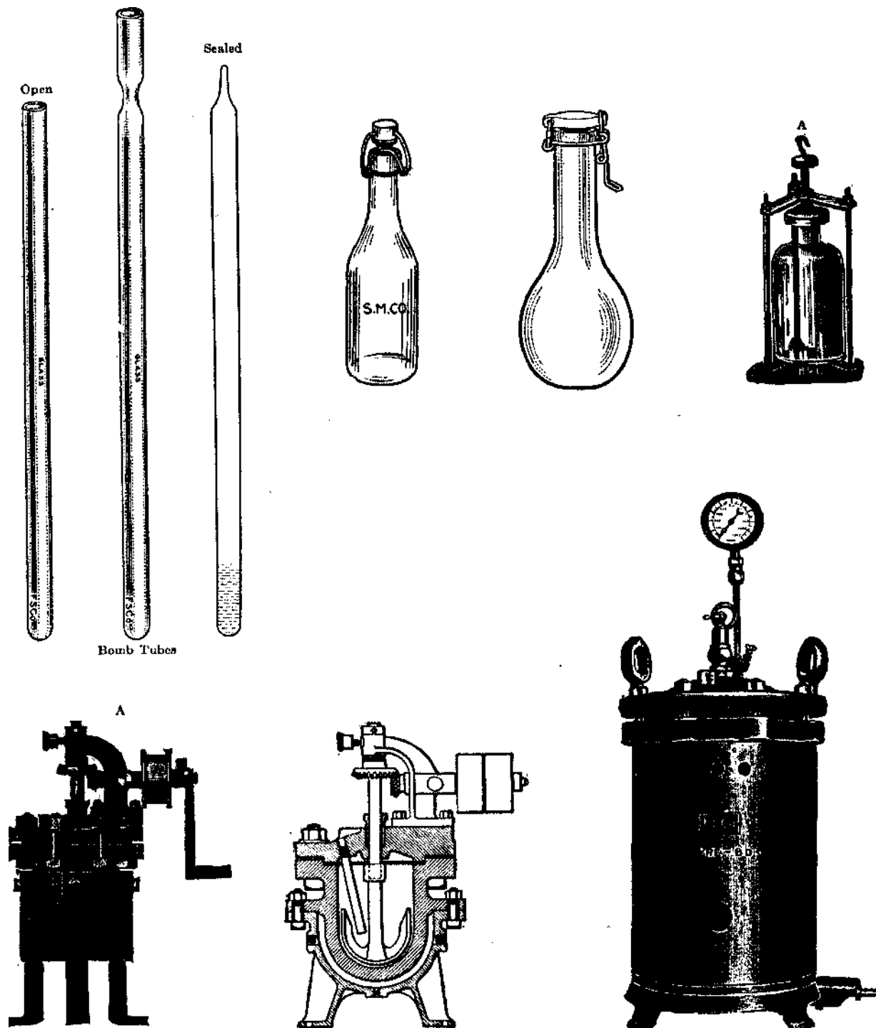
FIG. 71.--Equipment for Reaction under Pressure -Autoclaves.
