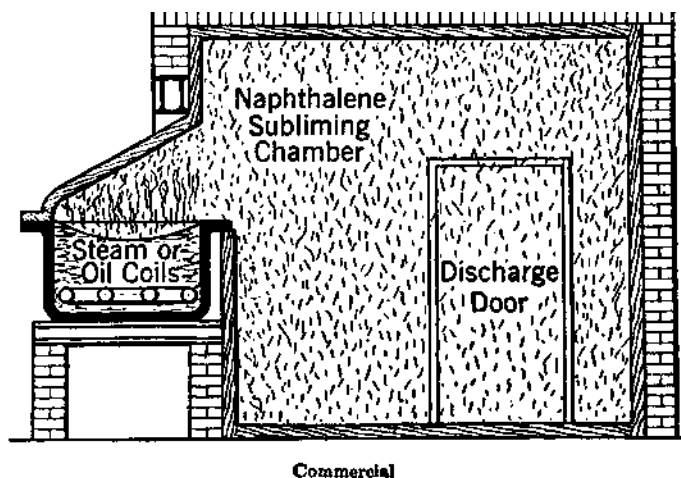
FIG. 72.—Sublimation Apparatus.
