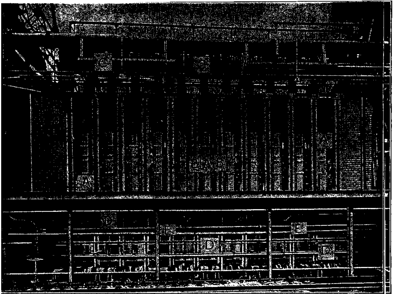
FIG. 64.—Battery of Becker Gas Ovens.
