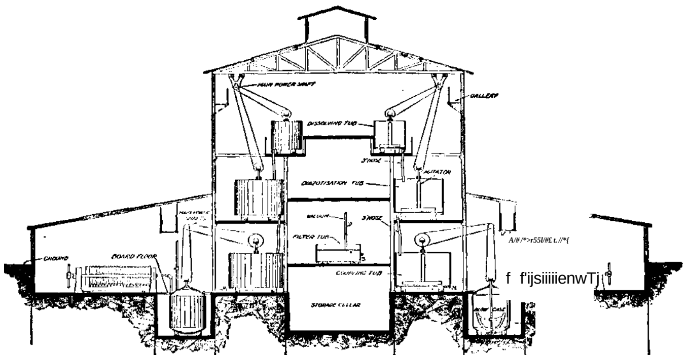
FIG. 73.—Azo Dye Plant.
