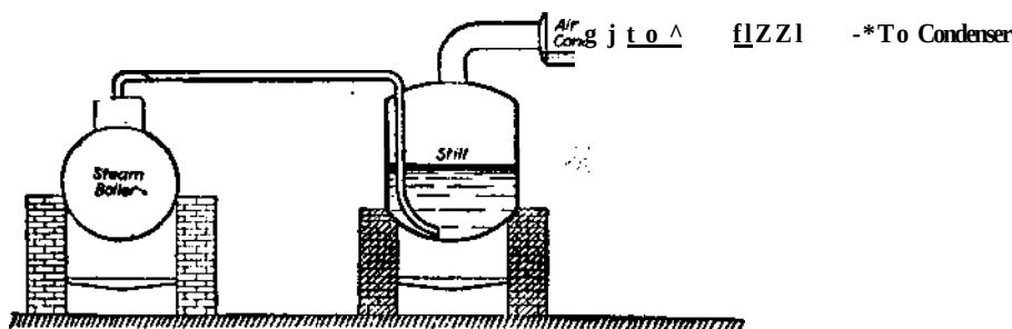
FIG. 69.—Industrial Steam Distillation.
