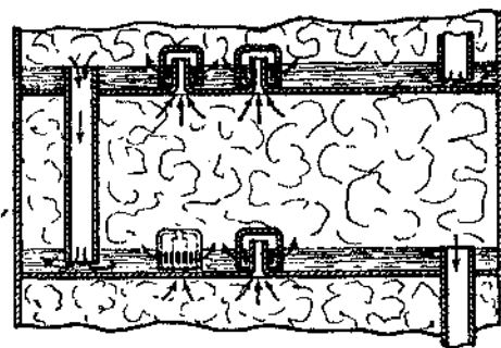
FIG. 31.—Section of a Fractionating Column.
