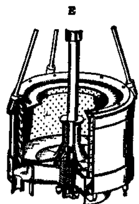
Centrifugal Filter
