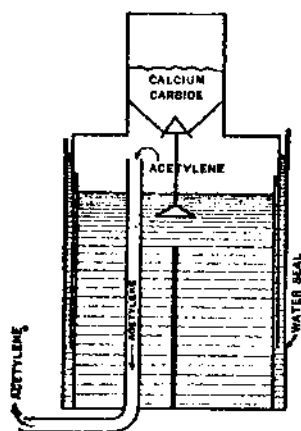
FIG. 19.—Acetylene Generator.
