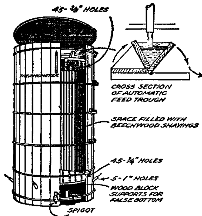
FIG. 44.—Vinegar Generator for "Quick" or Generator Process.
