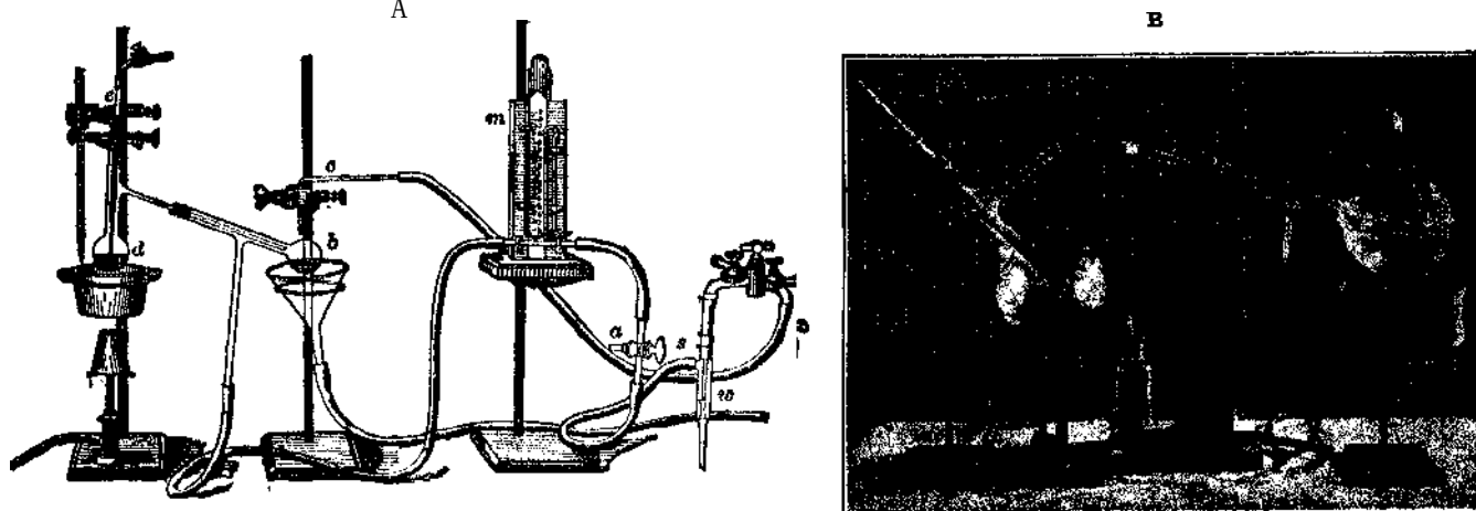
FIG. 74.—Laboratory Vacuum Distillation Apparatus.
