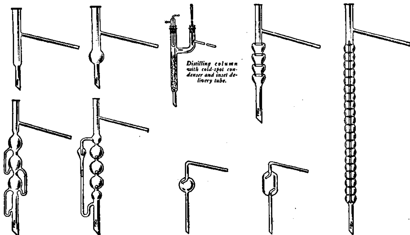
FIG. 11.—Distilling Columns and Bulbs.
