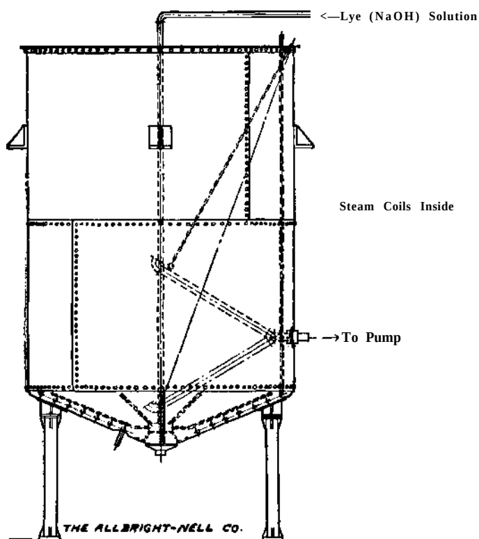
FIG. 46.—Kettle for Soap Manufacture.
