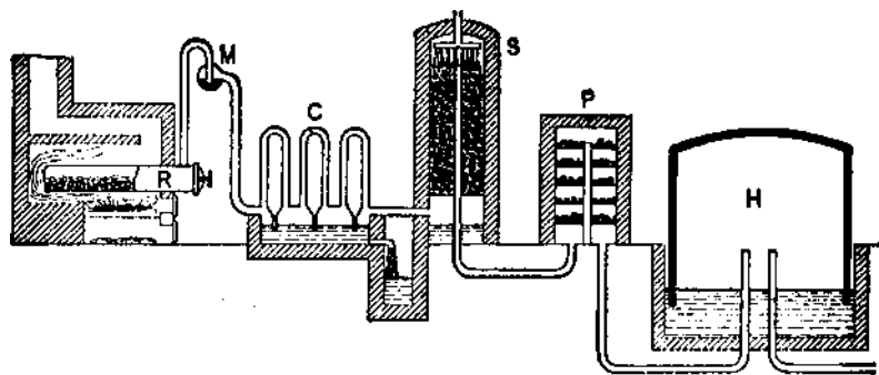
FIG. 63.—Diagram of a Plant for Making Coal Gas.
