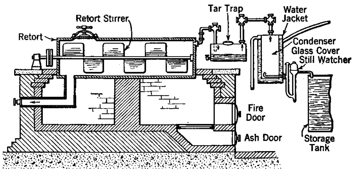
Fia. 41.—Diagram of Acetone Plant.
