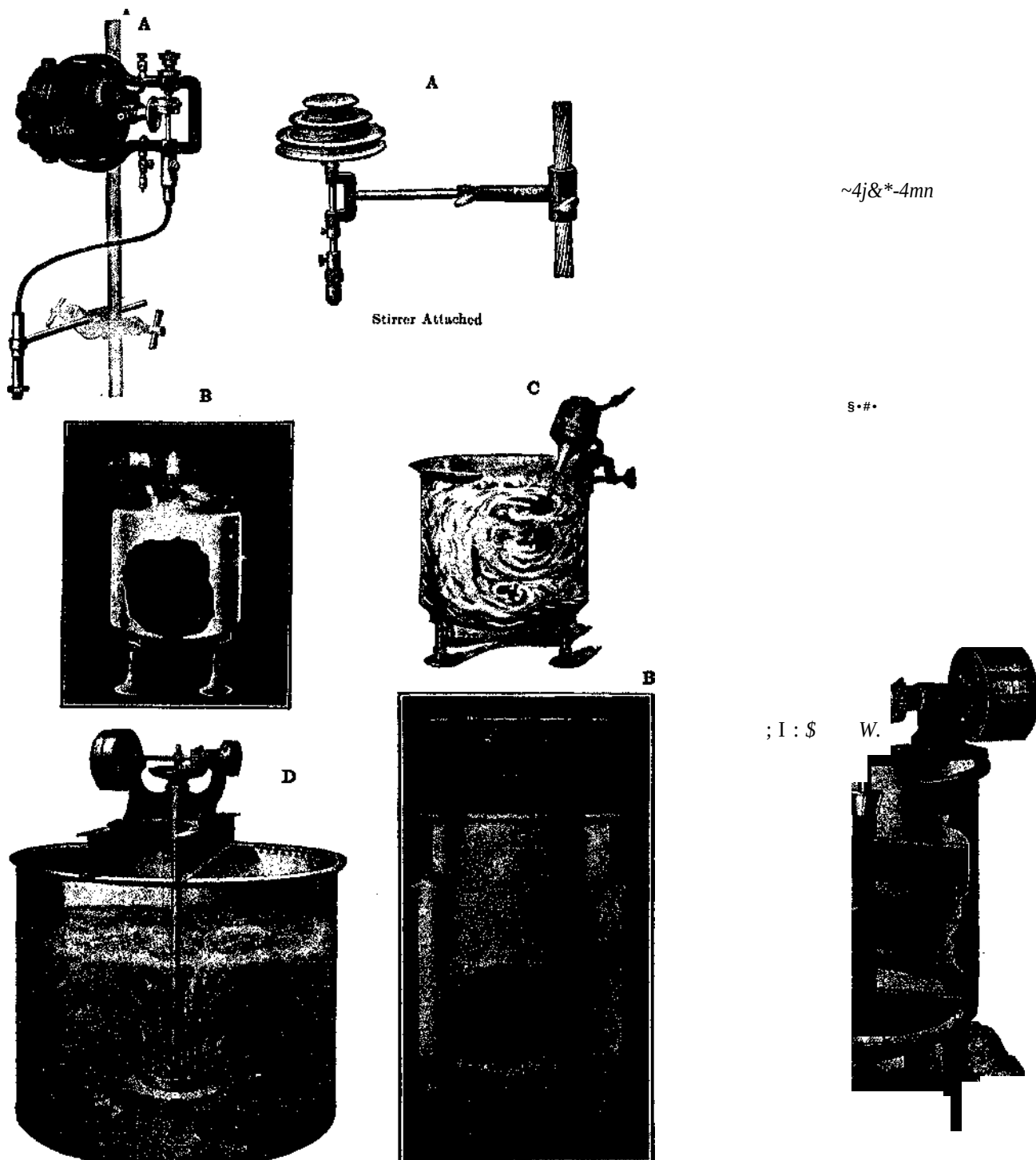
FIG 53,—Stirring and Mixing Devices
