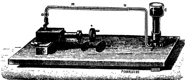
FIG. 8.—Apparatus of Bonnier and Mangin, for analysis of gases given off by plants. c , Reservoir of Mercury; m m , graduated tube; v , screw of piston, which enables the gas to be drawn into the graduated tube and measured; and after it the potash and pyrogallic solutions successively, each being thoroughly brought into contact with the gas in the dilatation a .
