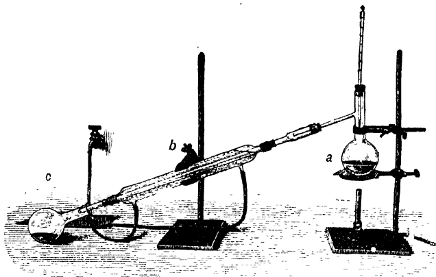
FIG. 4 — Distillation apparatus.
