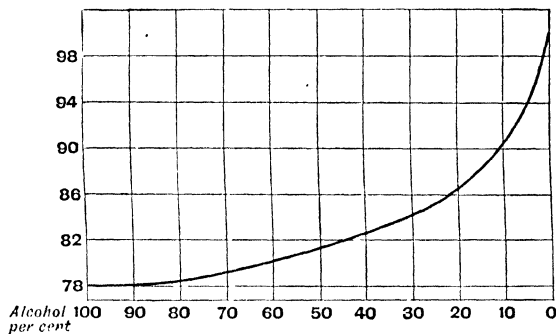
FIG. 5.—Boiling-point curve of alcohol and water mixtures.
