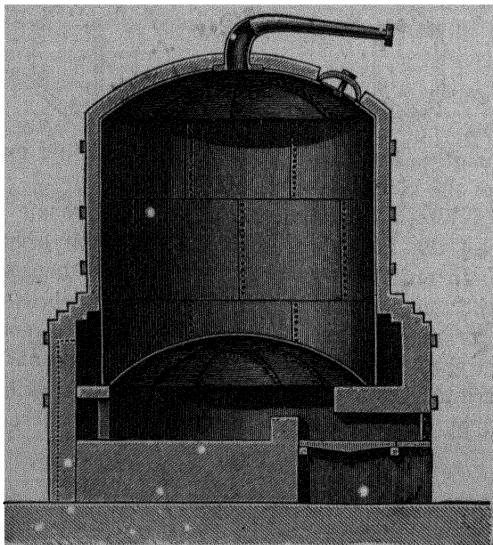
FIG. 58A.—Tar still
