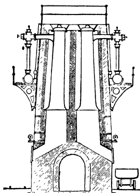
FIG. 31.—Shale retort.
