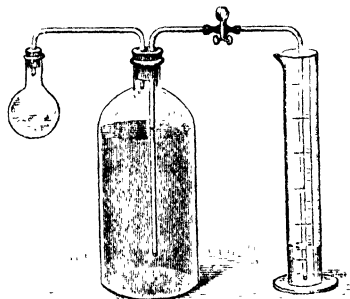
FIG. 15.—Measurement of the volume of hydrogen formed on dissolving a known weight of sodium in alcohol.
