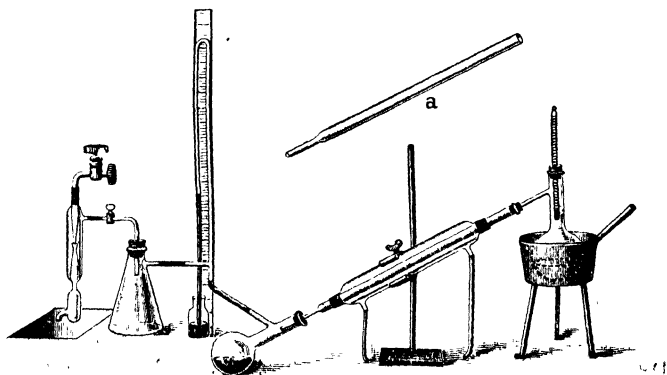
FIG. 62.—Apparatus for distillation under reduced pressure
