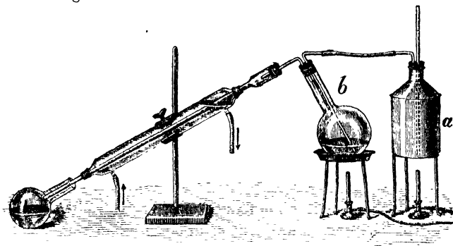
FIG. 61.—Distillation in steam.
