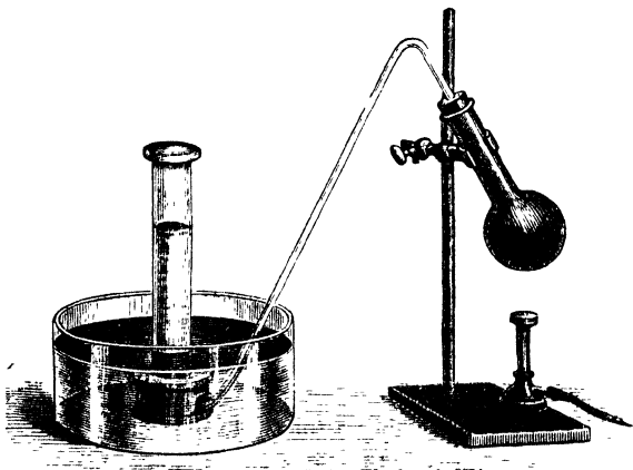
FIG. 29.—Preparation of marsh-gas from potassium acetate.
