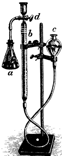
FIG. 56.—Lunge's Nitrometer for the estimation of urea.
