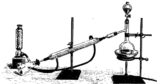
FIG. 16.—Preparation of ethyl bromide.
