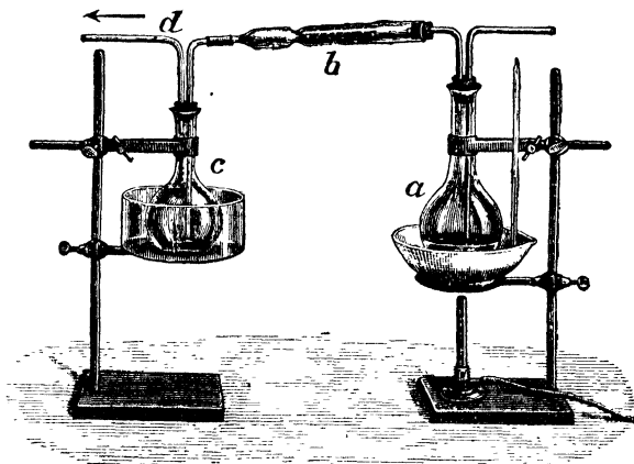
FIG. 30 Preparation of formaldehyde.
