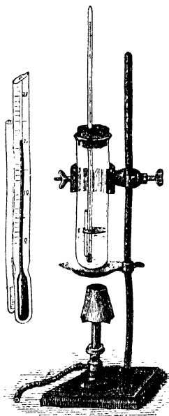
FIG. 2.—Apparatus for determining the melting-point.
