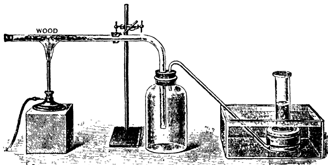
FIG. 26.—The destructive distillation of wood.
