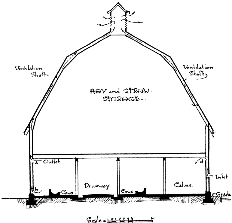
FIG. 64.—Elevation Woodland Dairy Farm barn. Note system of ventilation a, outlet in summer; b, outlet in winter, and d, inlet at all times. Also the dirt-tight floor over the stock. Straw for bedding as well as hay for feed is stored in the loft.
