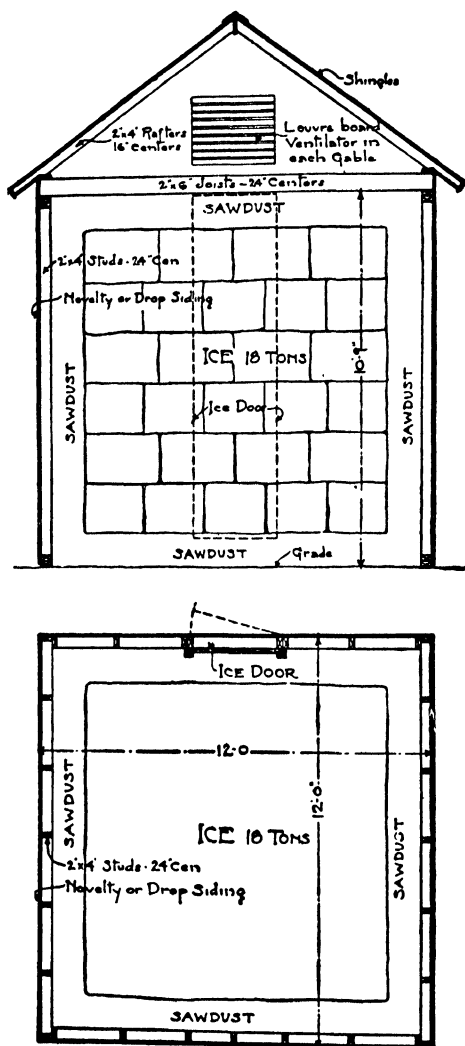
FIG. 100 — Ice house, old style. Ice covered over and around with saw dust. Reproduced from "Practical Cold Storage," by Madison Cooper. (Published by Nickerson and Collins Co., Chicago.)
