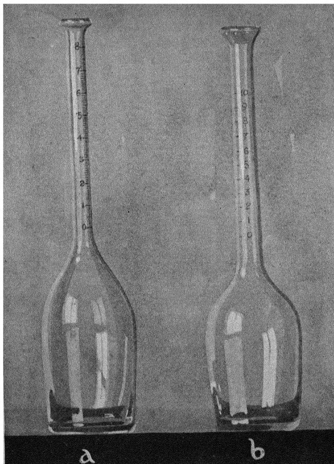
FIG. 104.—Milk test bottles. a is very much preferable to b . First, in having a slender neck, which will permit of accurate reading of the fat; second, in having sloping shoulders. Fat will lodge under the abrupt shoulder of b , and thus reduce the reading; third, the top of a is not flaring as b . A milk tested in duplicate in two bottles such as these would not read the same.
