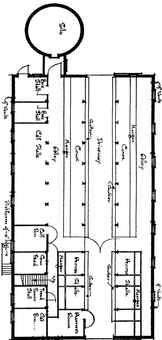
GENERAL DAIRY BARN Scale = \frac{1}{4} " = 1'-0" FIG. 63.—Plan of general farm and dairying barn on Woodland Dairy Farm, Monticello, Minn. Note broad driveway and out-facing of stock.
