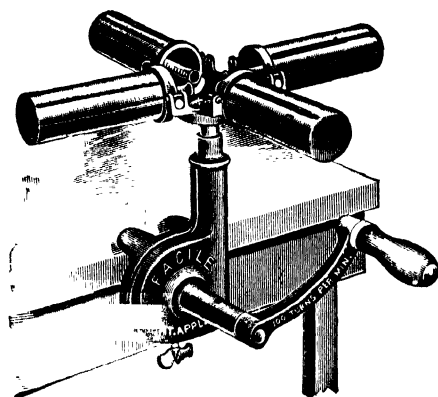
FIG. 109.—An inexpensive tester, yet one not to recommend for general farm use. The samples cool too quickly in this and if a bottle were to break, the acid would be liable to do injury.
