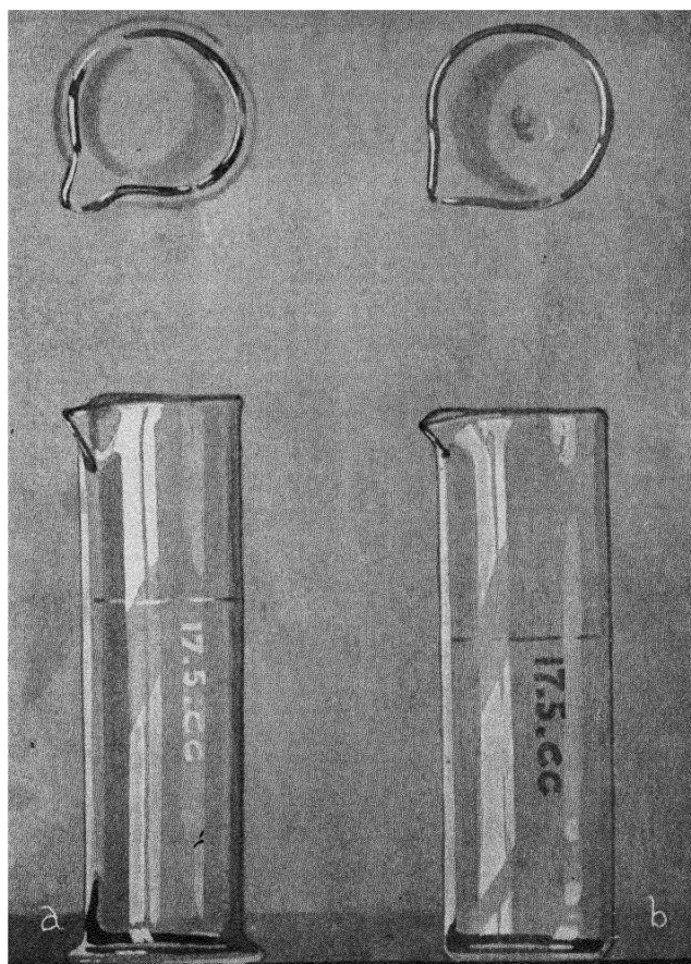
FIG. 103.—Acid measures. a is preferable to b on account of the flaring base, which renders it less liable to tip over, and the lip out of which the acid is poured is not so wide from side to side, thus easier to pour from without spilling.
