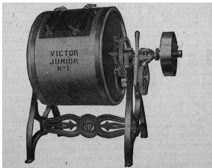
FIG. 117.—A cylindrical churn and butter worker combined.
