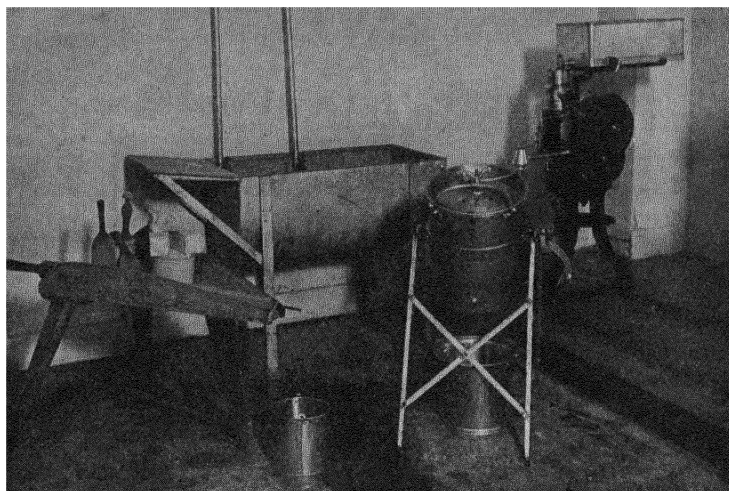
FIG. 116.—Cream separator churn and butter worker suited to the needs of the small dairy.
