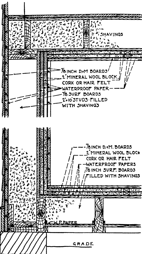
FIG. 98.—Showing method of insulating the walls in the insulated ice house. Reproduced from "Practical Cold Storage," by Madison Cooper. (Published by Nickerson and Collins Co., Chicago.)
