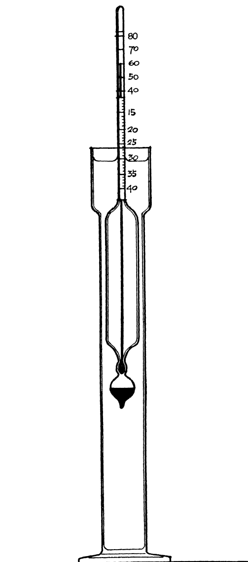
FIG. 126.—The lactometer is used for the detection of skimming and watering of milk. At temperature 60 degrees F. the lactometer will read about 31 or 32.
