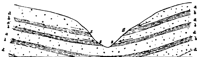
FIG. 137.—DRAINAGE IN SYNCLINAL STRATA. a, a = pervious beds; b, b = impervious beds; s, s = springs.
