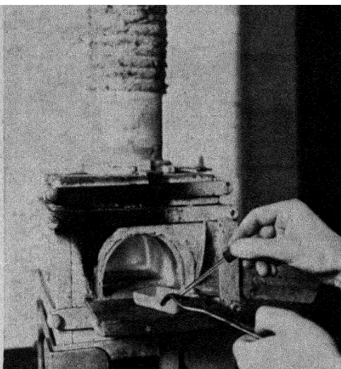
Fig. 5. —DETERMINATION OF ASH IN COAL (2). The silica dish is inserted into an open-ended muffle furnace at 800° C., until combustion is complete.
