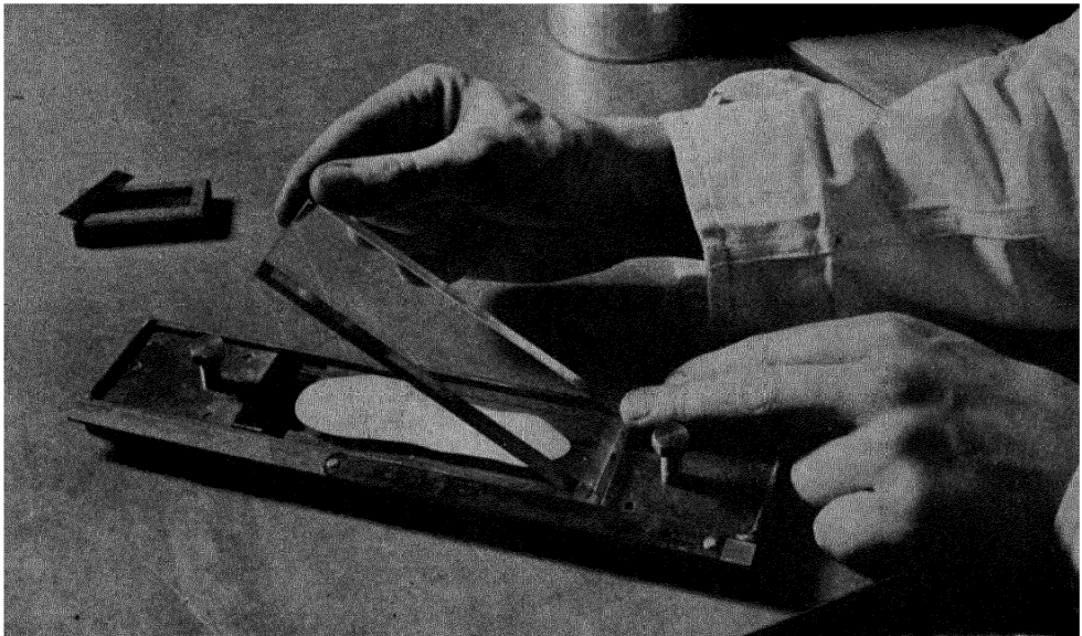
Fig. 6.—MEASUREMENT OF HIDING POWER WITH THE TRANSMETER.
