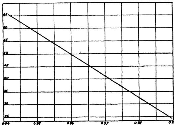
Fig. 1.—GRAPH SHOWING THE RELATIONSHIP BETWEEN SPECIFIC GRAVITY AND DRY RUBBER CONTENT OF PRESERVED LATEX.
