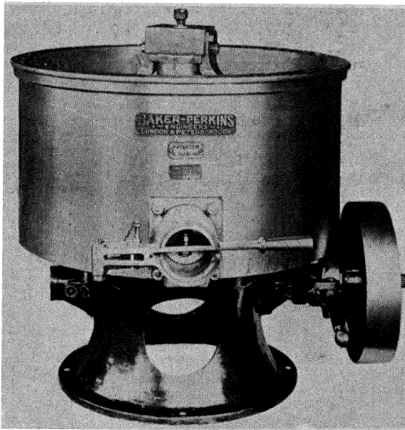
Fig. 7. —A CHOCOLATE STORAGE KETTLE.
