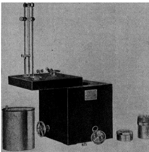
Fig. 1A.—THE ADIABATIC CALORIMETER. Showing the hot and cold water supply, measuring flask and motor for driving pump and stirrers.
