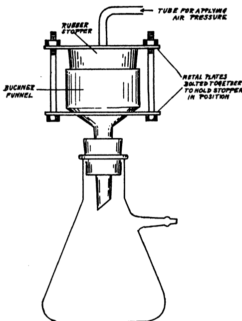
Fig. 3.—APPARATUS FOR FILTERING LATEX PRIOR TO THE DETERMINATION OF pH VALUE.
