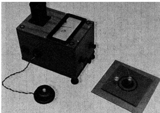
Fig. 8.—THE SPECIFIC RESISTANCE MAY BE ROUGHLY TESTED ON A MEGGER.
