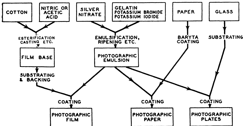
Fig. 1.—THE GENERAL SCHEME OF MANUFACTURE.
