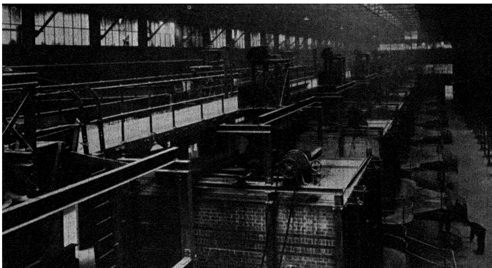
Fig. 1. —BATTERY OF CONTINUOUS HYDROCHLORIC ACID FURNACES.
