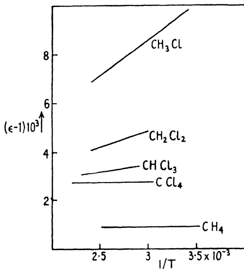
FIG. 22. Temperature-dependence of the dielectric constant of various gases according to Sanger [S1].
