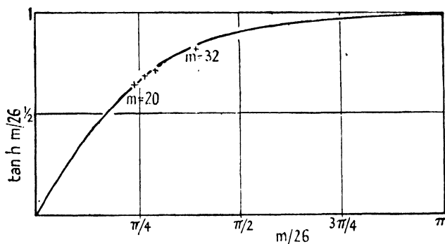
FIG. 32. Comparison of the theoretical dependence of the relaxation time on chain length with experimental values, according to [F5].
