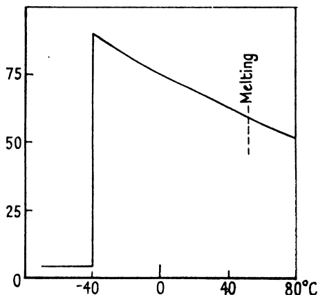
FIG. 34. Temperature-dependence of the dielectric constant of solid ethylene cyanide according to White and Morgan [W4] showing an order-disorder transition near -40^\circ\text{C} . without a discontinuity at melting.
