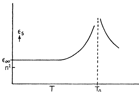
FIG. 10. Temperature-dependence of the dielectric constant of a dipolar solid showing an order-disorder transition, schematically.
