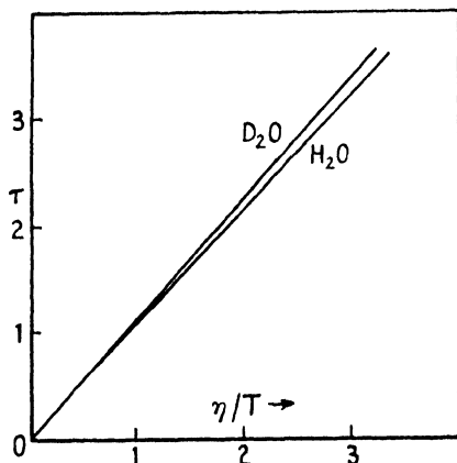
FIG. 42. Dependence of relaxation time \tau on \eta/T ( \eta = viscosity) for water and heavy water, according to Collie, Hasted, and Ritson [C3].
