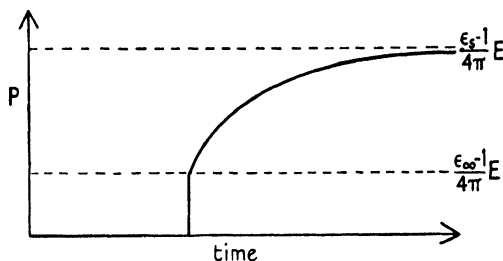
FIG. 2. Time-dependence of the polarization P of a dielectric when a constant electric field E is suddenly applied to it.
