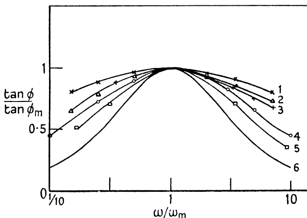
FIG. 37. Frequency-dependence of loss angle according to Hartshorn, Megson, and Rushton [HI] for various materials.
