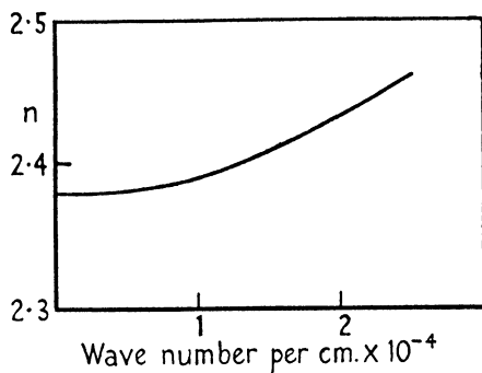
FIG. 19. Dependence of the refractive index n of diamond on the wave number according to measurements collected by Whitehead and Hackett [W6].
