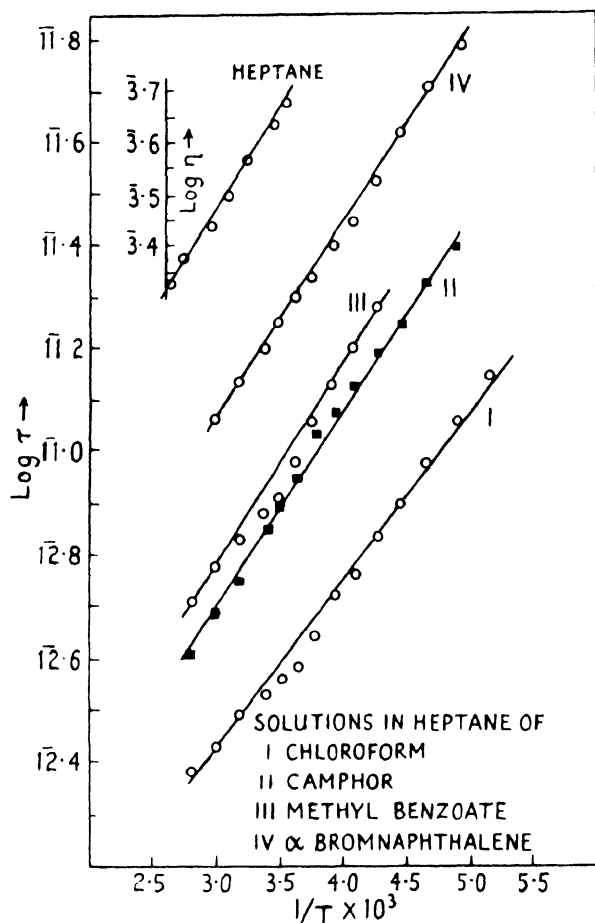
FIG. 27. Temperature-dependence of the relaxation time \tau of various solutions in heptane, and of the viscosity \eta of heptane, according to Whiffen and Thompson [W2].
