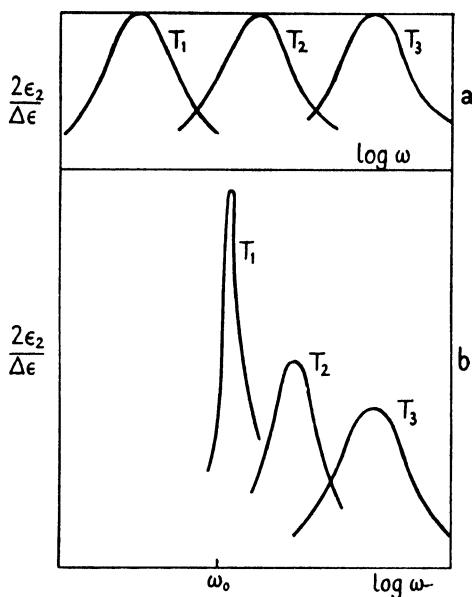
FIG. 17. Frequency dependence of dielectric loss for three different temperatures T_1 < T_2 < T_3 (schematically). (a) Debye case; (b) resonance case.
