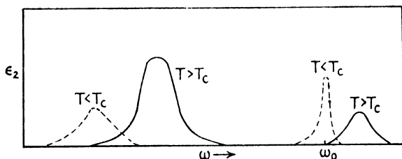
FIG. 36. Frequency-dependence of dielectric loss, ——— above and - - - - below the transition temperature T_c (schematically). \omega_0/2\pi represents the lowest resonance frequency which is usually in the far infra-red or in the ultra-high electric frequency region.
