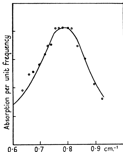
FIG. 24. Calculated and measured absorption spectrum of ammonia at 10 cm. pressure according to Bleaney and Penrose [B3].
