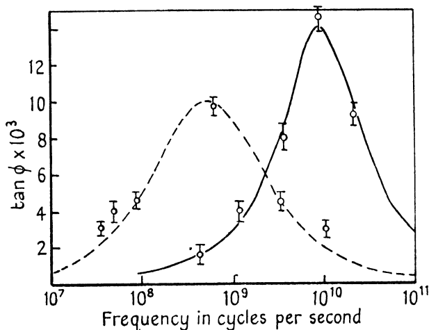
FIG. 25. Loss angle of dilute solutions of benzophenone in benzene (maximum near 10^{10} cycles) and paraffin; experimental values according to Jackson and Powles [J3]. The full line represents a Debye curve (equation 16.6, or 16.8 with \beta = 1 ); the dotted line represents equation 16.8 with \beta = 5 .
