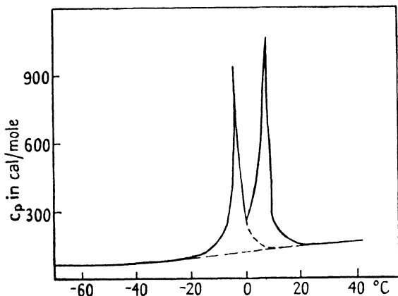
FIG. 46. Temperature-dependence of the specific heat c_p of a paraffin ( m = 15 ) according to Ubbelohde [U1], showing a transition at about -3^\circ \text{C.} and melting. Extrapolations of 'normal' specific heat is indicated.
