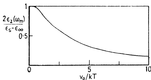
FIG. 15. Dependence of the maximum value of the loss, \epsilon_2(\omega_m) , on the width v_0 of the range of heights of potential barriers.
