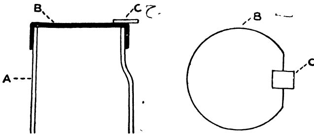
FIG 76—Diagram to show the principle of Wiggers' optical manometer a , seen in vertical section b , view from above A metal tube A, flattened on one side, has covering its open end a tightly stretched rubber membrane B In the middle of the flattened part of the metal tube is a light mirror C The metal tube is connected with the arterial cannula by thick rubber tubing the whole is filled with sodium bicarbonate solution.
