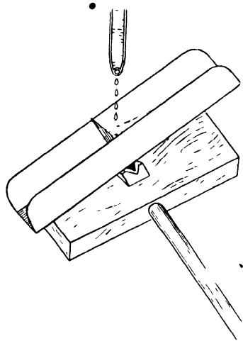
FIG 83—Diagram of tilter The rocking movements are recorded either by allowing the accumulated fluid to actuate a tambour, or by an electro-magnetic signal
