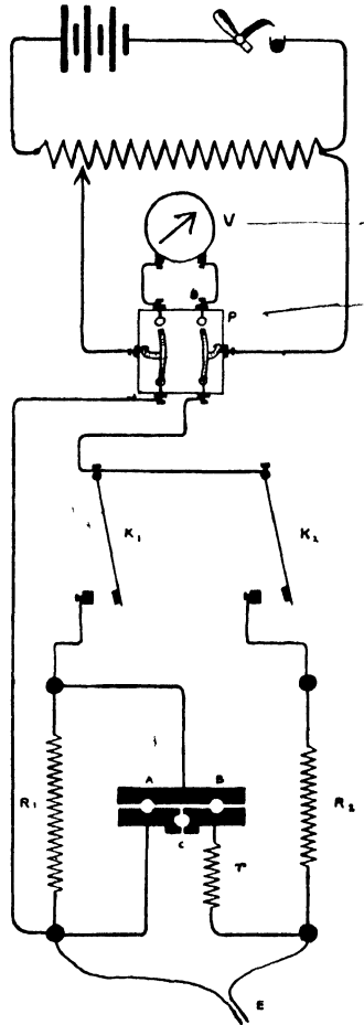
FIG 47—Diagram of circuit for determination of excitation-time by Keith-Lucas pendulum. K_1 and K_2 represent the keys of the pendulum, R_1 , R_2 , and r are non-inductively wound resistances of 10,000\omega , 7,000\omega , and 3,000\omega respectively, by means of one or more plugs in the holes at A, B, or C, the resistances may be combined in different ways. The electrodes E are non-polarisable (Ag-AgCl).
