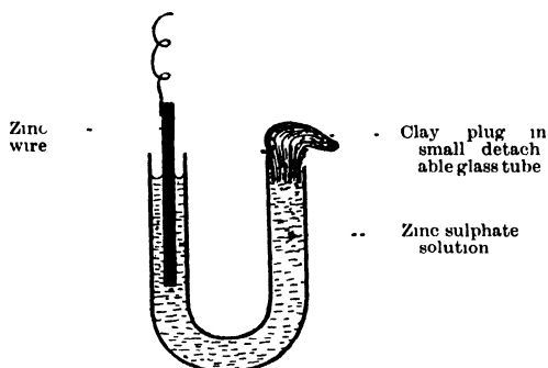
FIG 8—Sanderson's pattern of non-polarisable electrode
