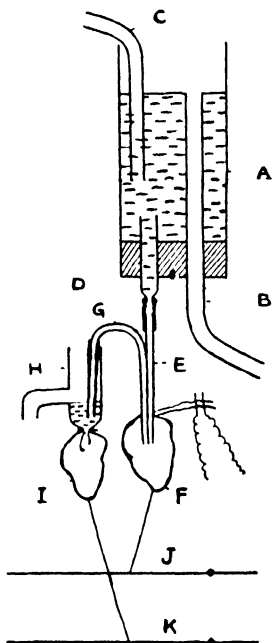
FIG 68 —The perfusion apparatus A is provided with an overflow tube B, the height of which can be varied, thus altering the perfusion pressure. The apparatus is supplied with fluid through the tube C, which is connected with a reservoir of Clark's solution (not shown in diagram). The fluid from A passes through the tube D to the inflow limb E of the double cannula which supplies the donor heart F. After irrigating the inside of the donor heart, the fluid passes by the outflow limb G to the glass cannulated tube H, to which is attached the recipient heart I. This cannulated tube is provided with a lateral overflow, so that the hydrostatic pressure of the fluid supplied to the recipient heart remains constant. J and K are the levers to which the hearts F and I are respectively attached.
