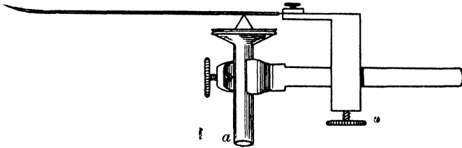
FIG 75—Diagram to show the principle of Fick's or Hurthle's membrane manometer a , tube terminating above in a tambour-like enlargement covered by a stout rubber membrane upon which is a metal disc and a wedge actuating a very light lever. The tube is connected by rubber pressure tubing with a cannula like that shown in Fig 71, and the whole is filled with sodium bicarbonate solution
