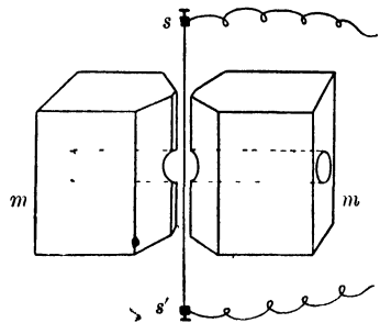
FIG 51.—Diagram of Einthoven string galvanometer. s , s' , wire or silvered quartz thread, stretched between the two poles of a powerful electro-magnet, m , m , which are perforated to allow a microscope to bear upon the thread.
