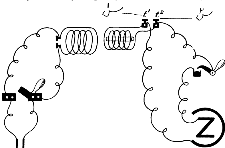
FIG 19.—Induction coil arranged for single shocks.
