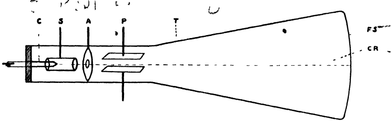
FIG 53—Diagram of cathode-ray oscillograph (Von Ardenne type) T, clear glass tube containing argon at low pressure, C, kathode, A, anode, S, screen for focusing ray, CR, kathode ray, FS, fluorescent screen covering end of tube, P, parallel plates to which action potentials, etc, are led, thus deflecting the ray
