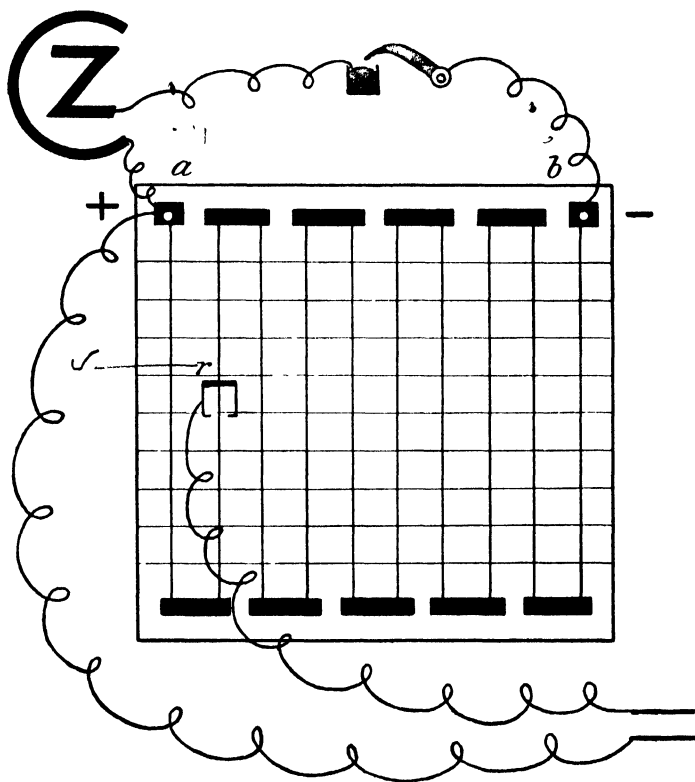
FIG. 18.—Diagram of the Oxford form of rheochord. a , b , rheochord wire zig-zagged upon a mahogany board, marked by cross lines into hundredths, r , rider.
