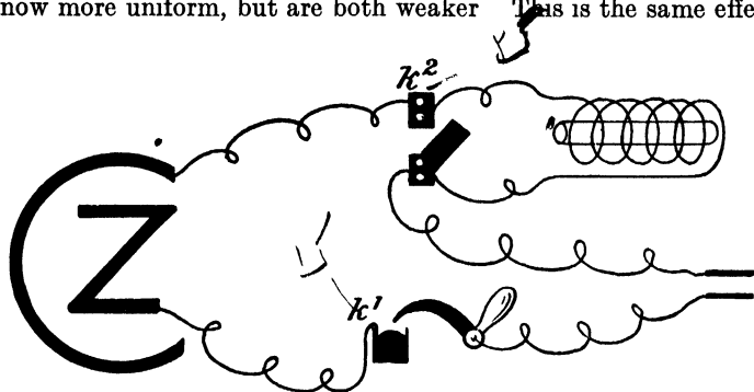
FIG. 22.—Experiment for showing effect of inductance in primary circuit.
