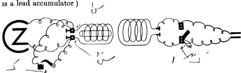
FIG 23.—Diagram of experiment to show the effect of closing and opening a side circuit to primary coil. k , key in side circuit, k^1 , key in secondary circuit
