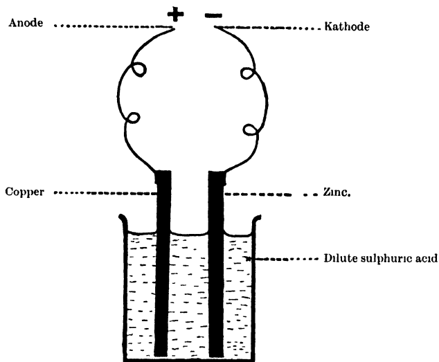
FIG. 1.—Voltaic couple.
