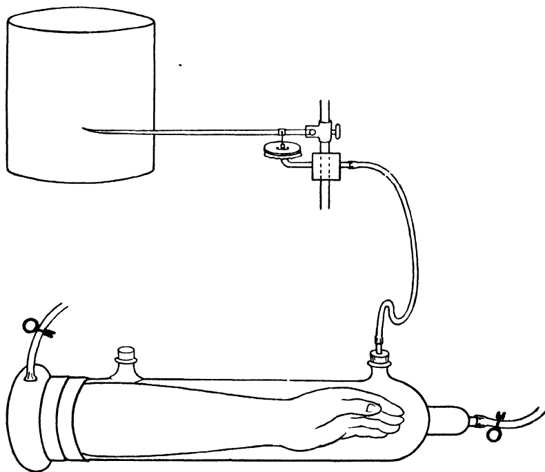
FIG. 81.—Mosso's arm-plethysmograph.
