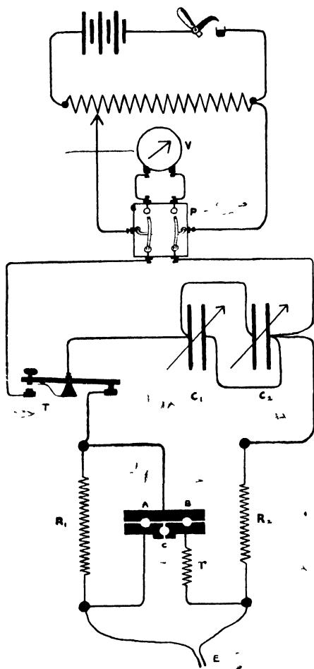
FIG 48.—Diagram of circuit for determination of excitation-time by condensers. C_1 is a condenser of 5 \mu\text{F} capacity, variable in steps of 1 \mu\text{F} , for the determination of the rheobase. C_2 is a condenser of 1 \mu\text{F} total capacity, variable in steps of 0.001 \mu\text{F} , for the determination of the excitation-time. The condensers are charged and discharged by means of the key T. The resistances have the same values as in Fig. 47
