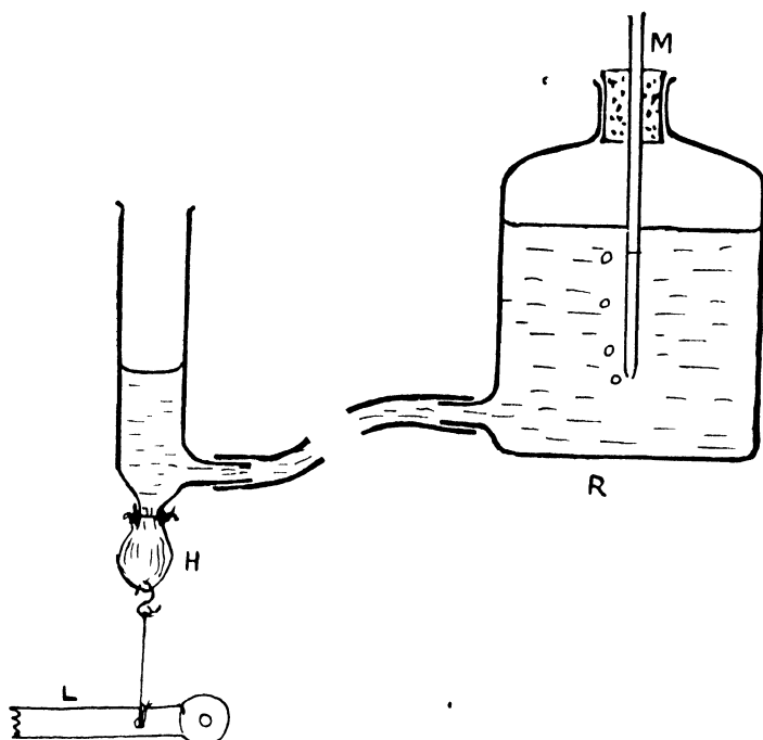
FIG 65—R, reservoir of Ringer's solution, connected with heart cannula by india-rubber tubing provided with a screw-clip (not shown in the diagram), M, Mariotte tube for maintaining a constant pressure, H, heart tied to cannula and connected by fine hook and thread to lever L
