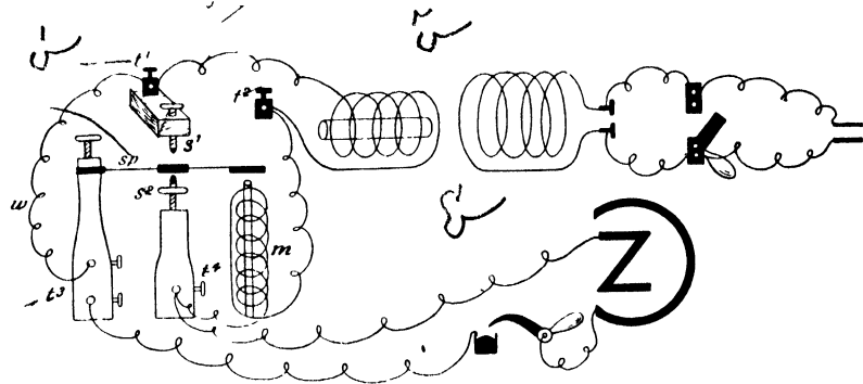
FIG. 21.—Diagram of the arrangements employed in the Helmholtz modification of du Bois-Reymond's induction coil. (For description see text.)
