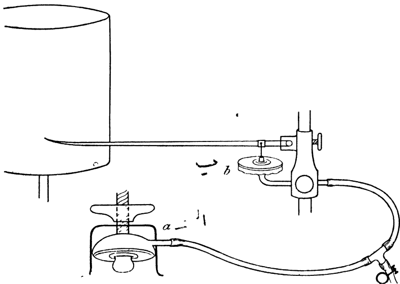
FIG. 72—Diagram of Marey's cardiograph. a , receiving tambour for fixing over apex beat, b , recording tambour connected with a by rubber tubing, with a lateral opening closed by a clip.
