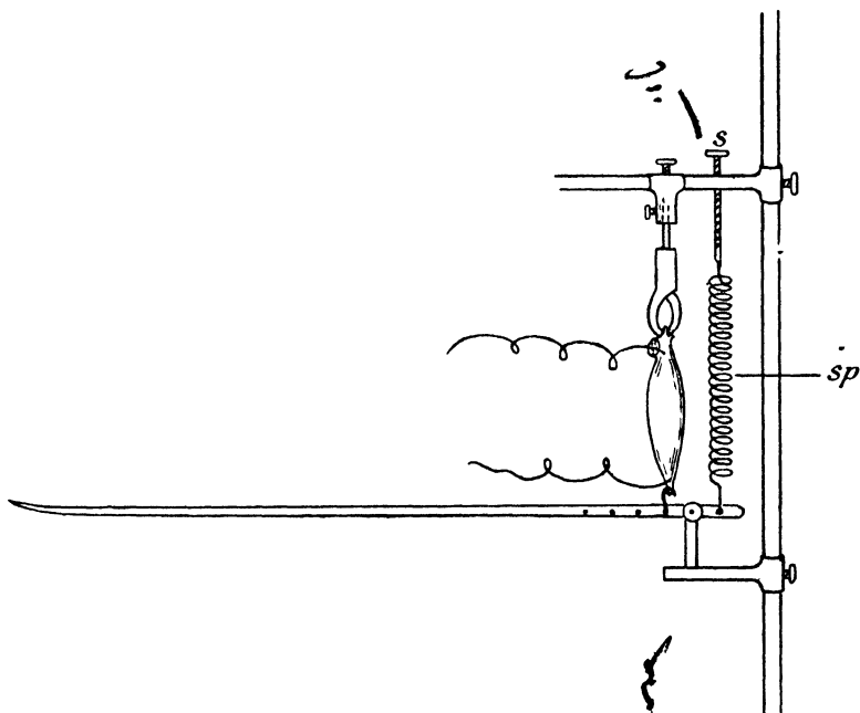
FIG. 31.—Method of studying isometric contraction. sp , spiral spring, s , screw for regulating its tension
