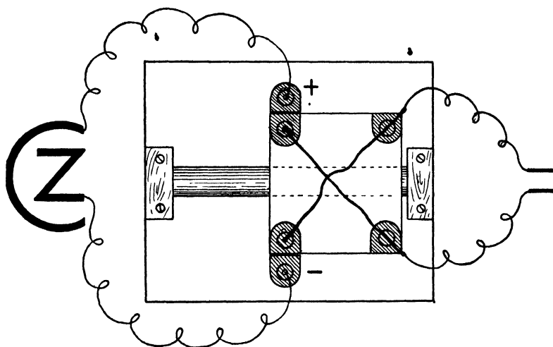
FIG 16 —Diagram of sliding commutator
