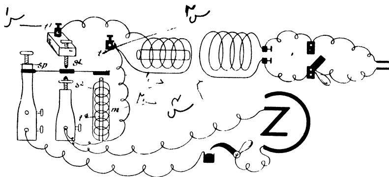
FIG. 20.—Diagram of du Bois-Reymond coil arranged for faradisation with Neef's hammer. (For description see text.)
