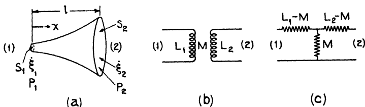
FIG. 18.—FINITE HORN, AND NETWORK EQUIVALENT.
