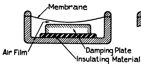
FIG. 4.—SECTION OF CONDENSER TRANSMITTER.
