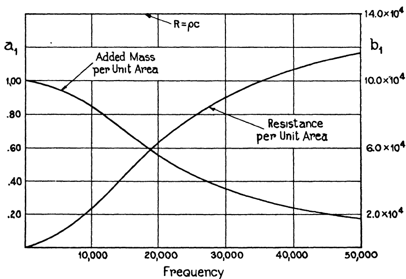
FIG. 13.—REACTIONS ON PULSATING SPHERE OF UNIT RADIUS IMMERSSED IN WATER.
