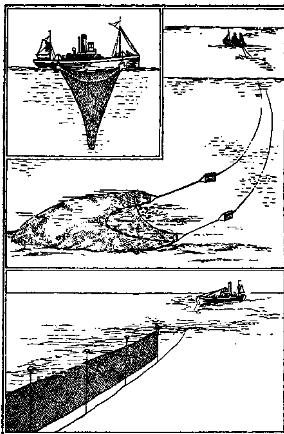
FIG. 12. Upper. Otter trawl, with Vignerón-Dahl extensions, sweeping over the bottom. (Inset: Trawl hauled close to the trawling gallows.) Lower, Herring drifter with drift nets.
