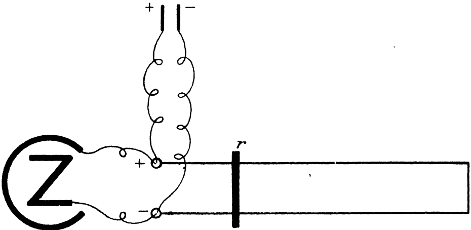
FIG. 21.—Double-wire rheochord.
