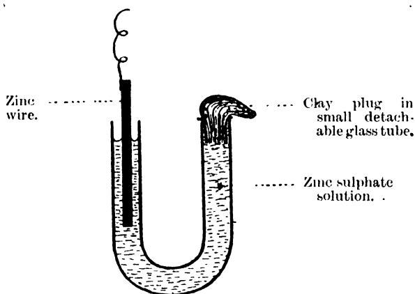
FIG. 8.—Sanderson's pattern of non-polarisable electrode.
