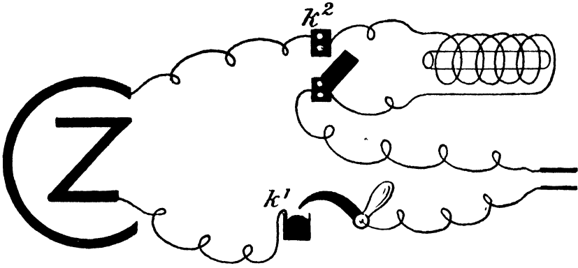
FIG. 25.—Experiment for showing effect of extra current.
