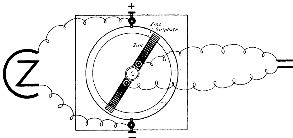
FIG. 30. — Diagram of Fleischl's rheonome.
