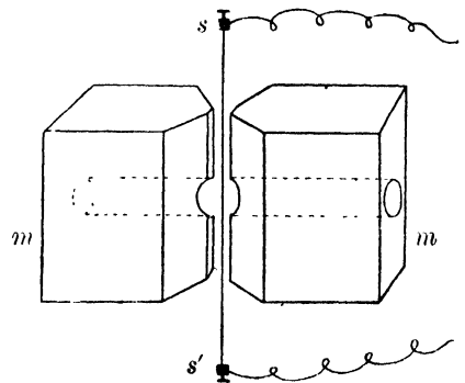
FIG. 54.—Diagram of Einthoven string galvanometer. s, s' , wire or silvered quartz thread, stretched between the two poles of a powerful electro-magnet, m, m , which are perforated to allow a microscope to bear upon the thread.
