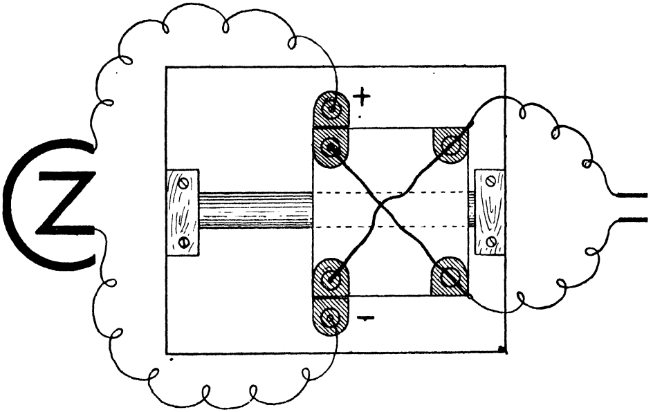
FIG. 18.—Diagram of sliding commutator.
