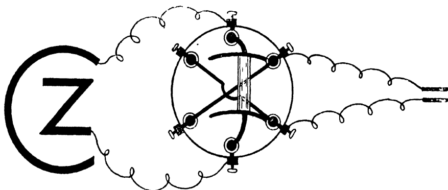
FIG. 15.—Diagram of Pohl's commutator.
