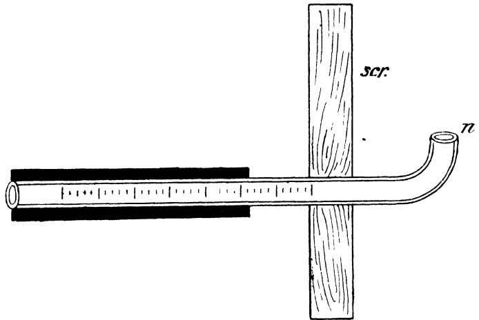
FIG. 90.—Zwaardemaker's olfactometer. n , nose-piece; sc , screen; t , porous tube sliding over graduated glass tube.
