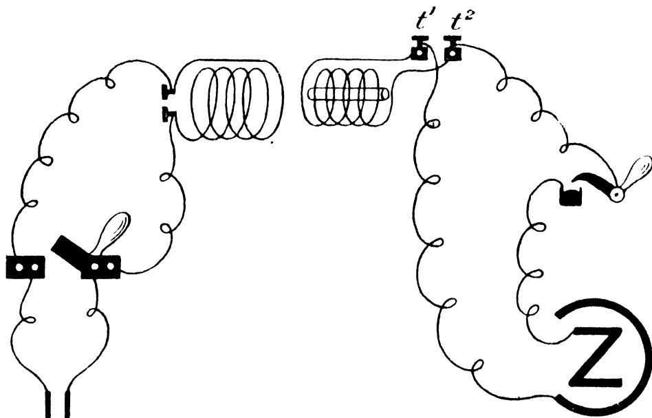
FIG. 22.—Induction coil arranged for single shocks.
