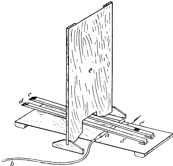
FIG. 86.—Weller's apparatus for reaction time. a , rubber tube closed at one end and at the other connected by b with a tambour (not shown); c , c' , d , d' , levers (with coloured patches) hinged near c' , d' , and resting on the rubber tube, a ; e , wooden screen. ( a should be placed on the other side of the screen.)
