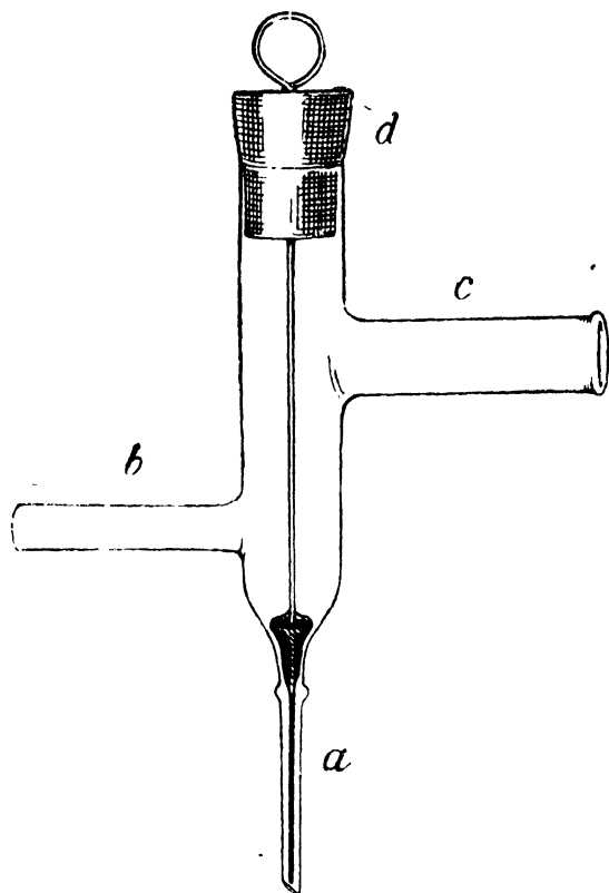
FIG. 73.—Cannula for insertion in the pulmonary artery through the wall of the right ventricle. (a) open end of cannula with plug of Chatterton's cement attached to wire passing through cork, d; b, lateral tube for connecting with recording apparatus; c, wash-out tube.
