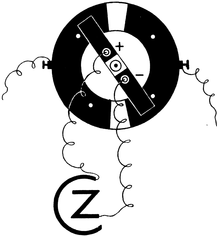
FIG. 17.—Rotatory commutator.
