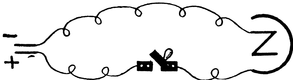
FIG. 12.—Friction key in a battery circuit; direct method of use.
