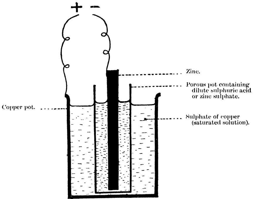
FIG. 3.—Daniell cell.
