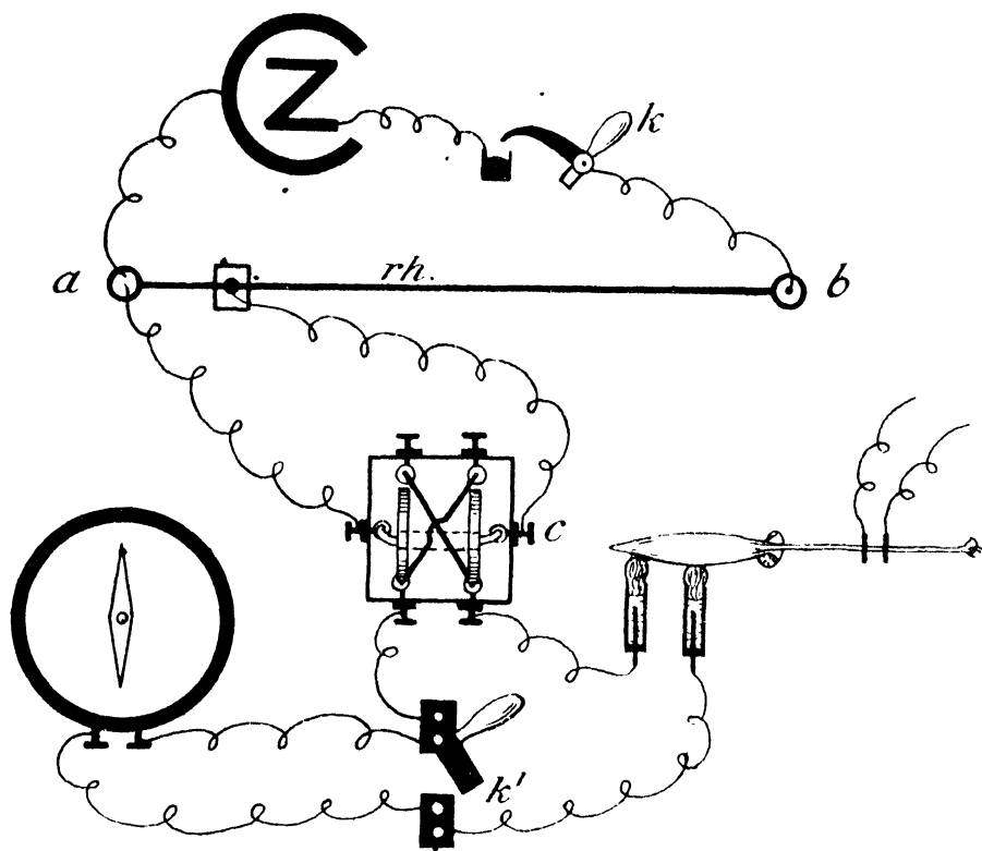
FIG. 55.—Diagram of arrangement of apparatus for studying muscle currents with galvanometer. g , galvanometer. The other letters as in Fig. 53.
