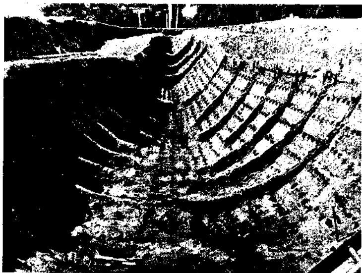
THE LINES OF THE GREAT OPEN ROWING-BOAT OF SUTTON HOO, SUFFOLK. Sixth-seventh century
