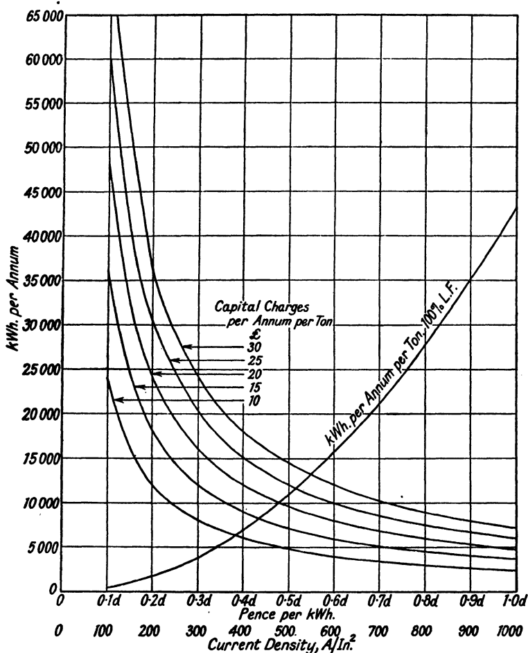
FIG. 1. CURVES RELATING CAPITAL CHARGES PER ANNUM AND KWH. PER ANNUM PER TON AT 100 PER CENT LOAD FACTOR
