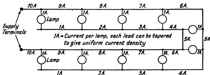
FIG. 6. EQUI-VOLTAGE LOOP FOR STREET LIGHTING
