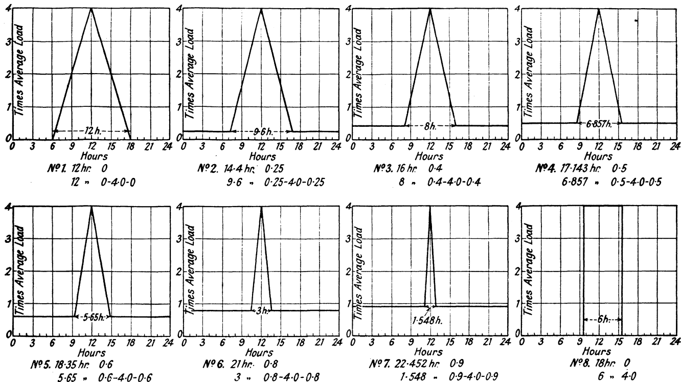
FIG. 3. EIGHT LOAD DIAGRAMS FOR ONE DAY All of 25% load factor: identical maximum and average loads.
