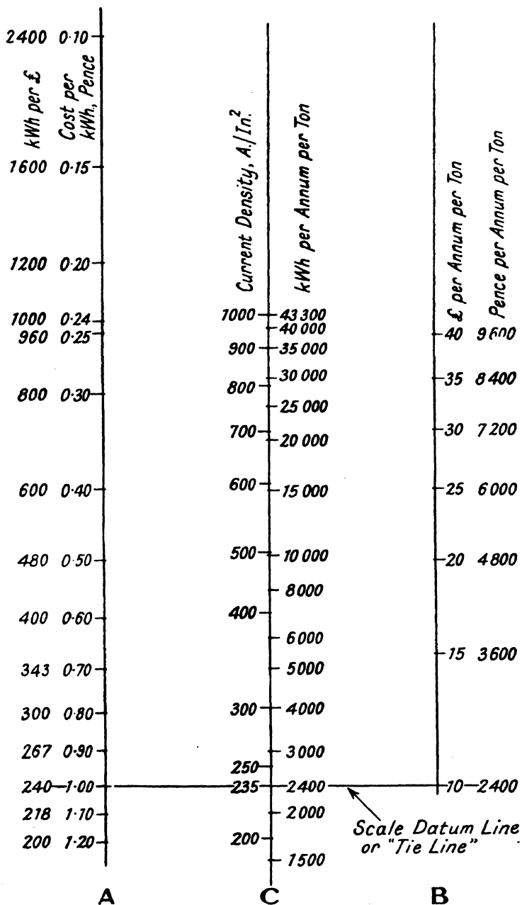
FIG. 2. NOMOGRAM EXPRESSING THE RELATIONS SHOWN IN FIG. 1
