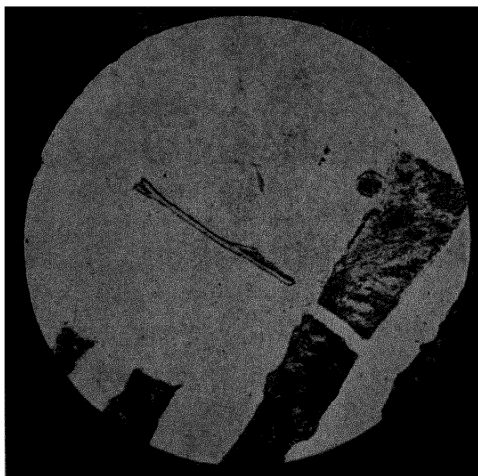
FIG. 37.—"STRUCTURAL EQUILIBRIUM," CEMENTITE AND FERRITE. Alloy No. 8.—C = 0.55% ( \times 100 ).
