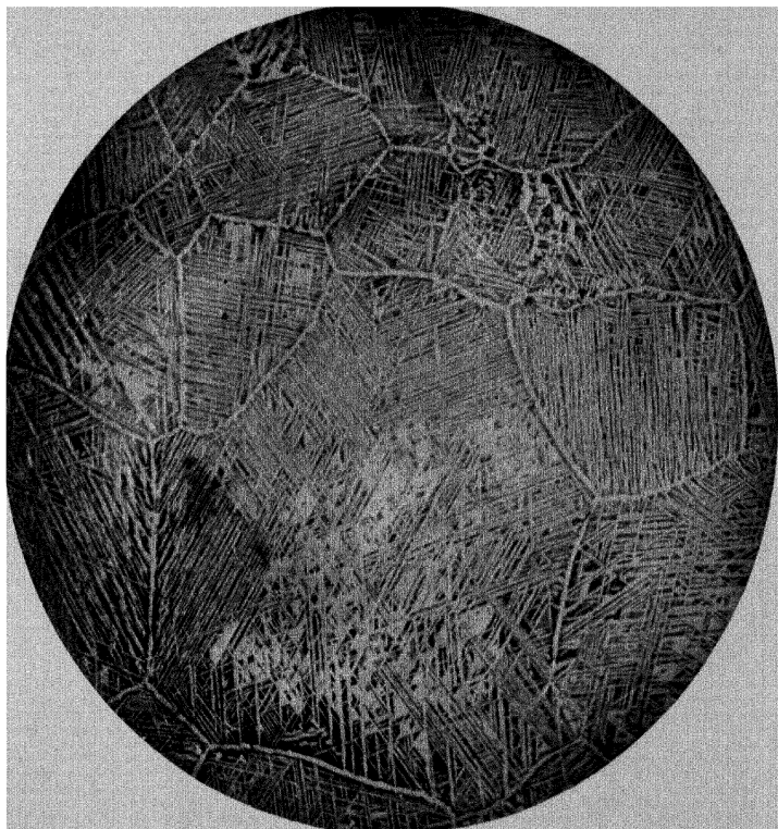
PHOT. 10 - "WIDMANSTATTEN STRUCTURE." Alloy No. 8—C = 0.55%—Ferrite and Pearlite—x 5.
