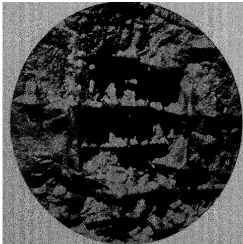
FIG. 3.—STEEL DENDRITES ON THE DAY SURFACE OF THE ALLOY NO. 2 × 10.
