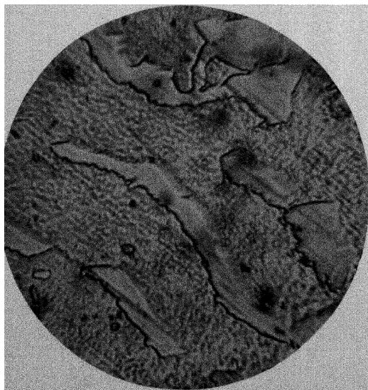
PHOT. 22.— \omega = 83^\circ —Alloy No. 1— \times 2,000 . (B. Broudt in the Author's Laboratory.)
