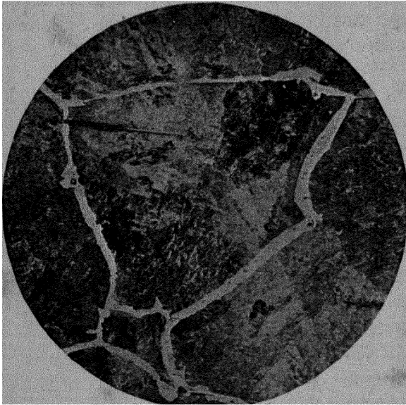
FIG. 30.—PEARLITE GRAINS INSIDE A FERRITE MESH (a former gamma grain). Alloy No. 5—C = 0.60%— \times 40 .
