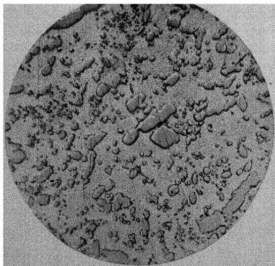
PHOT. 32. Damiron Blade from the Author's collection. C = 1.60% — \times 1,000 . (B. Brandt in the Author's Laboratory.)
