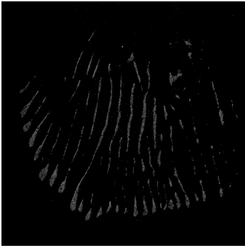
FIG. 36.—“PEARLITE FRINGE” ( \times 250 ). (Stead, Migratory Habit , fig. 4.)
