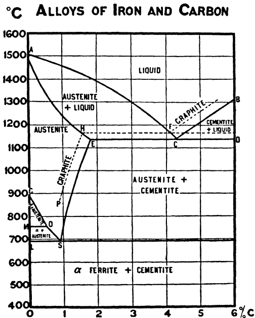
FIG. 20.—IRON CARBON EQUILIBRIUM DIAGRAM.
