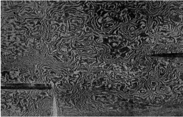
PHOT. 33.—DAMASCINE BLADE NO. 1 FROM D. K. TSCHERNOFF'S COLLECTION. × 5/4.
