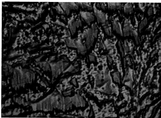
PHOT. 25.—Alloy No. 21- \omega = 6°— \times 3000 (E. Brandt in the Author's Laboratory.)
