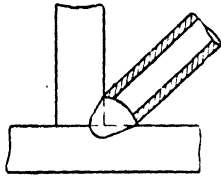
Fig. 72. Touch technique of welding
