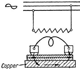
Fig. 141. Diagram of twin-spot welding
