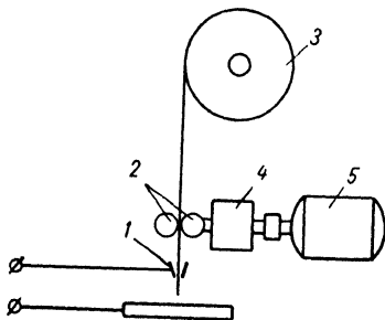
Fig. 118. Diagram of an automatic welding head
