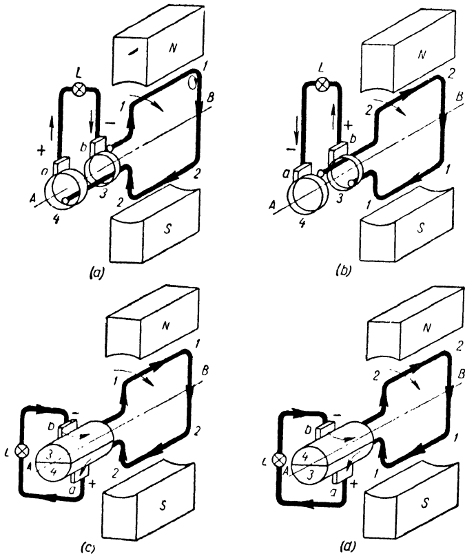
Fig. 11. Operating principle of a commutator.
