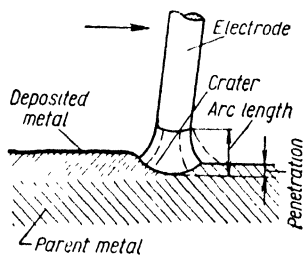
Fig. 27. Diagram of a welding arc
