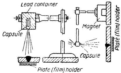
Fig. 147. Weld inspection by gamma-rays
