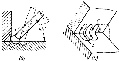
Fig. 65. Electrode motion in welding a fillet weld
