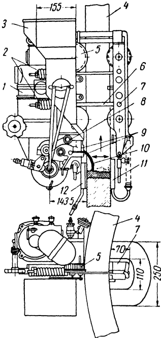
Fig. 132. Automatic machine for vertical seams
