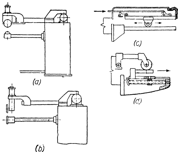
Fig. 143. Seam welding:
