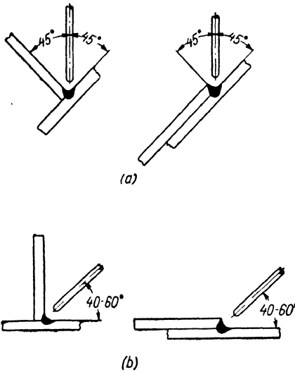
Fig. 126. Electrode and welding position in welding fillet welds
