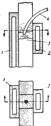
Fig. 130. Electroslag welding as applied to vertical seams
