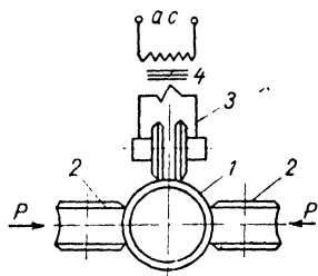
Fig. 144. Diagram of butt-seam welding of pipes
