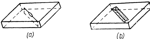
Fig. 93. Preparation of a crack for welding up; a—original crack; b—vee'd-out crack
