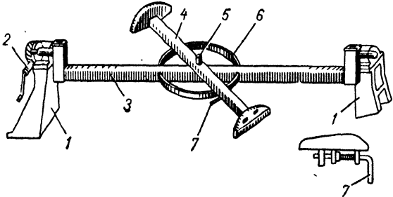
Fig. 104. Hand-operated positioner
