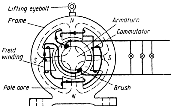
Fig. 12. D.c. shunt-wound generator (as viewed from the commutator end)
