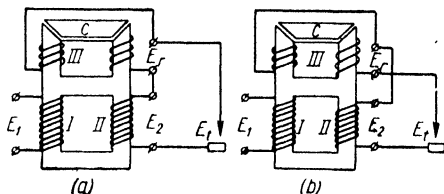
Fig. 39. Diagram of a welding transformer with a reactor wound on a common core
