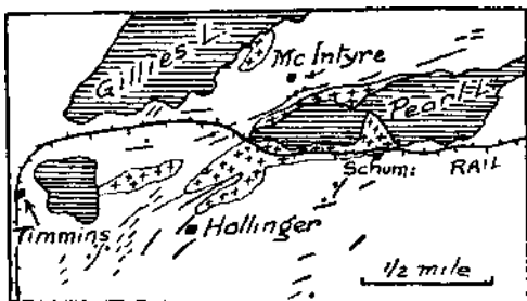
FIG. 137.—The Granite area near the Hollinger and McIntyre mine9 in the Porcupine Goldfield. The numerous veins appear as short lines, and porphyry is shown by crosses. The large dots are mine-shafts
