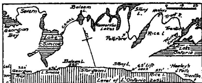
FIG. 147.—Map of the Trent Canal system, linking Lake Huron to Lake Ontario by the Severn and Trent Rivers. Below is a vertical section along the Waterway showing the levels of the smaller lakes above Lake Ontario
