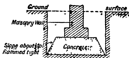
Showing correct method of building concrete foundations
