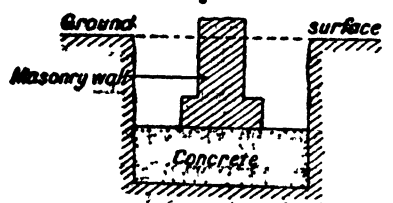
Showing ordinary method of building concrete foundations
