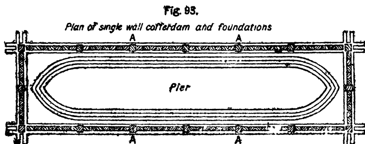
Fig. 93. Plan of single wall coffer-dam and foundations.
