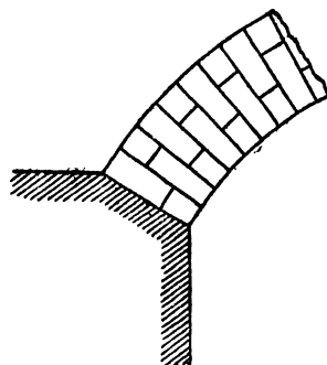
Alternate rings of half and whole bricks
