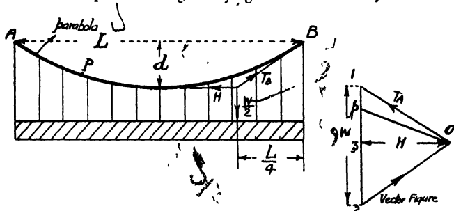
Fig. 157.—Suspension Bridge with Uniform Load.
