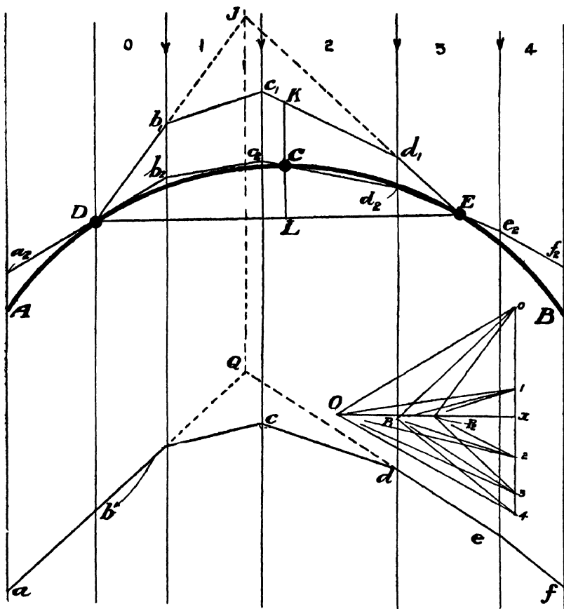
Fig. 168.—Link Polygon through three given Points.
