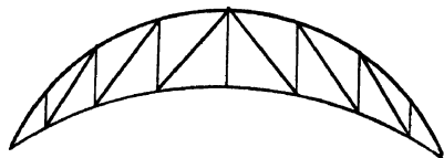
Fig. 237.—Types of Roof Trusses.
