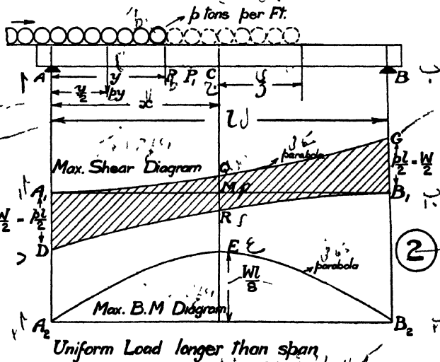
Fig. 81.—Rolling Loads.
