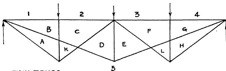
FINK TRUSS.
