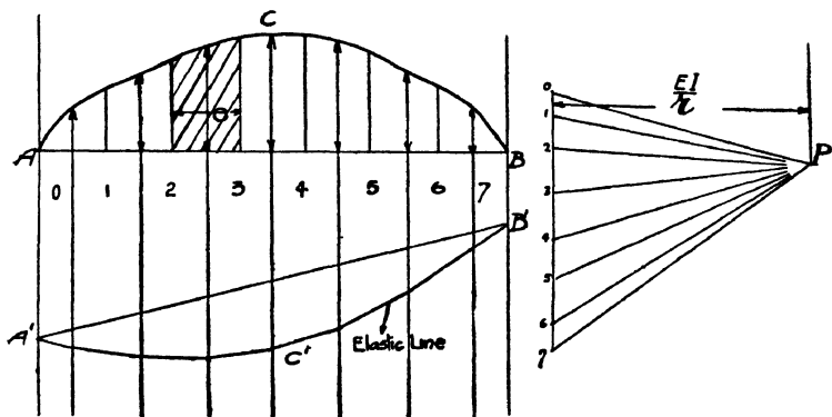
Fig. 89.—Graphical Construction for Deflections.
