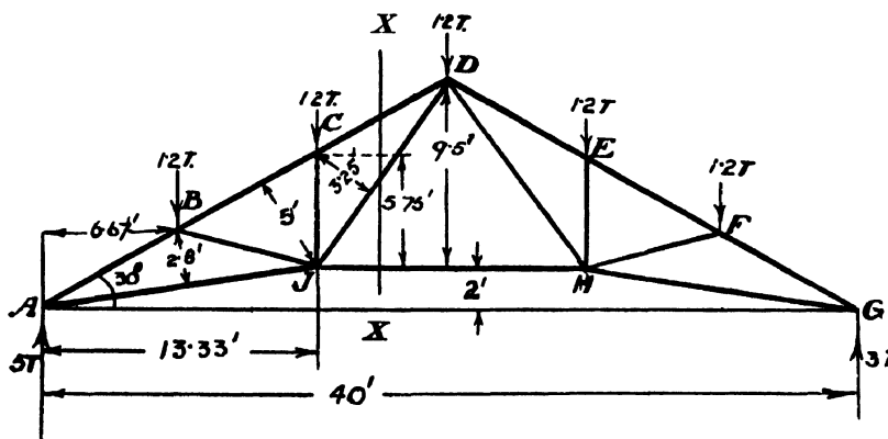
Fig. 140.—Example on Method of Moments.
