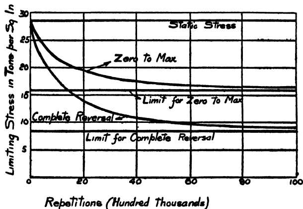
Fig. 10.—Repetitions of Stress.
