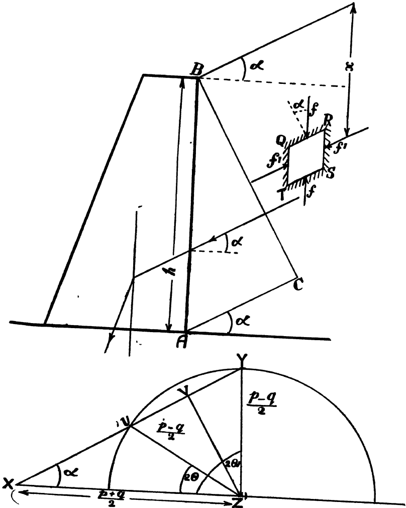
Fig. 185.—Rankine's Theory for Surcharged Retaining Wall.
