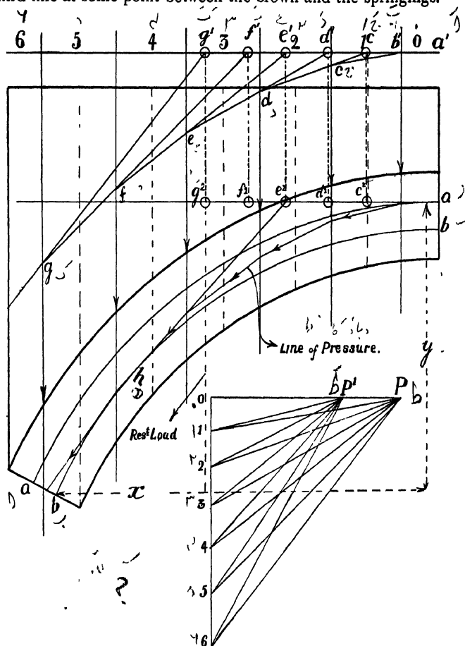
Fig. 195.—Critical Line of Pressure for Masonry Arch.
