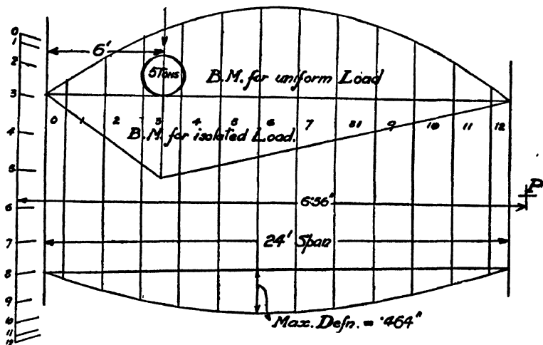
Fig. 90.—Example on Deflections.
