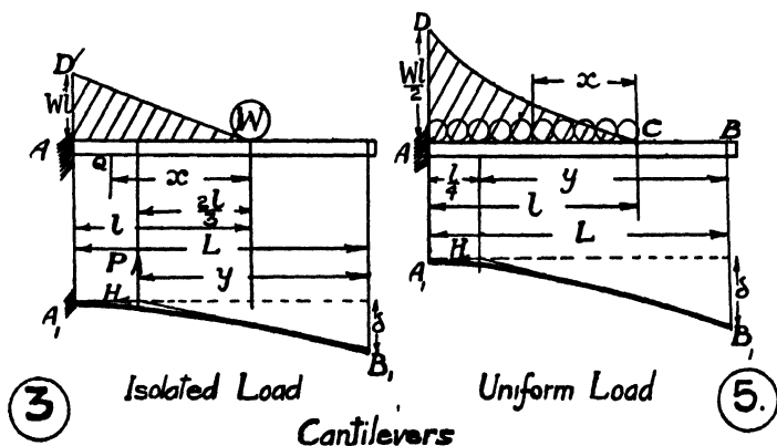
Fig. 87.—Deflections of Beams.
