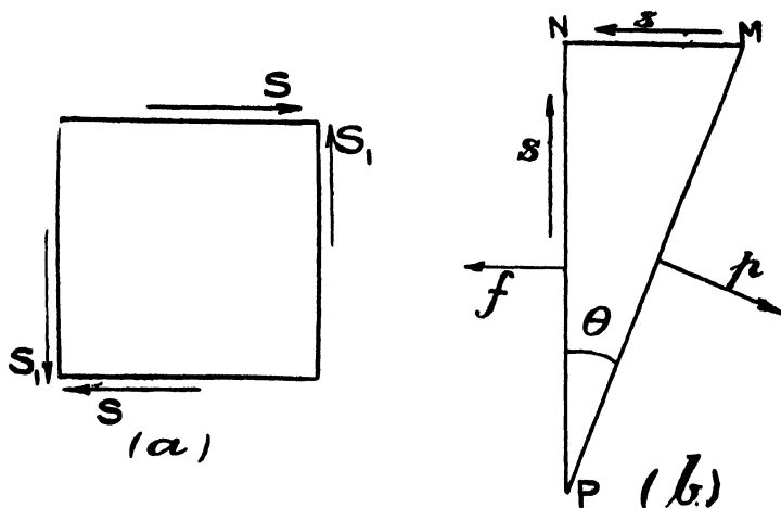
Fig. 7.—Combined Normal and Shear Stress.
