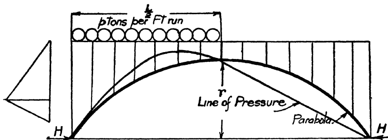
Fig. 166.—Parabolic Arch half covered with Uniform Load.
