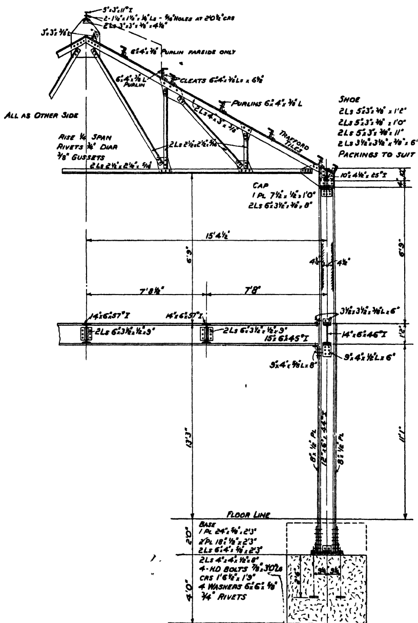
Fig. 239.—Roof Beam and Stanchion: details for two-storey building.
