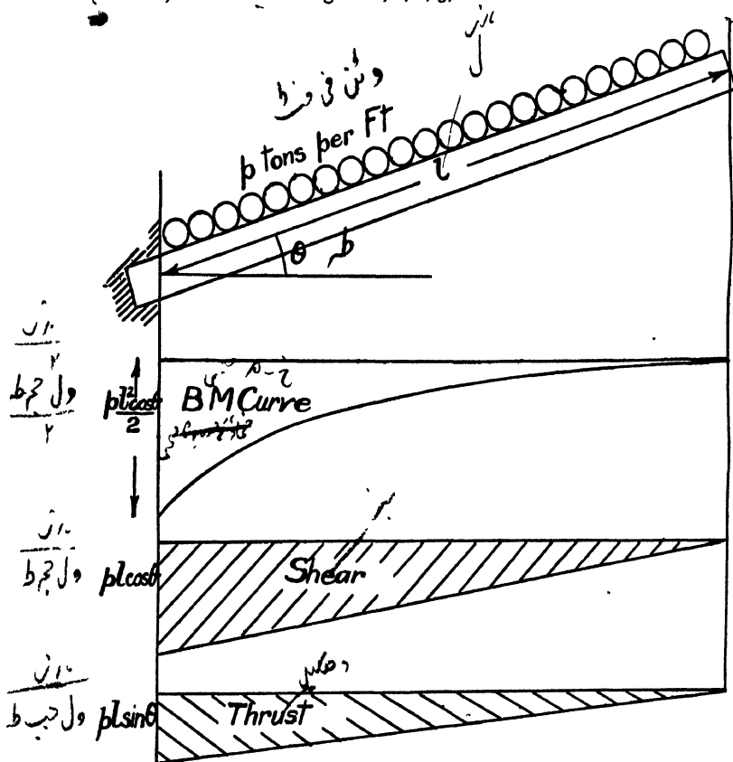
Fig. 65a.—Sloping Cantilever with Uniform Load.
