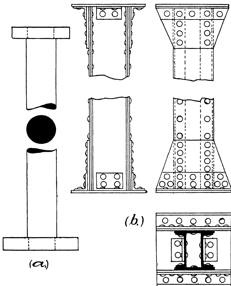
Fig. 215.—Column, Caps, and Bases.
