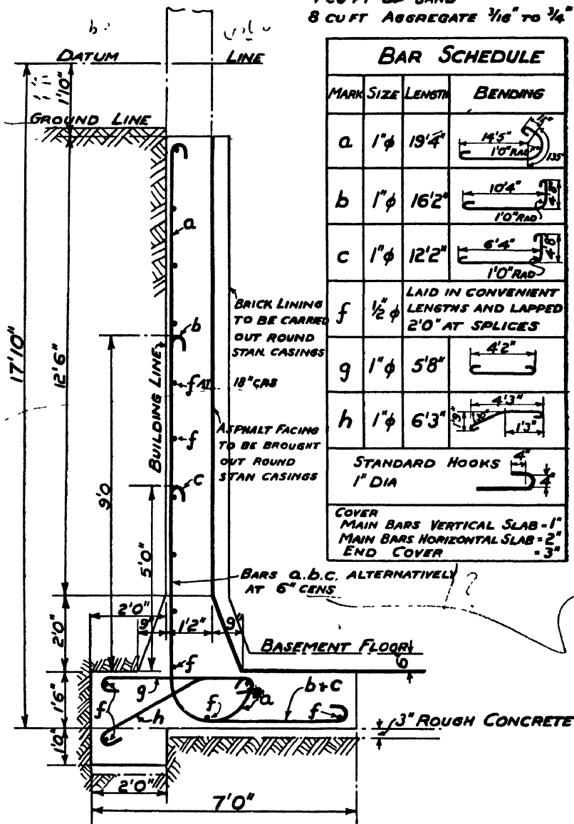
Fig. 212.—Reinforced Concrete Retaining Wall.
