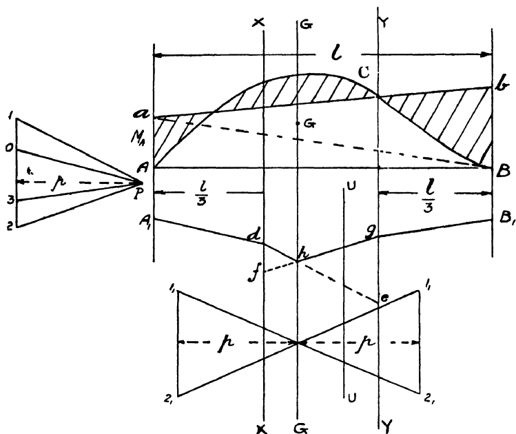
Fig. 107.—Continuous Beams—Graphical Treatment.
