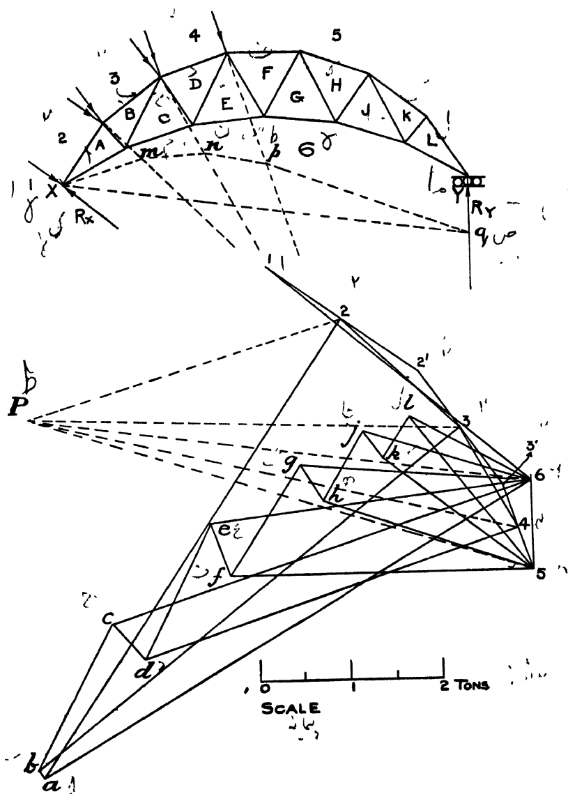
Fig. 136.—Wind Pressure on Curved Roof Truss.
