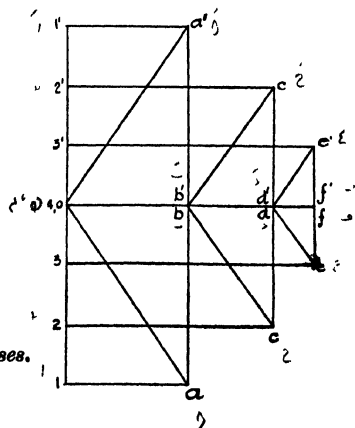
'N' or Linville Girder
