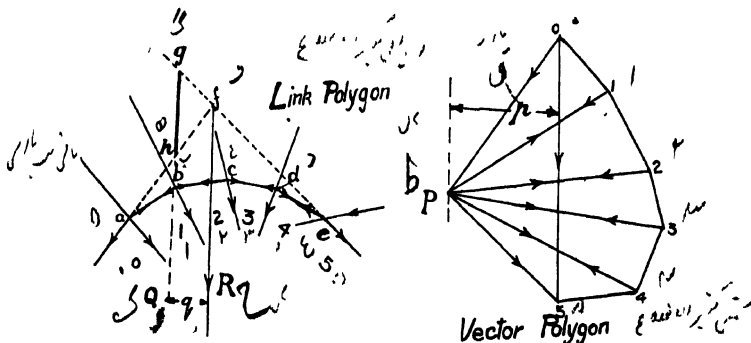
Fig. 16.—Link and Vector Polygon Construction.
