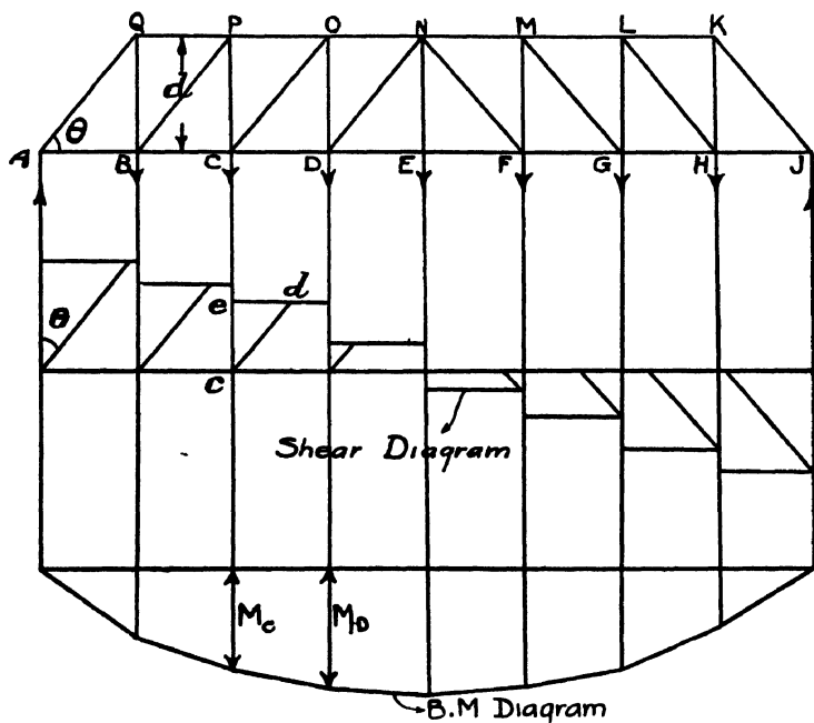
Fig. 142.—Method of Moments for Parallel Girder.
