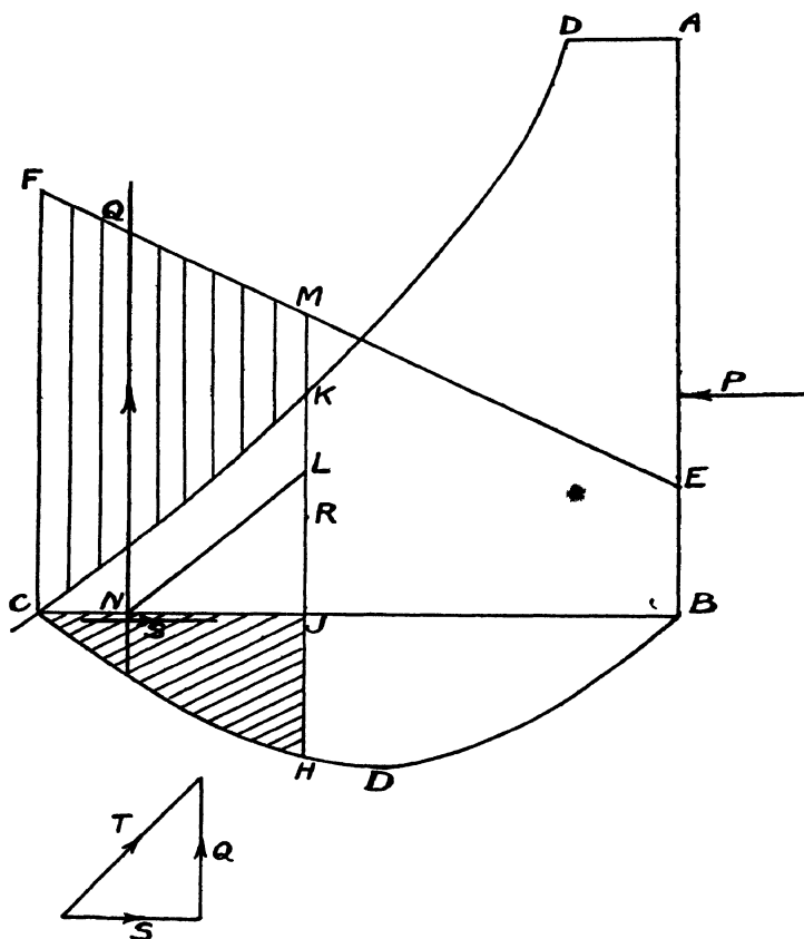
Fig. 180.—Stresses on Vertical Sections of Dams.
