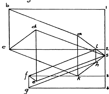
FINK TRUSS.
