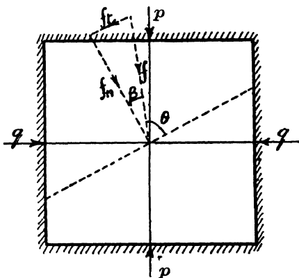
Fig. 182.—Rankine's Theory of Earth Pressure.
