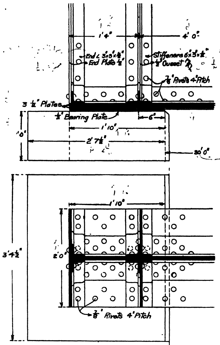
Fig. 273.—Girder Bearings.
