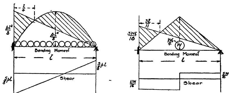
Figs. 110 and 111.—Beams Fixed at one End and Supported at the other.
