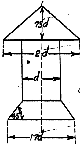
COUNTERSUNK HEAD.
