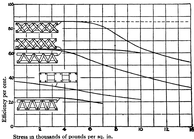
Fig. 154b.—Efficiency of Bracing.
