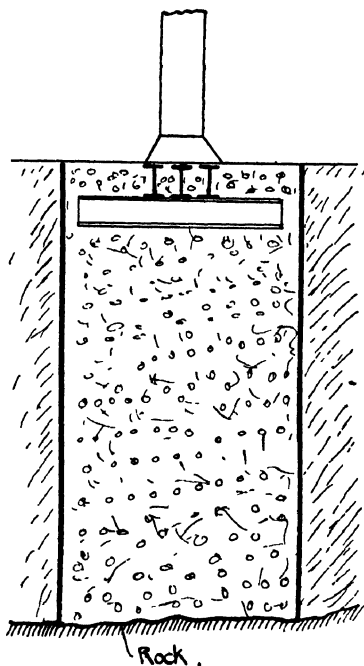
Fig. 224.—Caisson Foundation.
