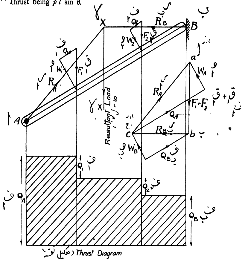
Fig. 65.—Inclined Beam, with Top End freely Supported.
