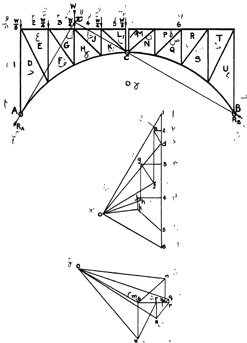
Fig. 132.—Truss with two portions Pin-jointed together.
