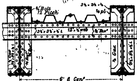
Fig. 256.—Trough Floor for Road Bridge.
