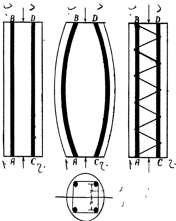
Fig. 208.—Reinforced-concrete Columns.
