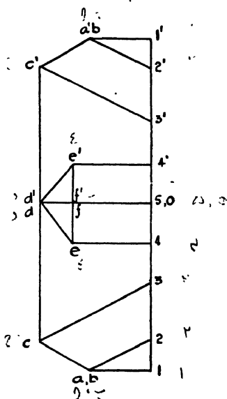
Fig. 128.—Station Roof Truss.
