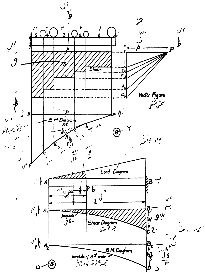
Fig. 53.—B.M. and Shear Diagrams for Cantilevers (continued).
