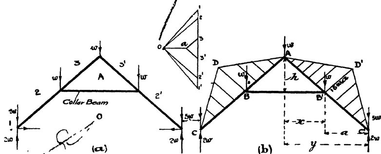
Fig. 248.—Collar Beam Truss.
