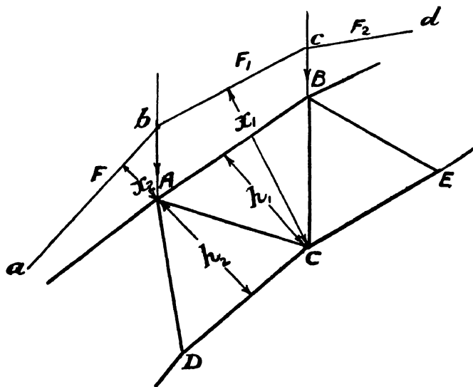
Fig. 145.—Stresses from Line of Pressure.
