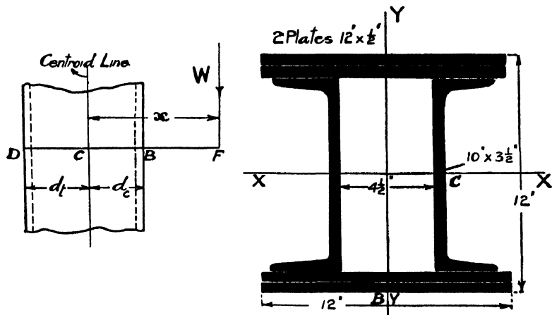
Fig. 155.—Columns with Eccentric Loads.
