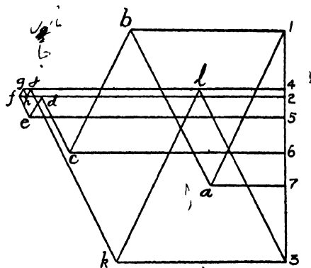
Fig. 125. - Warren Girder unevenly Loaded.
