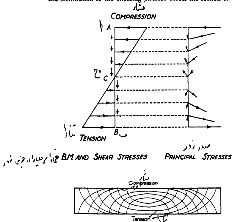
Fig. 72.—Principal Stresses in Beams.
