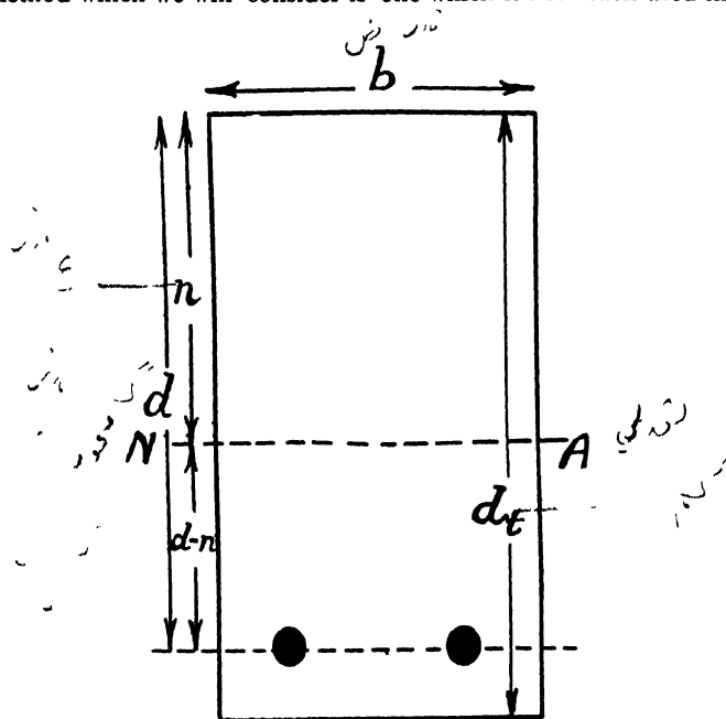
Fig. 198.—Notation for Reinforced-concrete Beams.
