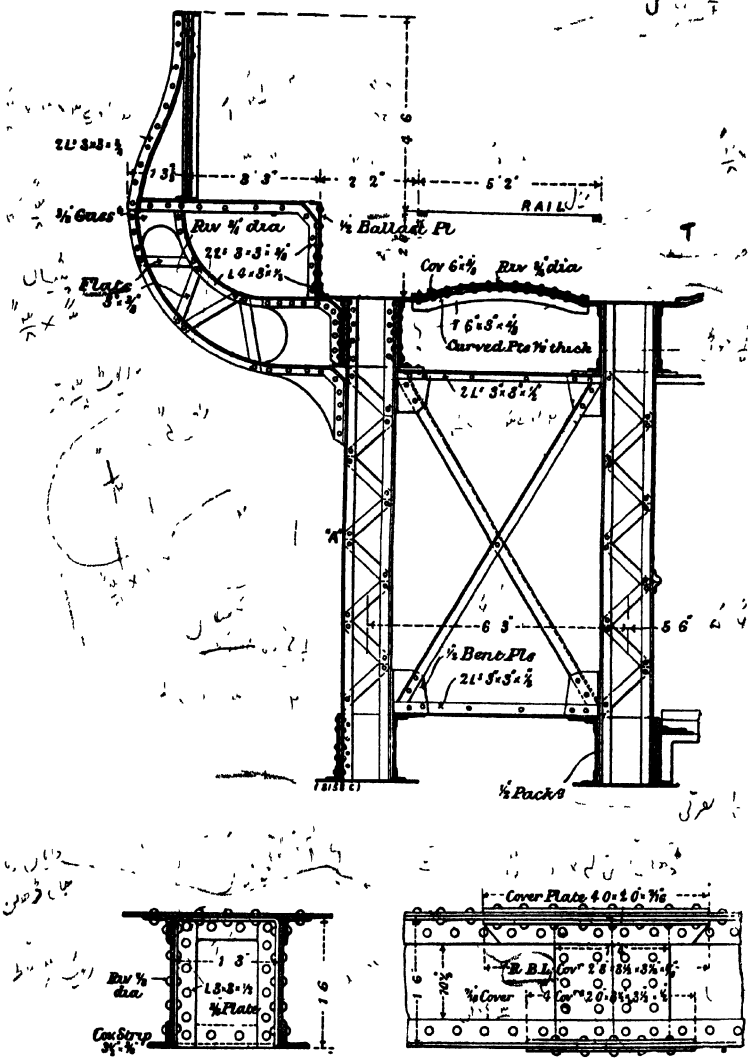
Fig. 272.—Bridge over River Clyde.
