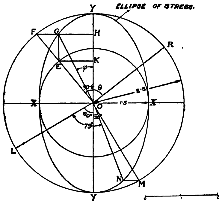
Fig. 6.—Ellipse of Stress.
