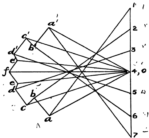
Fig. 131.—Crescent Roof Truss.
