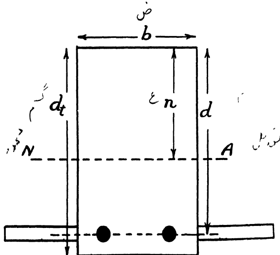
Fig. 199.—Reinforced-concrete Beams. Method 1.
