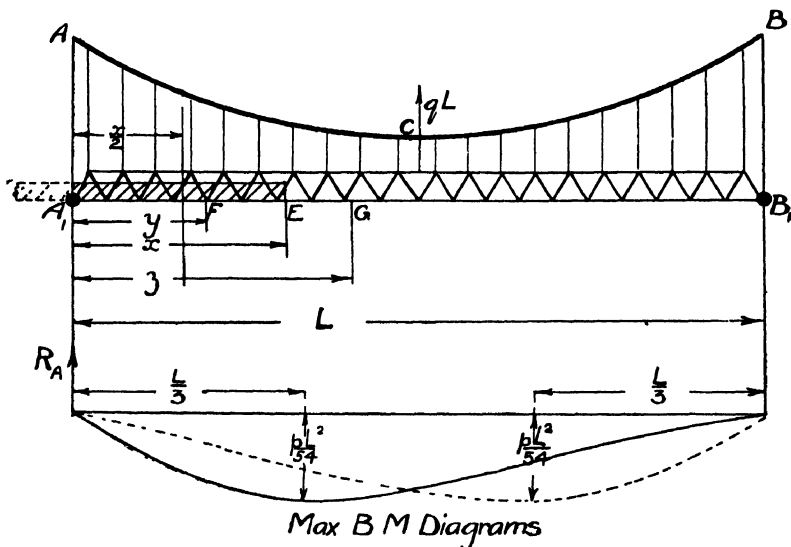
Fig. 183.—Stiffening Girder without Central Hinge.
