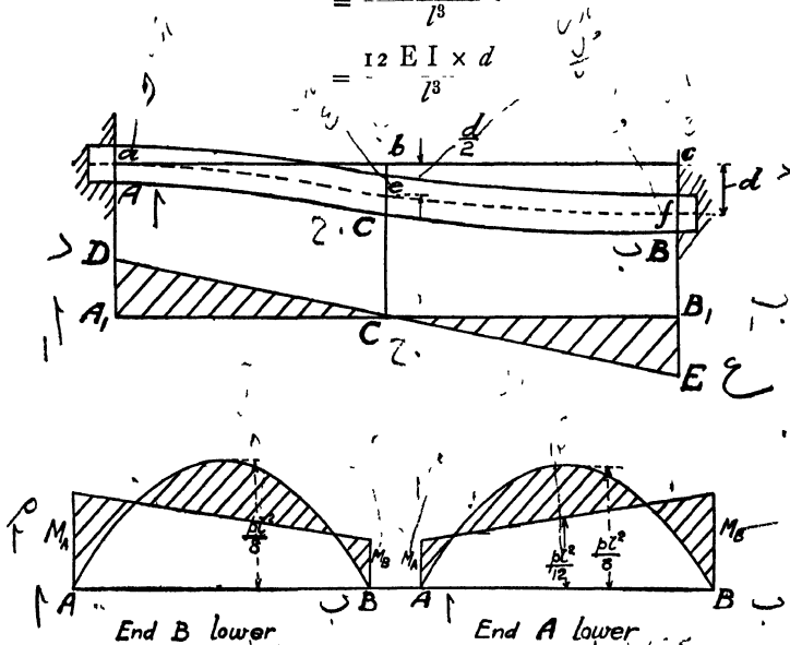
Fig. 99.—Beams with Ends fixed at different Levels.
