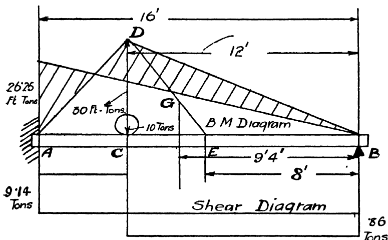
Fig. 113.—Example of Beam Fixed at one End and Supported at other.
