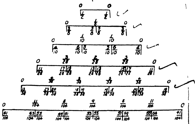
Fig. 106.—B.M. and Reactions on Uniformly Loaded Continuous Beams of Equal Spans.
