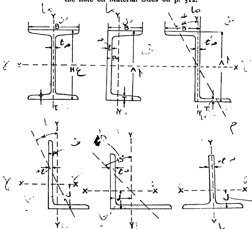
Fig. A.—Properties of British Standard Sections.
