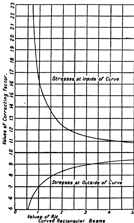
Fig. 75A.—Stresses in Curved Beams.
