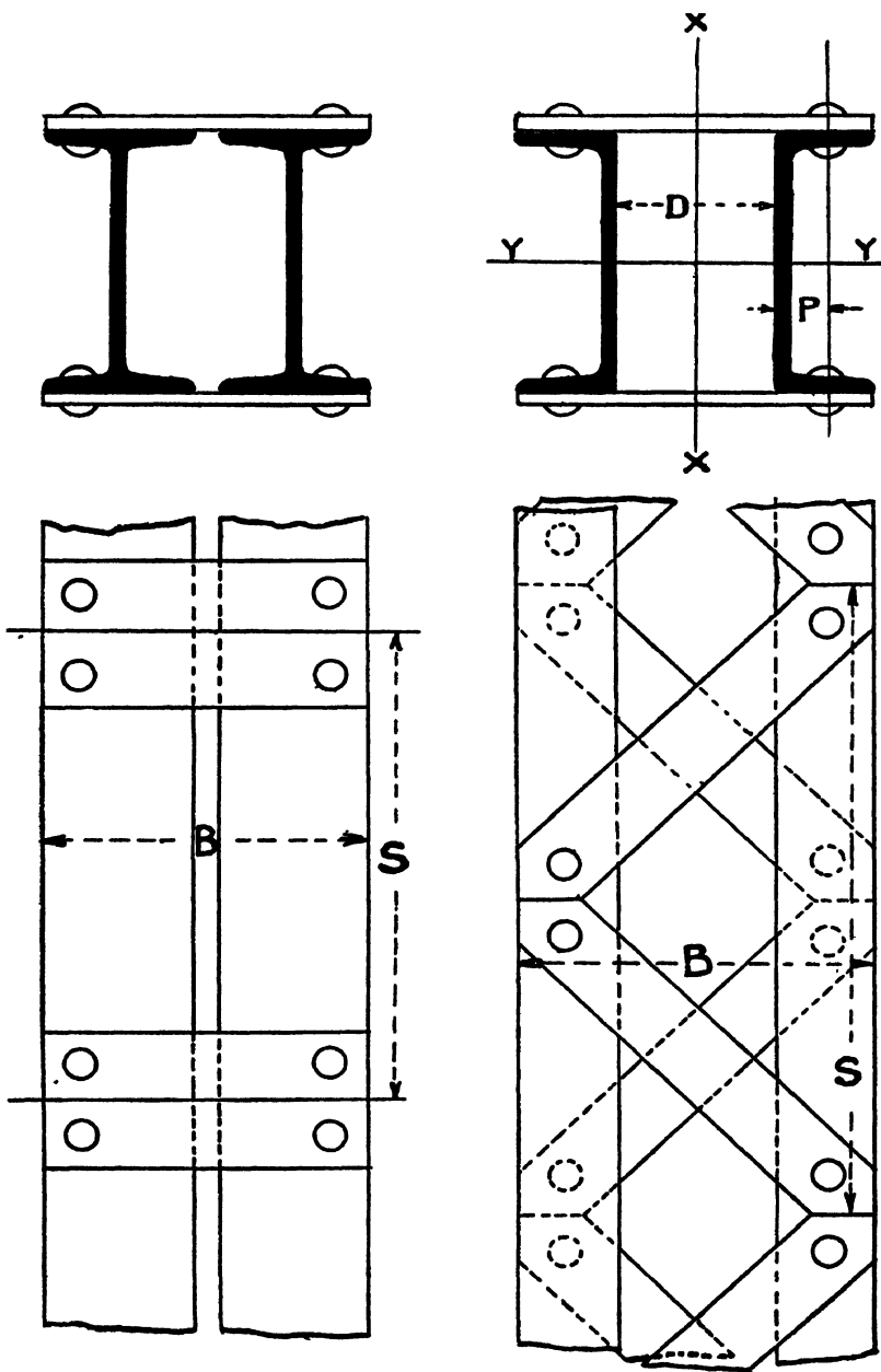
Fig. 154a.—Columns with Open Webs.
