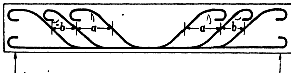
Fig. 206.—Shear Reinforcement.
