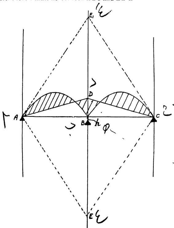
Fig. 103.—Continuous Beam with three Supports
