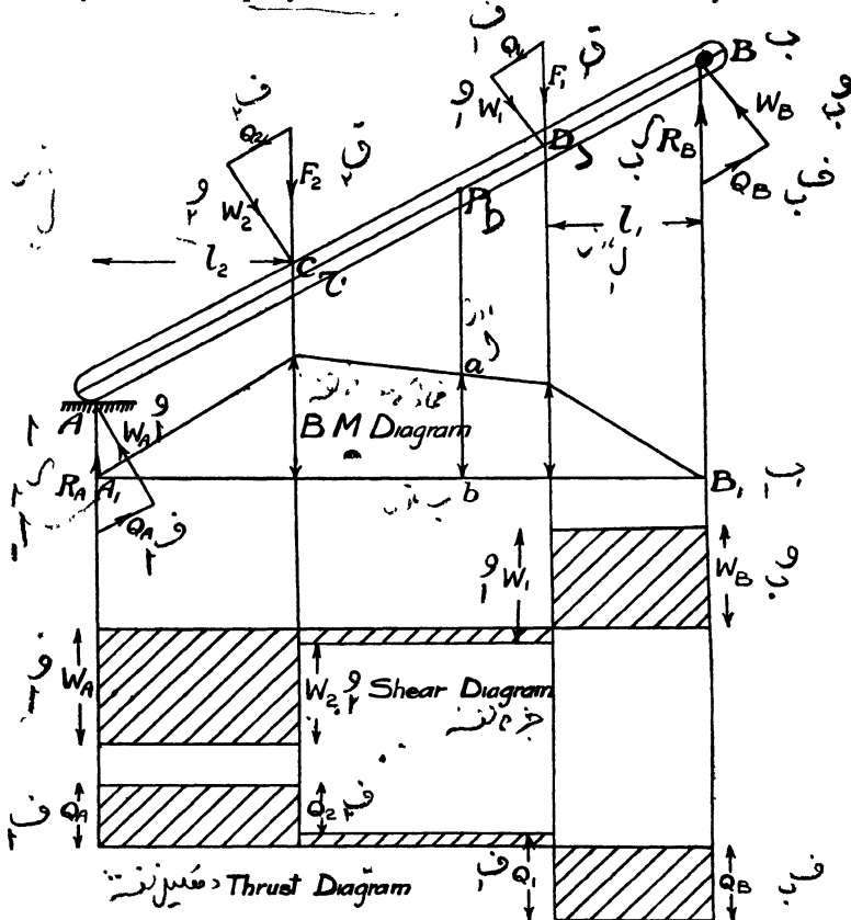
Fig. 64.—Inclined Beam with Lower End freely Supported.
