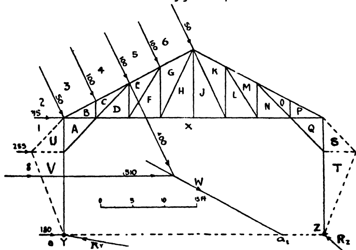
Fig. 138.—Roof Truss with Knee-bracing.
