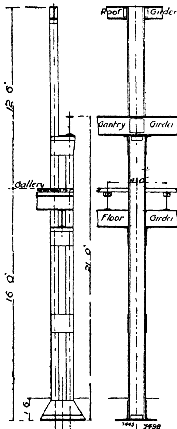
Fig. 219.—Column for Workshop.
