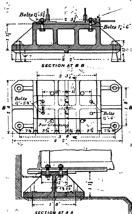
Fig. 274.—Bearing at Fixed End.
