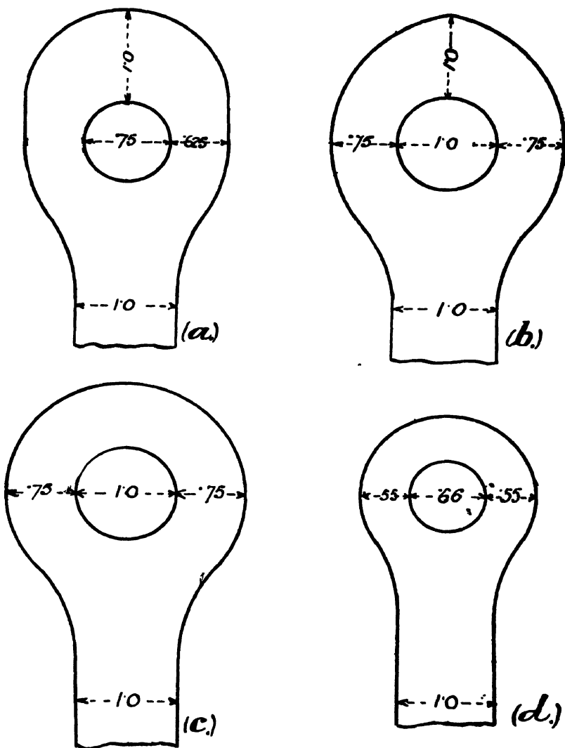
Fig. 245.—Forms of Eye Bars.
