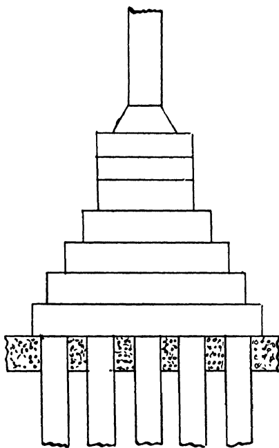
Fig. 223.—Pile Foundation.
