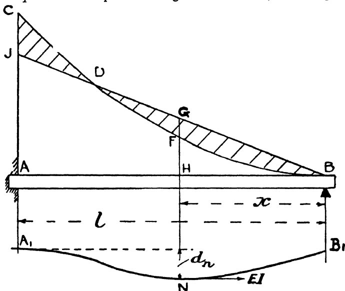
Fig. 93B.—Deflections of Beams.
