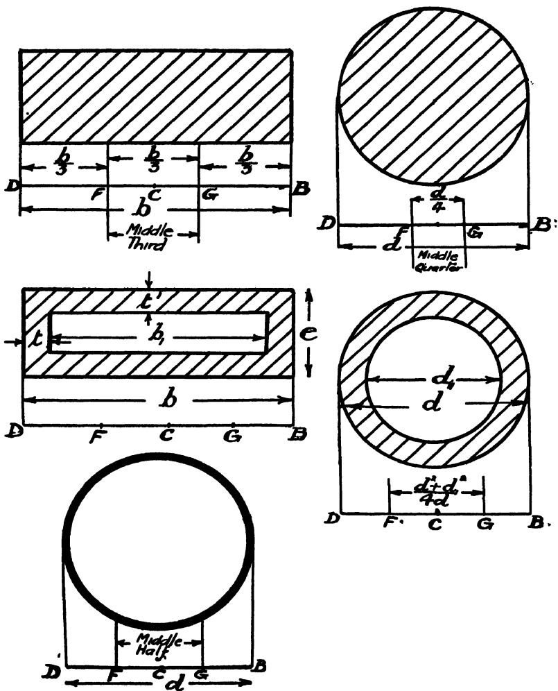
Fig. 174.—Masonry Structures.
