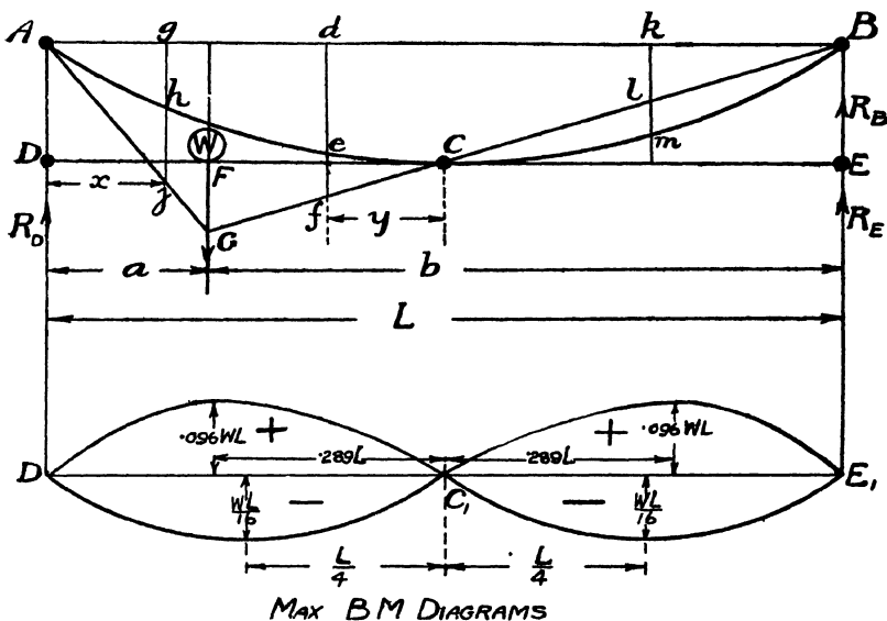
Fig. 161.—Hinged Stiffening Girders with Isolated Rolling Load.
