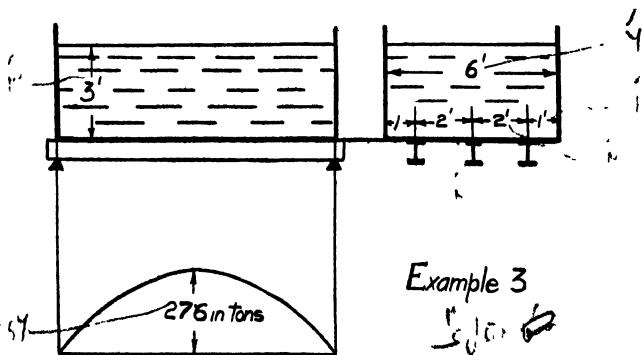
Fig. 70.—Examples of Beams.
