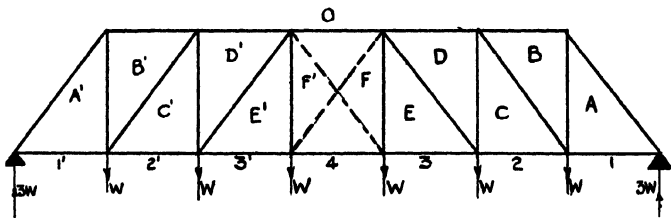
'N' or Linville Girder
