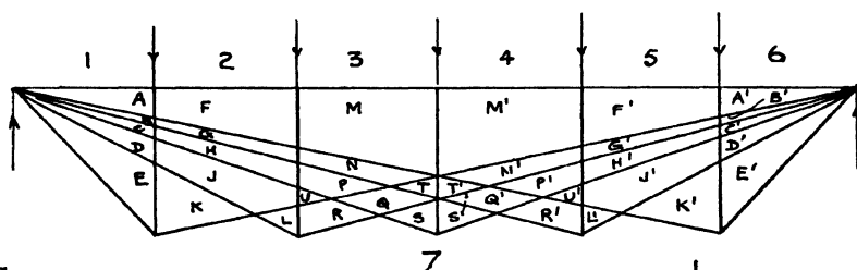
BOLLMAN TRUSS.
