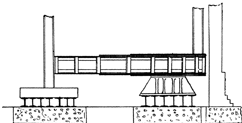
Fig. 225.—Cantilever Foundation.
