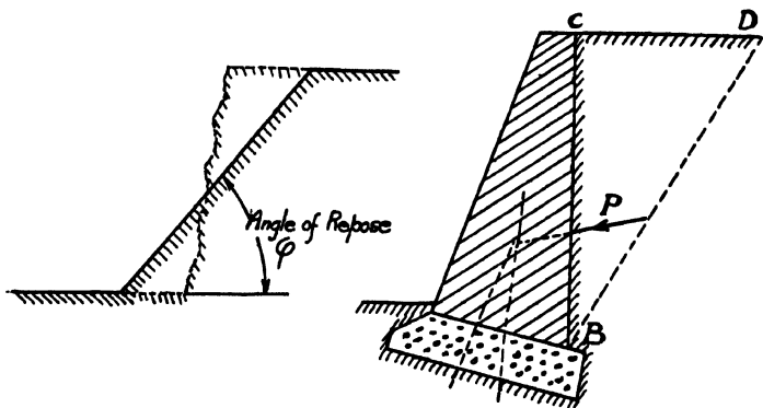
Fig. 181.—Stability of Earthwork.
