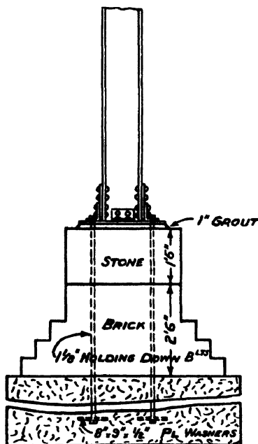
Fig. 221—Brick Pier Foundation.
