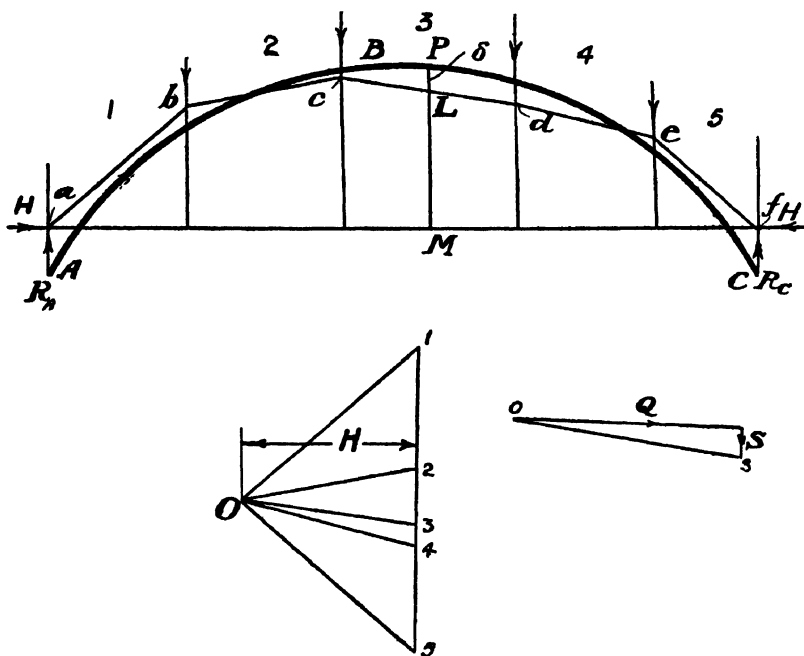
Fig. 164.—Stresses in Arches. Eddy's Theorem.
