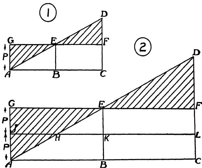
Fig. 11.—Sudden or Dynamic Loading.
