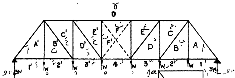
PRATT TRUSS.
