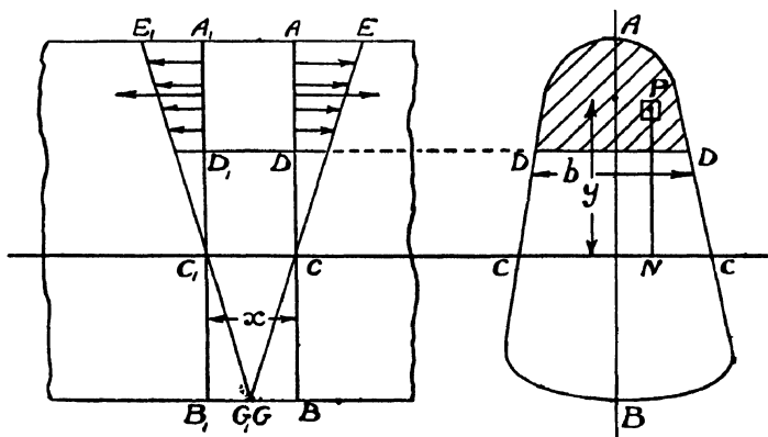
Fig. 116.—Distribution of Shear.
