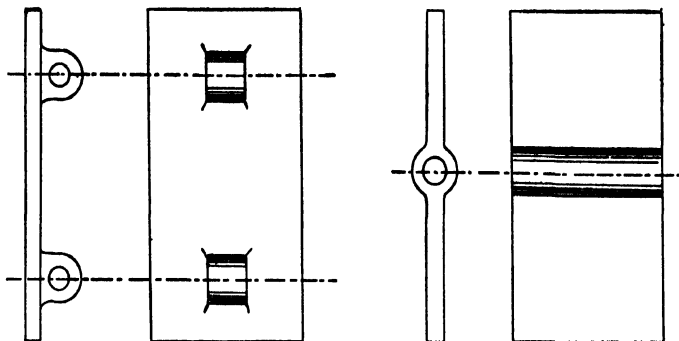
Fig. 228.—Cast-iron Separator for Girders.
