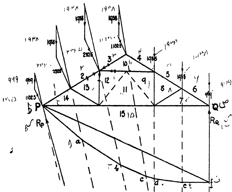
DEAD LOAD AND WIND PRESSURE ON ROOFS
