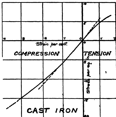
Fig. 2.—Stress-strain Diagrams.
