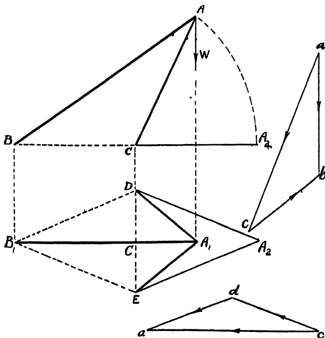
Fig. 152.—Stresses in Shear Legs.
