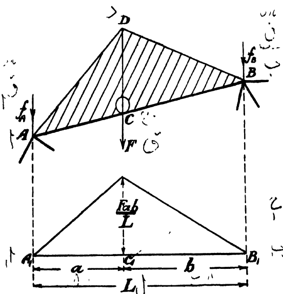
Fig. 136a.—Local Bending in Framed Structures.
