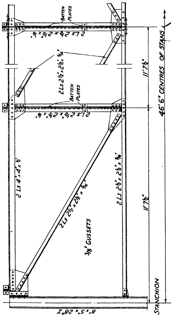
Fig. 242.—Detail of Main Girder for Roof in Fig. 241.
