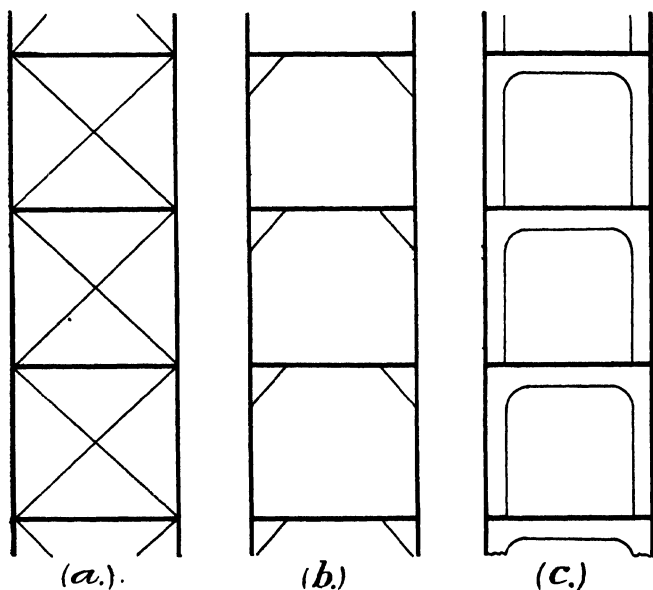
Fig. 226.— Transverse Bracing for Buildings.
