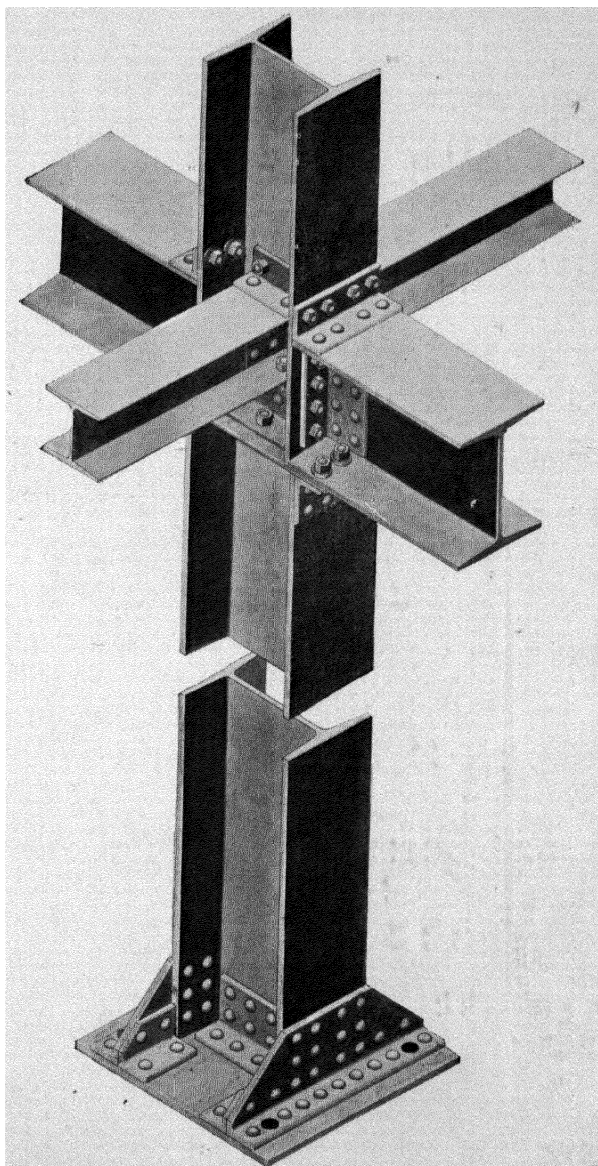
Fig. 216.—Broad Flange Beams and Connections with Column.
