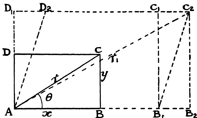
Fig. 8.—Combined Strains.
