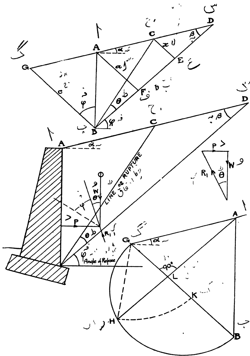
Fig. 187.—Wedge Theory of Earth Pressure.
