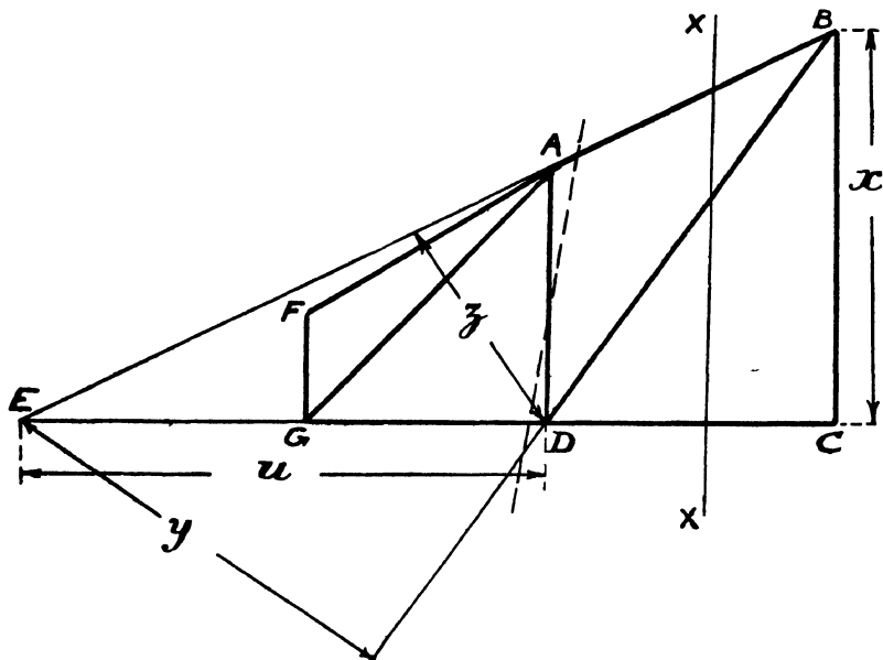
Fig. 139.—The Method of Moments.
