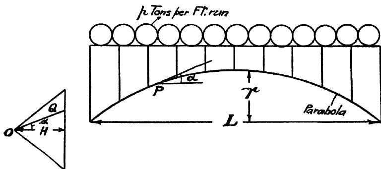
Fig. 165.—Parabolic Arch with Uniform Load.
