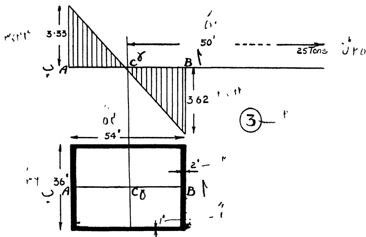
Fig. 79.—Combined Bending and Direct Stress.
