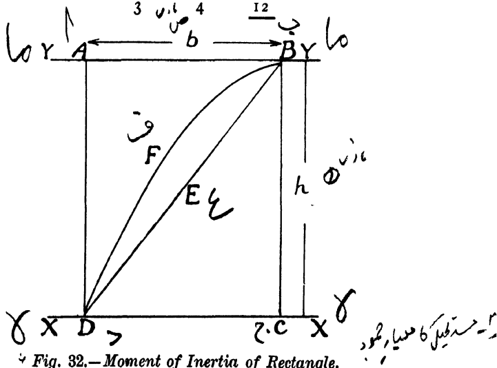
Fig. 32.—Moment of Inertia of Rectangle.
