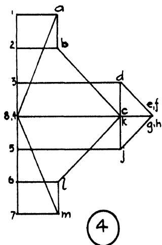
Fig. 148.—Whipple-Murphy Truss.
