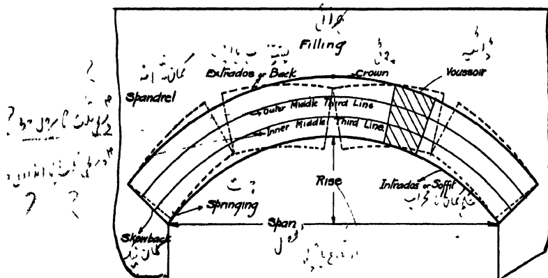
Fig. 194.—Masonry Arches.
