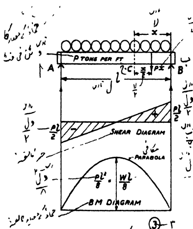
Fig. 54.—Simply-supported Beams.
