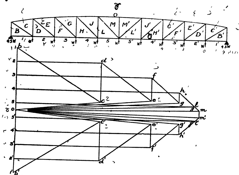
Fig. 130.—Hog Back 'N' Girder.
