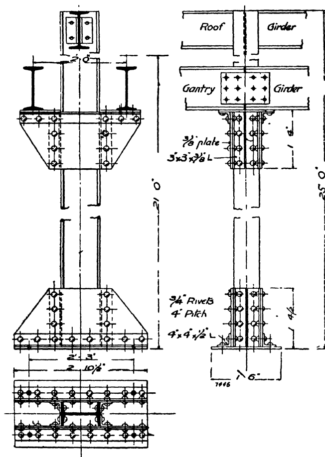
Fig. 218.—Column for Workshop.
