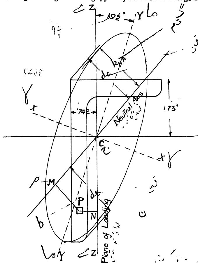
Fig. 76.—Stresses in Asymmetrical Sections.
