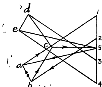
RECIPROCAL DIAGRAM
