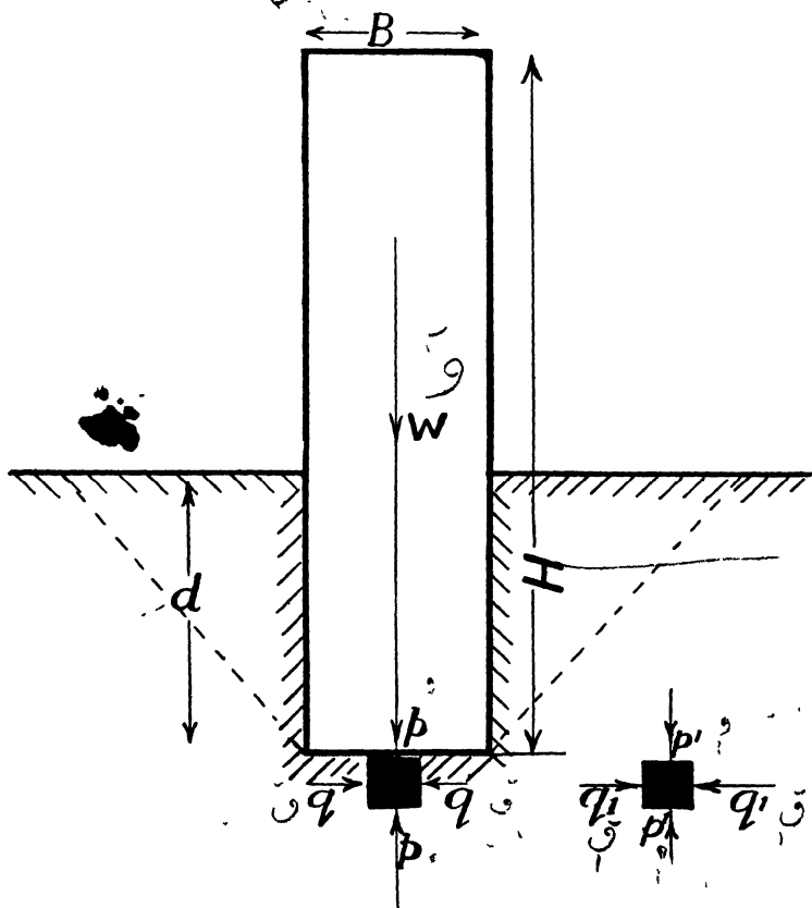
Fig. 186.—Rankine's Theory for Depth of Foundations.
