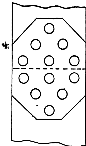
Fig. 44.—Zig-zag Riveting.
