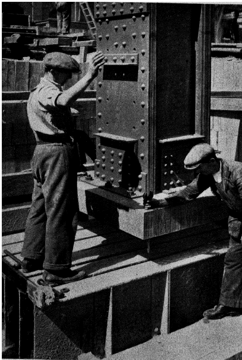
Fig. 217. — Slab Base for Steel Stanchion.
