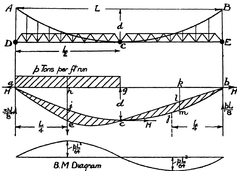
Fig. 160.—Suspension Bridge with Hinged Stiffening Girders.
