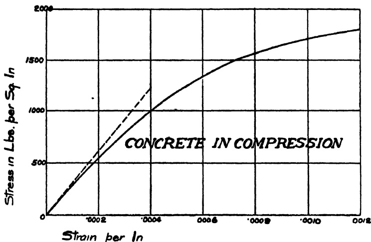
Fig. 3.— Stress-strain Diagram for Concrete in Compression.
