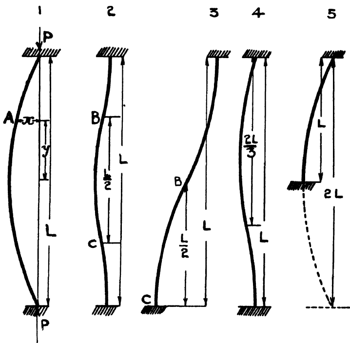
Fig. 153.—Methods of Fixing Ends of Columns.
