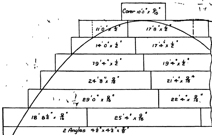
Fig. 264.—Arrangement of Flange Splices.
