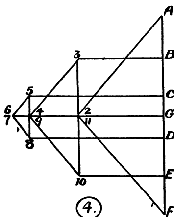
Fig. 147 — Lattice Girder
