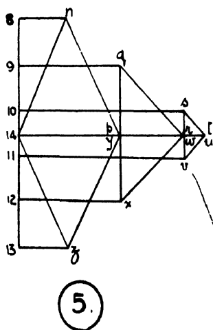
Fig. 148.—Whipple-Murphy Truss.
