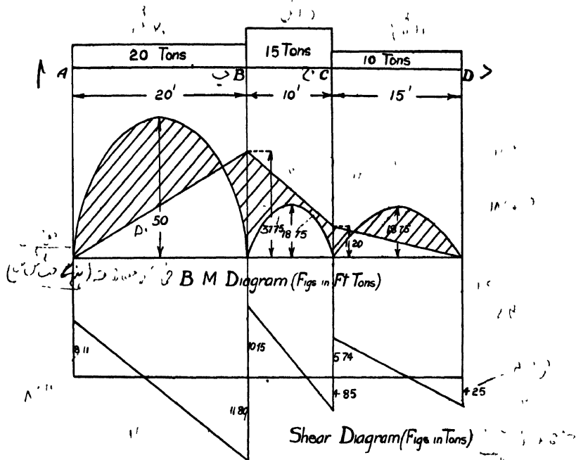
Fig. 105.—Continuous Beam of Three Spans.
