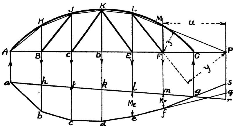
Fig. 141.—Method of Moments using B.M. Diagram.
