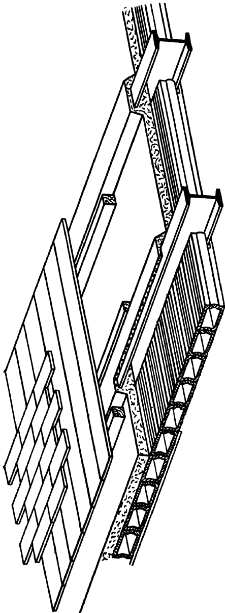
Fig. 236.—Hollow-Tile and Filler-Joist Floor.
