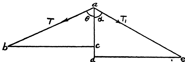
Fig. 159.—Stresses in Anchor Cables.
