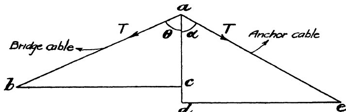
Fig. 158.—Stresses in Anchor Cables.
