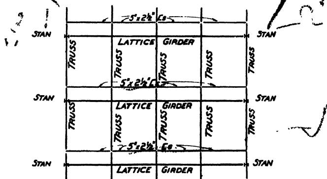
Fig. 243.—Plan showing Arrangement of Trusses and Girders in Part of Fig. 241.
