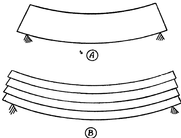
Fig. 115.—Horizontal Shear in Beams.
