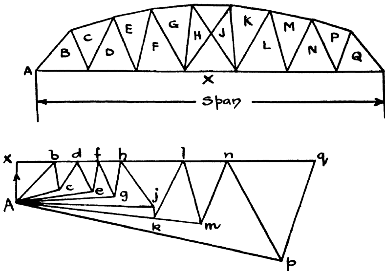
Fig. 146a.—Reciprocal Diagram for Stresses in Diagonals.
