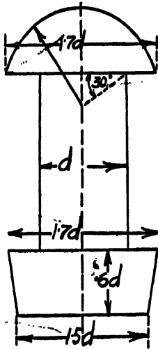
PAN HEAD.
