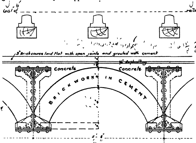
Fig. 255.—'Jack Arch' Floor.
