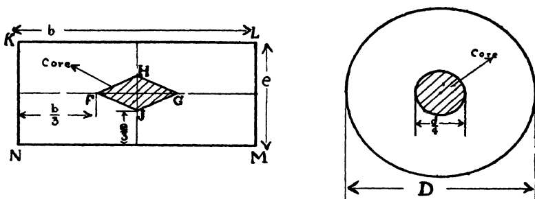
Fig. 175.—Cores of Sections.
