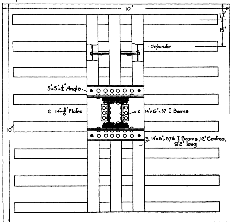
Fig. 222.—Grillage Foundation.
