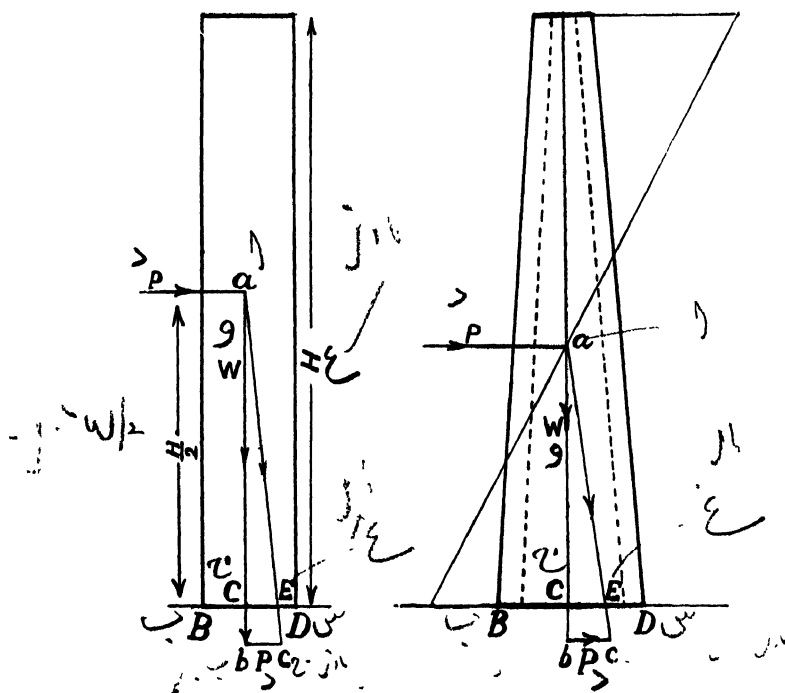
Fig. 192.—Stability of Walls and Chimneys.
