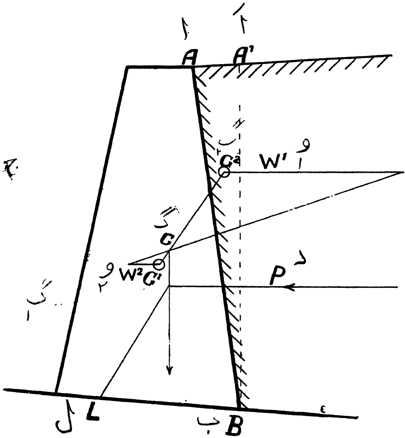
Fig. 188.—Wedge Theory for Retaining Wall with Sloping Back.
