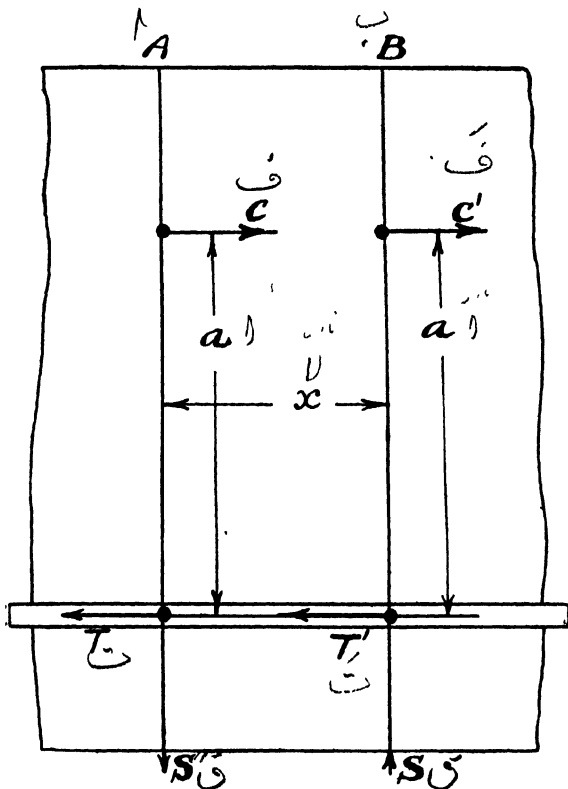
Fig. 207.—Shear Stresses in Reinforced Beams.
