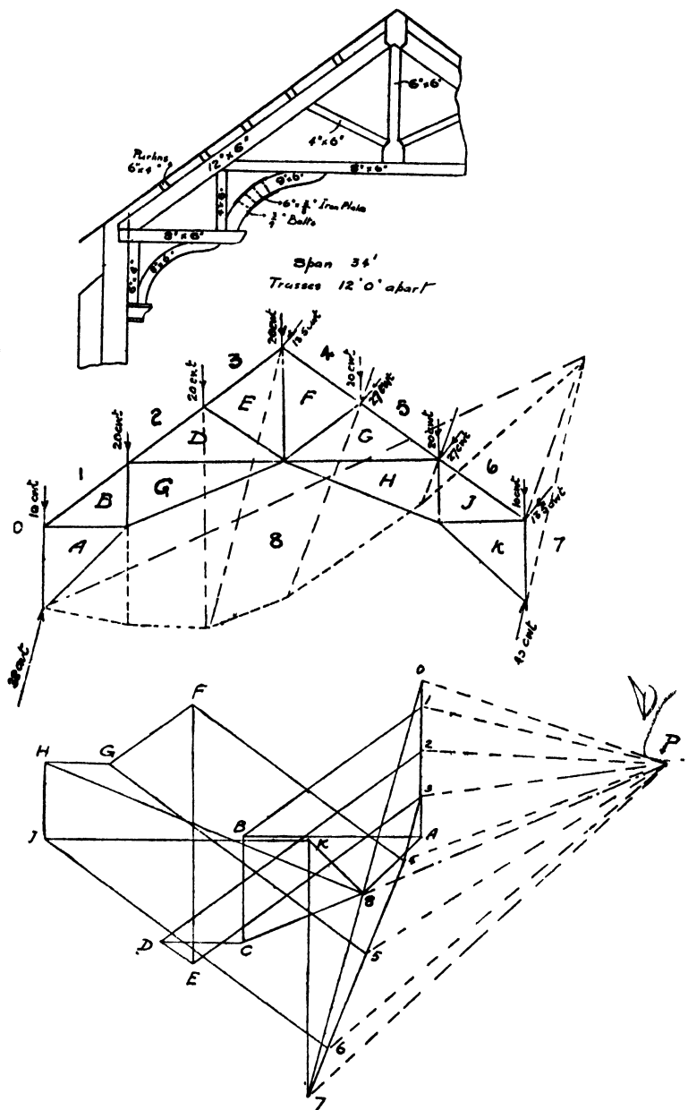
Fig. 249.—Hammer Beam Trusses.
