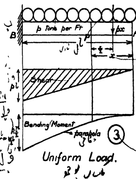
Fig. 52.—B.M. and Shear Diagrams for Cantilevers.
