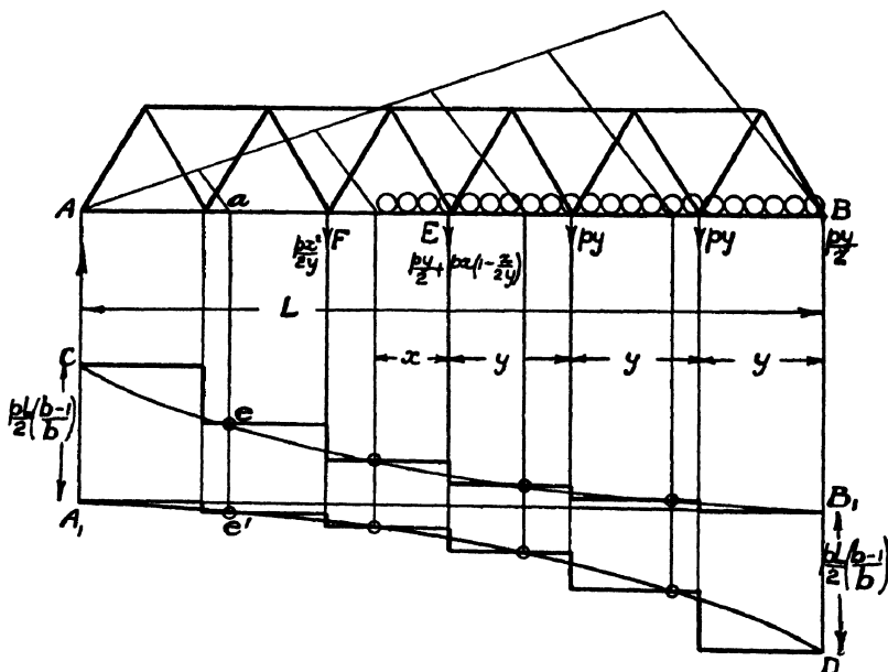
Fig. 146.—Maximum Stresses in Diagonals for Rolling Loads.
