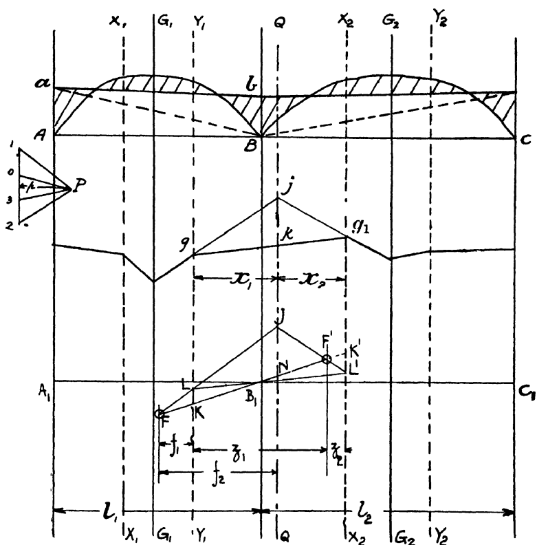
Fig. 108.—Continuous Beams—Fixed Points.
