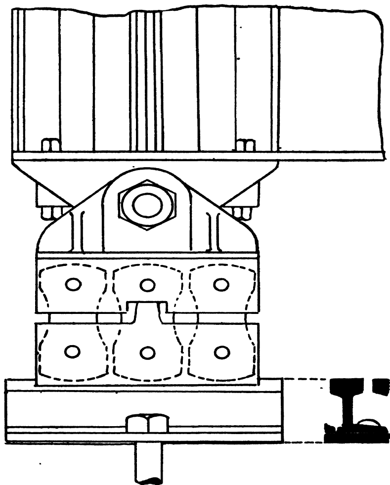
Fig. 276.—Combined Rocker and Roller Bearing.
