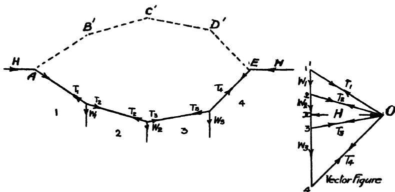
Fig. 156.—Stresses in Loaded Cable.
