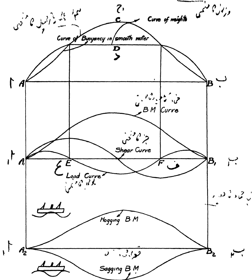
Fig. 59.—B.M. and Shear Curves for Ships.
