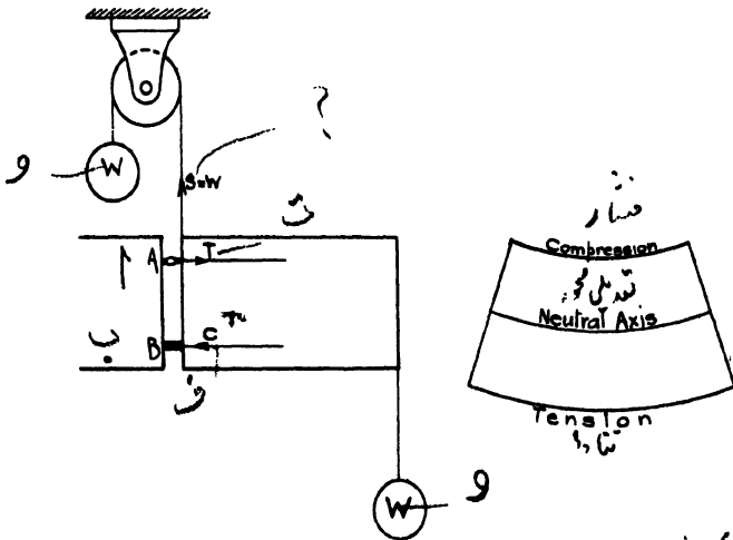
Fig. 68.—Stresses in Beams.
