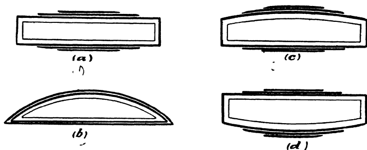
Fig. 261.—Plate Girders of Uniform Strength.
