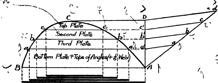
Fig. 262.—Curtailment of Flange Plates.
