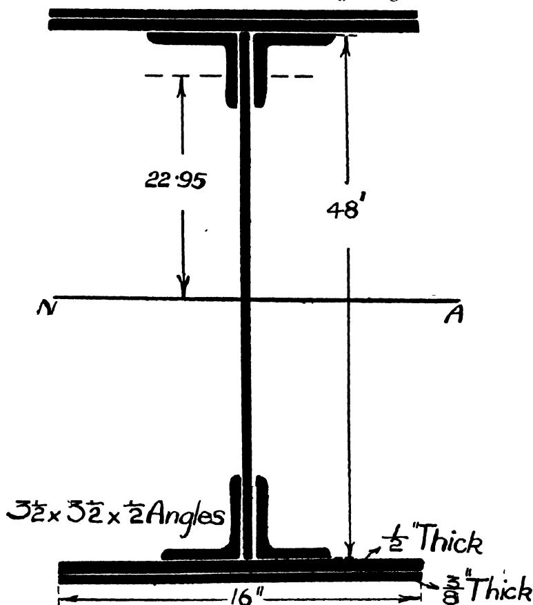
Fig. 280.—Plate Girder Section.
