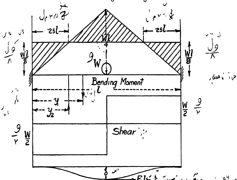
Fig. 96.—Fixed Beam, with Central Load.
