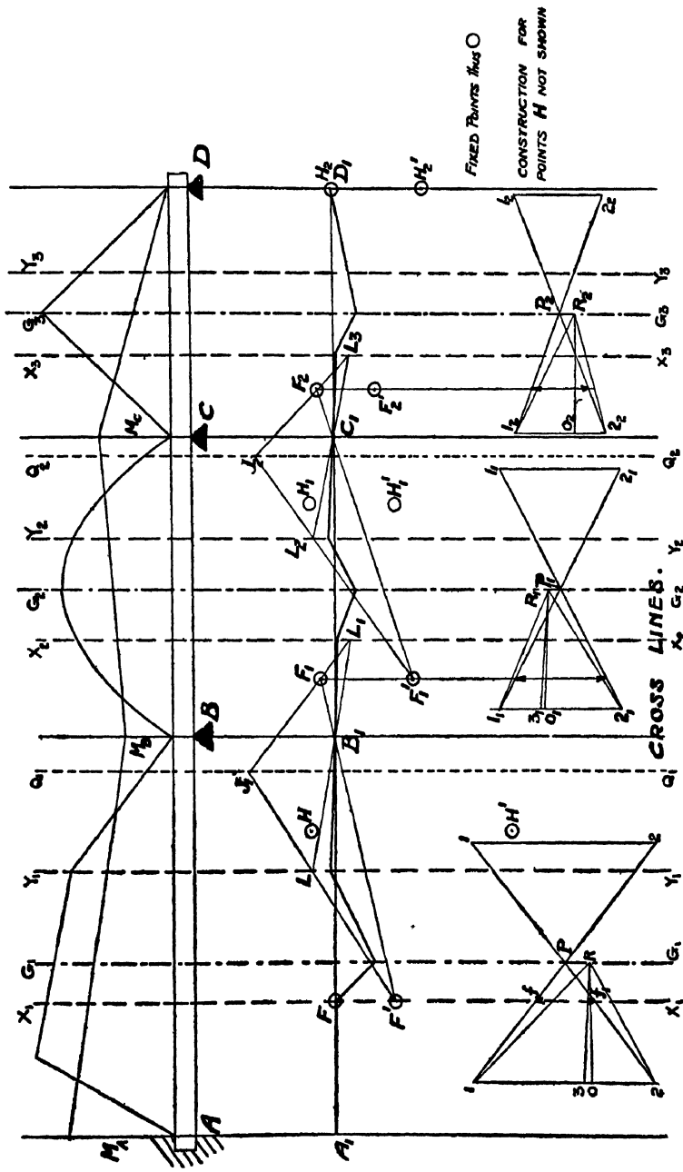
Fig. 109.—Graphical Investigation of Continuous Beam of three Spans.
