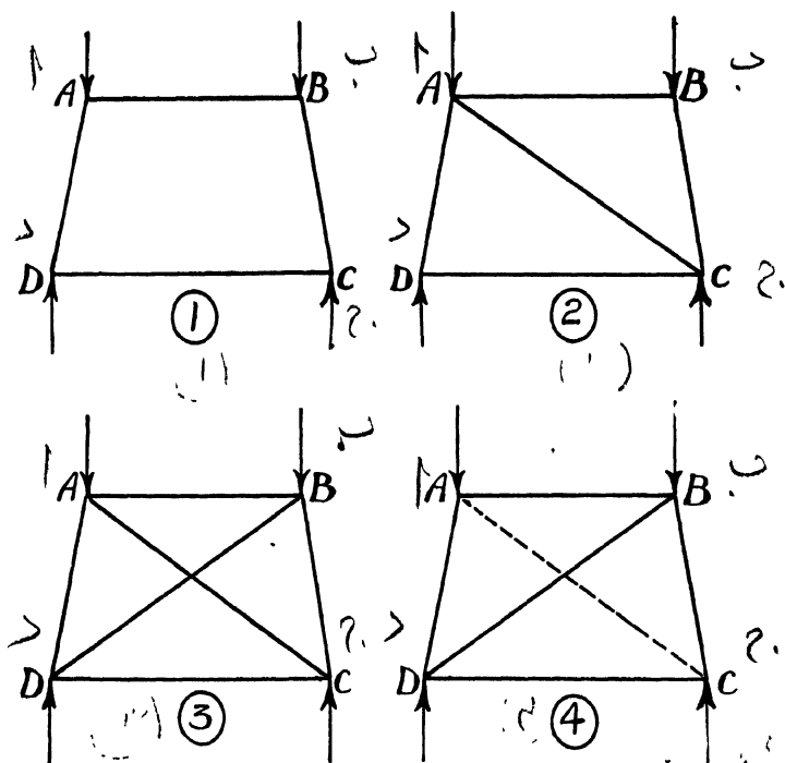
Fig. 122.—Kinds of Framed Structures.
