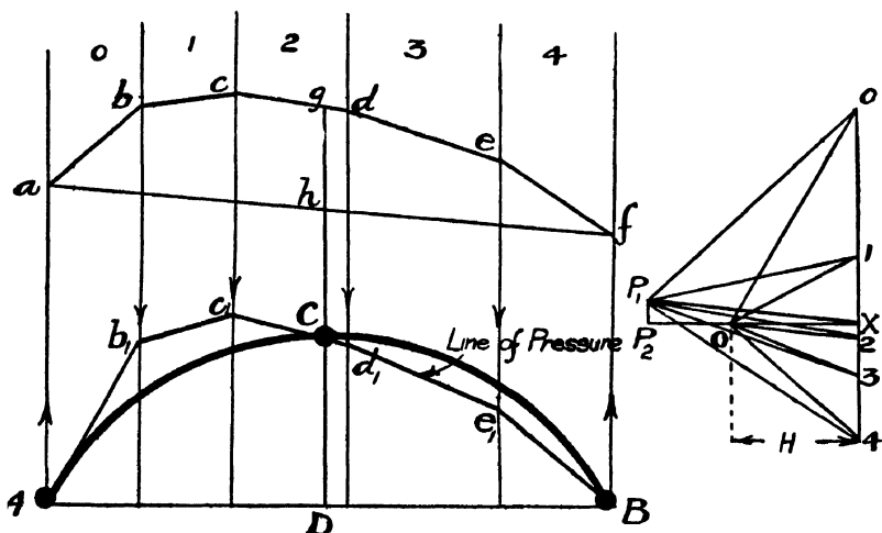
Fig. 167.—Three-pinned Arch.
