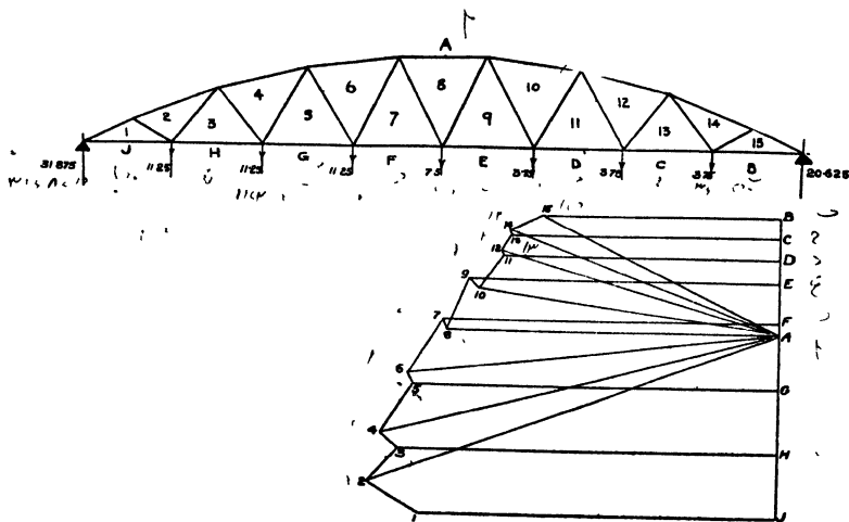
Fig. 129.—Bowstring Truss with Live Load on Half Span.
