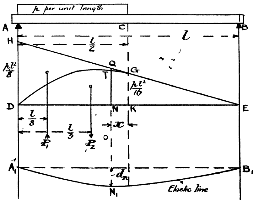
Fig. 93A.—Deflections of Beams.
