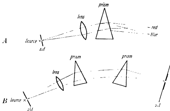
Figure 15. Spectrometers
