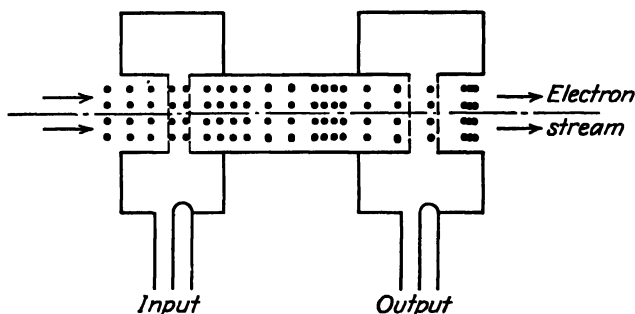
FIG. 67.—A two-gap velocity modulation amplifier tube using two resonant cavities.
