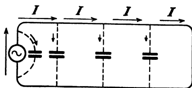
FIG. 35. —Even at low frequency the loop current must be nonuniform, though perhaps very slightly.
