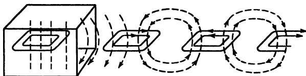
FIG. 64.—With the cavity wall removed, a coupling would exist to outside space because of the mutual induction of electric and magnetic fields.
