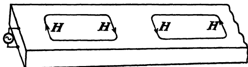
FIG. 100.—Two of the magnetic field lines H on the inside of the rectangular wave guide.
