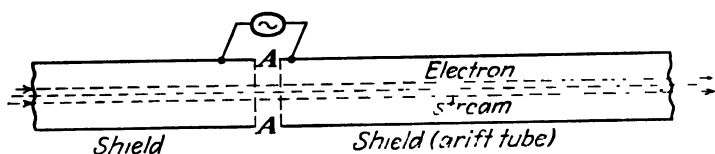
FIG. 20.- An electron stream can be velocity-modulated by applying alternating voltage across a gap in the stream's shield.
