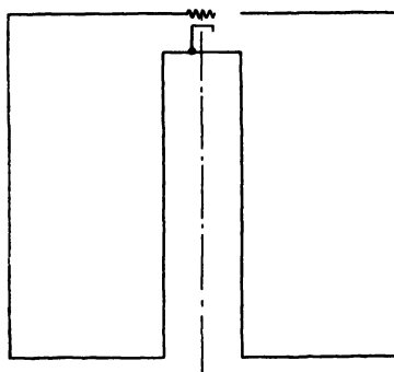
FIG. 76. A shorted length of coaxial line connected between grid and cathode of an electron tube.
