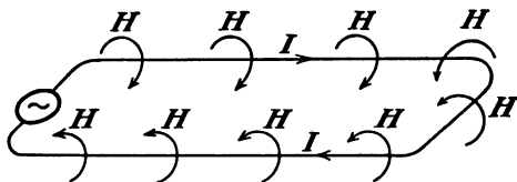
FIG. 30.—The low-frequency picture includes a uniform loop current surrounded by a magnetic field everywhere in phase with the current.
