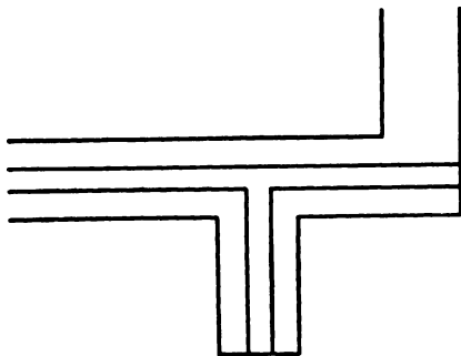
FIG. 111.—Typical microwave systems consist of much discontinuous plumbing.
