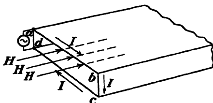
FIG. 96.—To maintain the cross-sectional a.c. voltage difference, some longitudinal a.c. magnetic field H and transverse side current I must exist.
