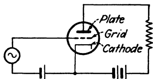
FIG. 16.—A change of grid-cathode voltage causes a change of current in the output resistor.
