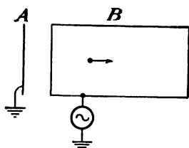
FIG. 18. —The electron inside the shield B does not notice the effect of the varying voltage between B and A .
