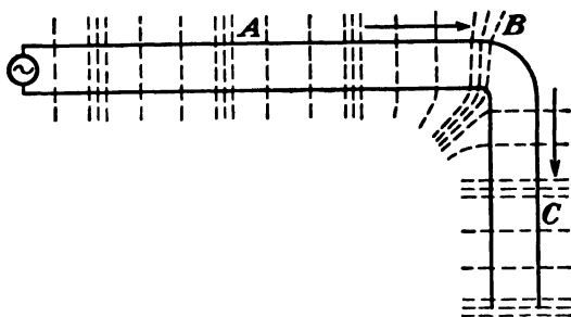
FIG. 74.--Some of the power is guided around the turn by the open line.
