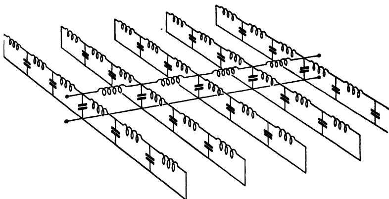
FIG. 103.—A better representation of the wave-guide-type wave that discloses the cross-sectional as well as longitudinal variations.
