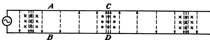
FIG. 80.—A longitudinal section of the line of Fig. 79. The electric field lines are perpendicular to the plates. The magnetic field lines (dots and crosses) are perpendicular to the electric field and parallel to the plates.
