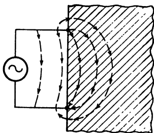
FIG. 7.—A source connected directly to the conducting slab tries to produce an electric field in the conductor.
