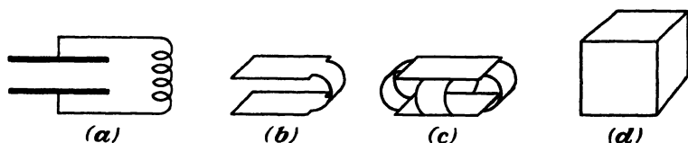
FIG. 48.—A progression from a common parallel LC circuit to a resonant cavity.
