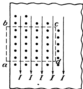
FIG. 10.—Cross section of part of the conductor. The arrows represent current flow parallel to the plane of the section. The dots represent magnetic flux lines caused by the current, these lines being perpendicular to the plane.
