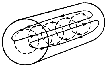
FIG. 62.—An oscillation mode in which the electric-field lines (dotted) also form closed loops.
