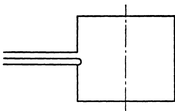
FIG. 112.—The current in the loop excites various modes in the cavity; the mode near resonance will have greatest magnitude.
