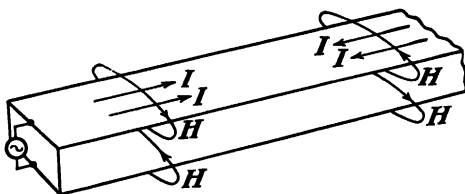
FIG. 99.— A few of the magnetic field lines H in the transmission-line-type wave at one instant.
