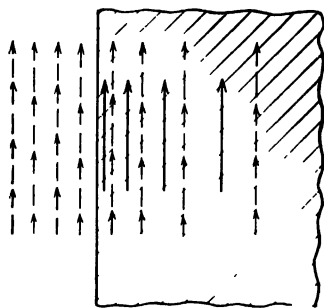
FIG. 12.—In an imperfect conductor, the electric field (dotted arrows) does not have to be zero inside the conductor, but both the electric field and the current density (solid arrows) fall off rapidly with penetration into the conductor at very high frequencies.
