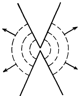
FIG. 117.—The outgoing principal wave on the antenna of Fig. 116.
