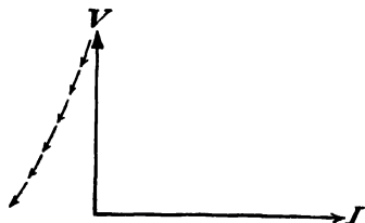
FIG. 36.—Assuming retardation and a uniform loop current I with a 90-deg. leading voltage V , the vector diagram refuses to balance.
