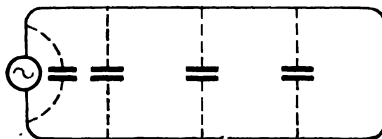
FIG. 34.—Charging current effects are represented by the distributed capacitance.
