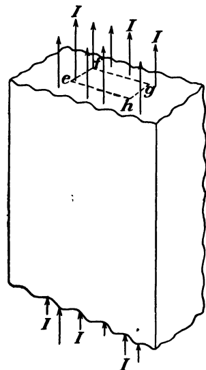
FIG. 11.—If there were current flow (indicated by the arrows) inside the conductor, magnetic field would have to exist around all or part of the loop efghe which links the current.
