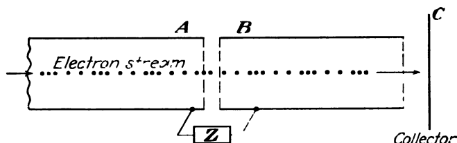
FIG. 26.—A current-density-modulated electron stream will produce a.c. currents in an impedance Z connected between the two cylinders through which the stream passes.
