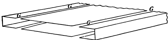
FIG. 94.—A distributed single-turn inductance is applied in parallel with the conductors of the line.
