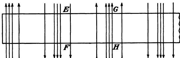
FIG. 81.--The two-plate transmission line from a plan view, showing the magnetic field lines.
