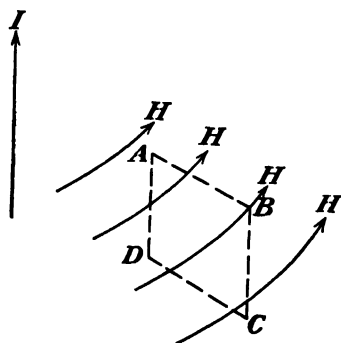
FIG. 38.—A rectangular loop ABCD whose plane passes through I is linked by magnetic field H .
