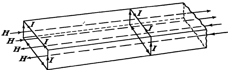
FIG. 105.—At the cut-off frequency, all the current I is transverse. The magnetic and electric fields and the current have phase angles that are independent of distance along the guide; the phase velocity is infinite.
