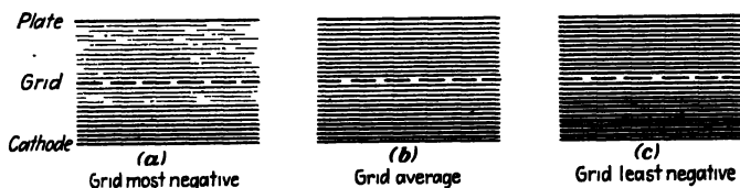
FIG. 24.— Instantaneous space-charge densities in a triode at low frequency.
