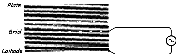
FIG. 23.-Very high frequency voltage applied between grid and cathode results in density waves in the space charge.
