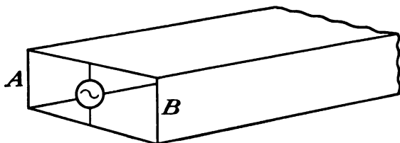
FIG. 91.—A wave guide of rectangular cross section.
