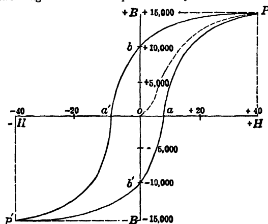
FIG. 119.—Hysteresis curve.
