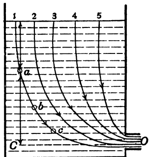
FIG. 60.—Stream lines of flow.
