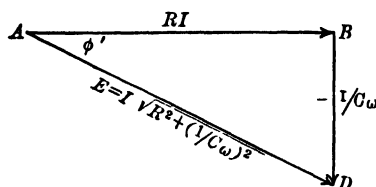
FIG. 139.—E.m.f. diagram.
