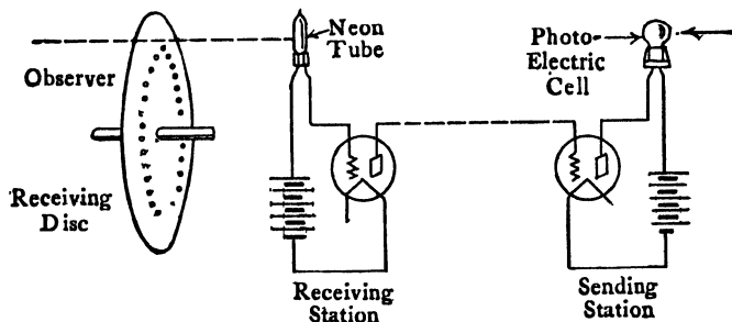
FIG. 206.—Television set-up.
