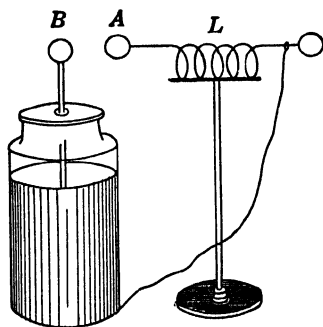
FIG. 199.—Oscillatory discharge.
