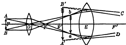
FIG. 191.—Compound microscope.
