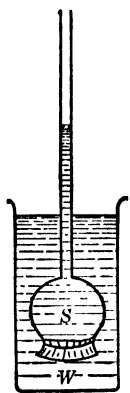
FIG. 72.—Osmotic-pressure apparatus.
