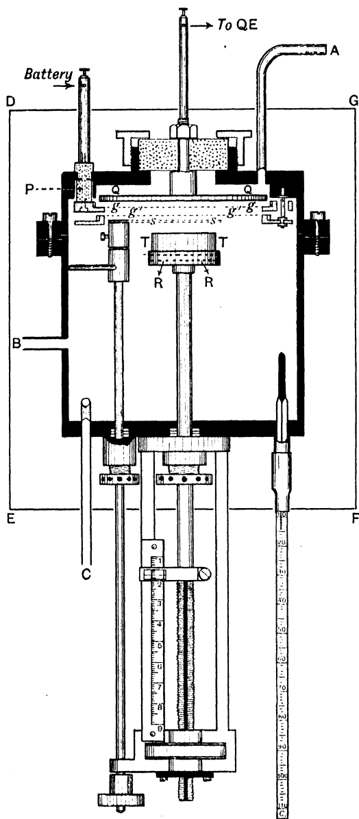
FIG. 6.—Apparatus for finding the range of \alpha rays.
