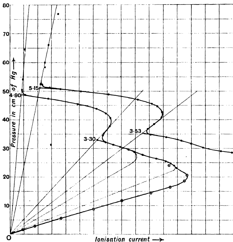
FIG. 27.—Ionisation curves of argon (upper curve) and air (lower curve); apparatus of Fig. 26.
