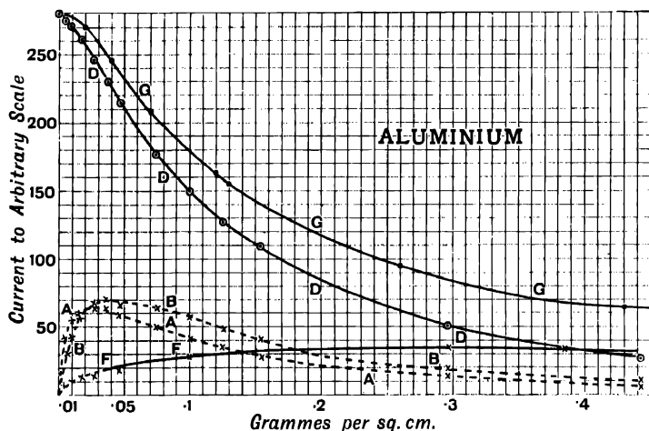
FIG. 40.—Cathode ray current from aluminium screens of varying weight.
