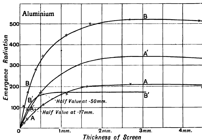
FIG. 47.—Absorption of Secondary \beta rays in Aluminium.
