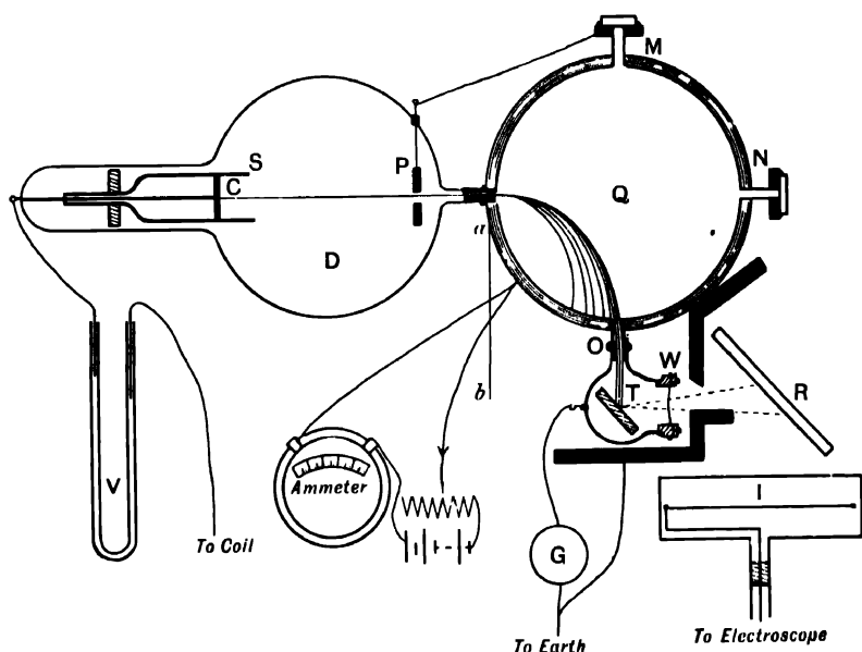
FIG. 57.—Whiddington's experiment.
