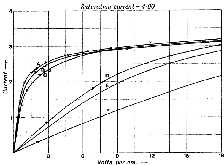
FIG. 29.—Curves showing the relation between the potential gradient and the ionisation current in air in various cases.
