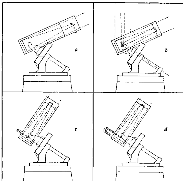
FIG. 16. Four Arrangements of the GO-Tinch Reflector of the Mt. Wilson Observatory
