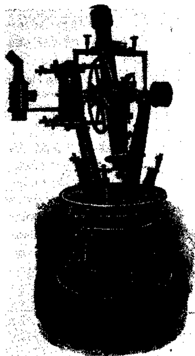
FIG. 31. A 5-Inch Altazimuth
