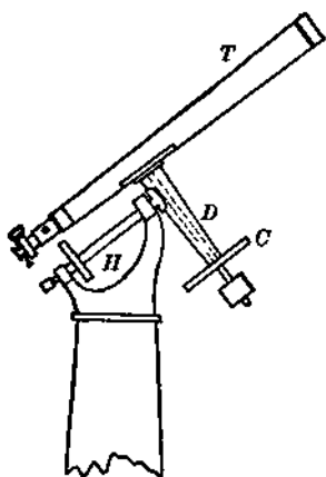
FIG. 17. The Equatorial Mounting
