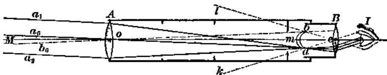
FIG. 12. The Simple Refracting Telescope
