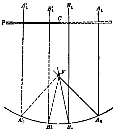
FIG. 35A. The Schmidt Camera
