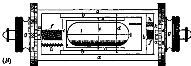
FIG. 32. The Filar Position Micrometer
