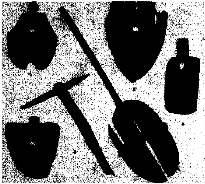
1, Oak shovel from stream-work, near Alfarmtn, 2 Ironshod shovel, 16th cent, found in stream work at Luxulyan, J, oak pickaxe found in peat moss at Rosetague, Bt Just, 4 and 5, oak shovel from stream-work on the Goss Moor and near Lanivet respectively, 6, spoon shovel hewn out of one piece of oak, from Cainou Stream
