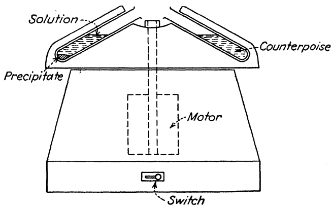
FIG. 4.—Diagram of centrifuge.
