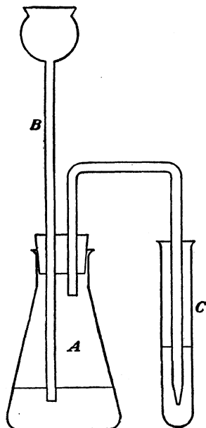
FIG. 13.—Apparatus for detecting \text{CO}_2 (macro scale).
