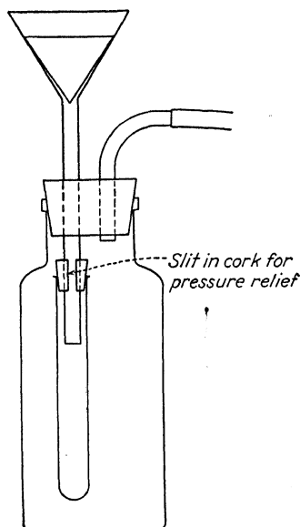
FIG. 3.—Filtration on a micro scale, using suction.
