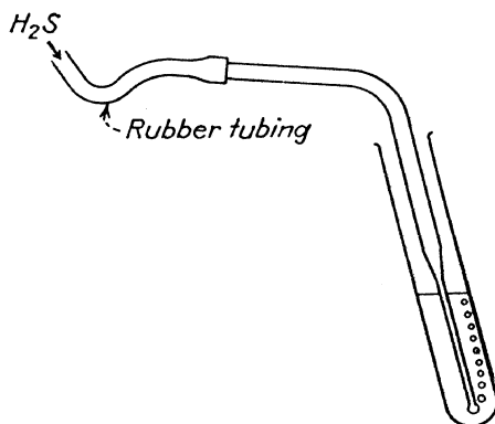
FIG. 6.—Precipitation by H_2S (micro method).
